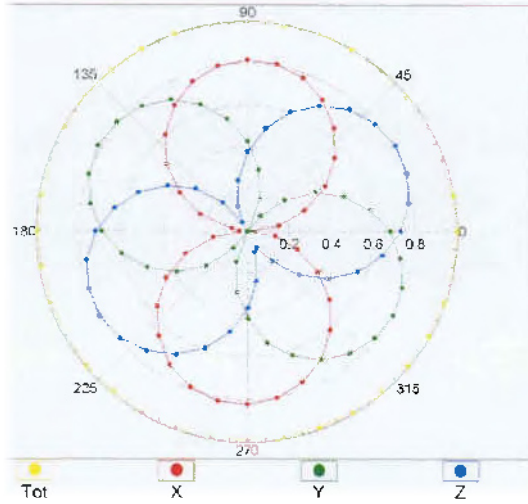
f=600 MHz,TEM
