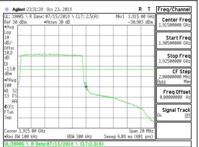
LTE B25 10MHz 16QAM High Channel RB50-0
