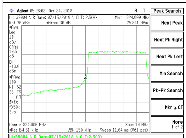
LTE B5 5MHz QPSK Low Channel RB25-0
