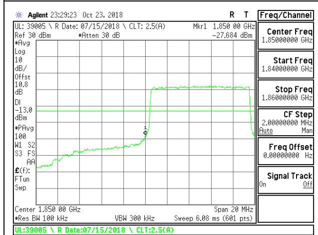
LTE B25 10MHz 16QAM Low Channel RB50-0
