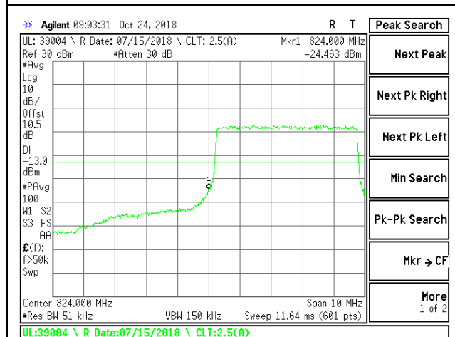
LTE B26 5MHz 16QAM Low Channel RB25-0
