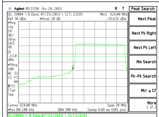
LTE B5 10MHz 16QAM Low Channel RB50-0
