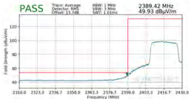
Plot 7-121. Radiated Restricted Lower Band Edge Measurement SISO ANT2 (Average)
