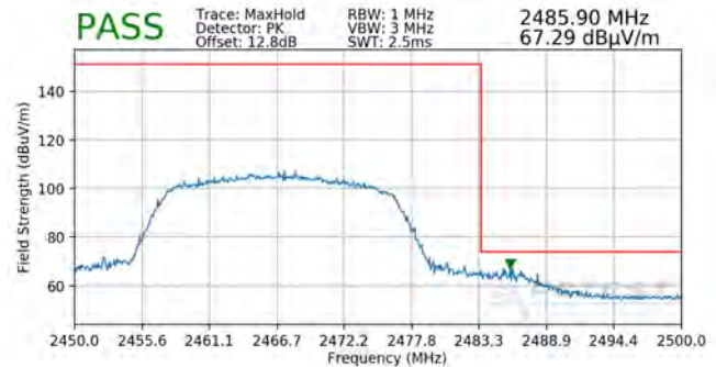
Plot 7-110. Radiated Restricted Band Edge Measurement SISO ANT1 with WCP (Peak)
