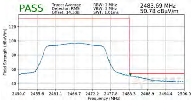
Plot 7-105. Radiated Restricted Upper Band Edge Measurement SISO ANT1 (Average)
