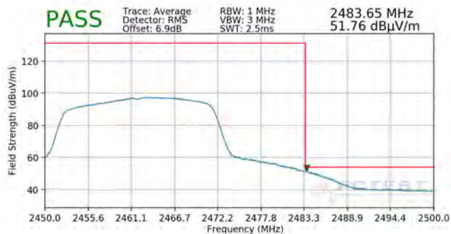
Plot 7-113. Radiated Restricted Upper Band Edge Measurement SISO ANT2 (Average)
