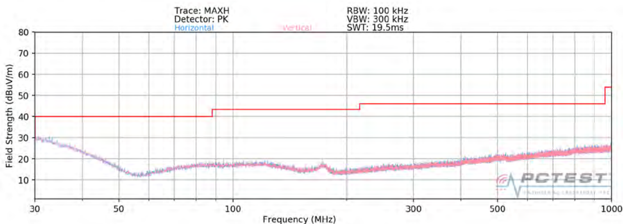
Plot 7-371. Radiated Spurious Plot below 1GHz (Dual Band Simult. Tx)
