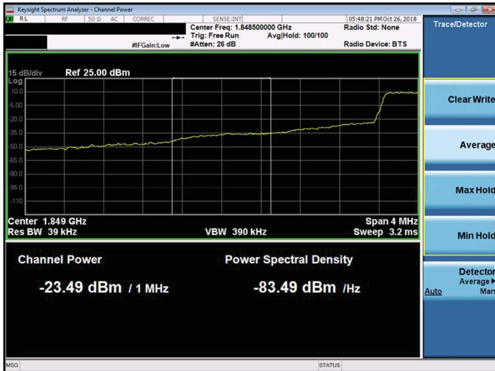
Plot 7-345. Lower Extended Band Edge Plot (Band 25/2 - 1.4MHz QPSK - Full RB Configuration)
