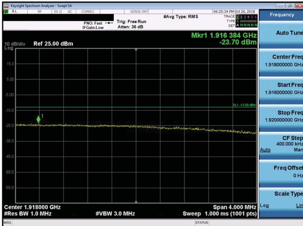
Plot 7-373. Upper Extended Band Edge Plot (Band 25 - 15.0MHz QPSK - Full RB Configuration)
