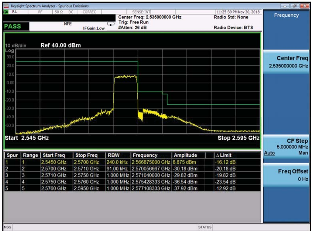
Plot 7-389. Upper ACP Plot (Band 7 ANT B - 5.0MHz QPSK - Full RB Configuration)
