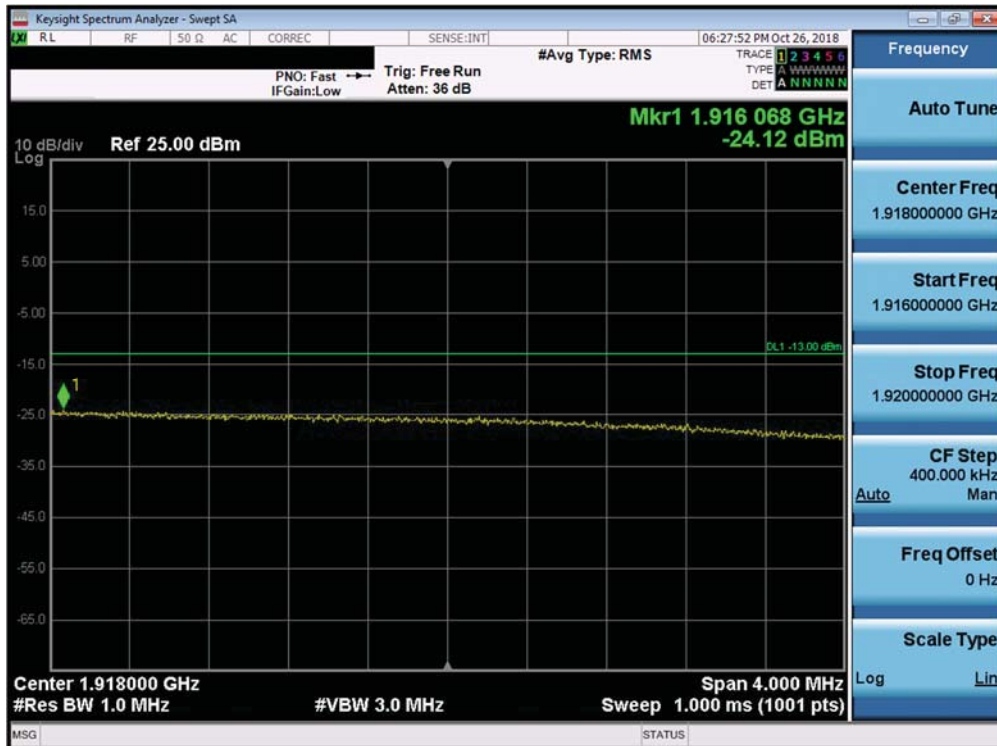
Plot 7-379. Upper Extended Band Edge Plot (Band 25 - 20.0MHz QPSK - Full RB Configuration)
