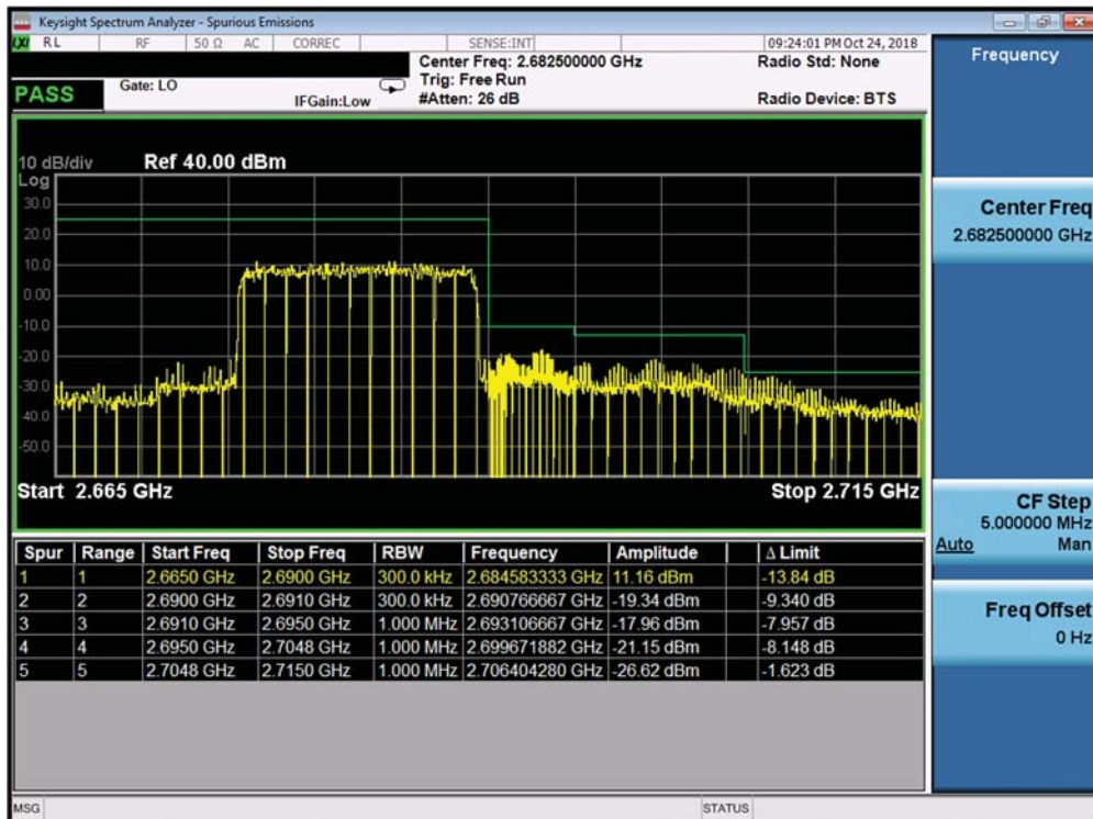
Plot 7-409. Upper ACP Plot (Band 41 PC2 - 15.0MHz QPSK - Full RB Configuration)
