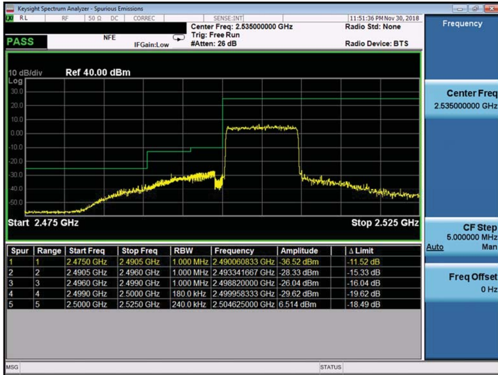
Plot 7-390. Lower ACP Plot (Band 7 ANT B - 10.0MHz QPSK - Full RB Configuration)
