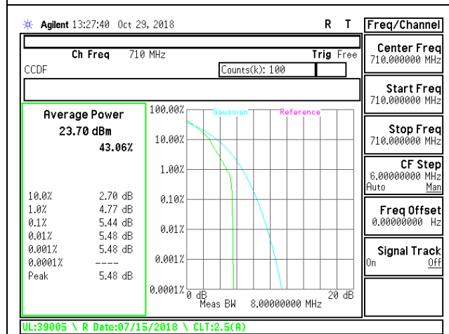
LTE B17 10MHz QPSK Mid Channel
