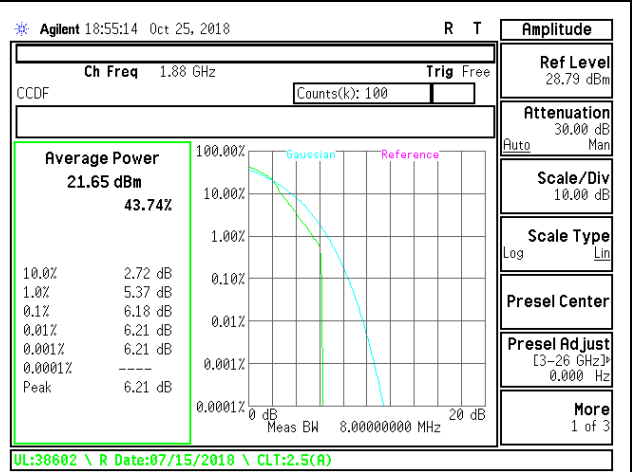
LTE B2 3MHz 16QAM Mid Channel
