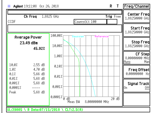
LTE B25 5MHz QPSK Mid Channel
