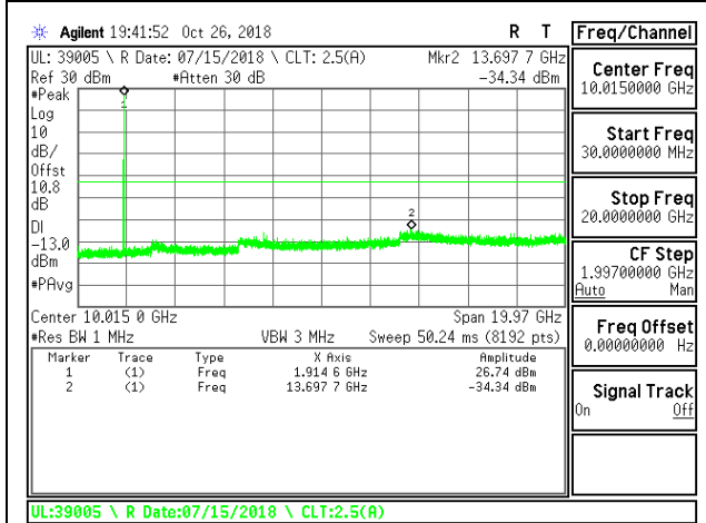
LTE B25 1.4MHz QPSK High Channel RB1-0
