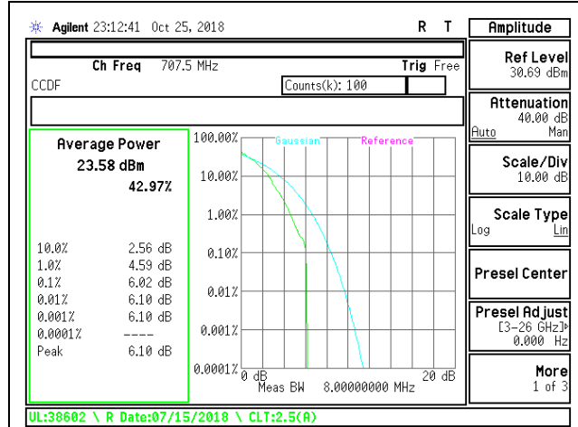
LTE B12 1.4MHz QPSK Mid Channel
