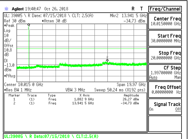
LTE B25 1.4MHz QPSK Mid Channel RB1-0
