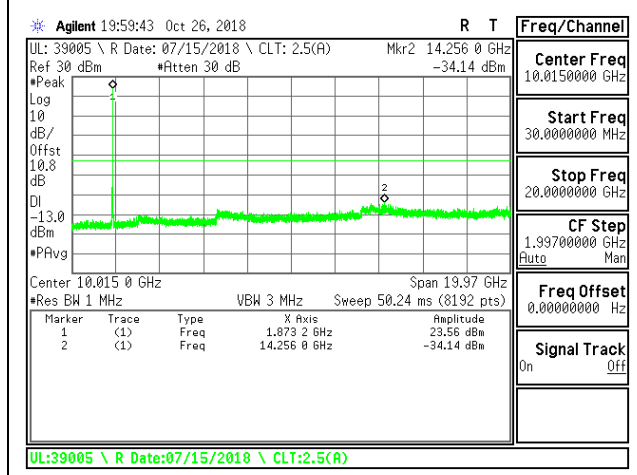
LTE B25 20MHz 16QAM Mid Channel RB1-0
