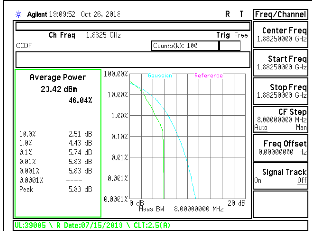
LTE B25 3MHz QPSK Mid Channel
