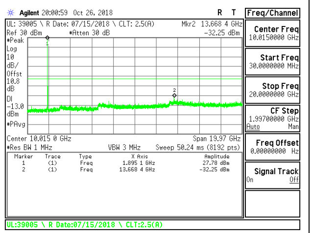
LTE B25 20MHz 16QAM High Channel RB1-0
