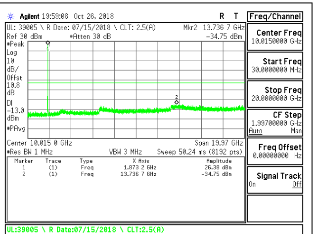
LTE B25 20MHz QPSK Mid Channel RB1-0
