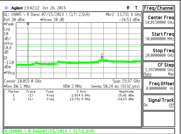
LTE B25 1.4MHz 16QAM High Channel RB1-0
