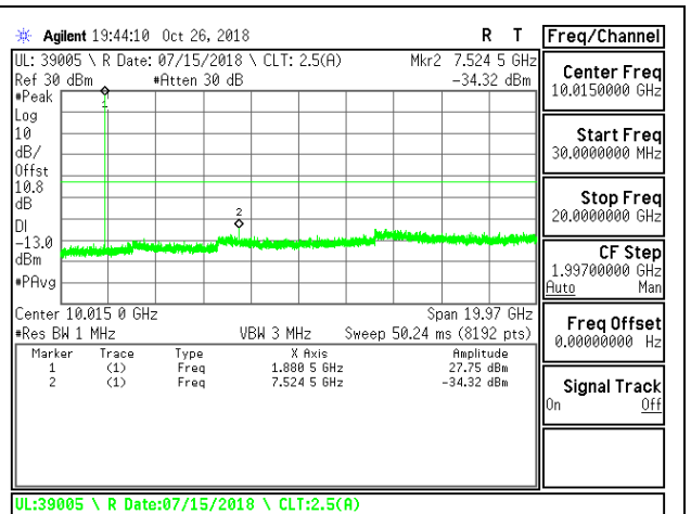
LTE B25 3MHz QPSK Mid Channel RB1-0
