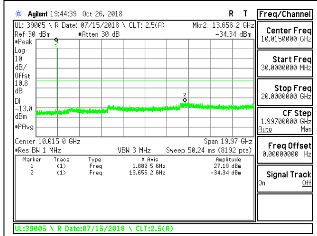
LTE B25 3MHz 16QAM Mid Channel RB1-0
