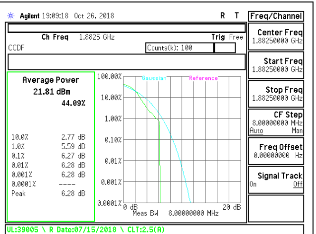
LTE B25 1.4MHz 16QAM Mid Channel
