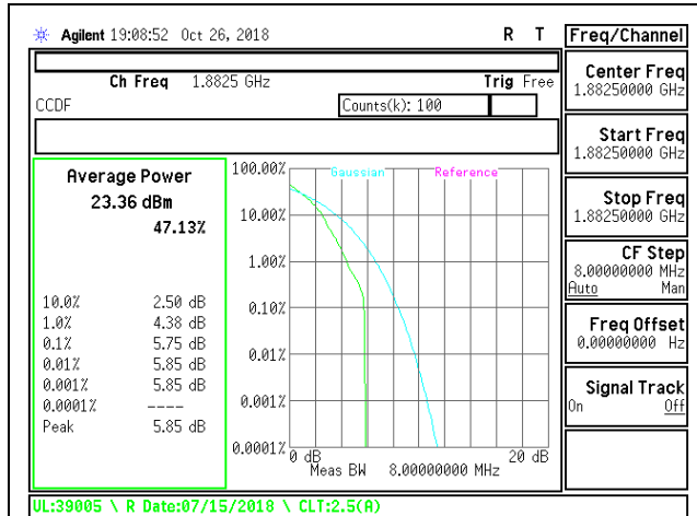
LTE B25 1.4MHz QPSK Mid Channel
