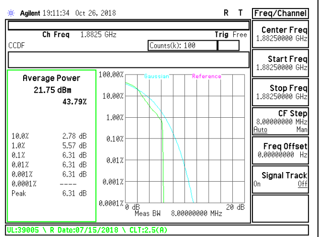
LTE B25 5MHz 16QAM Mid Channel
