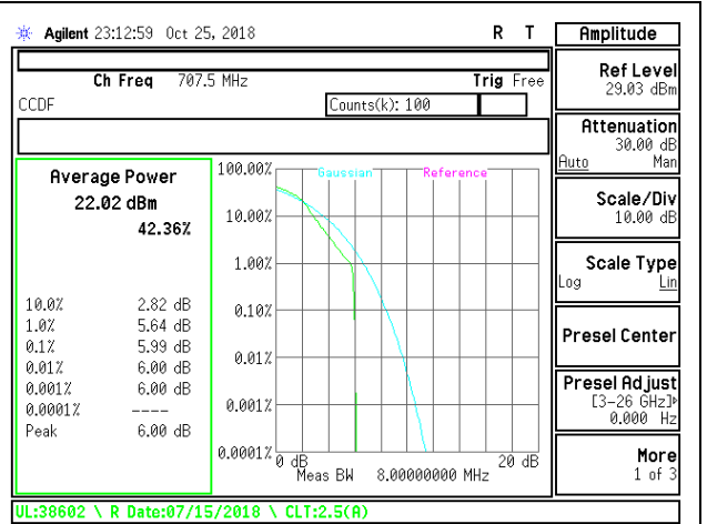
LTE B12 1.4MHz 16QAM Mid Channel
