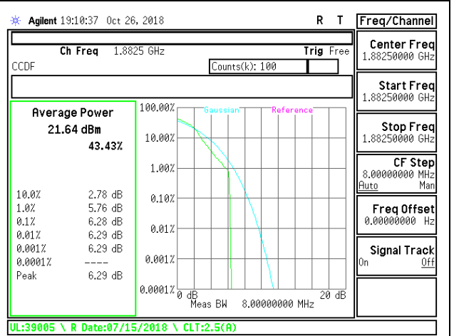
LTE B25 3MHz 16QAM Mid Channel
