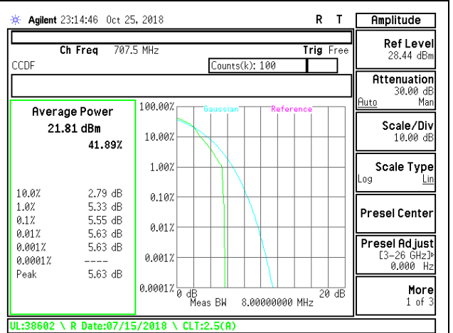
LTE B12 5MHz 16QAM Mid Channel
