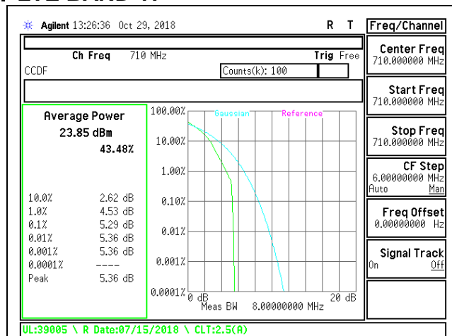
LTE B17 5MHz QPSK Mid Channel
