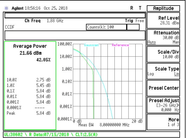
LTE B2 5MHz 16QAM Mid Channel
