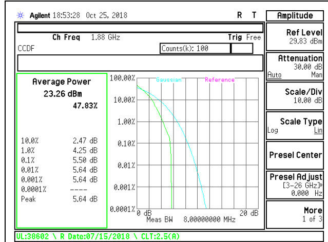
LTE B2 1.4MHz QPSK Mid Channel
