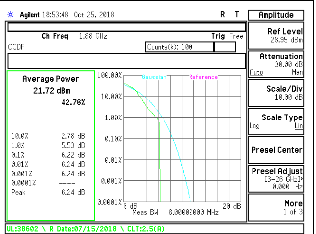
LTE B2 1.4MHz 16QAM Mid Channel
