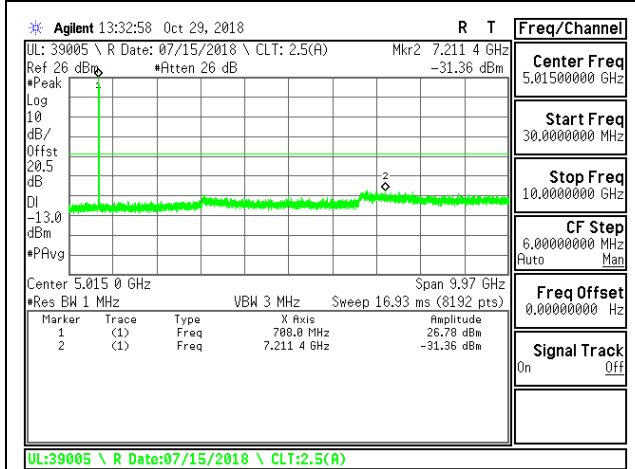
LTE B17 5MHz 16QAM Mid Channel RB1-0
