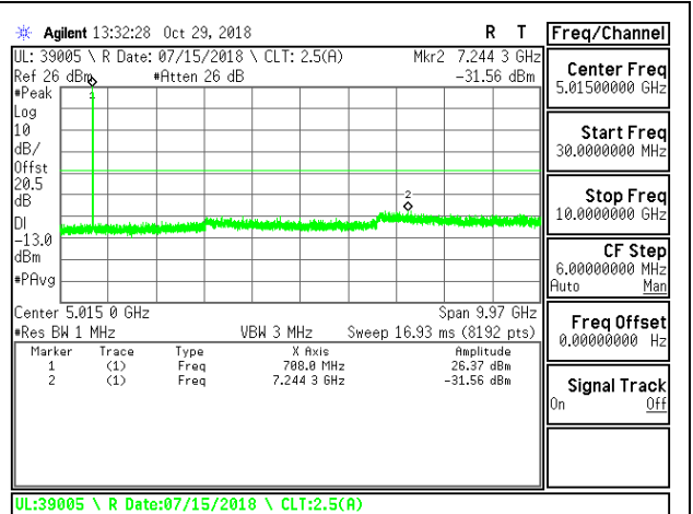
LTE B17 5MHz QPSK Mid Channel RB1-0
