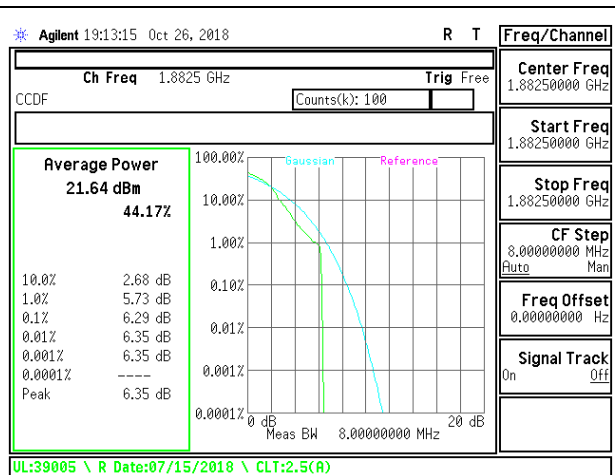
LTE B25 15MHz 16QAM Mid Channel
