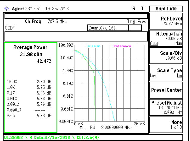
LTE B12 3MHz 16QAM Mid Channel
