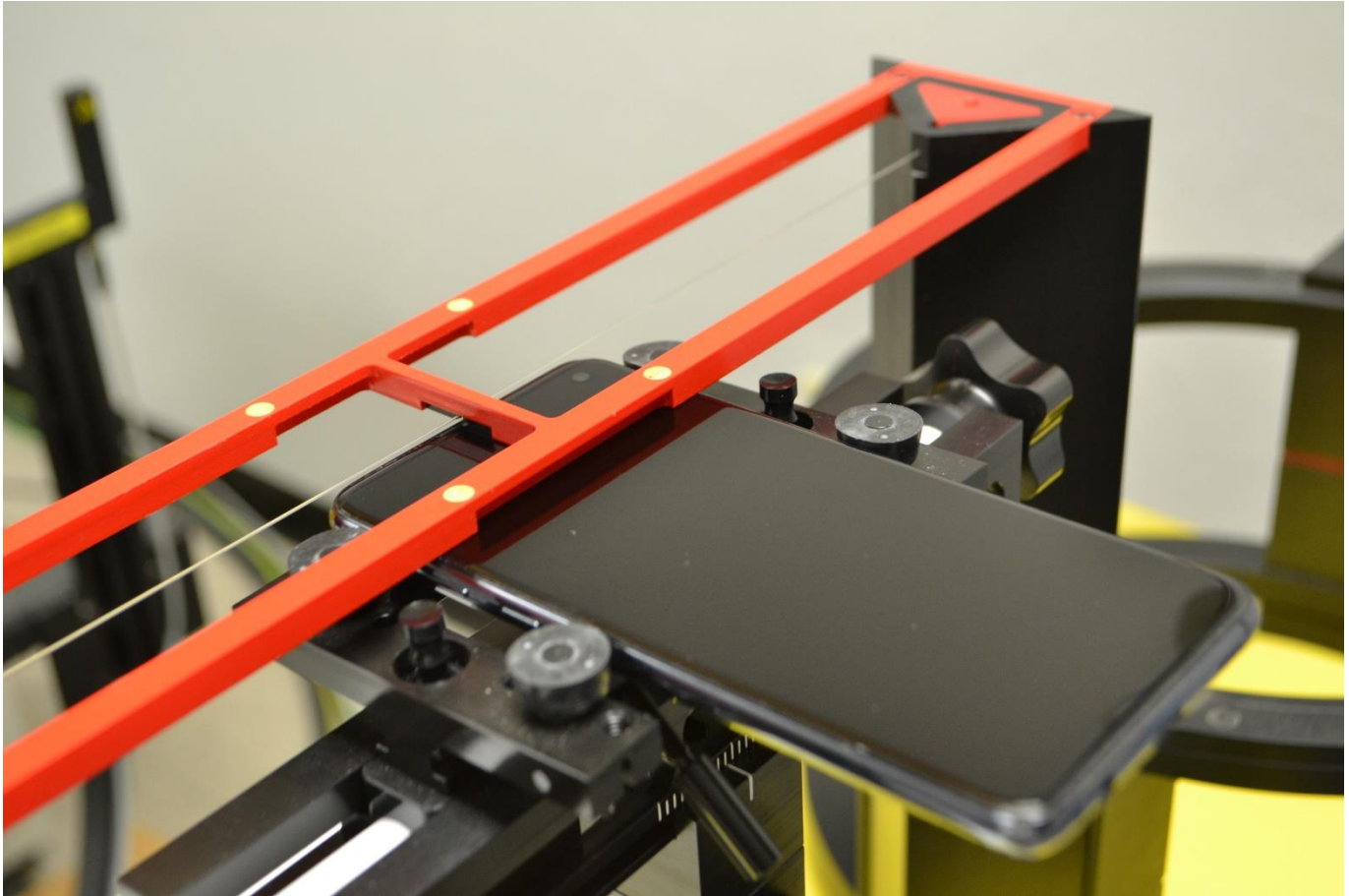
Setup Photo Front View of the DUT
