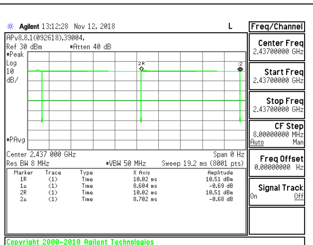
DUTY CYCLE 802.11b MODE Chain 1
