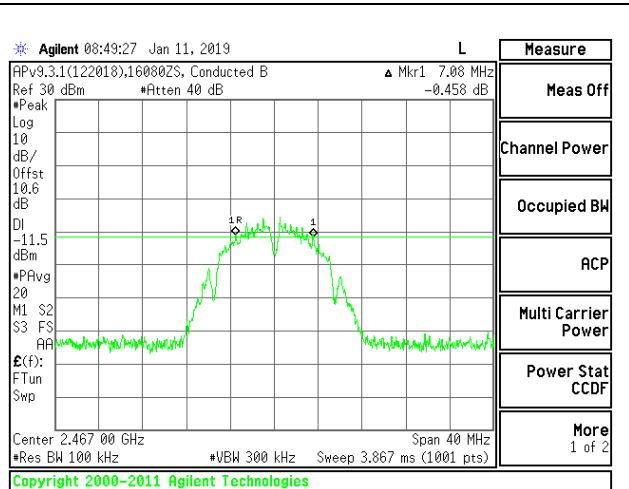
HIGH CHANNEL 12
