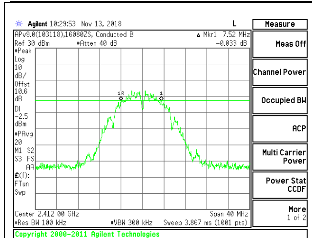
LOW CHANNEL 1
