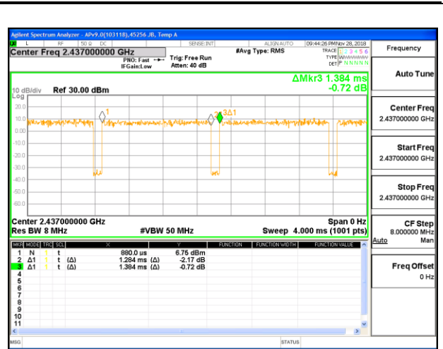
802.11ax HE20 OFDMA, 106T MODE
