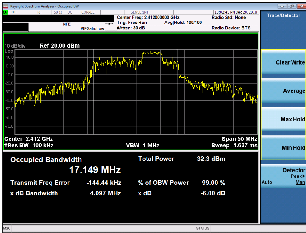
Plot 7-16. 6dB Bandwidth Plot SISO ANT2 (802.11ax OFDMA – 52 Tones – Ch. 1)
