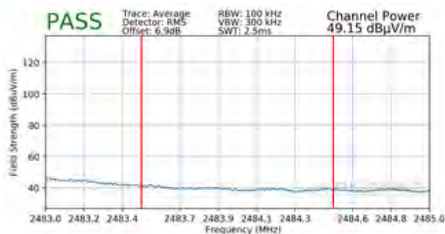
Plot 7-157. Radiated Restricted Upper Band Edge Measurement CDD (Average)
