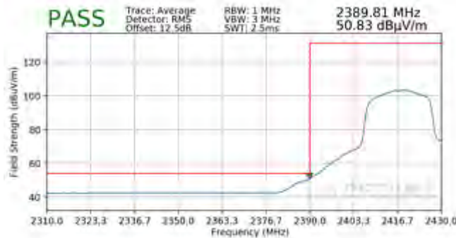
Plot 7-135. Radiated Restricted Lower Band Edge Measurement MIMO (Average)
