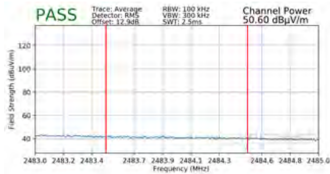
Plot 7-145. Radiated Restricted Band Edge Measurement MIMO with WCP (Average)
