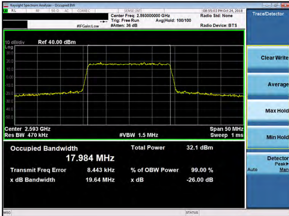
Plot 7-79. Occupied Bandwidth Plot (Band 41 PC3 - 20.0MHz QPSK - Full RB Configuration)
