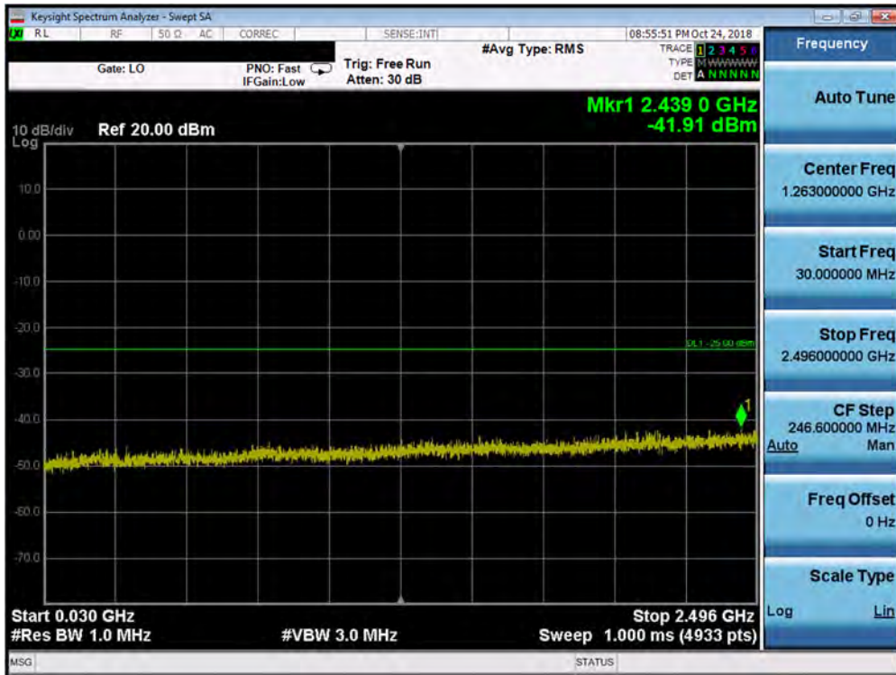
Plot 7-124. Conducted Spurious Plot (Band 41 PC3 - 20.0MHz QPSK - RB Size 1, RB Offset 0 - Mid Channel)
