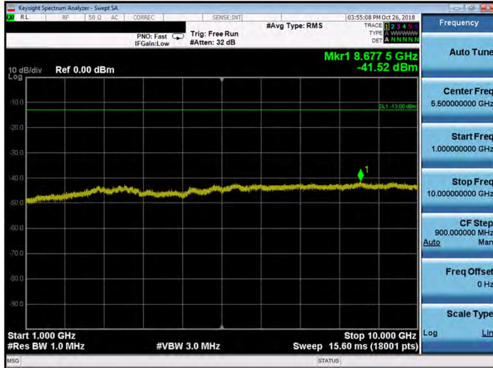
Plot 7-90. Conducted Spurious Plot (Band 12 - 5.0MHz QPSK - RB Size 1, RB Offset 0 - High Channel)
