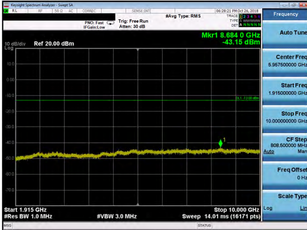
Plot 7-116. Conducted Spurious Plot (Band 25/2 - 15.0MHz QPSK - RB Size 1, RB Offset 0 - Mid Channel)
