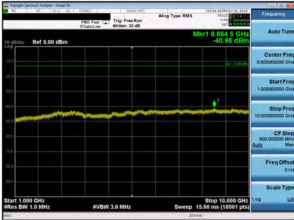
Plot 7-84. Conducted Spurious Plot (Band 12 - 5.0MHz QPSK - RB Size 1, RB Offset 0 - Low Channel)
