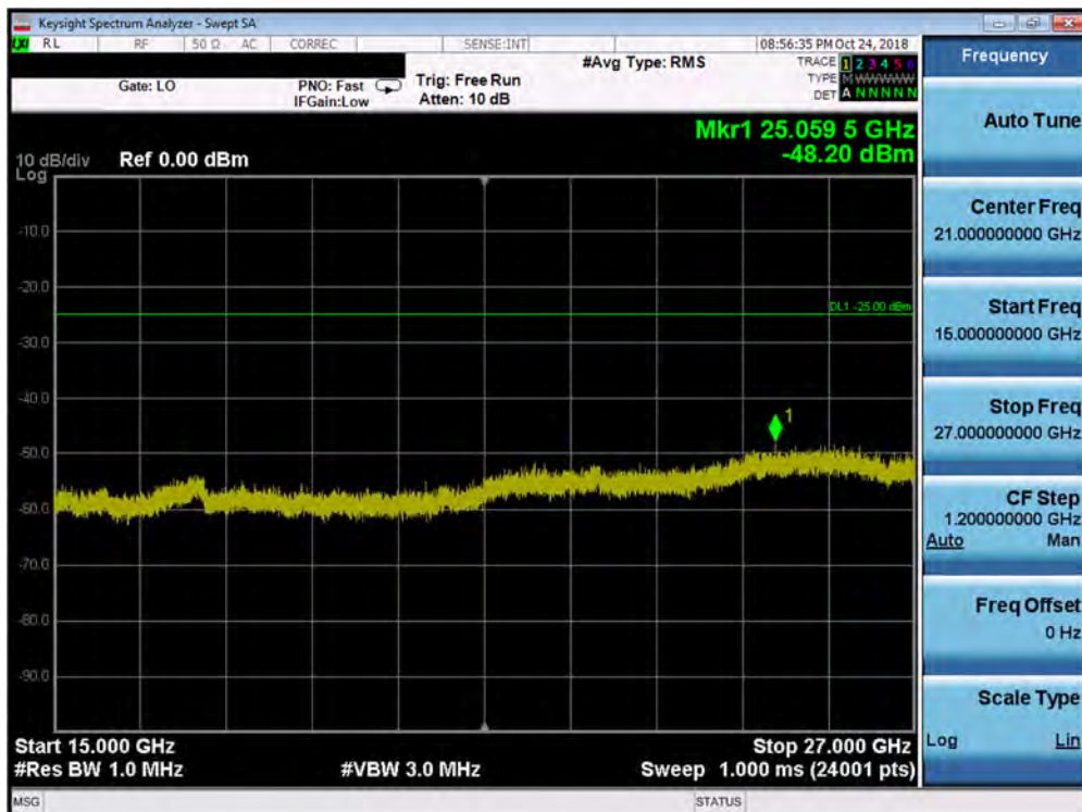
Plot 7-126. Conducted Spurious Plot (Band 41 PC3 - 20.0MHz QPSK - RB Size 1, RB Offset 0 - Mid Channel)
