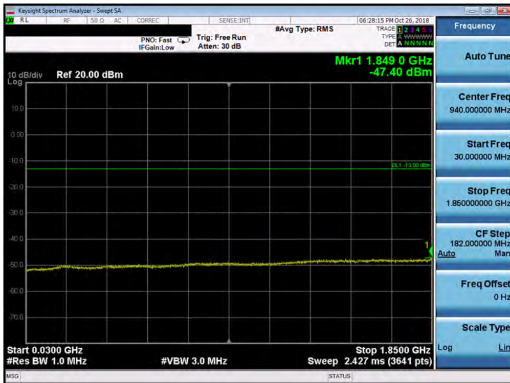
Plot 7-115. Conducted Spurious Plot (Band 25/2 - 15.0MHz QPSK - RB Size 1, RB Offset 0 - Mid Channel)
