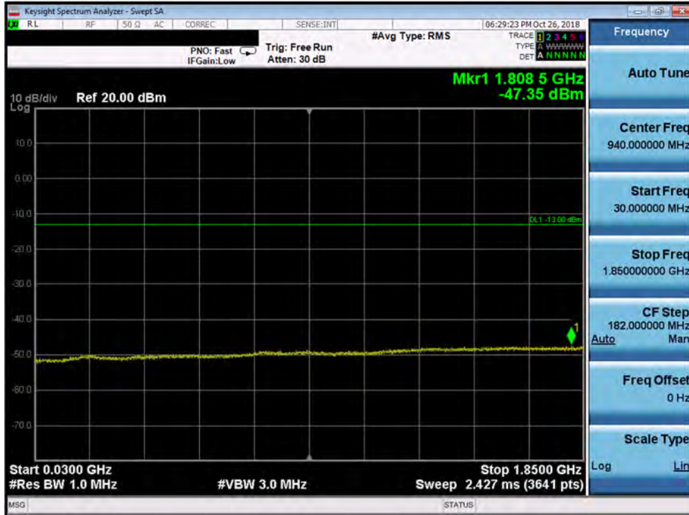
Plot 7-118. Conducted Spurious Plot (Band 25/2 - 15.0MHz QPSK - RB Size 1, RB Offset 0 - High Channel)
