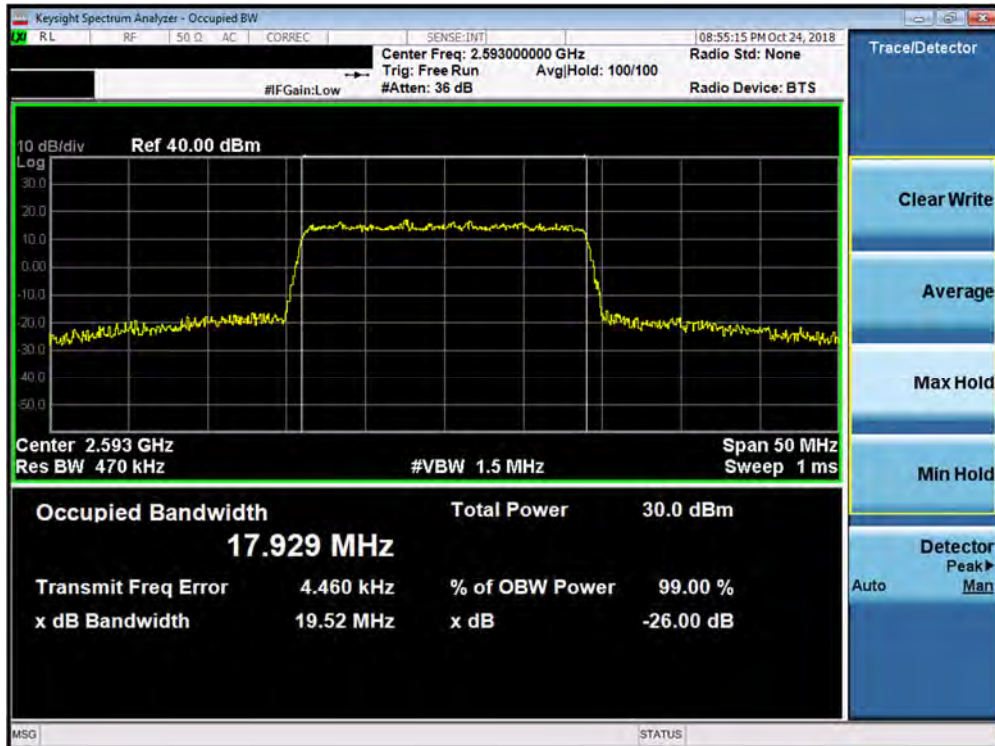
Plot 7-81. Occupied Bandwidth Plot (Band 41 PC3 - 20.0MHz 64-QAM - Full RB Configuration)
