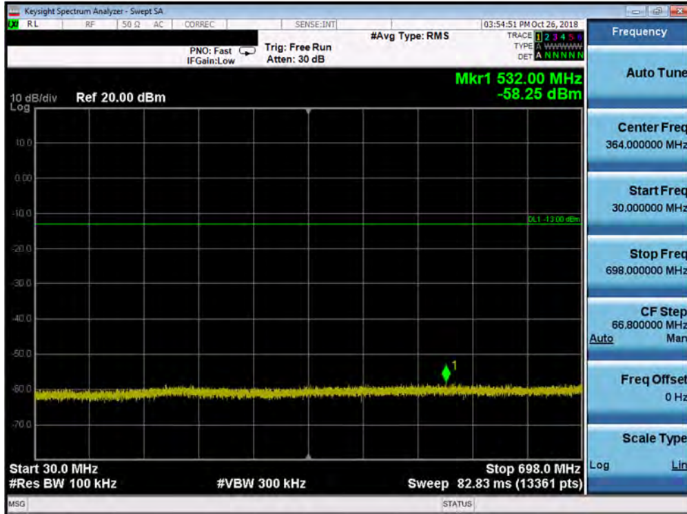
Plot 7-88. Conducted Spurious Plot (Band 12 - 5.0MHz QPSK - RB Size 1, RB Offset 0 - High Channel)
