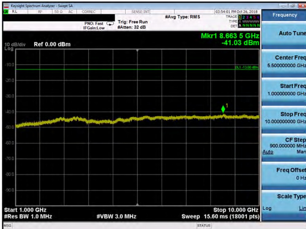
Plot 7-87. Conducted Spurious Plot (Band 12 - 5.0MHz QPSK - RB Size 1, RB Offset 0 - Mid Channel)
