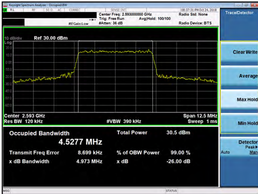
Plot 7-71. Occupied Bandwidth Plot (Band 41 PC3 – 5.0MHz 16-QAM - Full RB Configuration)
