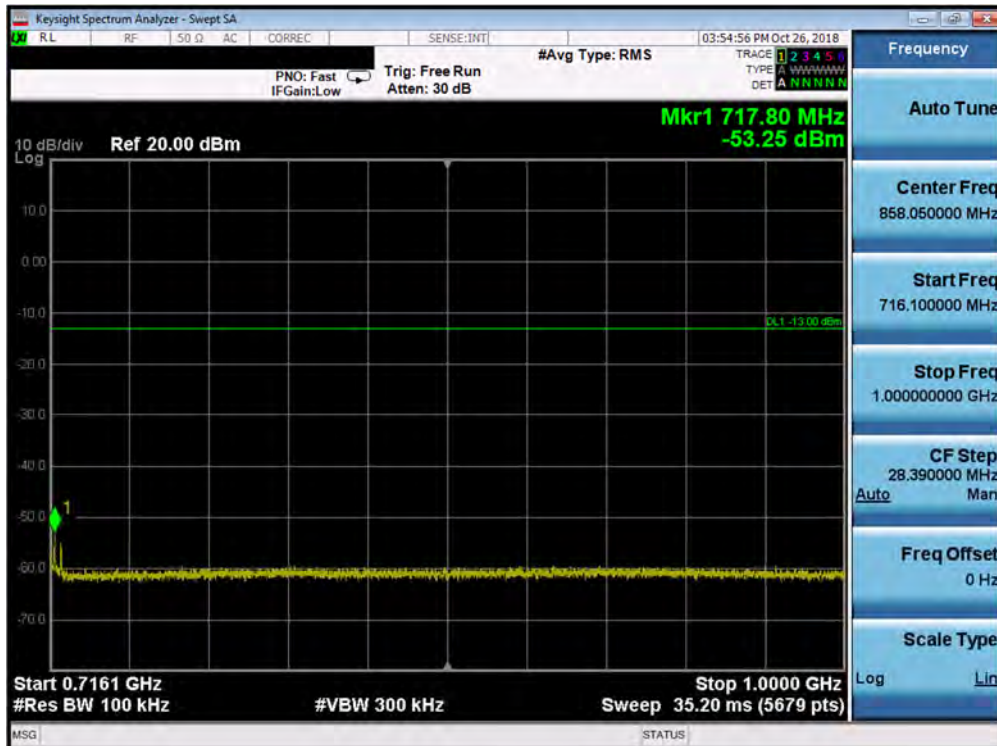
Plot 7-89. Conducted Spurious Plot (Band 12 - 5.0MHz QPSK - RB Size 1, RB Offset 0 - High Channel)
