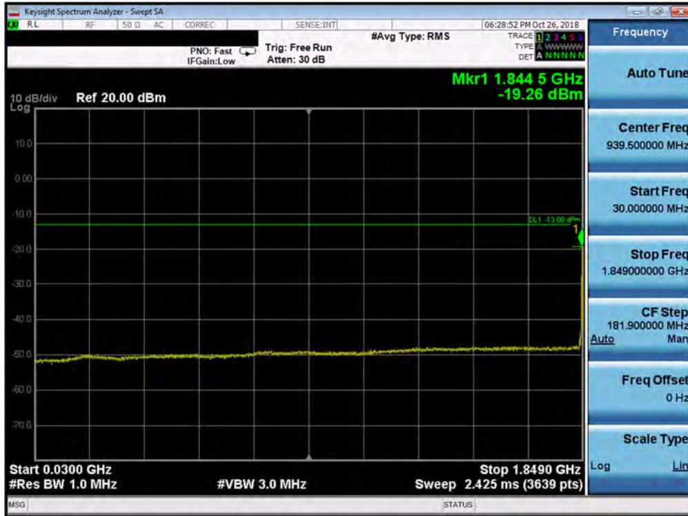
Plot 7-112. Conducted Spurious Plot (Band 25/2 - 15.0MHz QPSK - RB Size 1, RB Offset 0 - Low Channel)
