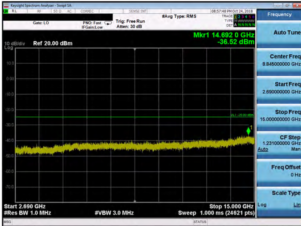
Plot 7-122. Conducted Spurious Plot (Band 41 PC3 - 20.0MHz QPSK - RB Size 1, RB Offset 0 - Low Channel)
