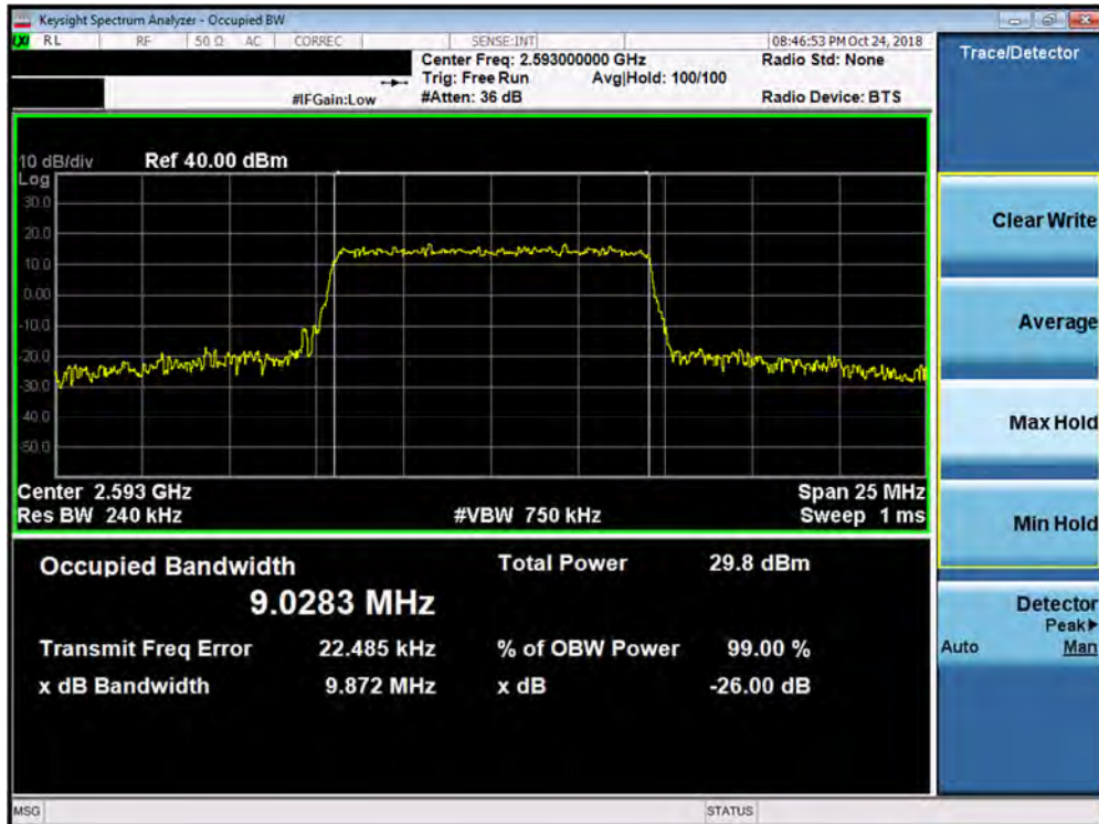
Plot 7-75. Occupied Bandwidth Plot (Band 41 PC3 - 10.0MHz 64-QAM - Full RB Configuration)
