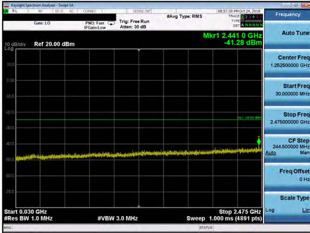
Plot 7-121. Conducted Spurious Plot (Band 41 PC3 - 20.0MHz QPSK - RB Size 1, RB Offset 0 - Low Channel)
