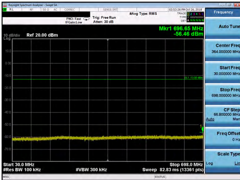
Plot 7-85. Conducted Spurious Plot (Band 12 - 5.0MHz QPSK - RB Size 1, RB Offset 0 - Mid Channel)
