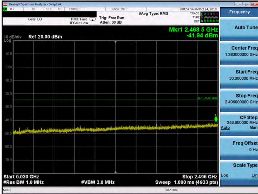
Plot 7-127. Conducted Spurious Plot (Band 41 PC3 - 20.0MHz QPSK - RB Size 1, RB Offset 0 - High Channel)
