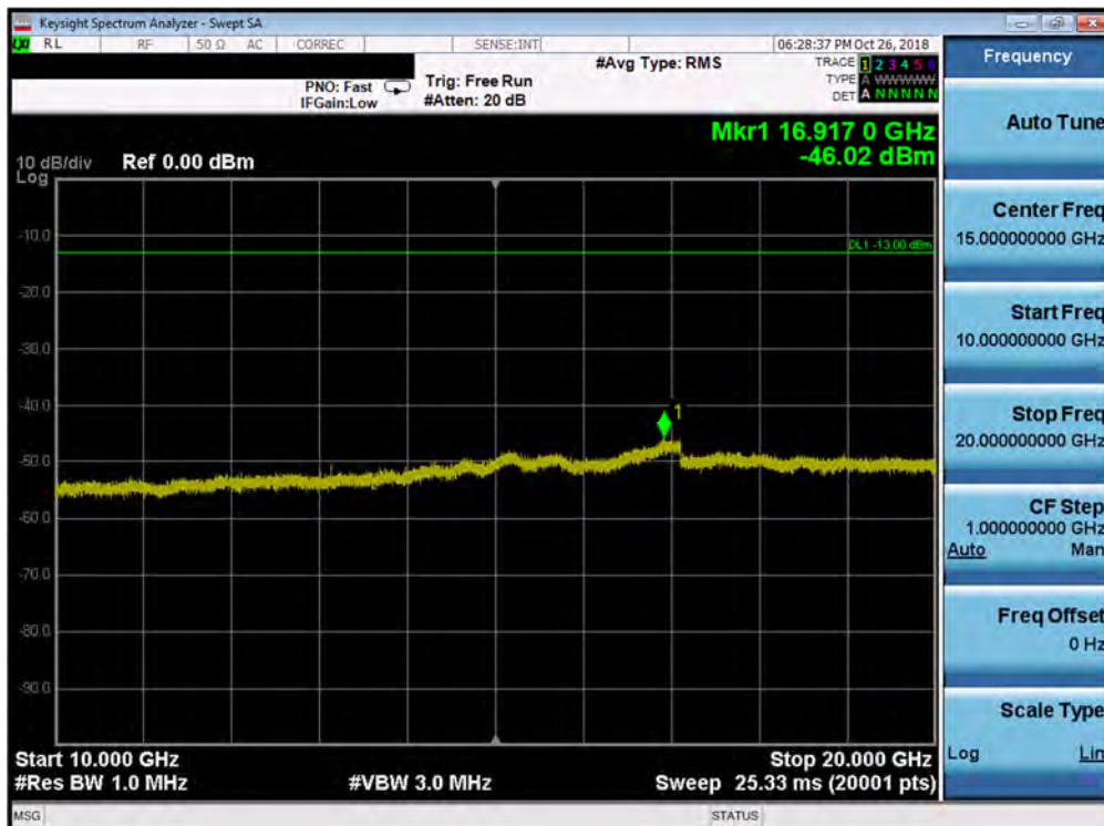
Plot 7-117. Conducted Spurious Plot (Band 25/2 - 15.0MHz QPSK - RB Size 1, RB Offset 0 - Mid Channel)
