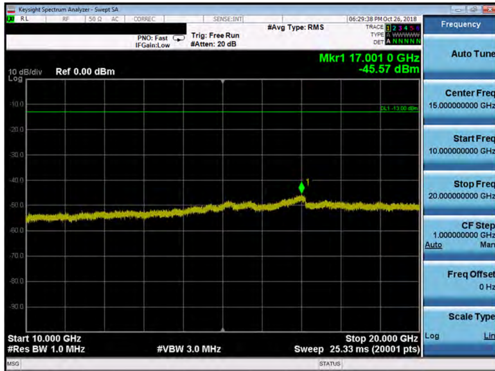
Plot 7-120. Conducted Spurious Plot (Band 25/2 - 15.0MHz QPSK - RB Size 1, RB Offset 0 - High Channel)
