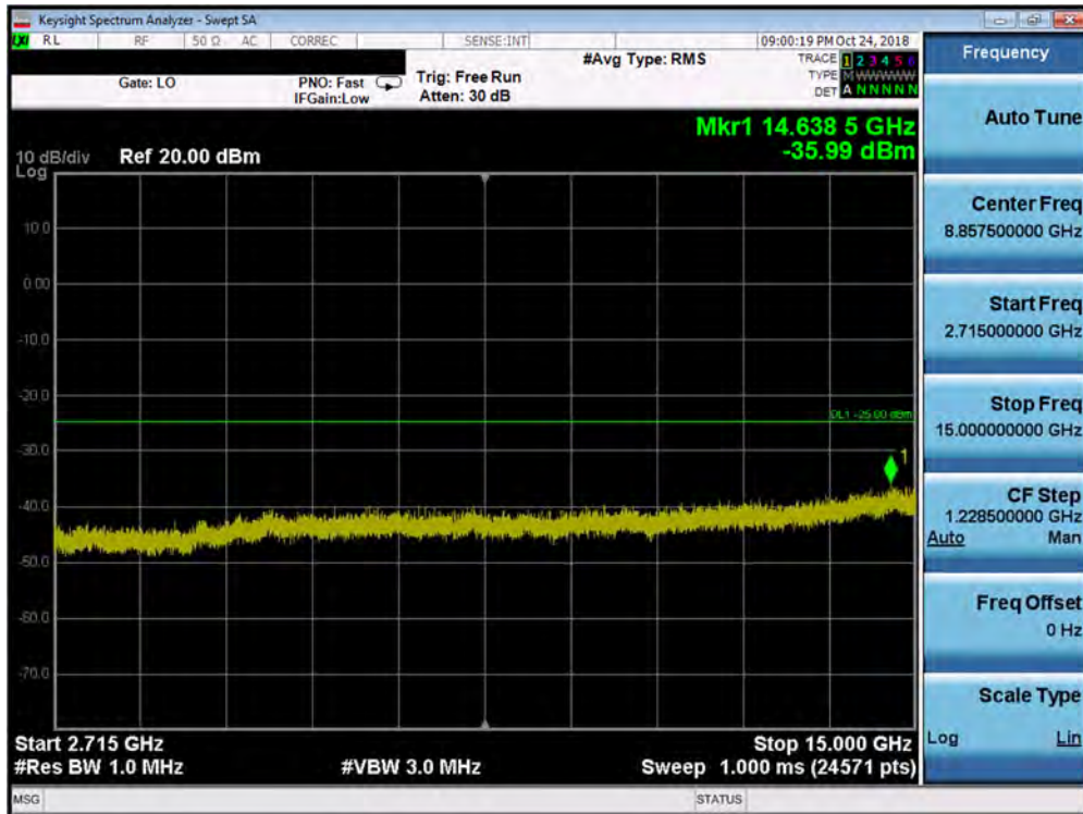
Plot 7-128. Conducted Spurious Plot (Band 41 PC3 - 20.0MHz QPSK - RB Size 1, RB Offset 0 - High Channel)
