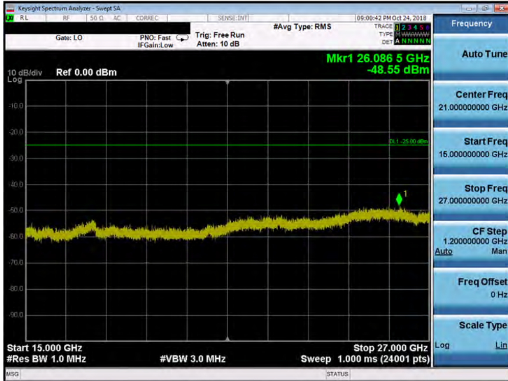
Plot 7-129. Conducted Spurious Plot (Band 41 PC3 - 20.0MHz QPSK - RB Size 1, RB Offset 0 - High Channel)
