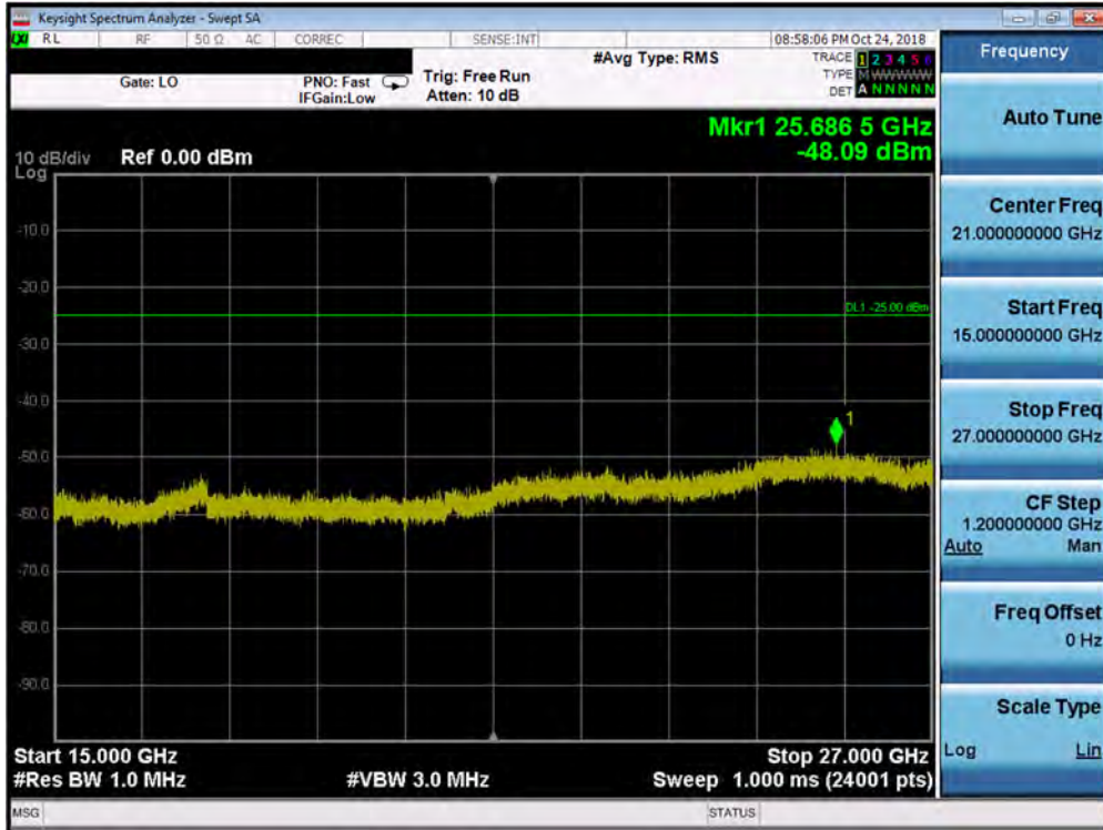
Plot 7-123. Conducted Spurious Plot (Band 41 PC3 - 20.0MHz QPSK - RB Size 1, RB Offset 0 - Low Channel)
