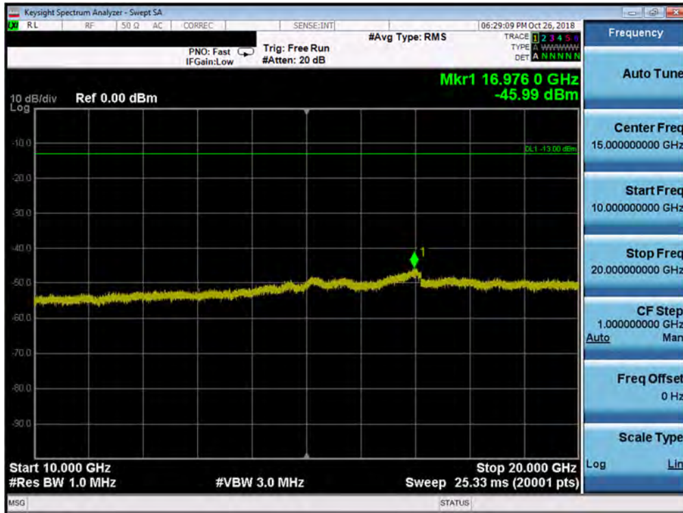
Plot 7-114. Conducted Spurious Plot (Band 25/2 - 15.0MHz QPSK - RB Size 1, RB Offset 0 - Low Channel)
