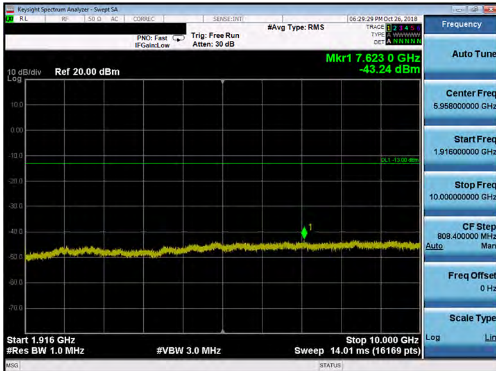
Plot 7-119. Conducted Spurious Plot (Band 25/2 - 15.0MHz QPSK - RB Size 1, RB Offset 0 - High Channel)
