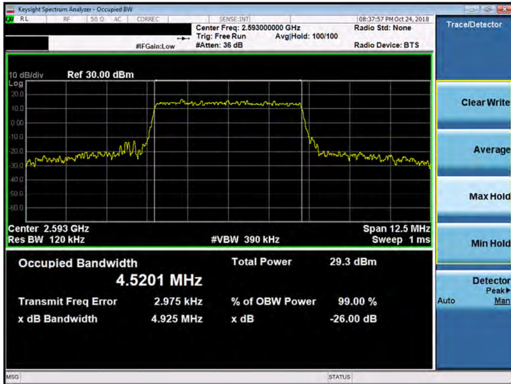
Plot 7-72. Occupied Bandwidth Plot (Band 41 PC3 – 5.0MHz 64-QAM - Full RB Configuration)
