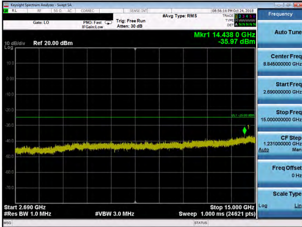
Plot 7-125. Conducted Spurious Plot (Band 41 PC3 - 20.0MHz QPSK - RB Size 1, RB Offset 0 - Mid Channel)
