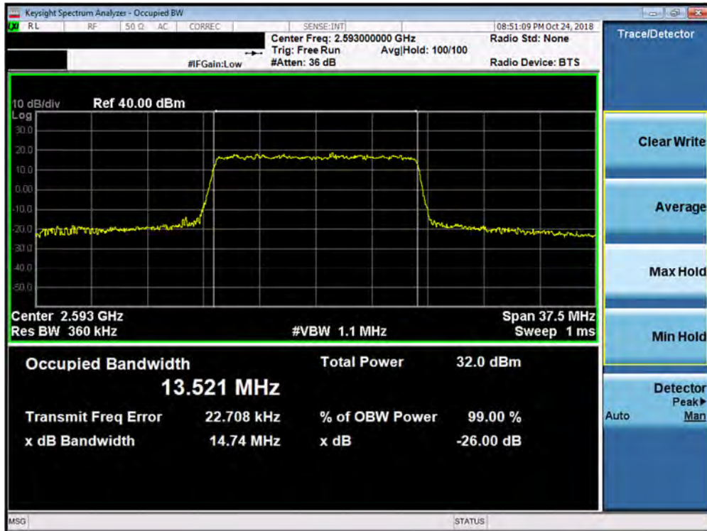
Plot 7-76. Occupied Bandwidth Plot (Band 41 PC3 - 15.0MHz QPSK - Full RB Configuration)
