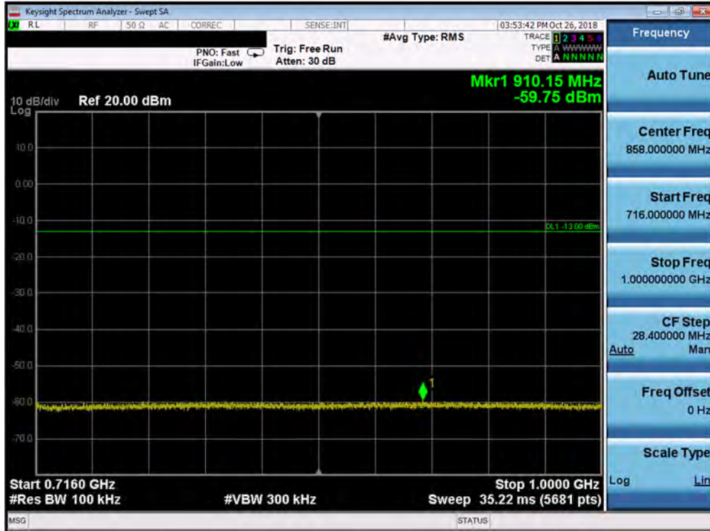
Plot 7-86. Conducted Spurious Plot (Band 12 - 5.0MHz QPSK - RB Size 1, RB Offset 0 - Mid Channel)
