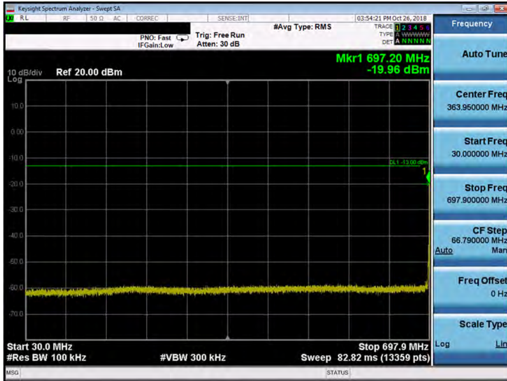
Plot 7-82. Conducted Spurious Plot (Band 12 - 5.0MHz QPSK - RB Size 1, RB Offset 0 - Low Channel)
