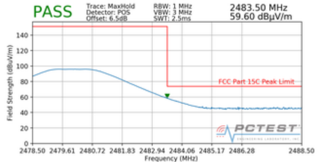
Plot 7-38. Radiated Restricted Upper Band Edge Measurement with WCP (Peak)
