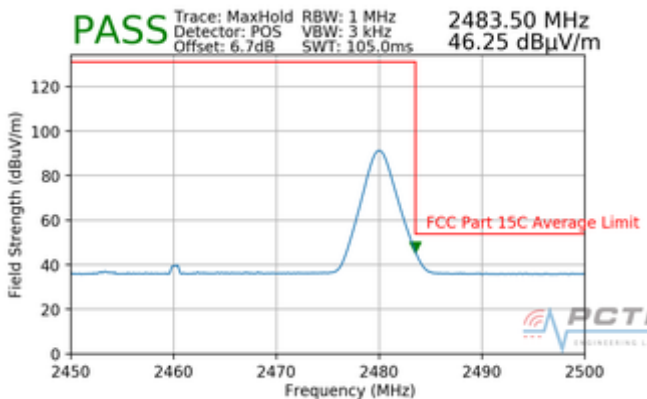
Plot 7-37. Radiated Restricted Upper Band Edge Measurement with WCP (Average)
