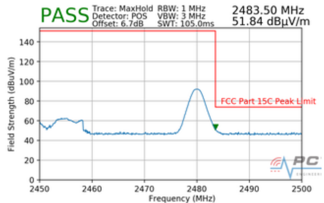
Plot 7-38. Radiated Restricted Upper Band Edge Measurement with WCP (Peak)
