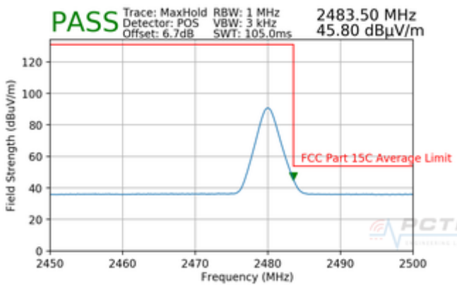
Plot 7-35. Radiated Restricted Upper Band Edge Measurement (Average)
