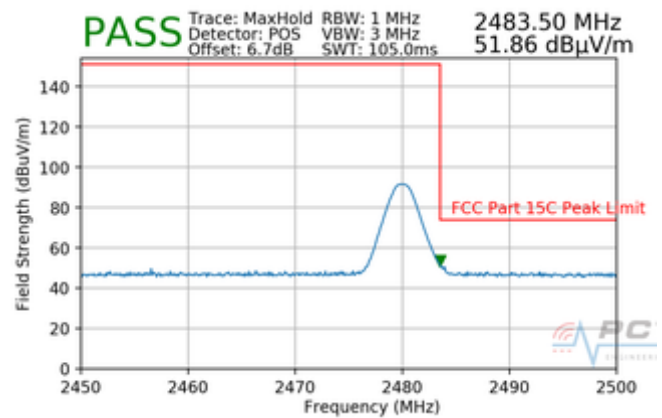
Plot 7-36. Radiated Restricted Upper Band Edge Measurement (Peak)
