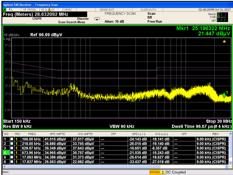
Plot 7-9. Line-Conducted Test Plot with Travel Adapter (N)
