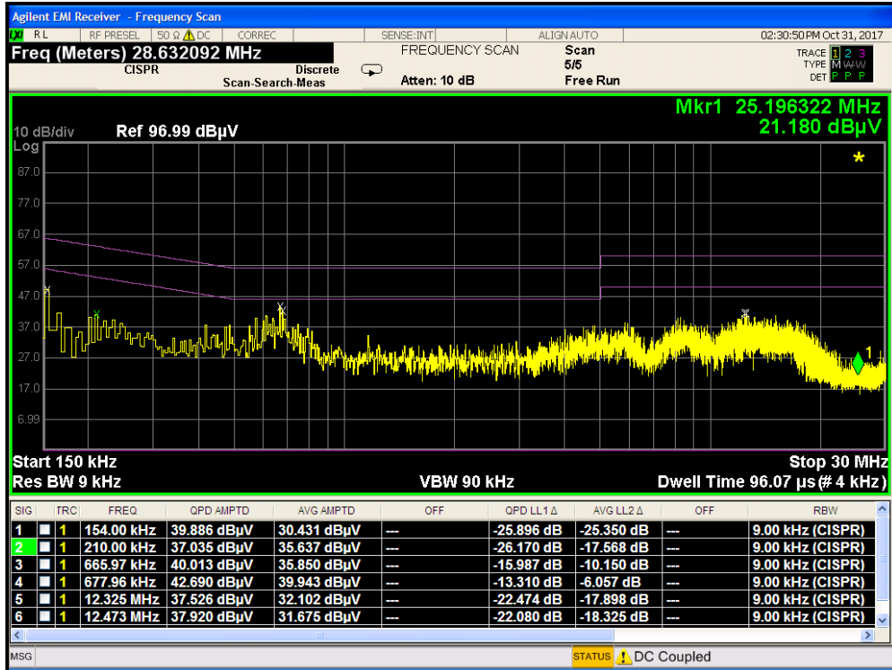
Plot 7-39. Line Conducted Plot Bluetooth LE with Travel Adapter (L1)
