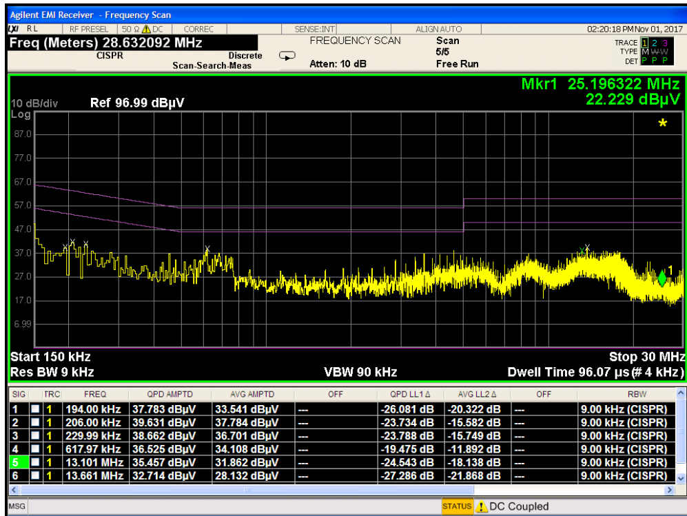
Plot 7-42. Line Conducted Plot Bluetooth LE with Wireless Charging Pad (N)
