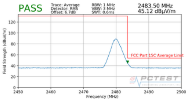
Plot 7-35. Radiated Restricted Upper Band Edge Measurement 2Mbps (Average)
