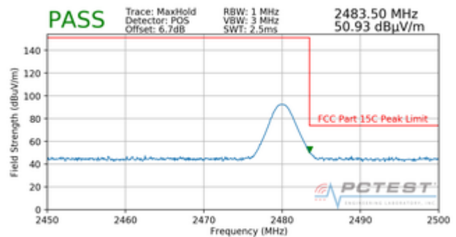
Plot 7-36. Radiated Restricted Upper Band Edge Measurement 2Mbps (Peak)
