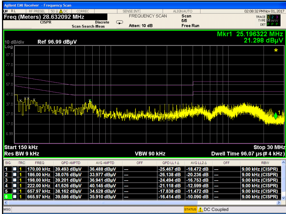
Plot 7-41. Line Conducted Plot Bluetooth LE with Wireless Charging Pad (L1)
