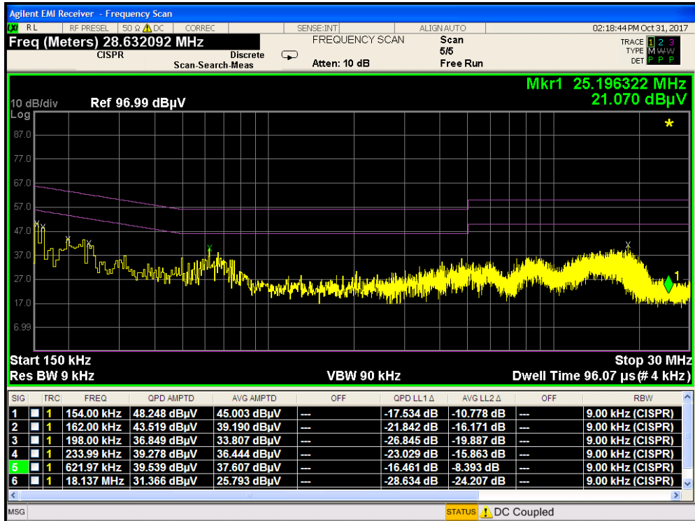
Plot 7-40. Line Conducted Plot Bluetooth LE with Travel Adapter (N)
