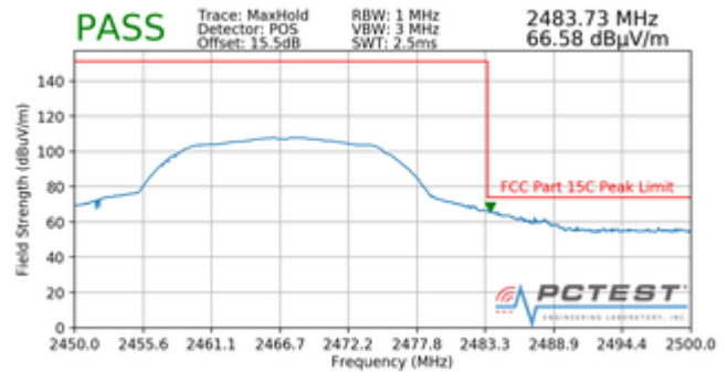
Plot 7-82. Radiated Restricted Upper Band Edge Measurement (Peak)
