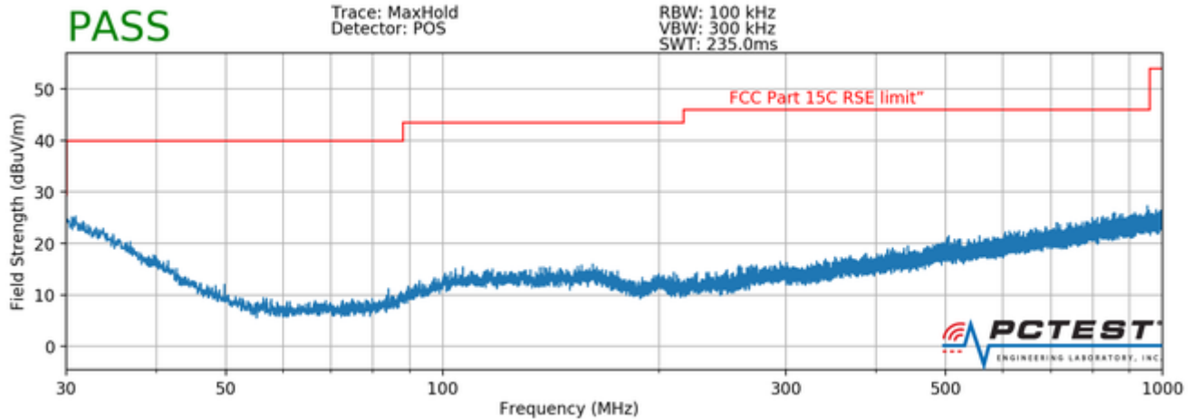
Plot 7-120. Radiated Spurious Plot below 1GHz (Pol. V)
