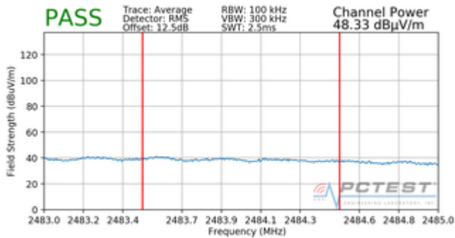
Plot 7-111. Radiated Restricted Upper Band Edge Measurement (Average)
