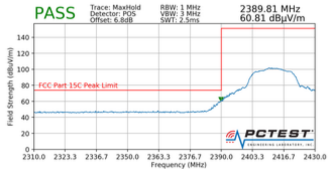
Plot 7-98. Radiated Restricted Lower Band Edge Measurement (Peak)
