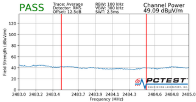
Plot 7-101. Radiated Restricted Upper Band Edge Measurement (Average)
