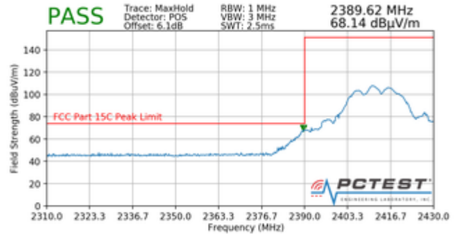
Plot 7-116. Radiated Restricted Band Edge Measurement with WCP (Peak)
