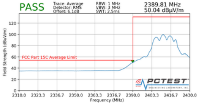
Plot 7-115. Radiated Restricted Band Edge Measurement with WCP (Average)
