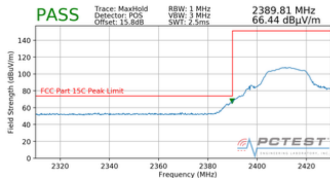
Plot 7-78. Radiated Restricted Lower Band Edge Measurement (Peak)
