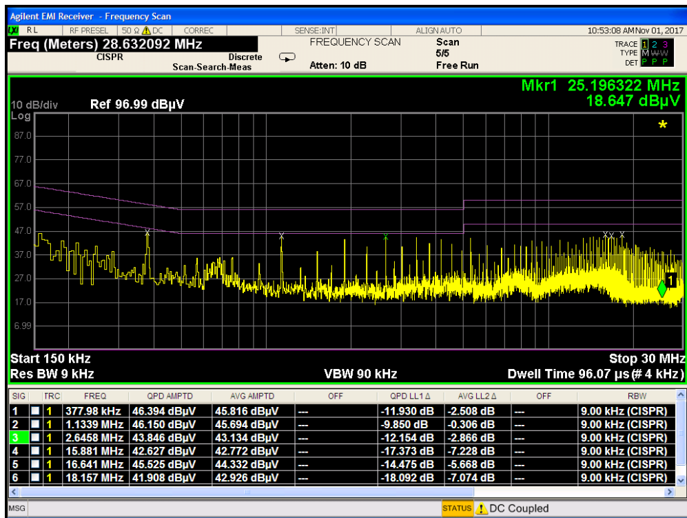
Plot 7-124. Line Conducted Plot 802.11b with Wireless Charging (N)
