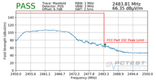
Plot 7-106. Radiated Restricted Band Edge Measurement with WCP (Peak)
