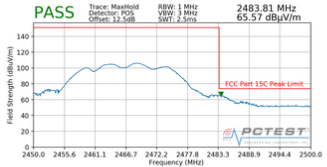
Plot 7-112. Radiated Restricted Upper Band Edge Measurement (Peak)
