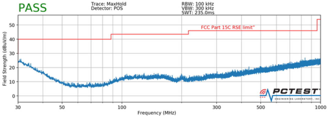
Plot 7-118. Radiated Spurious Plot below 1GHz (Pol. V)
