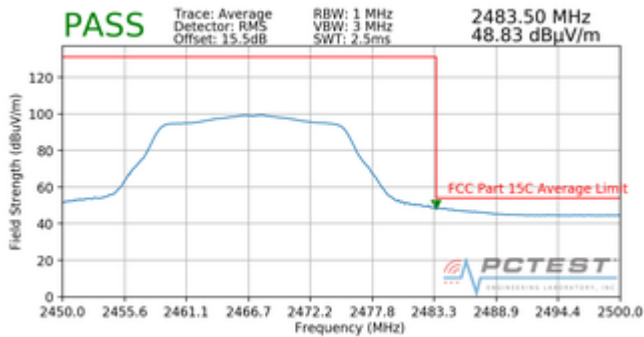
Plot 7-81. Radiated Restricted Upper Band Edge Measurement (Average)
