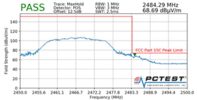
Plot 7-102. Radiated Restricted Upper Band Edge Measurement (Peak)
