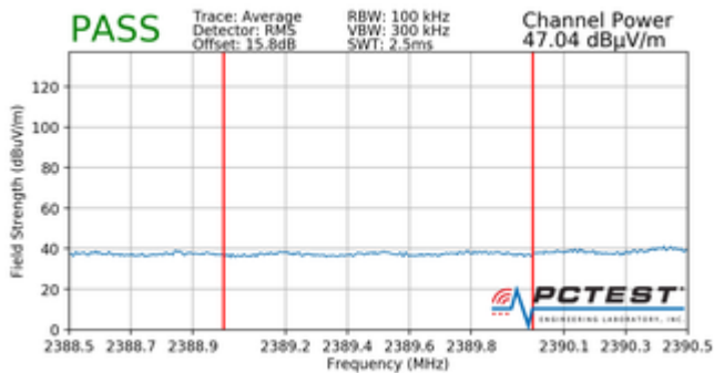
Plot 7-97. Radiated Restricted Lower Band Edge Measurement (Average)
