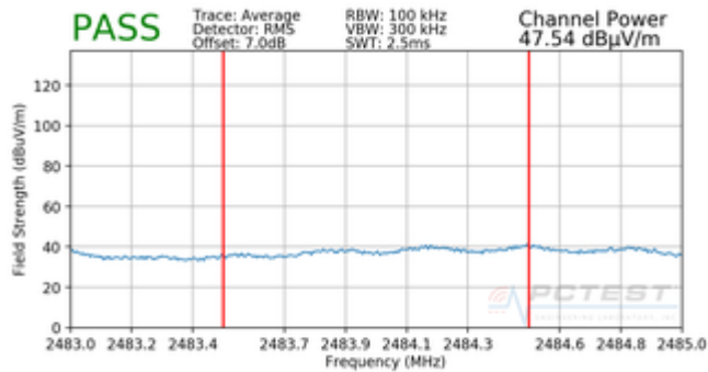
Plot 7-105. Radiated Restricted Band Edge Measurement with WCP (Average)
