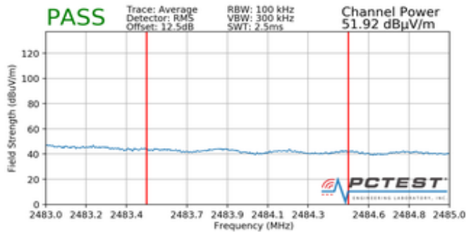
Plot 7-95. Radiated Restricted Band Edge Measurement with WCP (Average)
