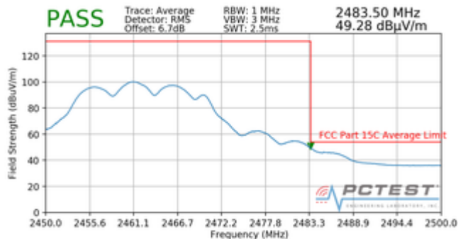
Plot 7-109. Radiated Restricted Upper Band Edge Measurement (Average)
