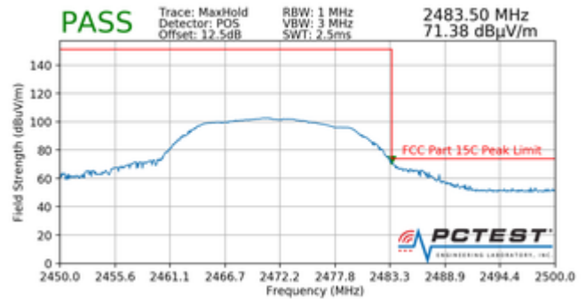
Plot 7-96. Radiated Restricted Band Edge Measurement with WCP (Peak)
