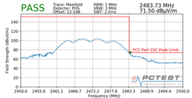
Plot 7-114. Radiated Restricted Upper Band Edge Measurement (Peak)
