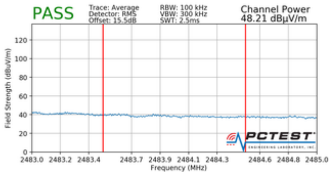
Plot 7-99. Radiated Restricted Upper Band Edge Measurement (Average)
