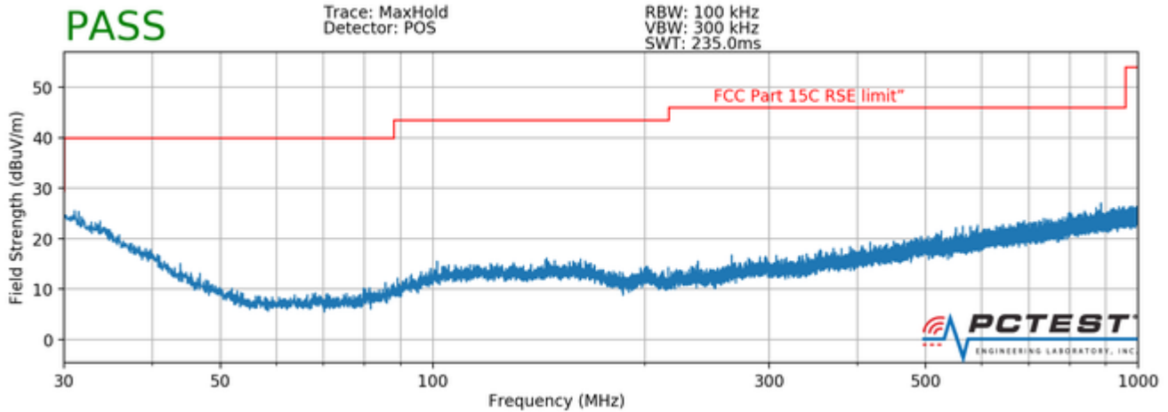
Plot 7-117. Radiated Spurious Plot below 1GHz (Pol. H)
