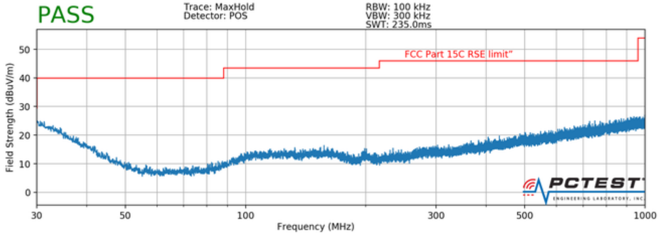
Plot 7-119. Radiated Spurious Plot below 1GHz (Pol. H)
