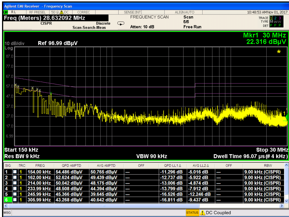
Plot 7-123. Line Conducted Plot 802.11b with Wireless Charging (L1)
