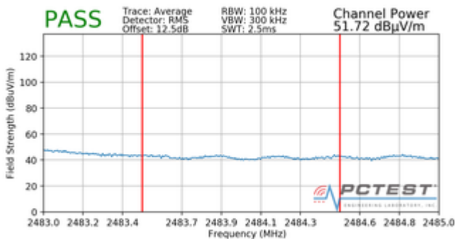
Plot 7-113. Radiated Restricted Upper Band Edge Measurement (Average)
