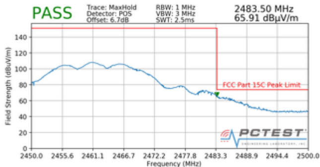
Plot 7-110. Radiated Restricted Upper Band Edge Measurement (Peak)
