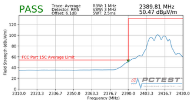
Plot 7-107. Radiated Restricted Lower Band Edge Measurement (Average)
