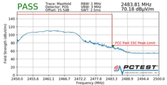
Plot 7-100. Radiated Restricted Upper Band Edge Measurement (Peak)
