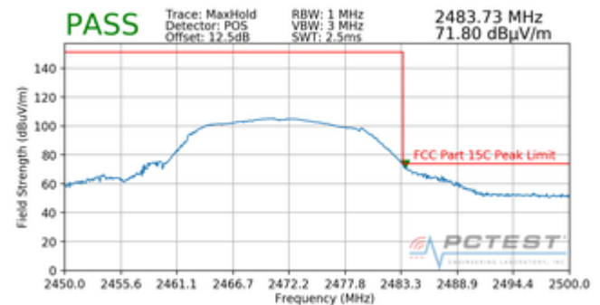
Plot 7-104. Radiated Restricted Upper Band Edge Measurement (Peak)
