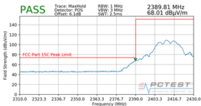
Plot 7-108. Radiated Restricted Lower Band Edge Measurement (Peak)
