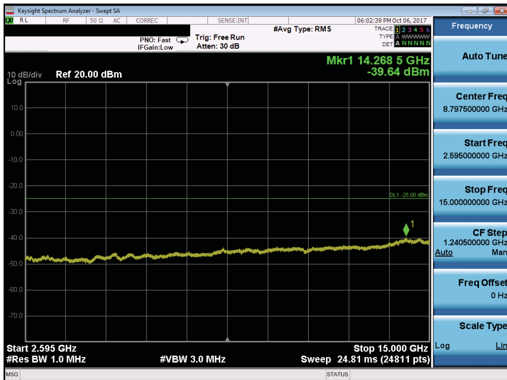
Plot 7-140. Conducted Spurious Plot (Band 7 - 5.0MHz QPSK - RB Size 1, RB Offset 0 - High Channel)
