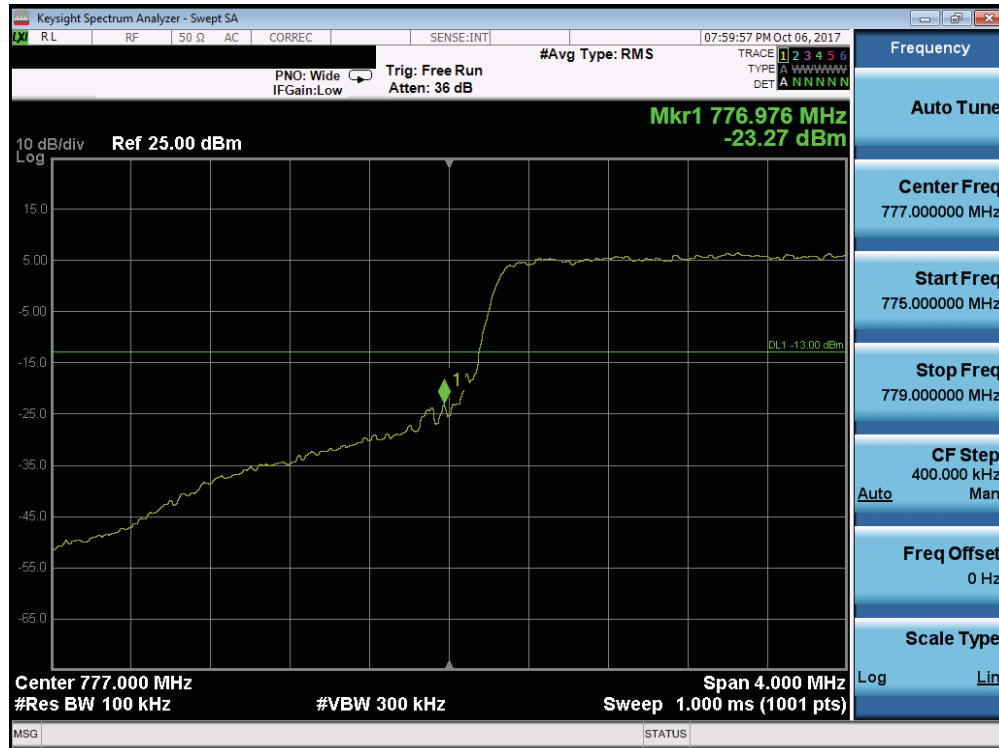
Plot 7-161. Lower Band Edge Plot (Band 13 - 5.0MHz QPSK - Full RB Configuration)
