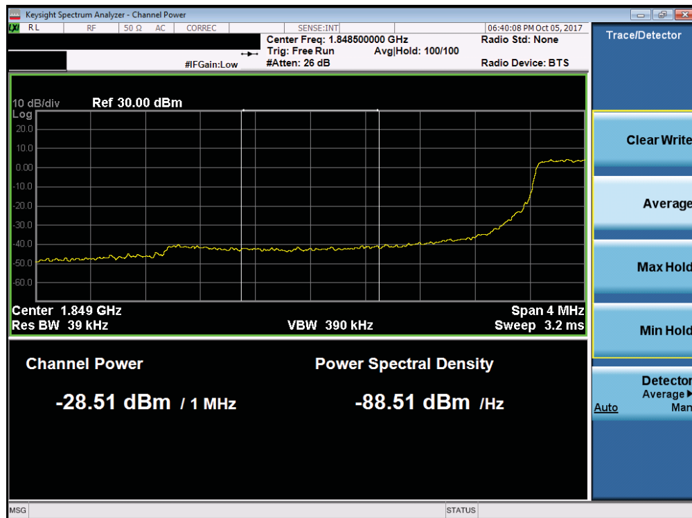
Plot 7-222. Lower Extended Band Edge Plot (Band 25/2 - 3.0MHz QPSK - Full RB Configuration)
