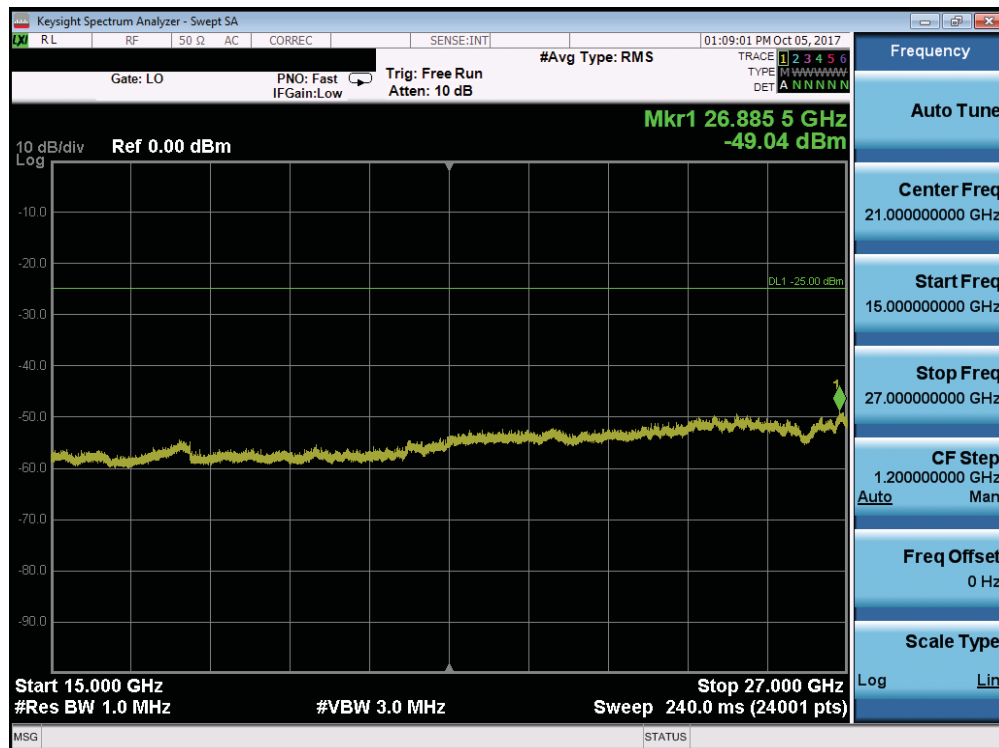
Plot 7-147. Conducted Spurious Plot (Band 38/41 - 10.0MHz QPSK - RB Size 1, RB Offset 0 - Mid Channel)
