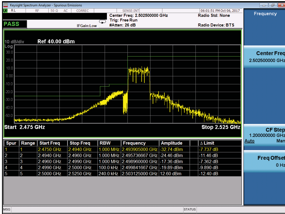
Plot 7-251. Lower ACP Plot (Band 7 - 5.0MHz QPSK - RB Size 25)
