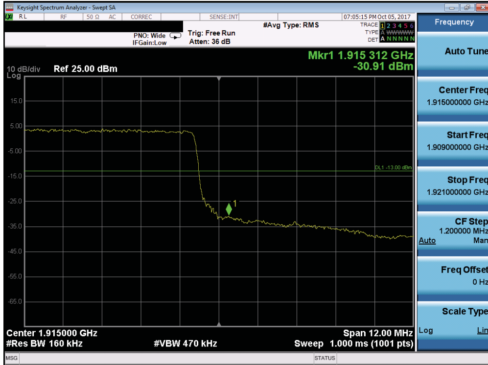
Plot 7-243. Upper Band Edge Plot (Band 25 - 15.0MHz QPSK - Full RB Configuration)
