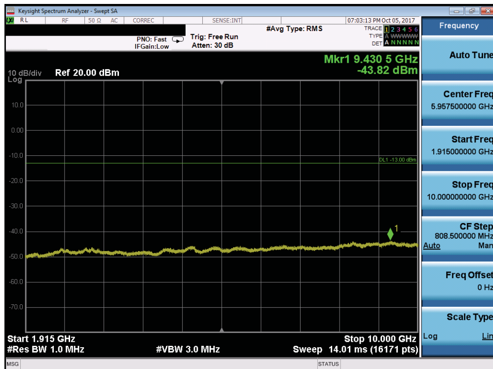
Plot 7-125. Conducted Spurious Plot (Band 25/2 - 15.0MHz QPSK - RB Size 1, RB Offset 0 - Low Channel)
