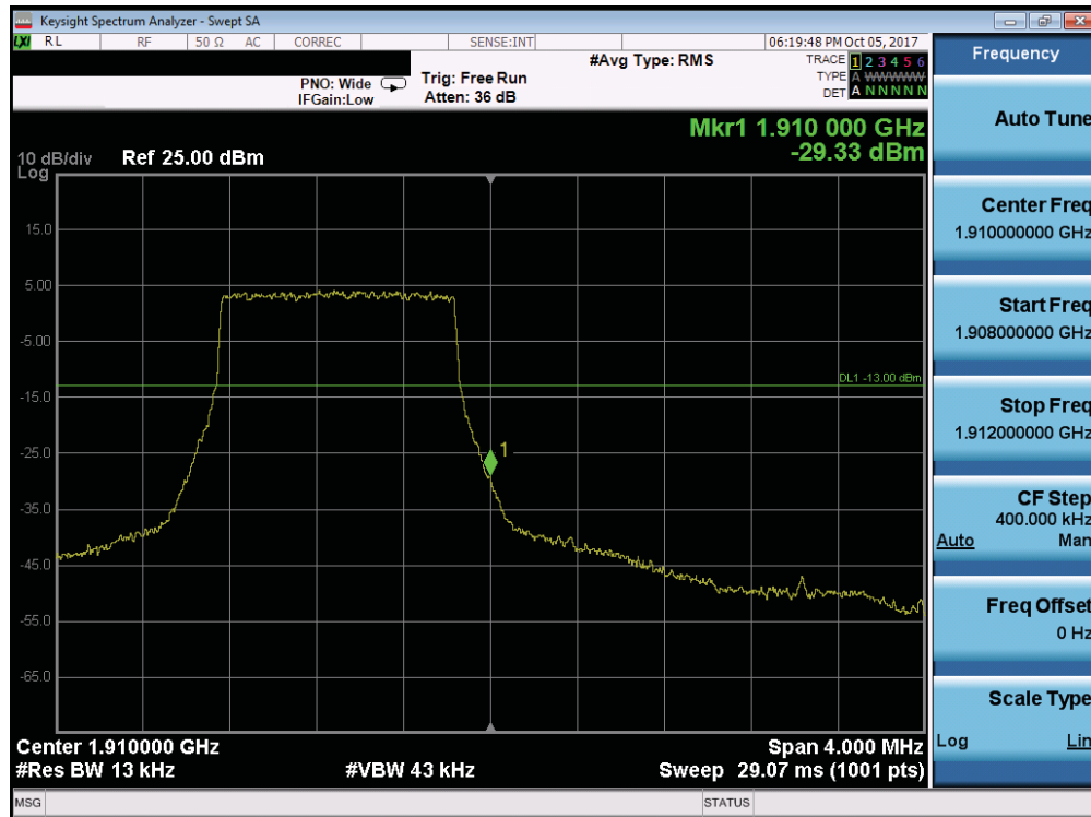
Plot 7-217. Upper Band Edge Plot (Band 2 - 1.4MHz QPSK - Full RB Configuration)
