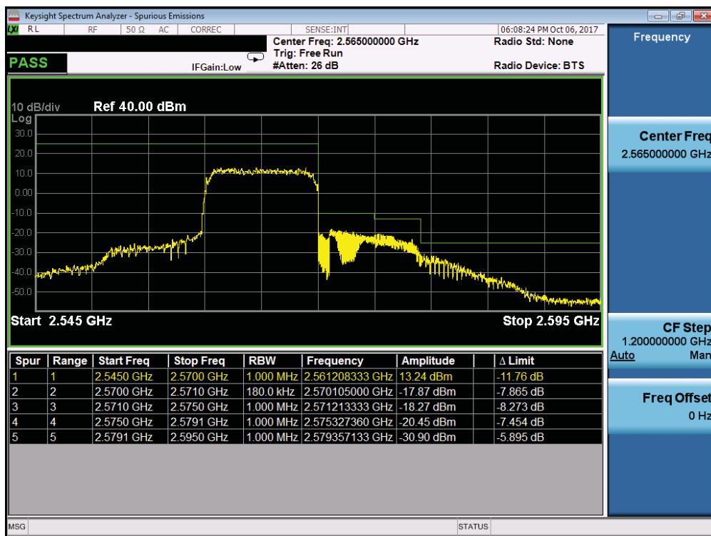
Plot 7-254. Upper ACP Plot (Band 7 - 10.0MHz QPSK - RB Size 25)
