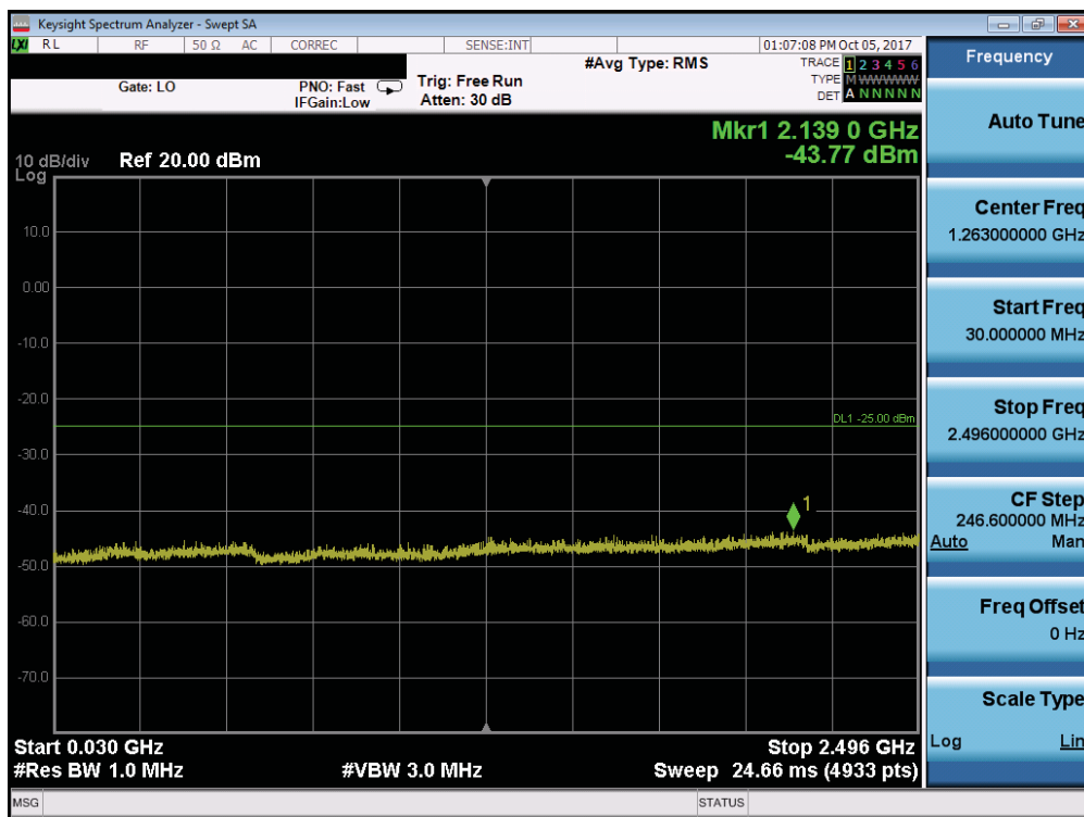
Plot 7-145. Conducted Spurious Plot (Band 38/41 - 10.0MHz QPSK - RB Size 1, RB Offset 0 - Mid Channel)
