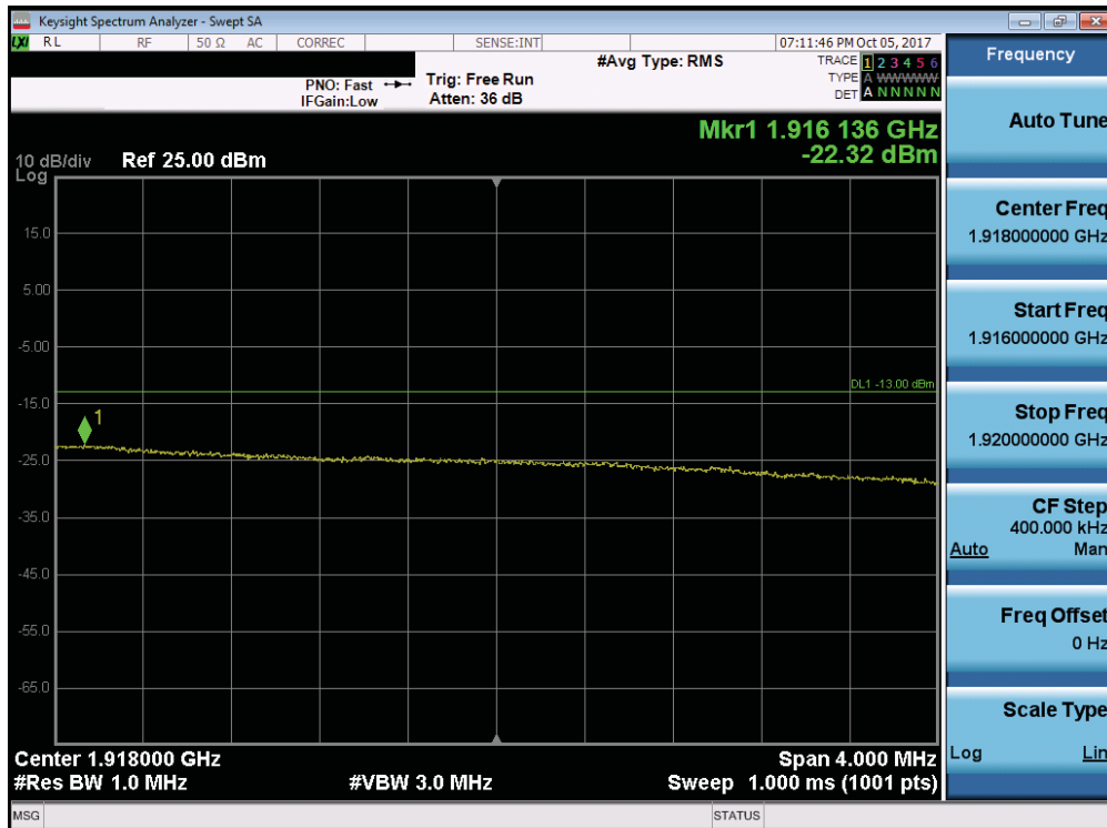
Plot 7-250. Upper Extended Band Edge Plot (Band 25 - 20.0MHz QPSK - Full RB Configuration)
