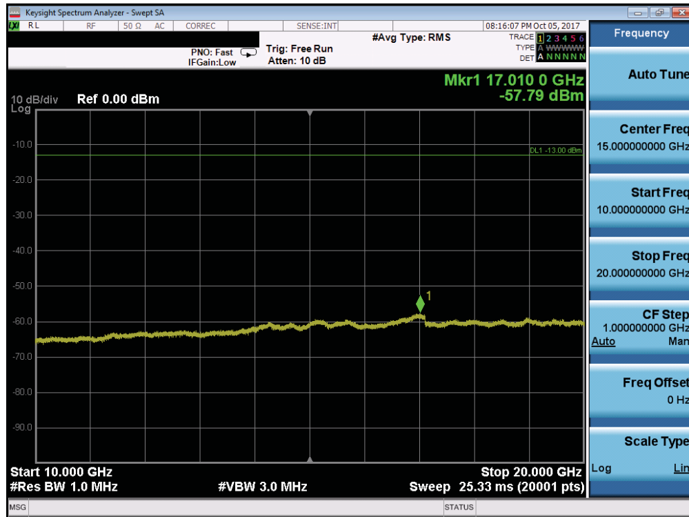
Plot 7-123. Conducted Spurious Plot (Band 66/4 - 10.0MHz QPSK - RB Size 1, RB Offset 0 - High Channel)
