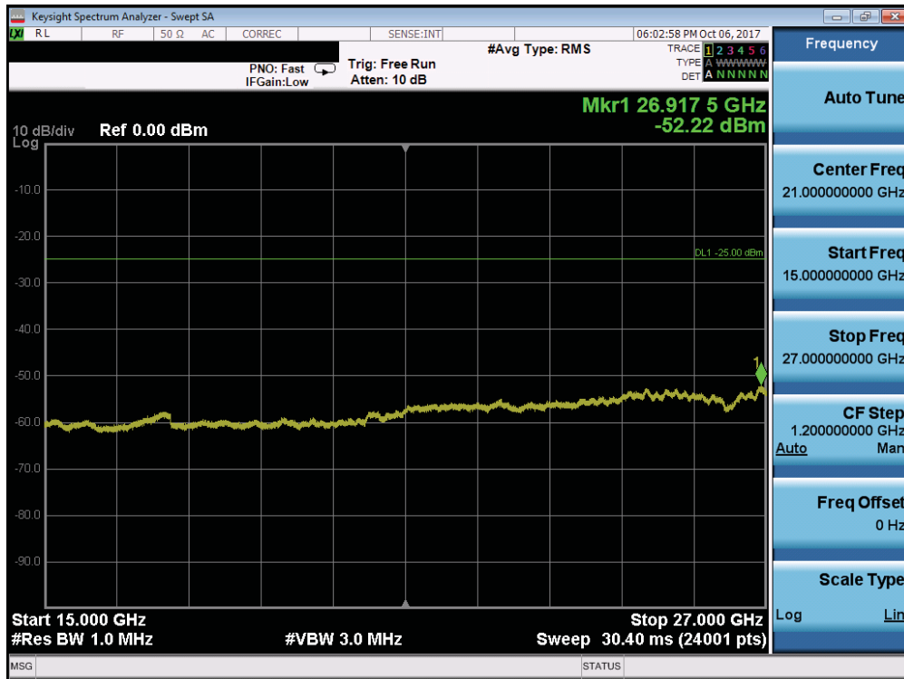
Plot 7-141. Conducted Spurious Plot (Band 7 - 5.0MHz QPSK - RB Size 1, RB Offset 0 - High Channel)
