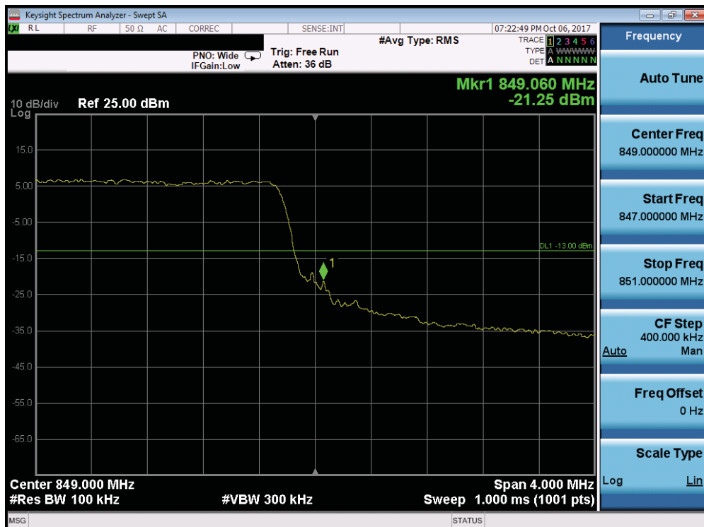
Plot 7-174. Upper Band Edge Plot (Band 5/26 – 5MHz QPSK - Full RB Configuration)
