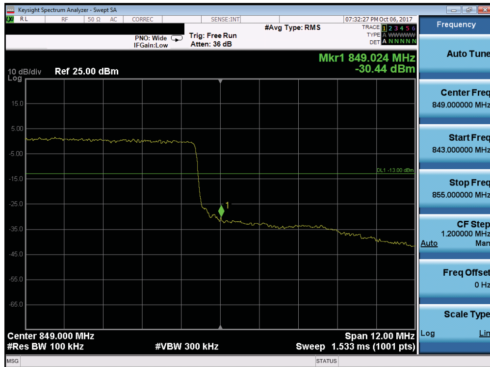
Plot 7-178. Upper Band Edge Plot (Band 26 - 15.0MHz QPSK - Full RB Configuration)
