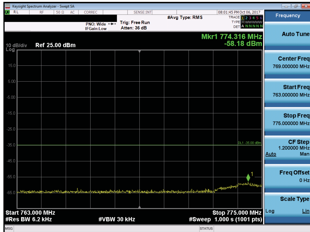
Plot 7-162. Lower Emission Mask (Band 13 - 5.0MHz QPSK - Full RB Configuration)
