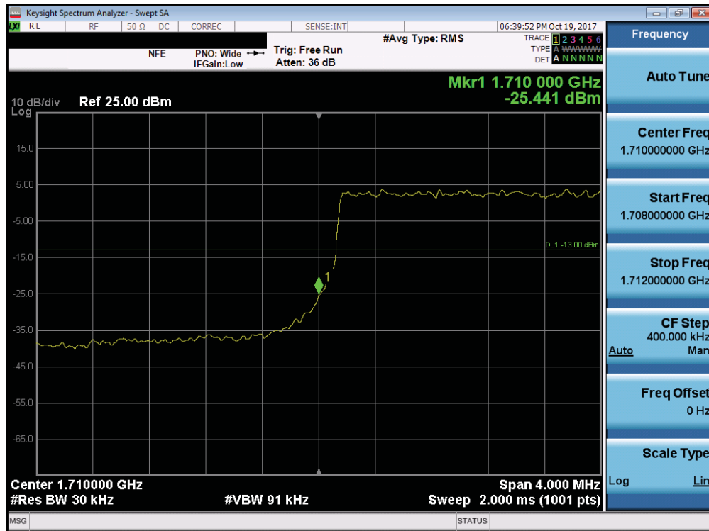
Plot 7-185. Lower Band Edge Plot (Band 66/4 - 3.0MHz QPSK - Full RB Configuration)
