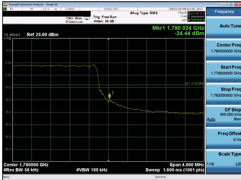
Plot 7-195. Upper Band Edge Plot (Band 66 - 5.0MHz QPSK - Full RB Configuration)
