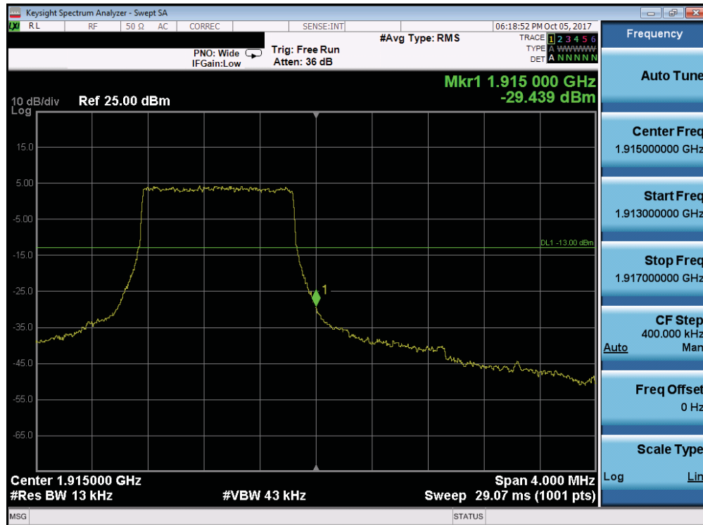
Plot 7-219. Upper Band Edge Plot (Band 25 - 1.4MHz QPSK - Full RB Configuration)
