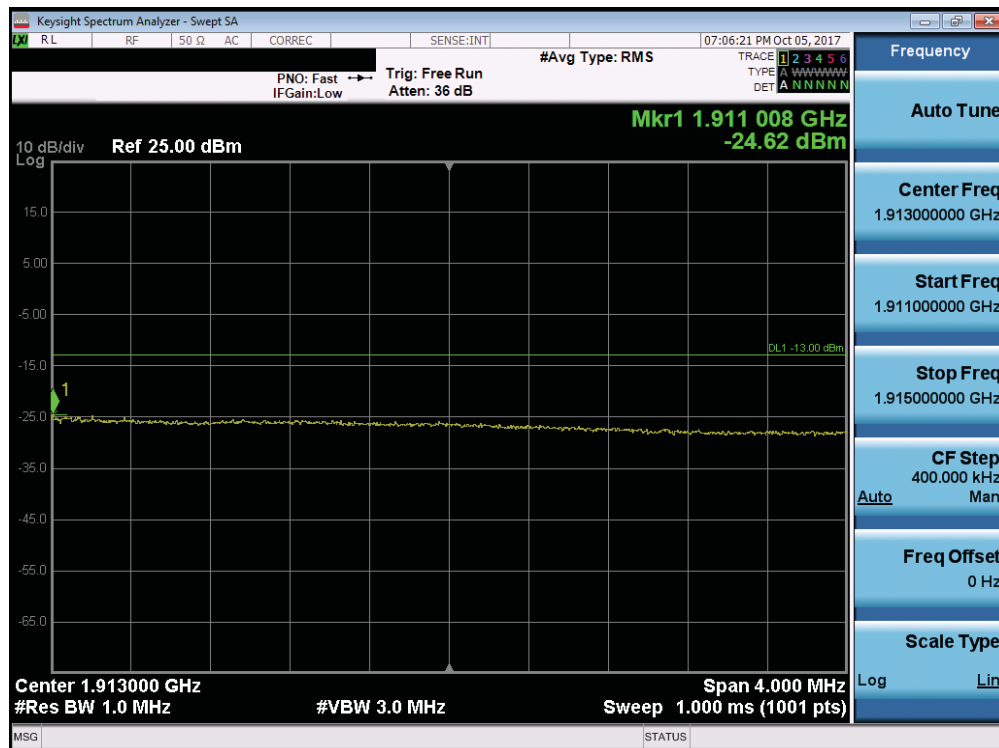
Plot 7-242. Upper Extended Band Edge Plot (Band 2 - 15.0MHz QPSK - Full RB Configuration)
