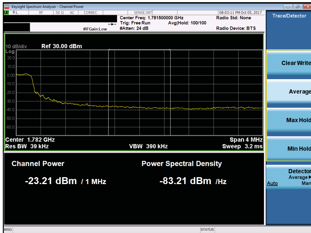
Plot 7-196. Upper Extended Band Edge Plot (Band 66 - 5.0MHz QPSK - Full RB Configuration)
