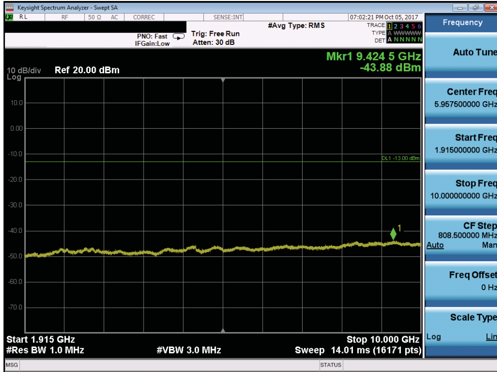
Plot 7-128. Conducted Spurious Plot (Band 25/2 - 15.0MHz QPSK - RB Size 1, RB Offset 0 - Mid Channel)
