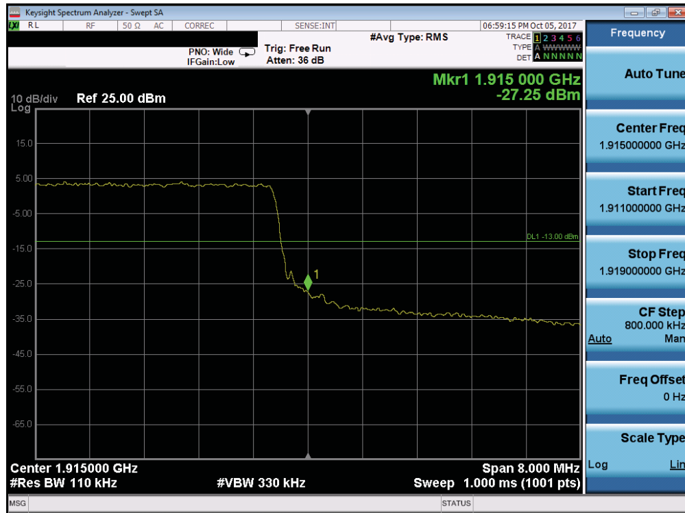
Plot 7-237. Upper Band Edge Plot (Band 25 - 10.0MHz QPSK - Full RB Configuration)
