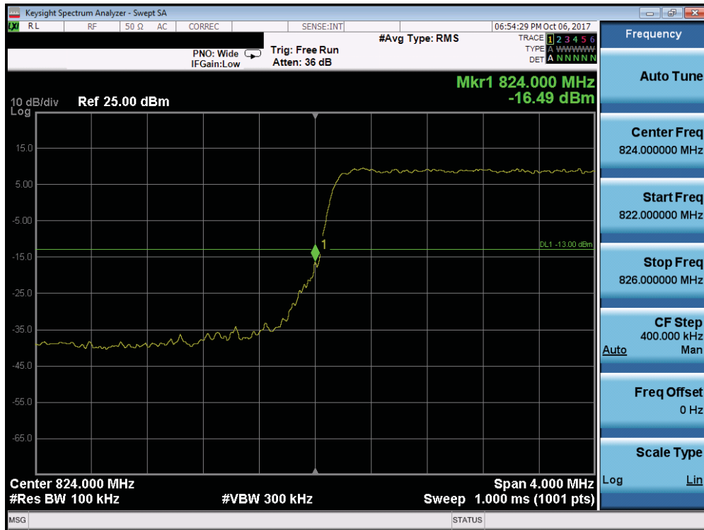
Plot 7-171. Lower Band Edge Plot (Band 5/26 – 3MHz QPSK - Full RB Configuration)
