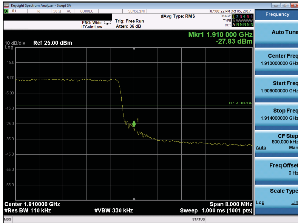
Plot 7-235. Upper Band Edge Plot (Band 2 - 10.0MHz QPSK - Full RB Configuration)
