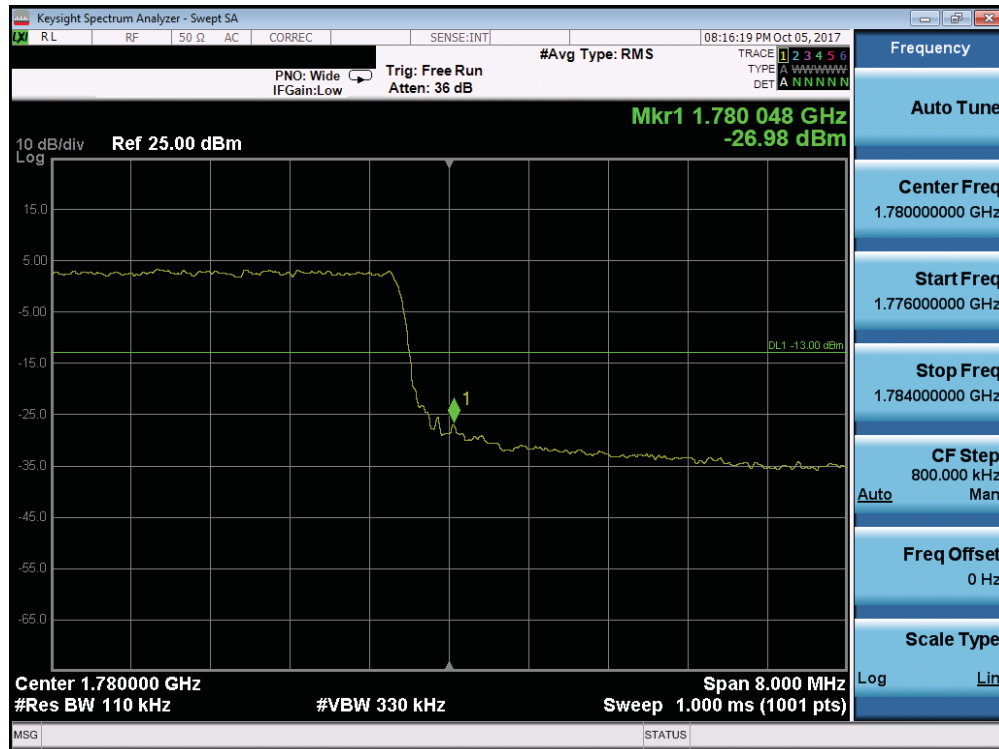
Plot 7-201. Upper Band Edge Plot (Band 66 - 10.0MHz QPSK - Full RB Configuration)
