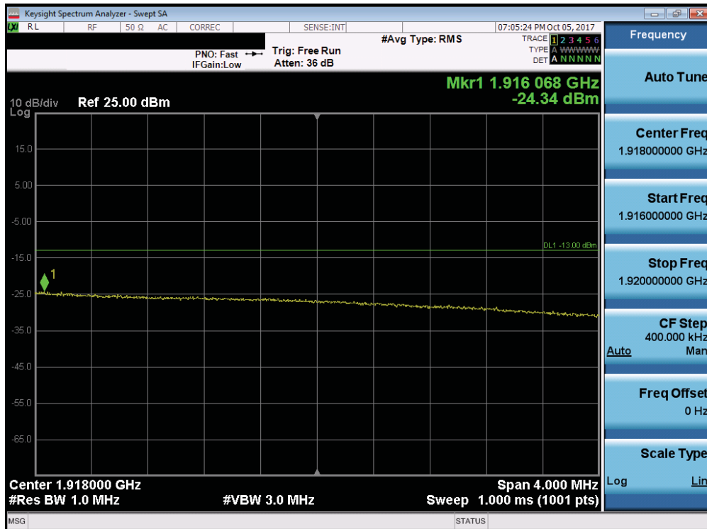
Plot 7-244. Upper Extended Band Edge Plot (Band 25 - 15.0MHz QPSK - Full RB Configuration)
