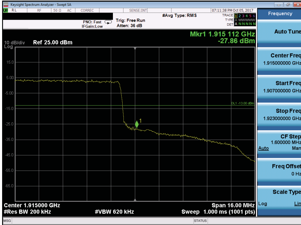
Plot 7-249. Upper Band Edge Plot (Band 25 - 20.0MHz QPSK - Full RB Configuration)
