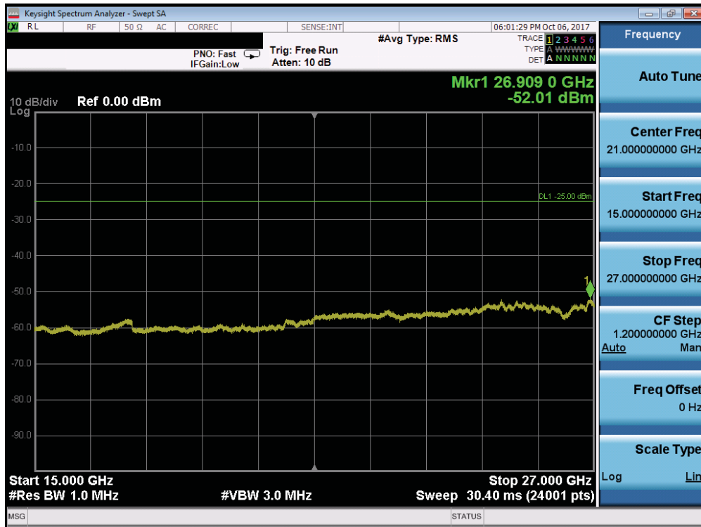
Plot 7-135. Conducted Spurious Plot (Band 7 - 5.0MHz QPSK - RB Size 1, RB Offset 0 - Low Channel)
