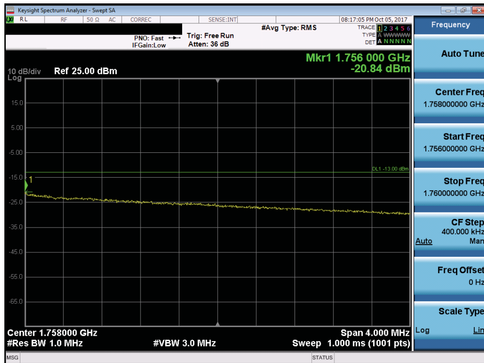
Plot 7-200. Upper Extended Band Edge Plot (Band 4 - 10.0MHz QPSK - Full RB Configuration)
