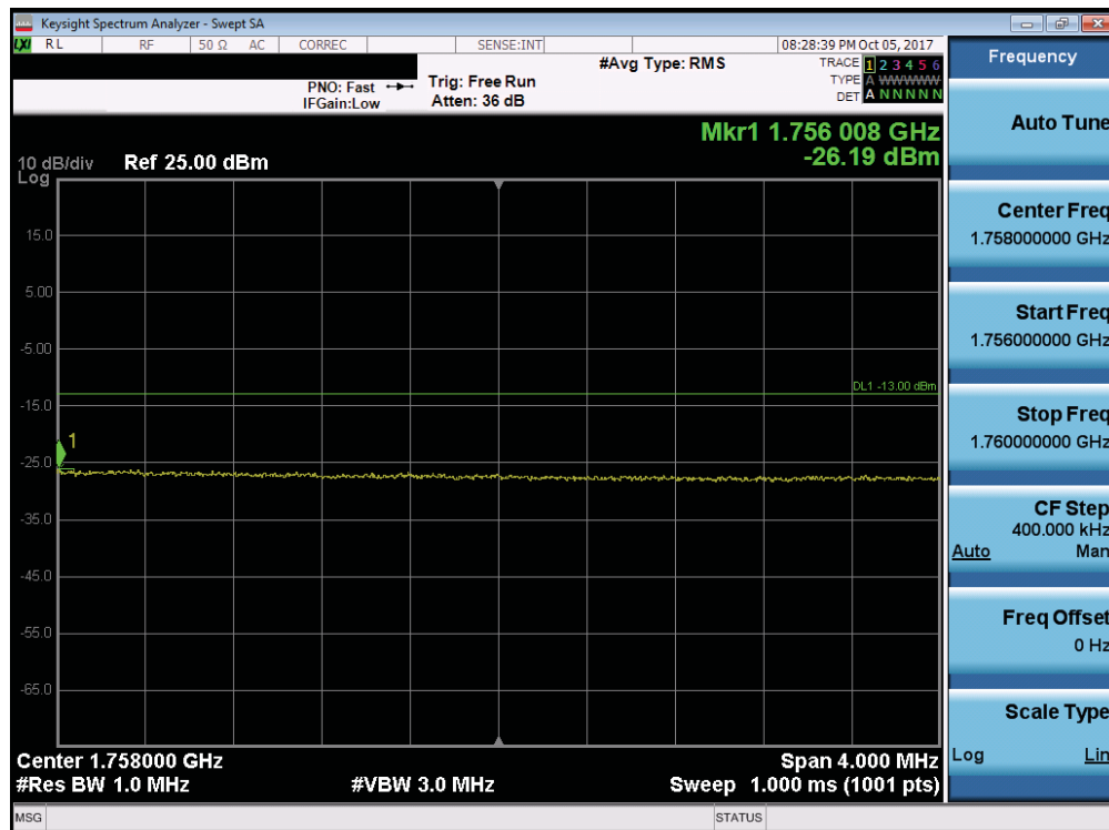
Plot 7-212. Upper Extended Band Edge Plot (Band 4 - 20.0MHz QPSK - Full RB Configuration)
