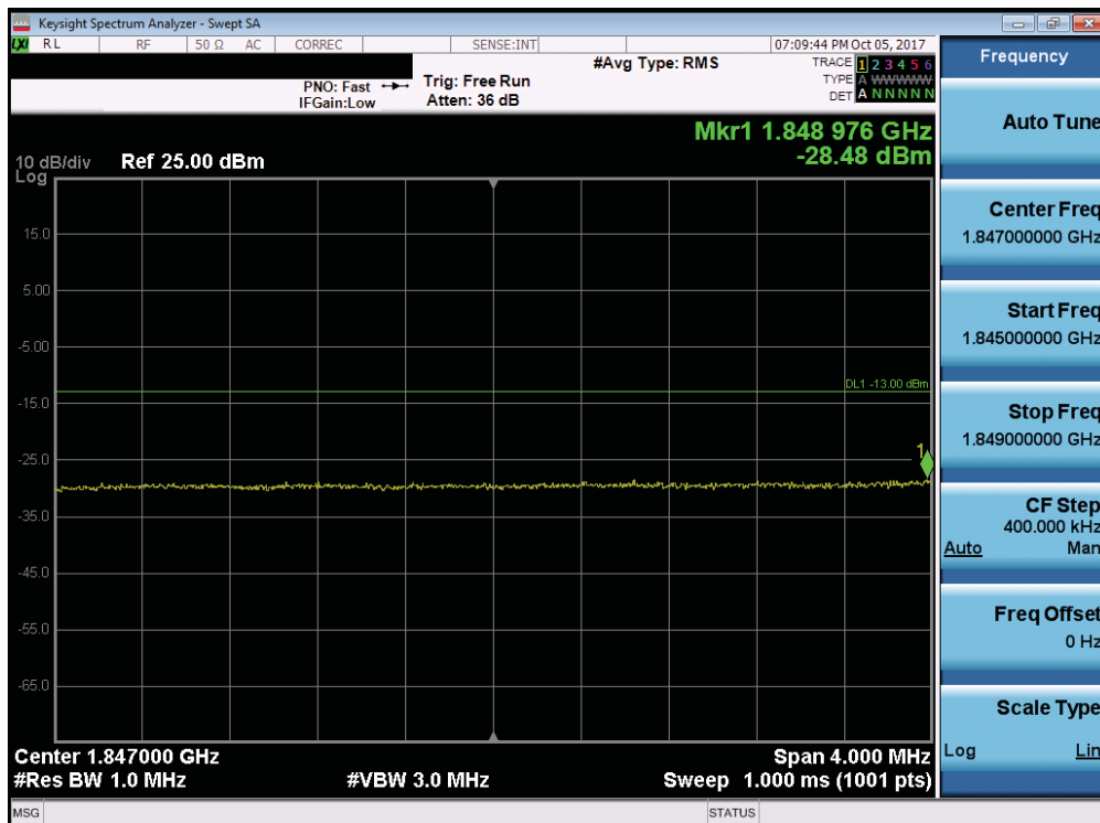
Plot 7-246. Lower Extended Band Edge Plot (Band 25/2 - 20.0MHz QPSK - Full RB Configuration)
