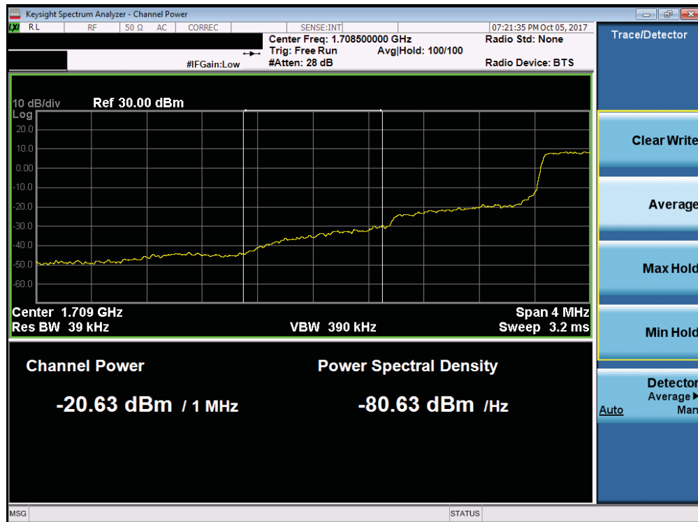
Plot 7-180. Lower Extended Band Edge Plot (Band 66/4 - 1.4MHz QPSK - Full RB Configuration)
