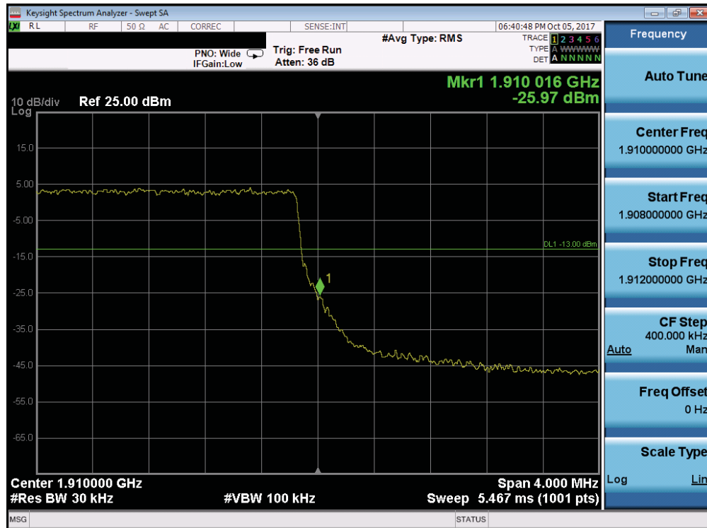
Plot 7-223. Upper Band Edge Plot (Band 2 - 3.0MHz QPSK - Full RB Configuration)
