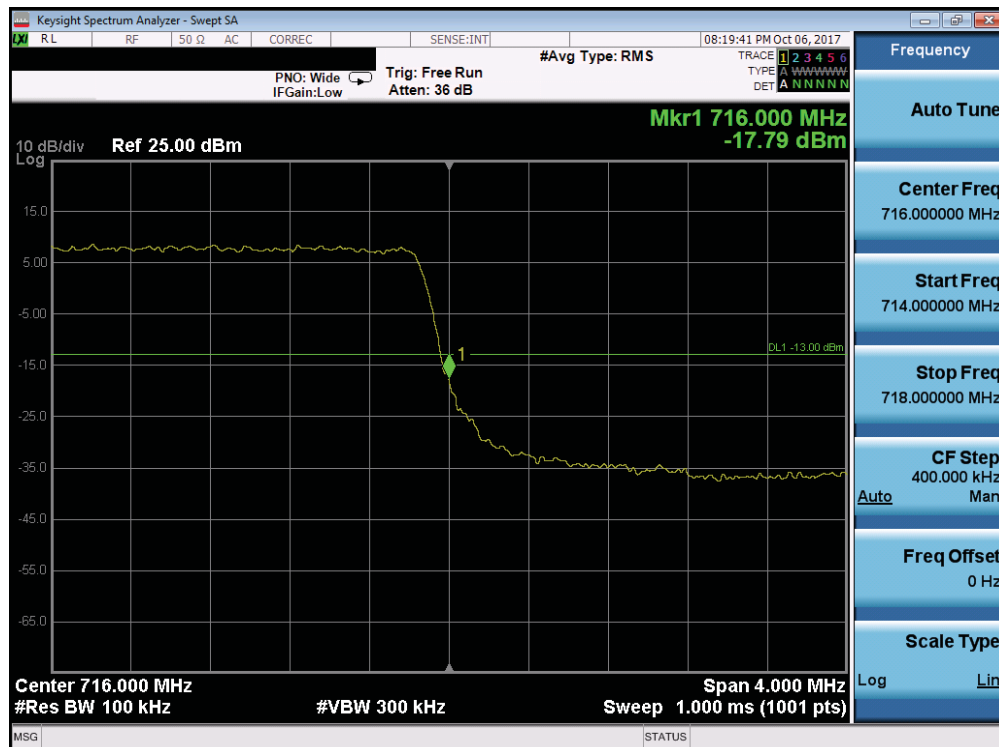
Plot 7-154. Upper Band Edge Plot (Band 12 - 3.0MHz QPSK - Full RB Configuration)
