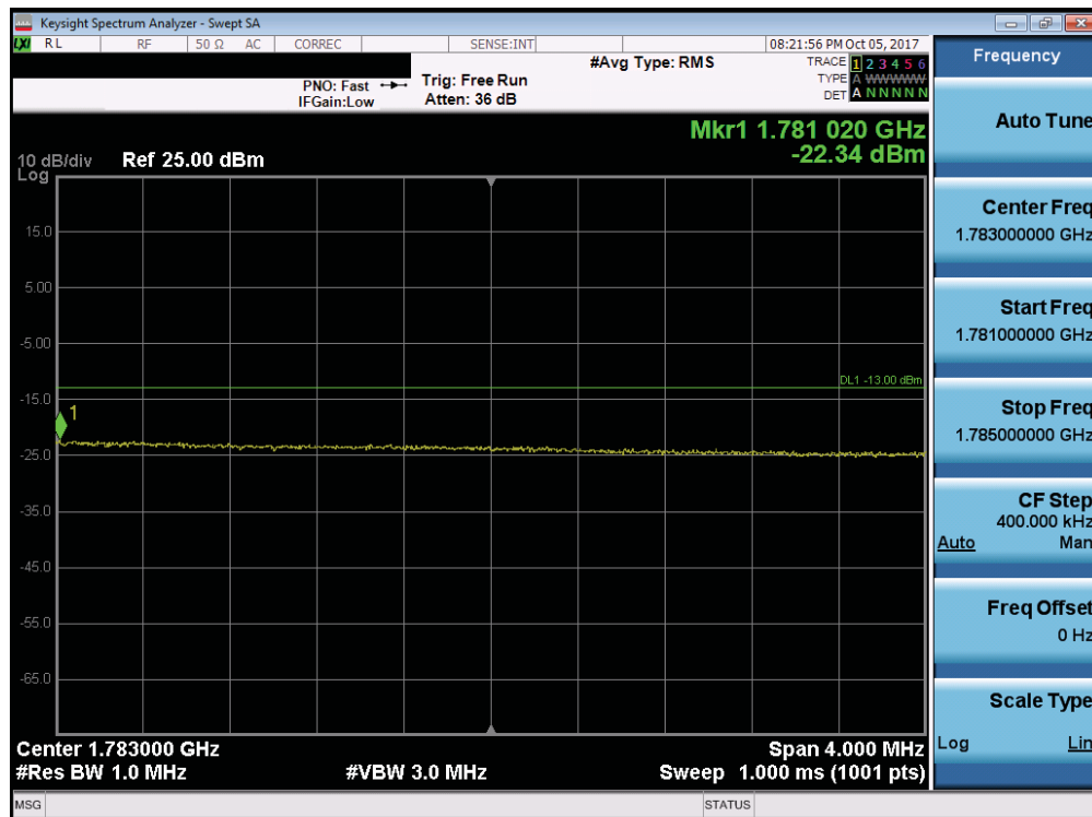
Plot 7-208. Upper Extended Band Edge Plot (Band 66 - 15.0MHz QPSK - Full RB Configuration)
