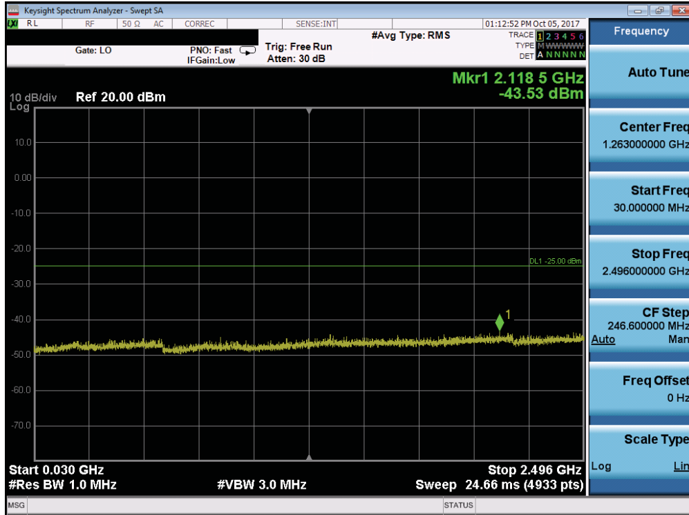
Plot 7-148. Conducted Spurious Plot (Band 38/41 - 10.0MHz QPSK - RB Size 1, RB Offset 0 - High Channel)
