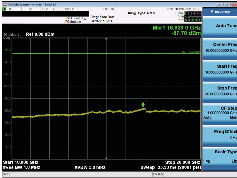
Plot 7-126. Conducted Spurious Plot (Band 25/2 - 15.0MHz QPSK - RB Size 1, RB Offset 0 - Low Channel)
