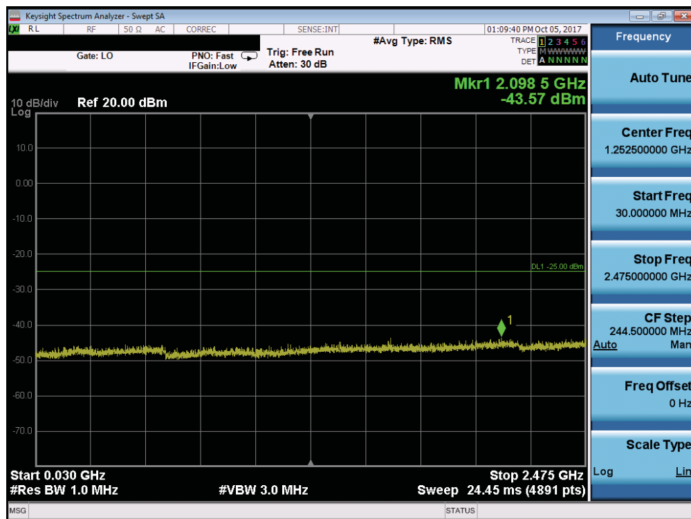
Plot 7-142. Conducted Spurious Plot (Band 38/41 - 10.0MHz QPSK - RB Size 1, RB Offset 0 - Low Channel)
