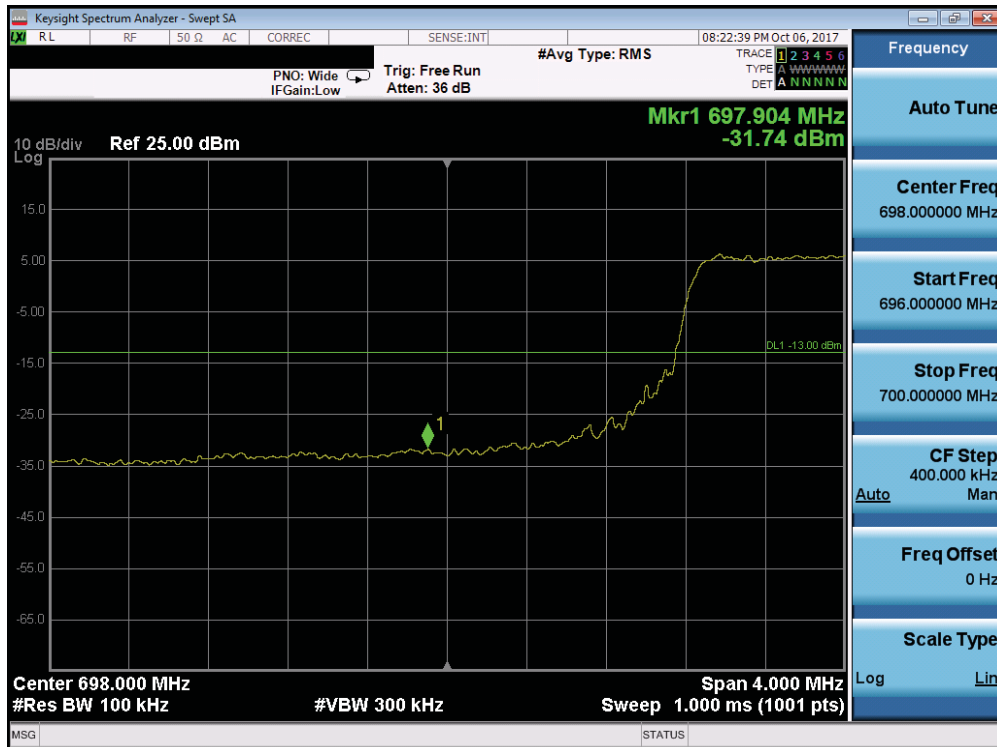
Plot 7-155. Lower Band Edge Plot (Band 12 - 5.0MHz QPSK - Full RB Configuration)
