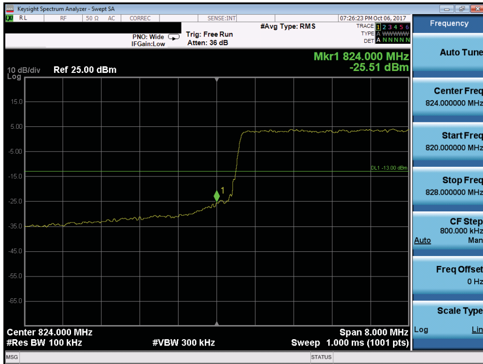
Plot 7-175. Lower Band Edge Plot (Band 5/26 – 10MHz QPSK - Full RB Configuration)
