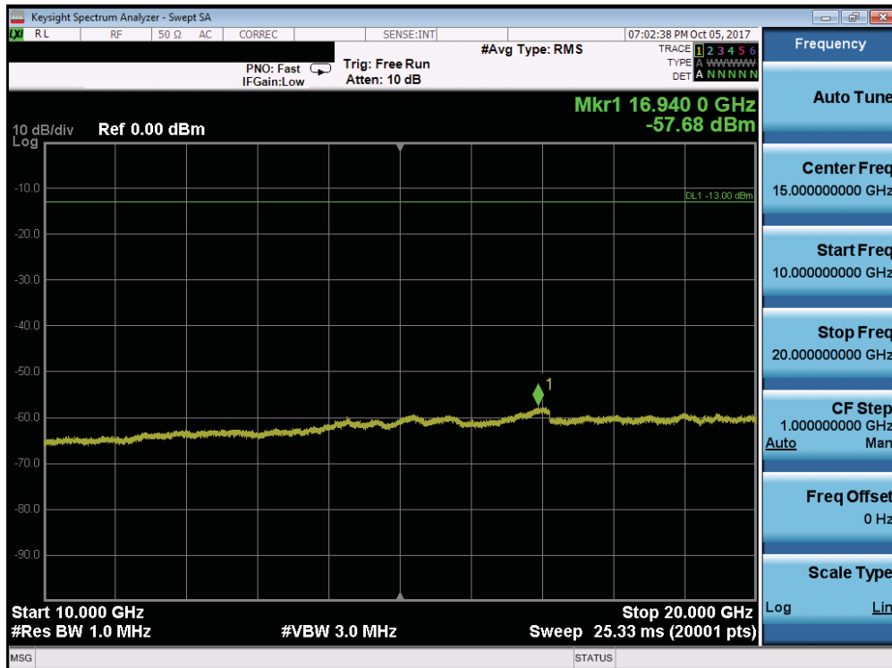
Plot 7-129. Conducted Spurious Plot (Band 25/2 - 15.0MHz QPSK - RB Size 1, RB Offset 0 - Mid Channel)
