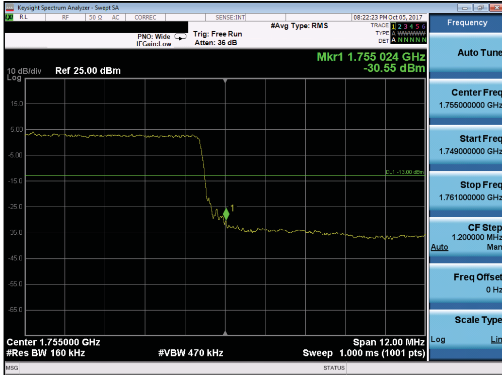
Plot 7-205. Upper Band Edge Plot (Band 4 - 15.0MHz QPSK - Full RB Configuration)
