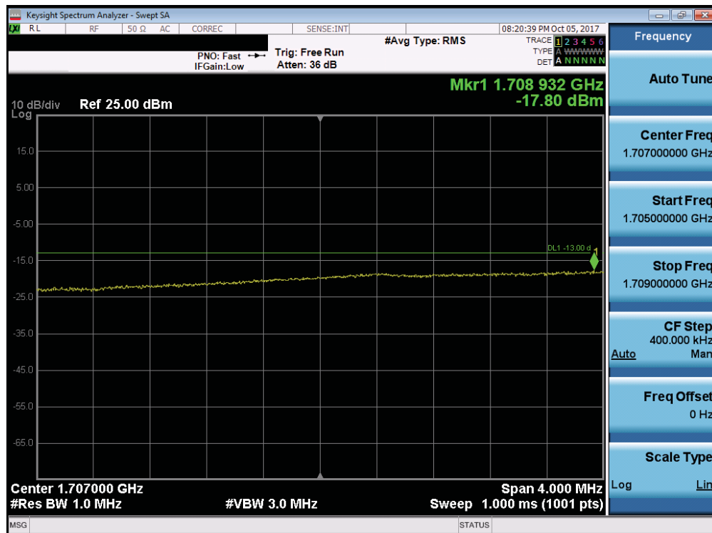
Plot 7-204. Lower Extended Band Edge Plot (Band 66/4 - 15.0MHz QPSK - Full RB Configuration)
