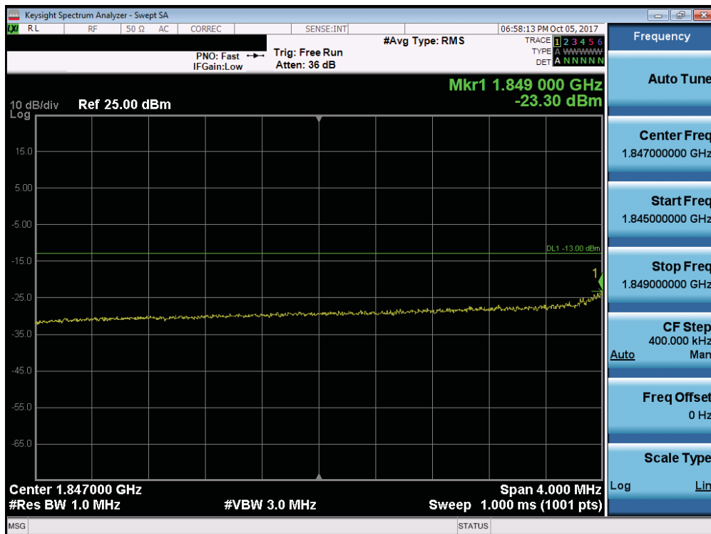
Plot 7-234. Lower Extended Band Edge Plot (Band 25/2 - 10.0MHz QPSK - Full RB Configuration)
