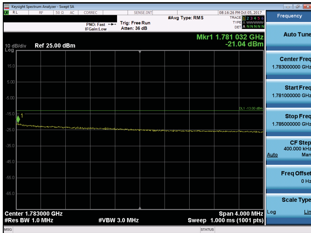
Plot 7-202. Upper Extended Band Edge Plot (Band 66 - 10.0MHz QPSK - Full RB Configuration)
