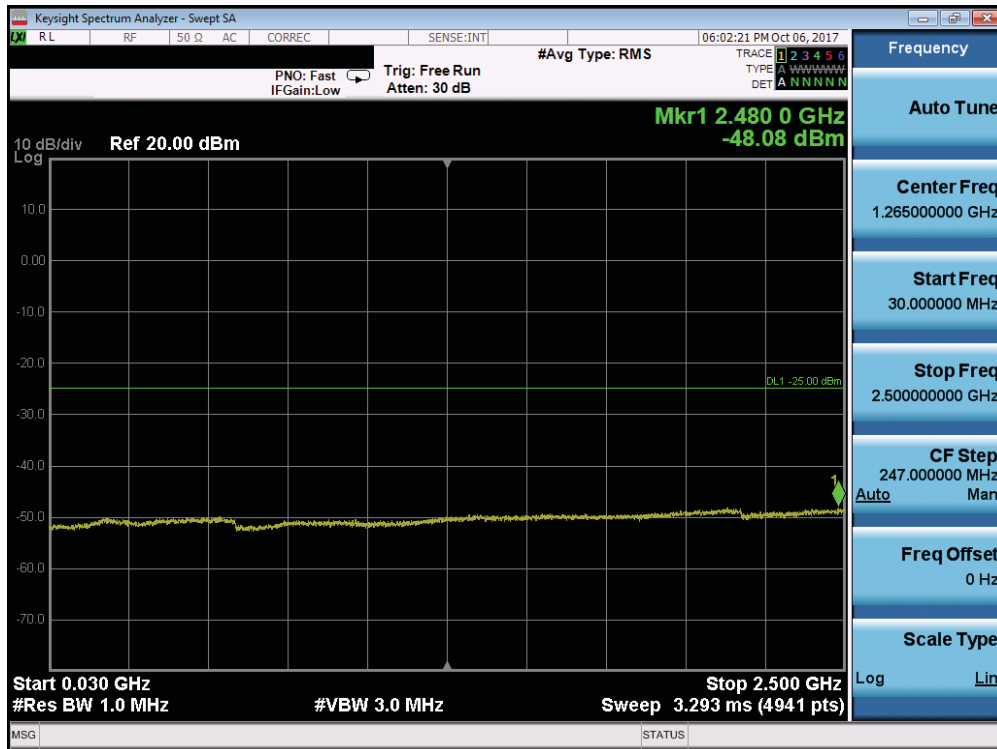
Plot 7-139. Conducted Spurious Plot (Band 7 - 5.0MHz QPSK - RB Size 1, RB Offset 0 - High Channel)
