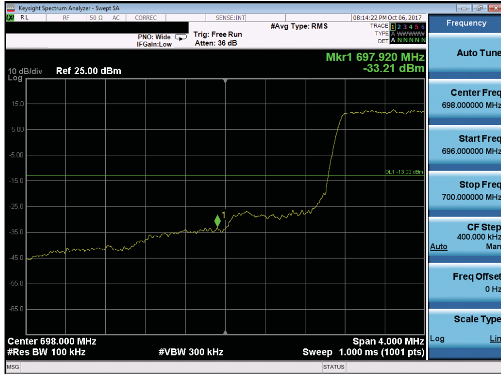
Plot 7-151. Lower Band Edge Plot (Band 12 - 1.4MHz QPSK - Full RB Configuration)
