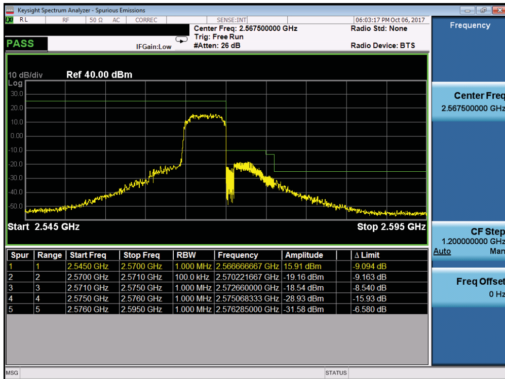
Plot 7-252. Upper ACP Plot (Band 7 - 5.0MHz QPSK - RB Size 25)
