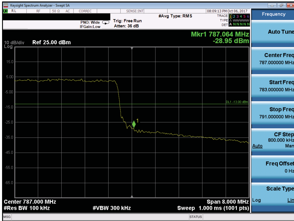
Plot 7-167. Upper Band Edge Plot (Band 13 - 10.0MHz QPSK - Full RB Configuration)
