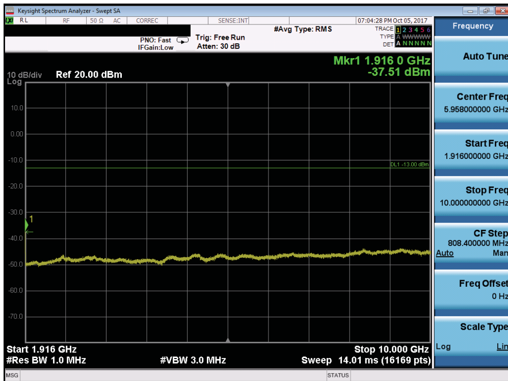
Plot 7-131. Conducted Spurious Plot (Band 25/2 - 15.0MHz QPSK - RB Size 1, RB Offset 0 - High Channel)
