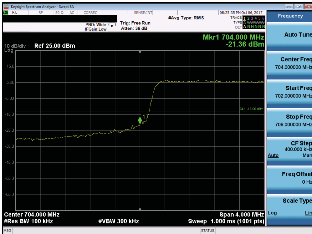
Plot 7-156. Lower Band Edge Plot (Band 17 - 5.0MHz QPSK - Full RB Configuration)
