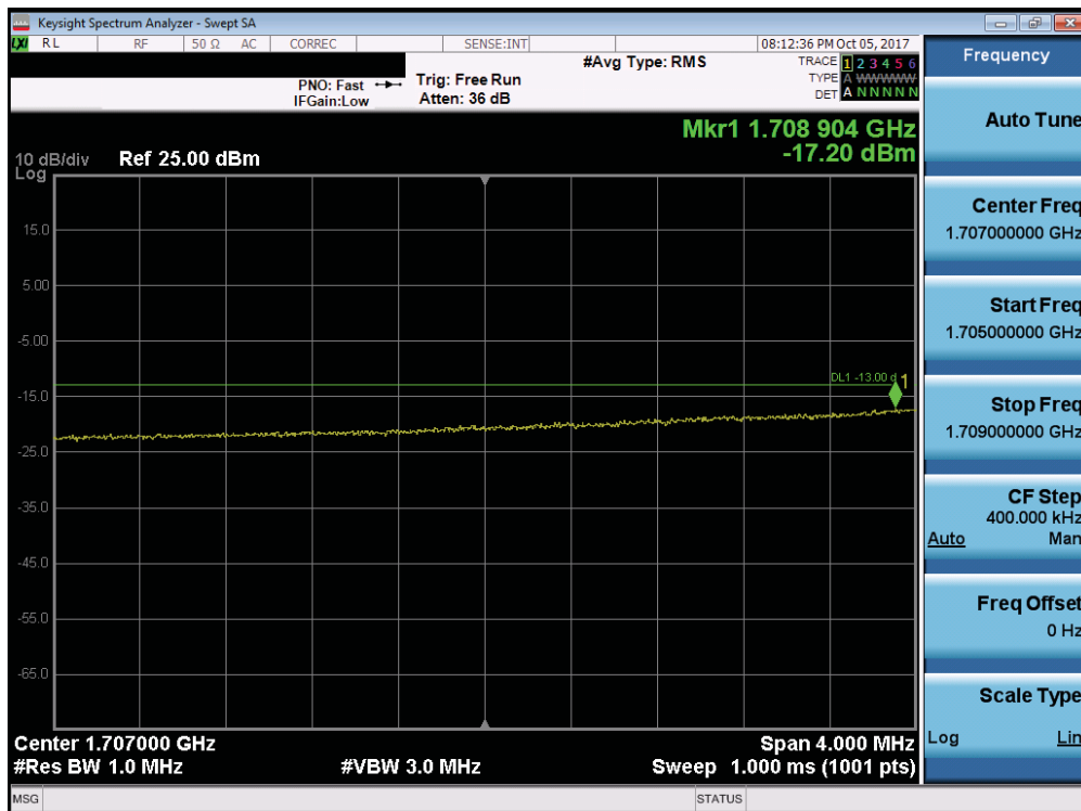
Plot 7-198. Lower Extended Band Edge Plot (Band 66/4 - 10.0MHz QPSK - Full RB Configuration)
