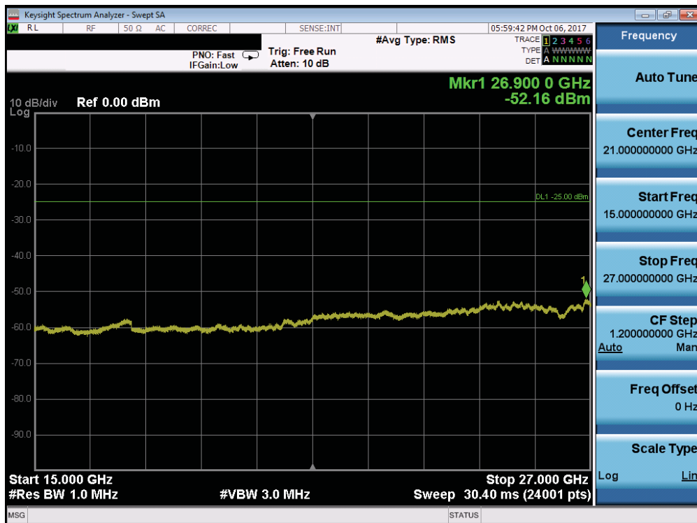
Plot 7-138. Conducted Spurious Plot (Band 7 - 5.0MHz QPSK - RB Size 1, RB Offset 0 - Mid Channel)
