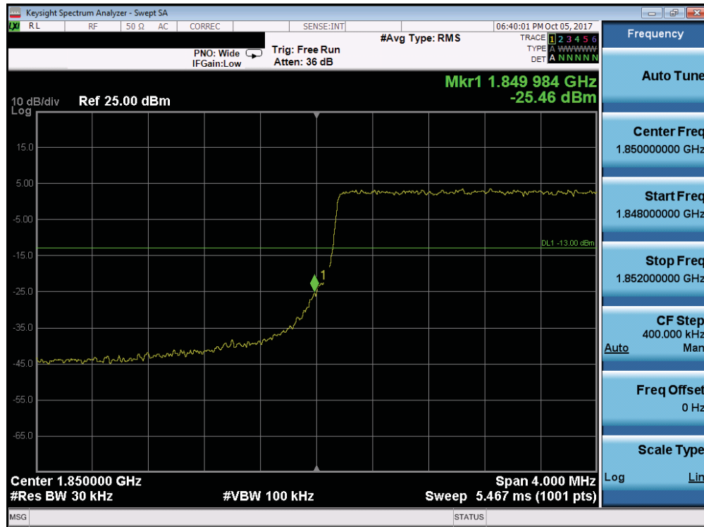
Plot 7-221. Lower Band Edge Plot (Band 25/2 - 3.0MHz QPSK - Full RB Configuration)
