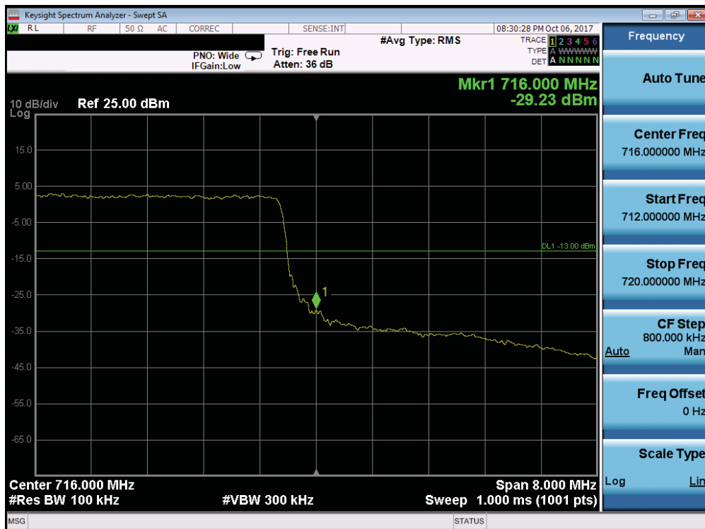
Plot 7-160. Upper Band Edge Plot (Band 12/17 - 10.0MHz QPSK - Full RB Configuration)
