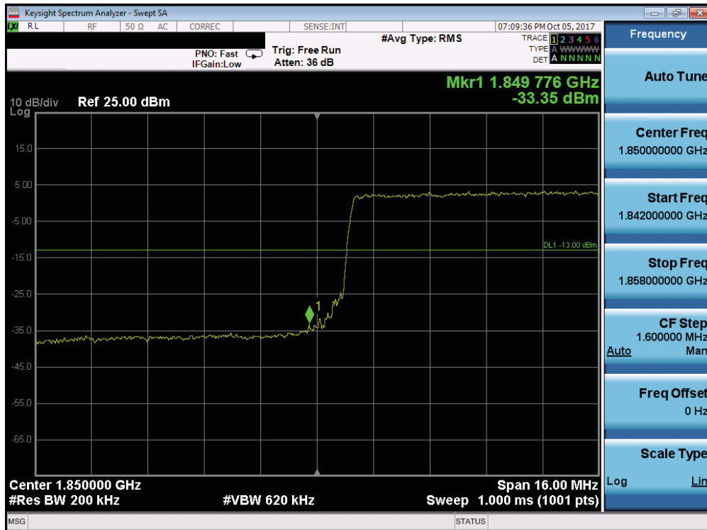
Plot 7-245. Lower Band Edge Plot (Band 25/2 - 20.0MHz QPSK - Full RB Configuration)
