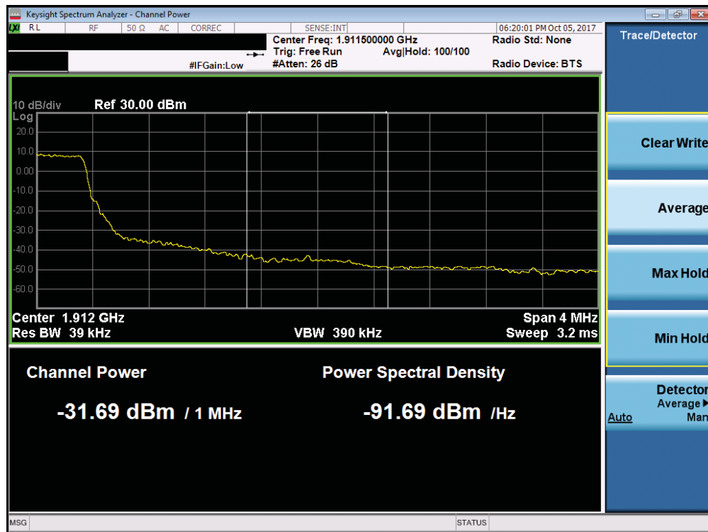
Plot 7-218. Upper Extended Band Edge Plot (Band 2 - 1.4MHz QPSK - Full RB Configuration)
