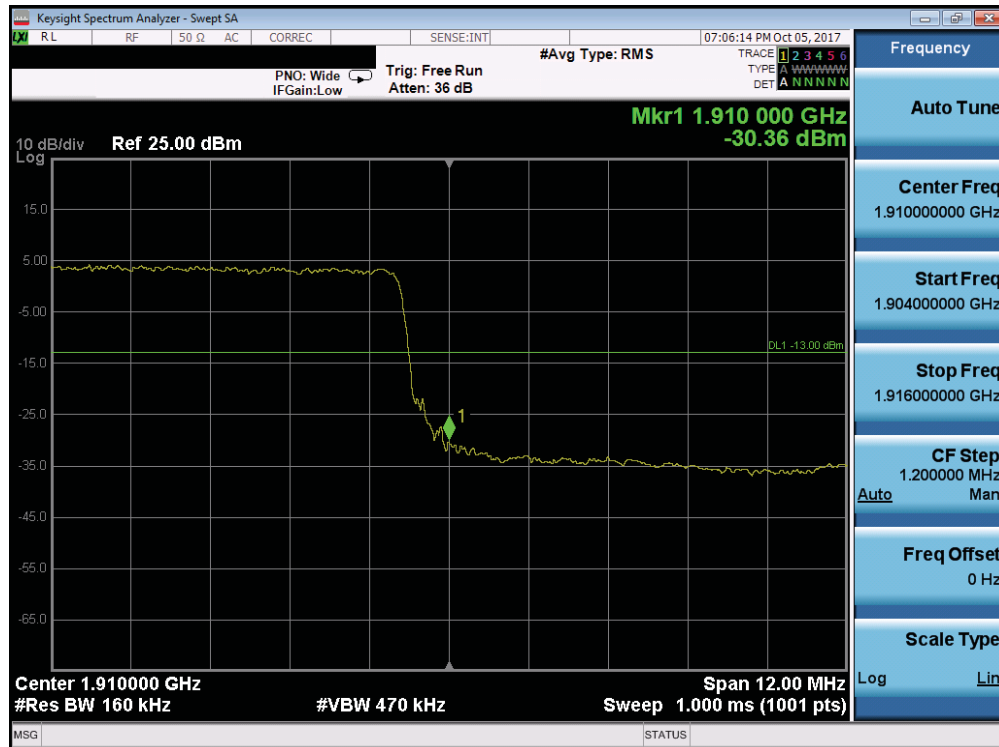
Plot 7-241. Upper Band Edge Plot (Band 2 - 15.0MHz QPSK - Full RB Configuration)
