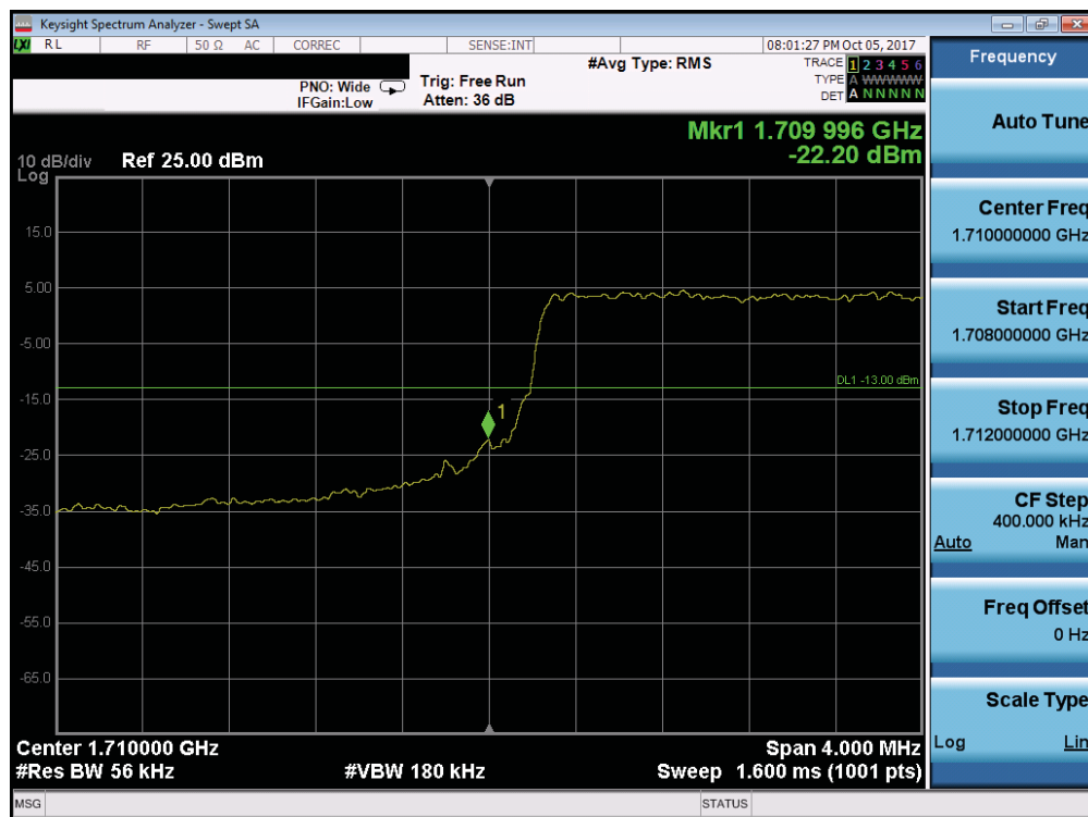
Plot 7-191. Lower Band Edge Plot (Band 66/4 - 5.0MHz QPSK - Full RB Configuration)
