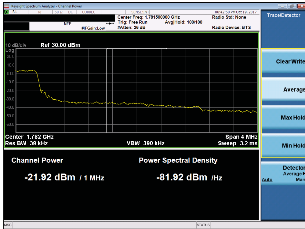
Plot 7-190. Upper Extended Band Edge Plot (Band 66 - 3.0MHz QPSK - Full RB Configuration)
