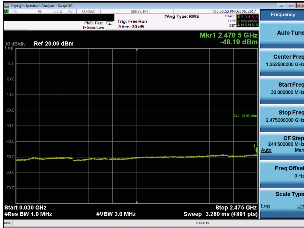
Plot 7-133. Conducted Spurious Plot (Band 7 - 5.0MHz QPSK - RB Size 1, RB Offset 0 - Low Channel)
