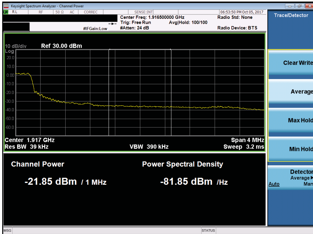
Plot 7-232. Upper Extended Band Edge Plot (Band 25 - 5.0MHz QPSK - Full RB Configuration)
