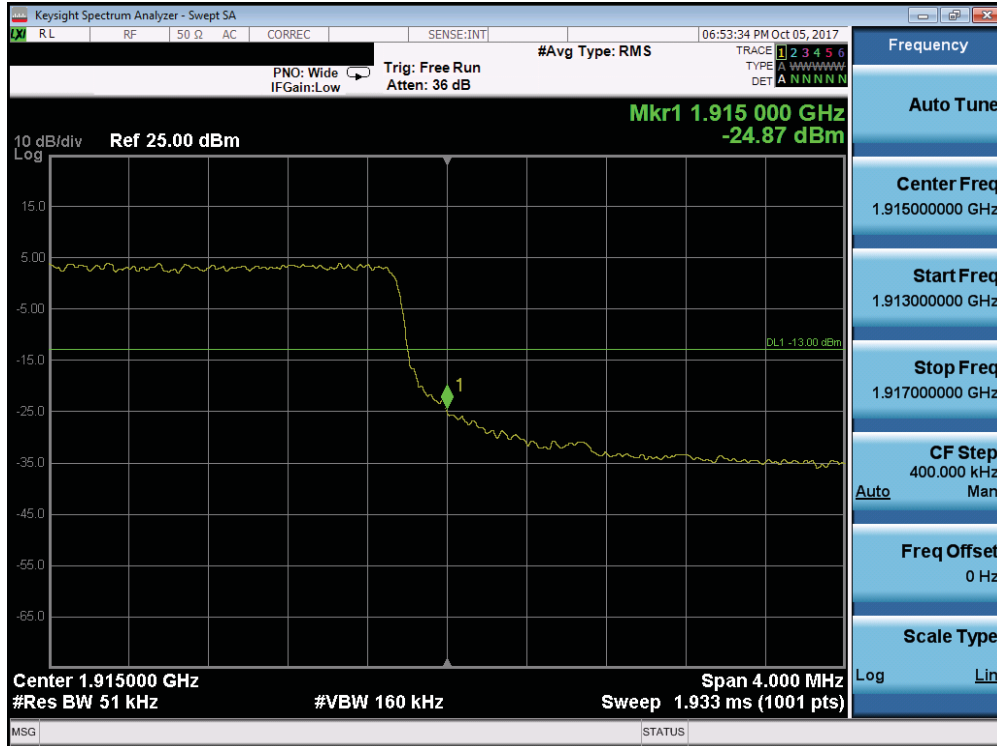
Plot 7-231. Upper Band Edge Plot (Band 25 - 5.0MHz QPSK - Full RB Configuration)
