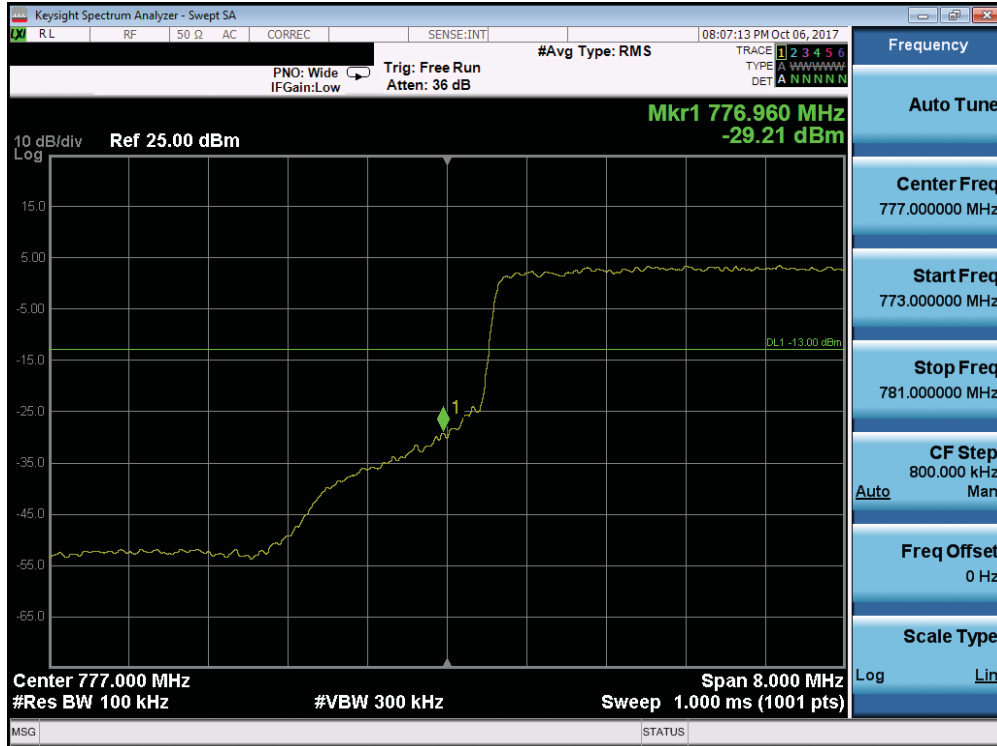
Plot 7-165. Lower Band Edge Plot (Band 13 - 10.0MHz QPSK - Full RB Configuration)
