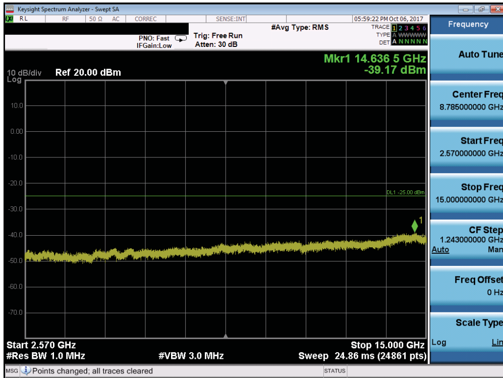
Plot 7-137. Conducted Spurious Plot (Band 7 - 5.0MHz QPSK - RB Size 1, RB Offset 0 - Mid Channel)
