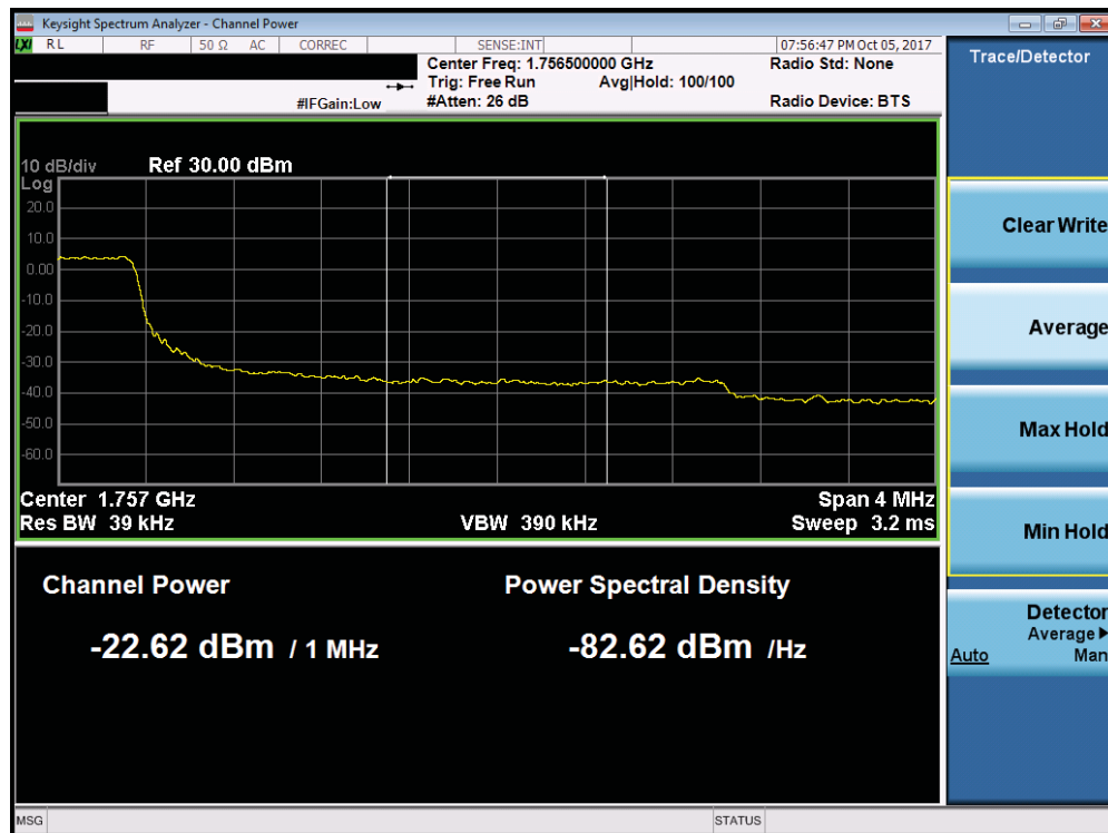
Plot 7-188. Upper Extended Band Edge Plot (Band 4 - 3.0MHz QPSK - Full RB Configuration)
