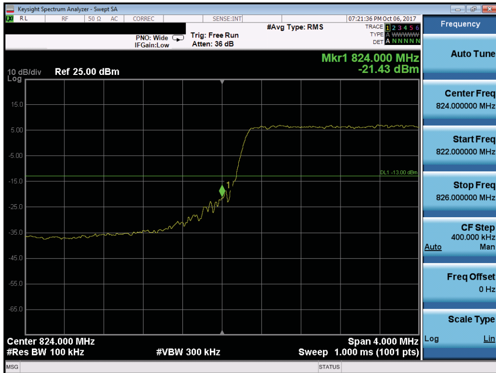
Plot 7-173. Lower Band Edge Plot (Band 5/26 – 5MHz QPSK - Full RB Configuration)
