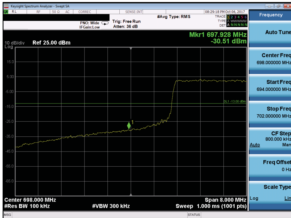
Plot 7-158. Lower Band Edge Plot (Band 12 - 10.0MHz QPSK - Full RB Configuration)
