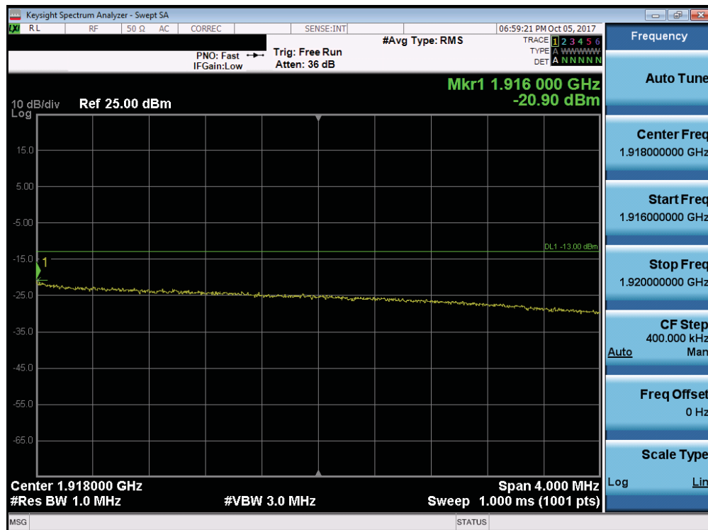
Plot 7-238. Upper Extended Band Edge Plot (Band 25 - 10.0MHz QPSK - Full RB Configuration)
