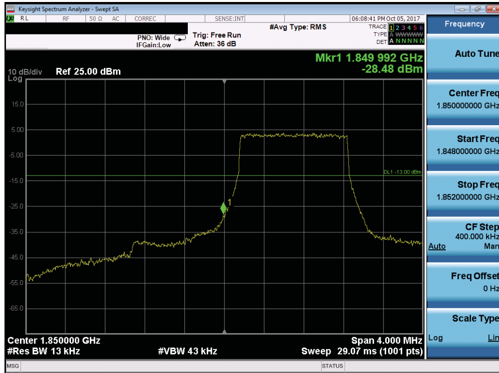
Plot 7-215. Lower Band Edge Plot (Band 25/2 - 1.4MHz QPSK - Full RB Configuration)
