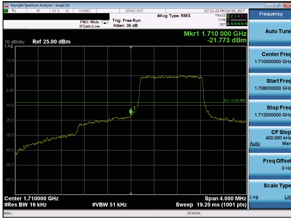
Plot 7-179. Lower Band Edge Plot (Band 66/4 - 1.4MHz QPSK - Full RB Configuration)
