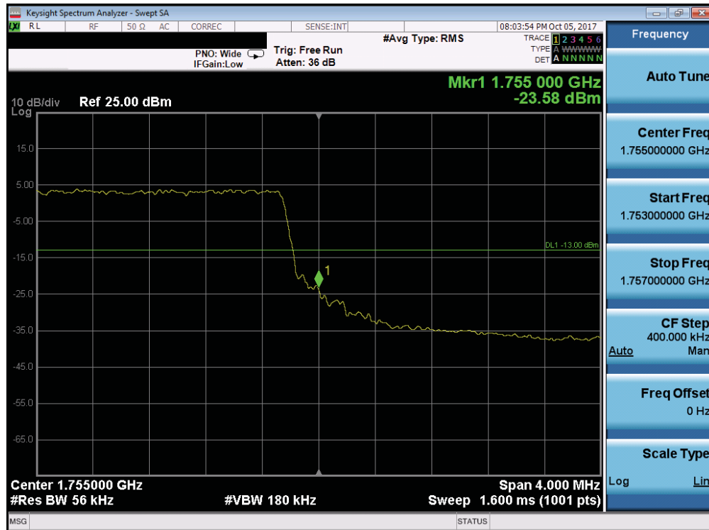
Plot 7-193. Upper Band Edge Plot (Band 4 - 5.0MHz QPSK - Full RB Configuration)
