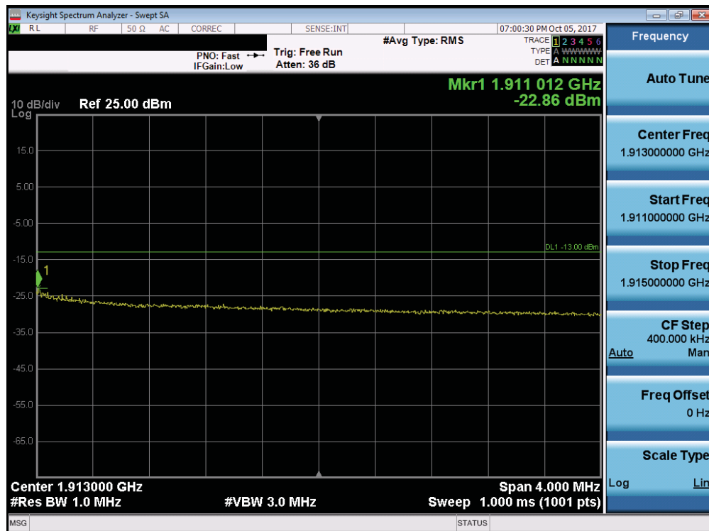
Plot 7-236. Upper Extended Band Edge Plot (Band 2 - 10.0MHz QPSK - Full RB Configuration)
