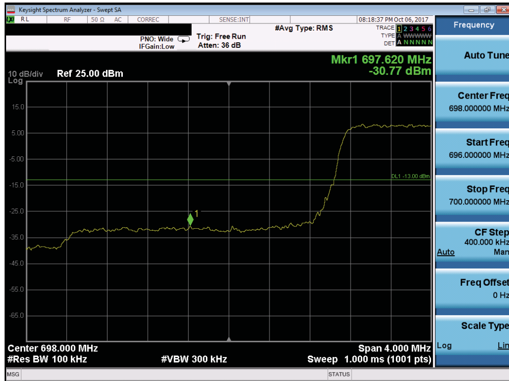
Plot 7-153. Lower Band Edge Plot (Band 12 - 3.0MHz QPSK - Full RB Configuration)
