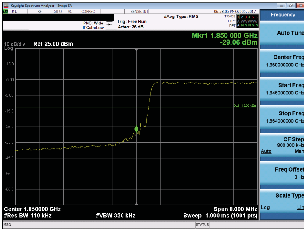
Plot 7-233. Lower Band Edge Plot (Band 25/2 - 10.0MHz QPSK - Full RB Configuration)
