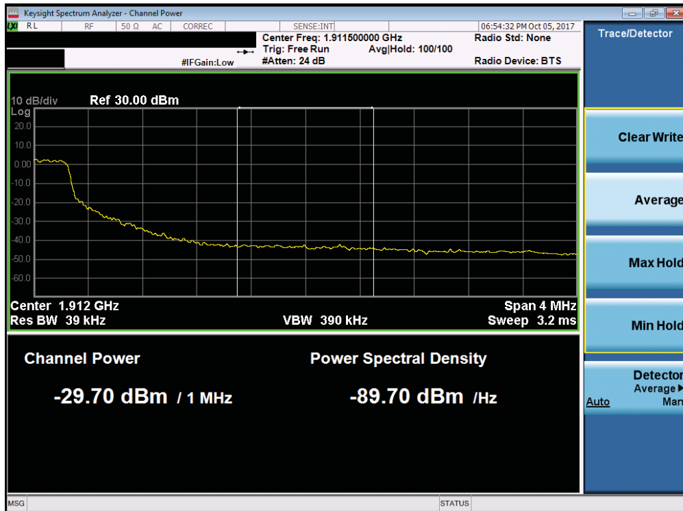
Plot 7-230. Upper Extended Band Edge Plot (Band 2 - 5.0MHz QPSK - Full RB Configuration)
