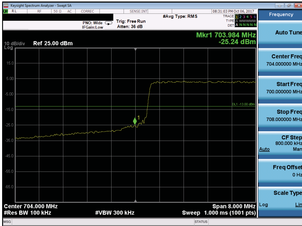
Plot 7-159. Lower Band Edge Plot (Band 17 - 10.0MHz QPSK - Full RB Configuration)
