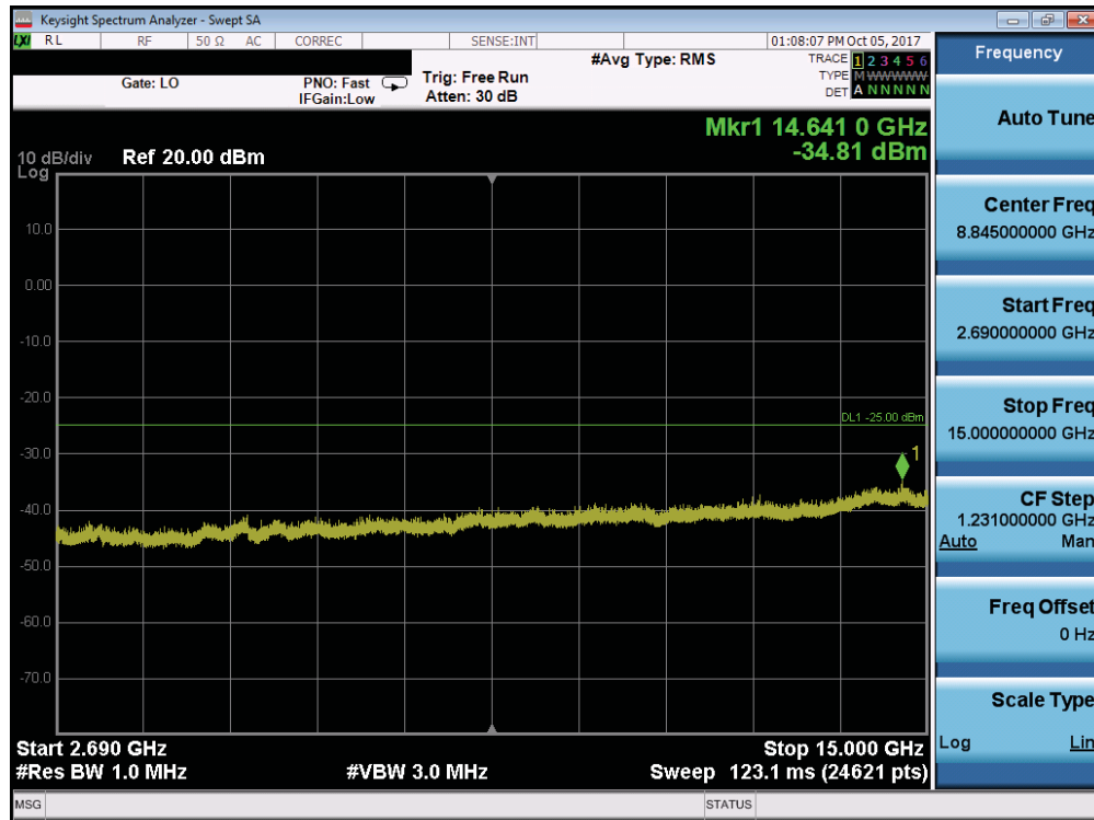
Plot 7-146. Conducted Spurious Plot (Band 38/41 - 10.0MHz QPSK - RB Size 1, RB Offset 0 - Mid Channel)
