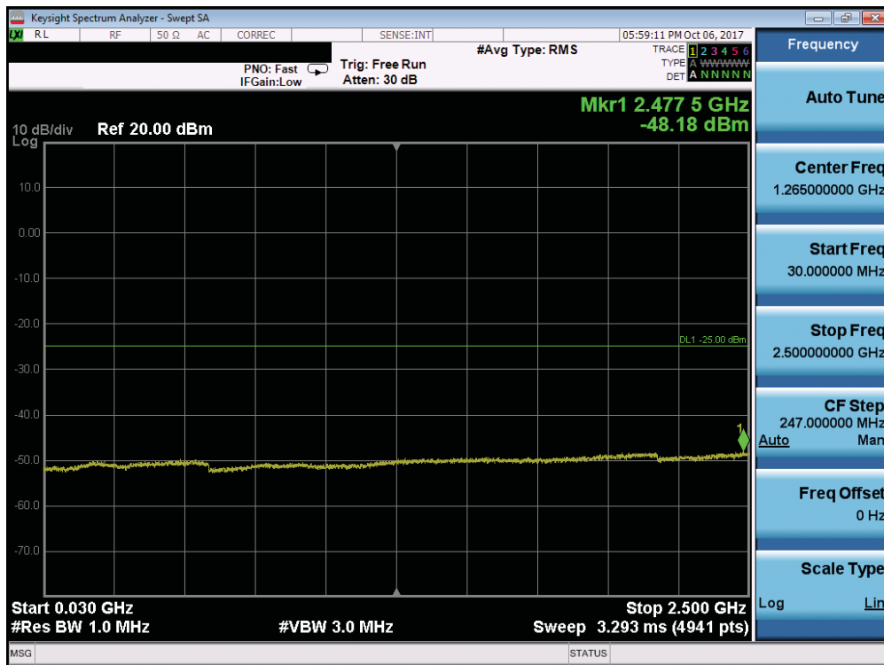
Plot 7-136. Conducted Spurious Plot (Band 7 - 5.0MHz QPSK - RB Size 1, RB Offset 0 - Mid Channel)
