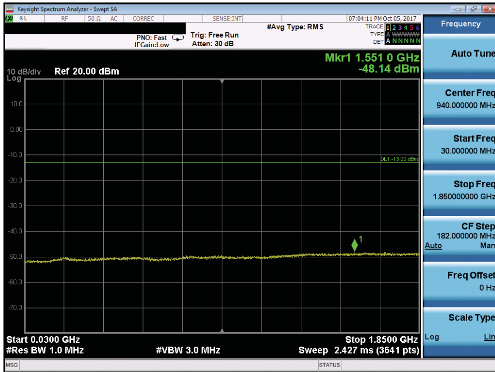
Plot 7-130. Conducted Spurious Plot (Band 25/2 - 15.0MHz QPSK - RB Size 1, RB Offset 0 - High Channel)
