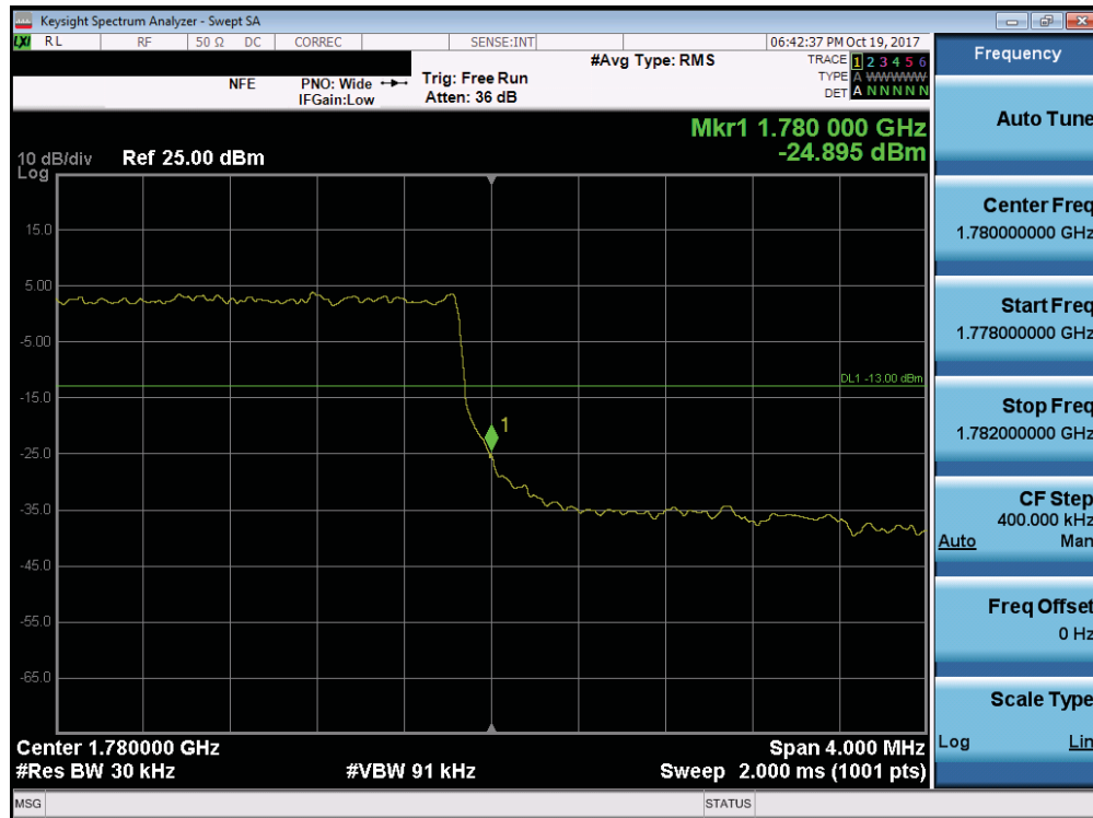
Plot 7-189. Upper Band Edge Plot (Band 66 - 3.0MHz QPSK - Full RB Configuration)
