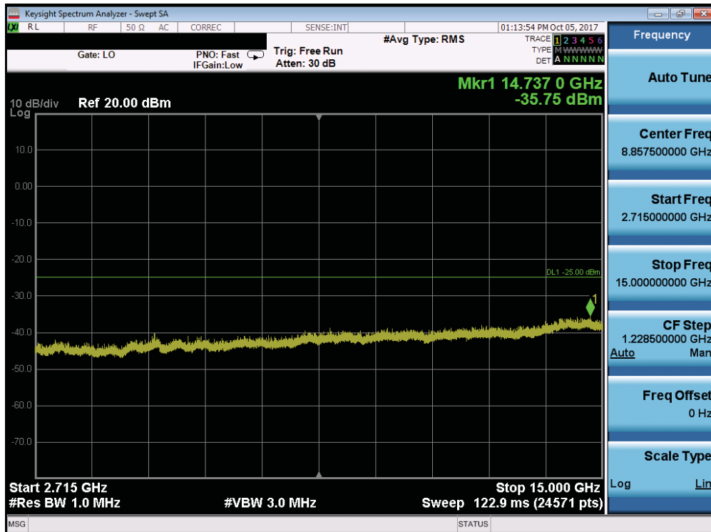
Plot 7-149. Conducted Spurious Plot (Band 38/41 - 10.0MHz QPSK - RB Size 1, RB Offset 0 - High Channel)
