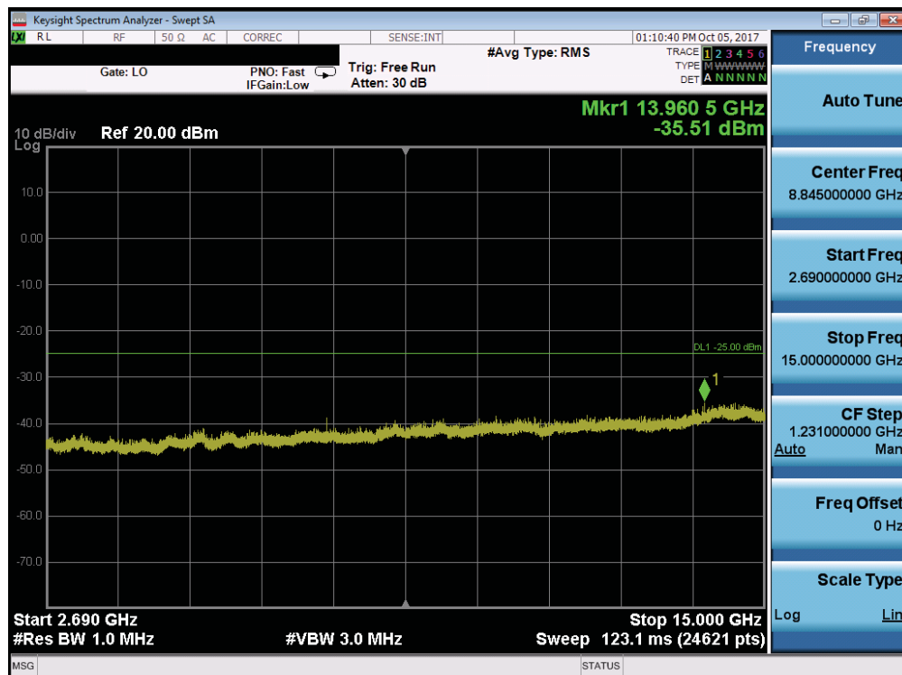
Plot 7-143. Conducted Spurious Plot (Band 38/41 - 10.0MHz QPSK - RB Size 1, RB Offset 0 - Low Channel)
