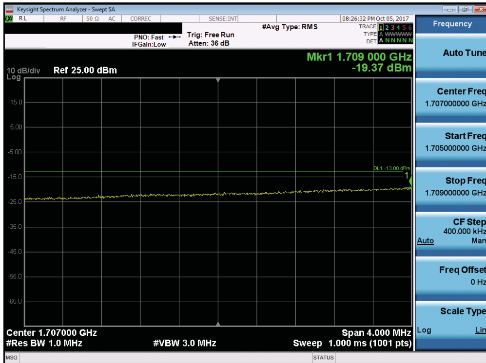
Plot 7-210. Lower Extended Band Edge Plot (Band 66/4 - 20.0MHz QPSK - Full RB Configuration)
