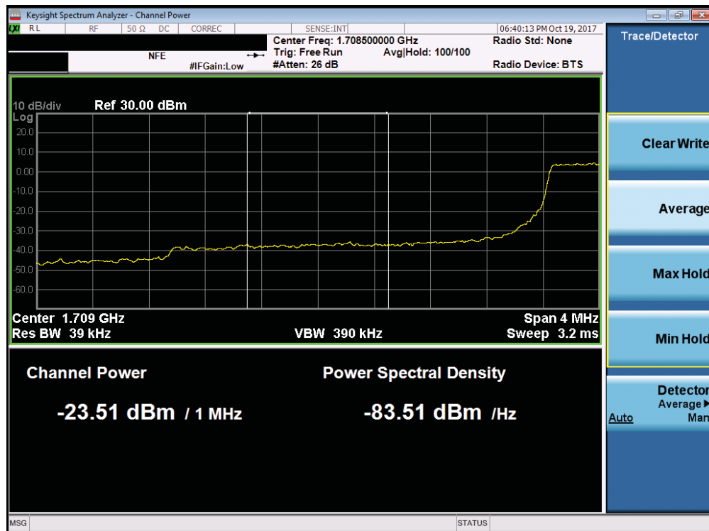
Plot 7-186. Lower Extended Band Edge Plot (Band 66/4 - 3.0MHz QPSK - Full RB Configuration)
