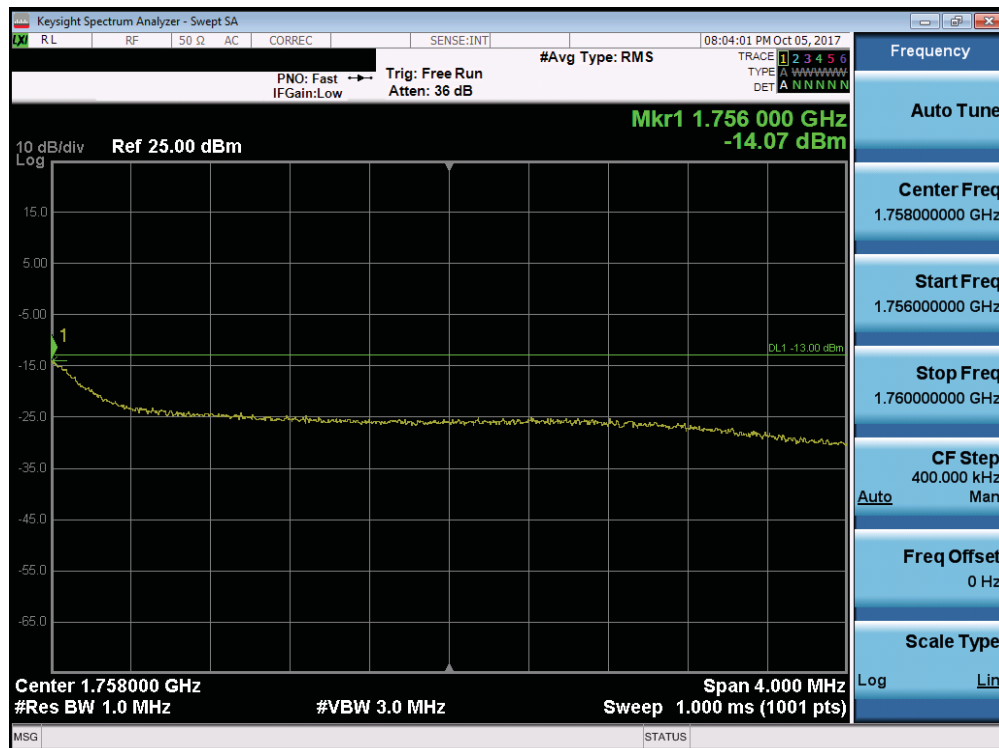
Plot 7-194. Upper Extended Band Edge Plot (Band 4 - 5.0MHz QPSK - Full RB Configuration)
