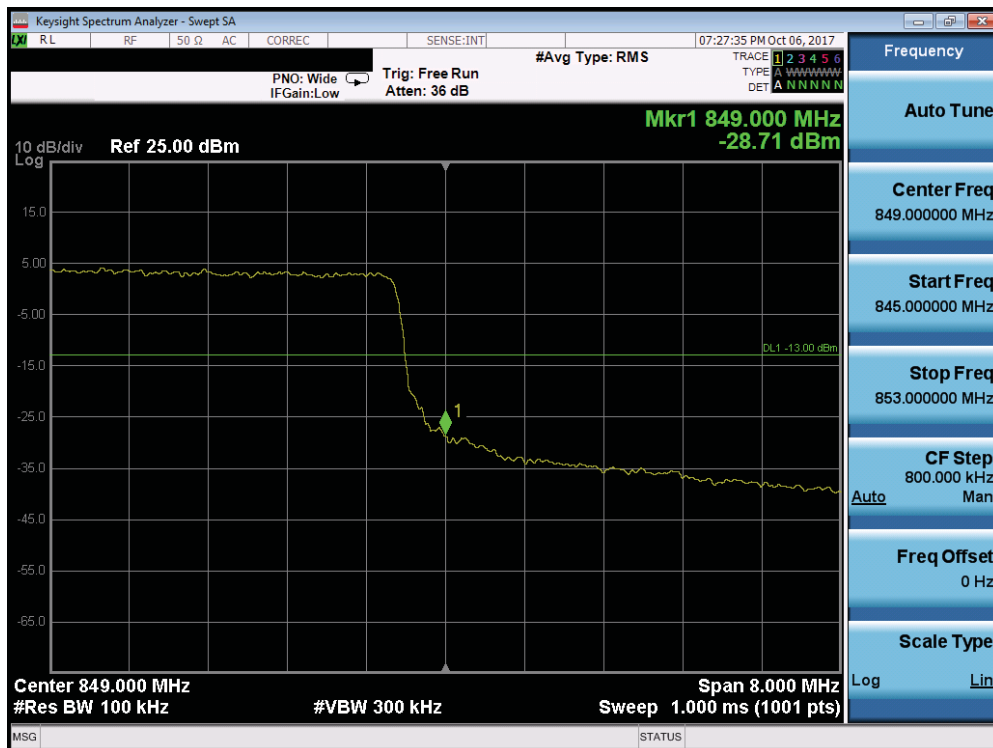
Plot 7-176. Upper Band Edge Plot (Band 5/26 – 10MHz QPSK - Full RB Configuration)
