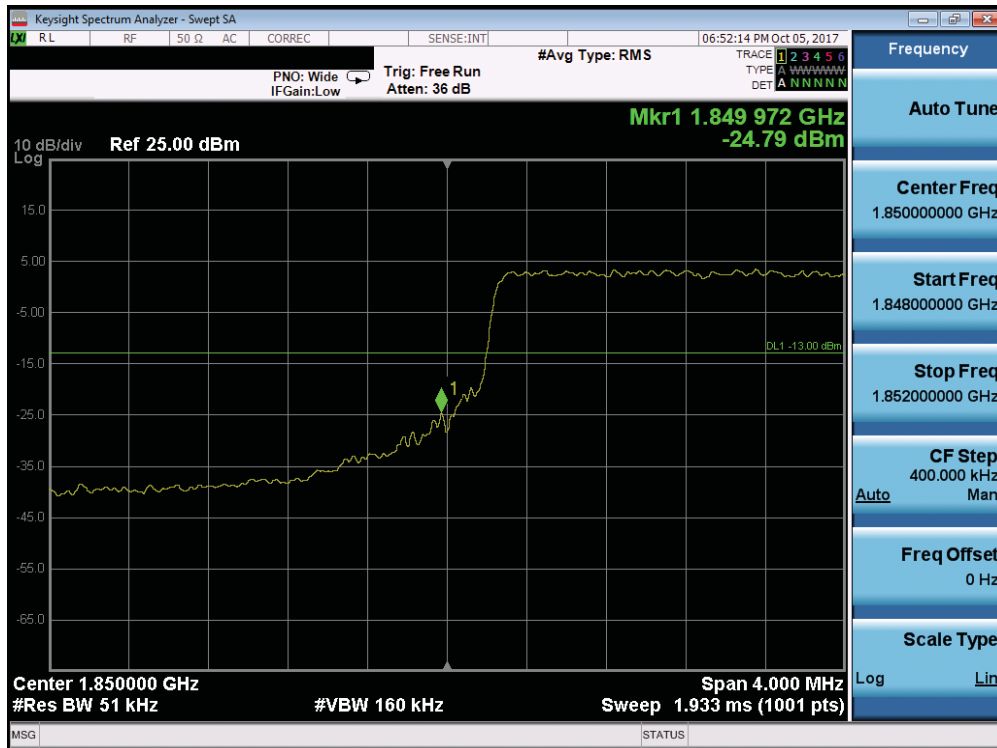
Plot 7-227. Lower Band Edge Plot (Band 25/2 - 5.0MHz QPSK - Full RB Configuration)
