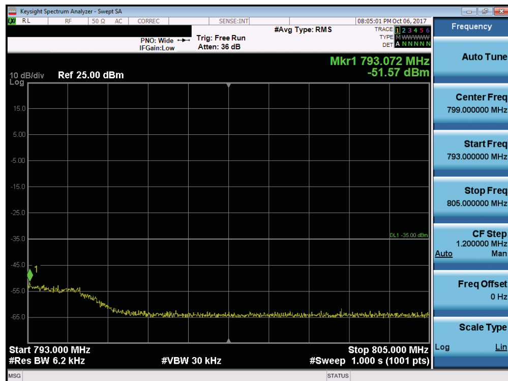
Plot 7-164. Upper Emission Mask (Band 13 - 5.0MHz QPSK - Full RB Configuration)
