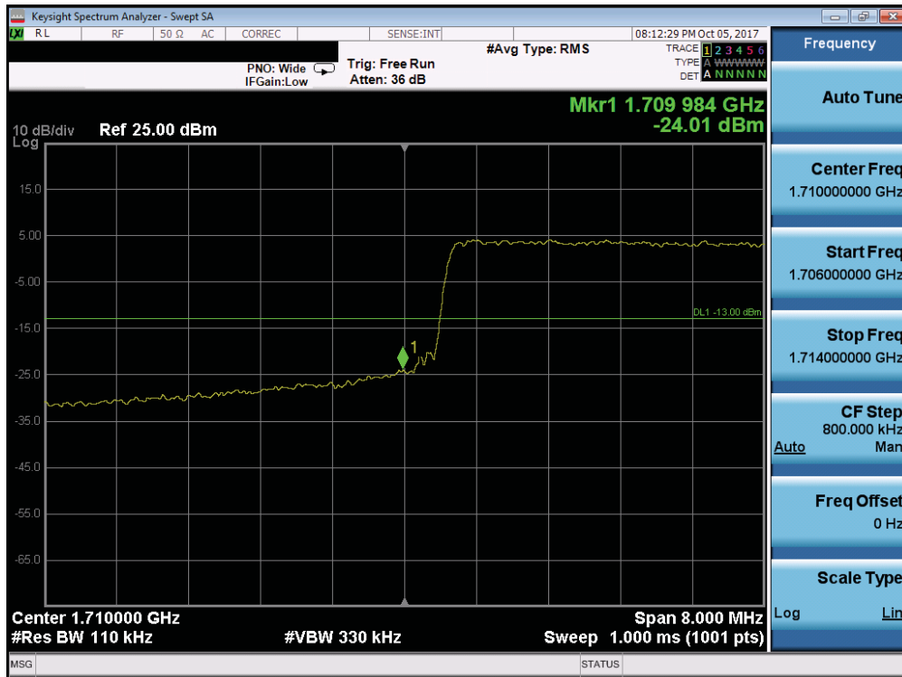
Plot 7-197. Lower Band Edge Plot (Band 66/4 - 10.0MHz QPSK - Full RB Configuration)
