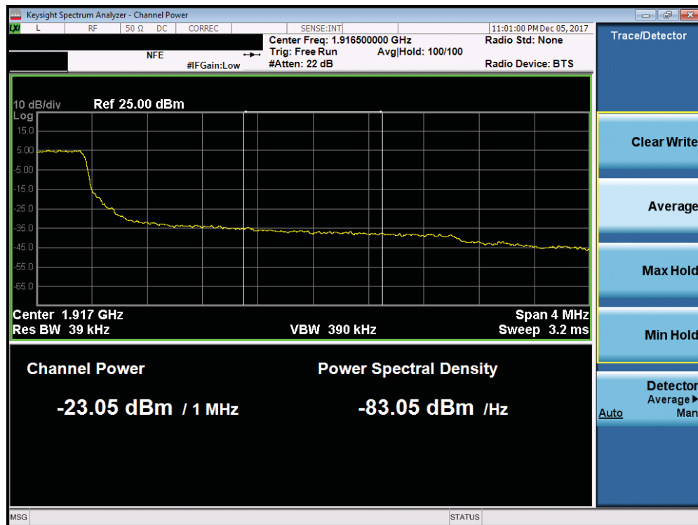
Plot 7-226. Upper Extended Band Edge Plot (Band 25 - 3.0MHz QPSK - Full RB Configuration)
