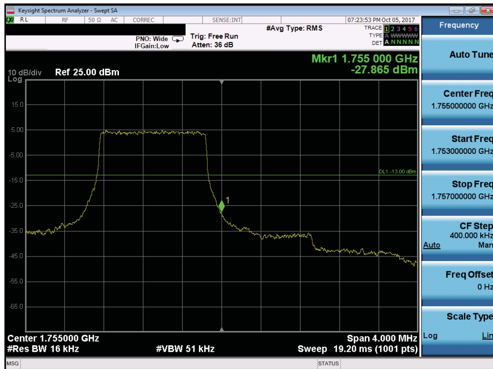
Plot 7-181. Upper Band Edge Plot (Band 4 - 1.4MHz QPSK - Full RB Configuration)
