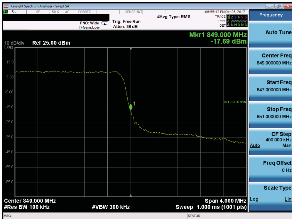
Plot 7-172. Upper Band Edge Plot (Band 5/26 – 3MHz QPSK - Full RB Configuration)
