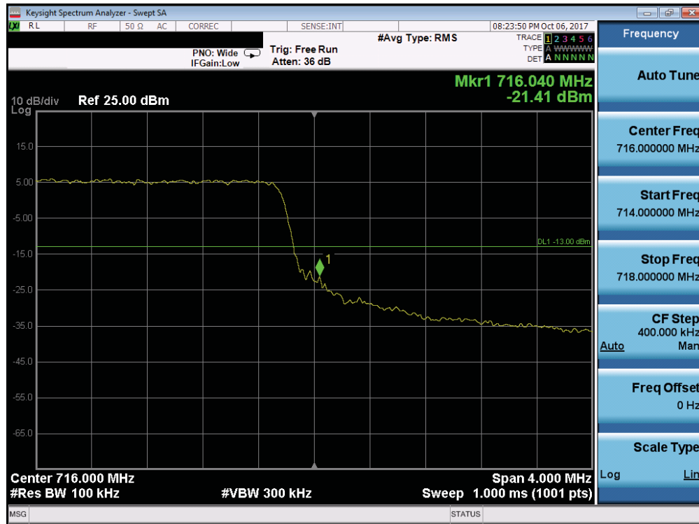
Plot 7-157. Upper Band Edge Plot (Band 12/17 - 5.0MHz QPSK - Full RB Configuration)
