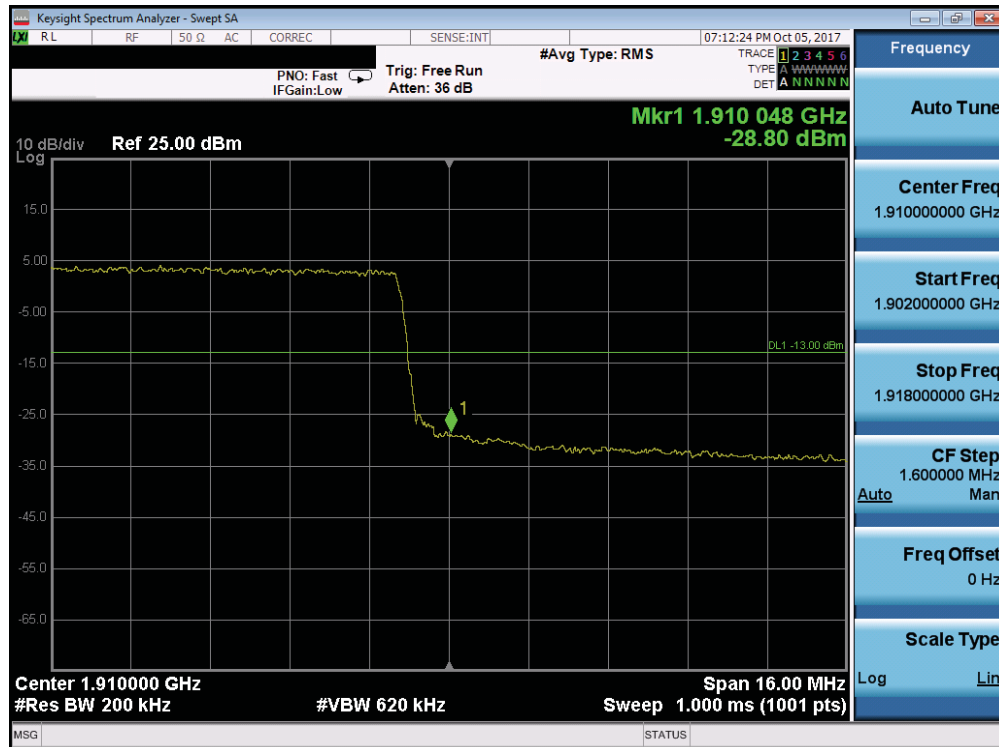
Plot 7-247. Upper Band Edge Plot (Band 2 - 20.0MHz QPSK - Full RB Configuration)
