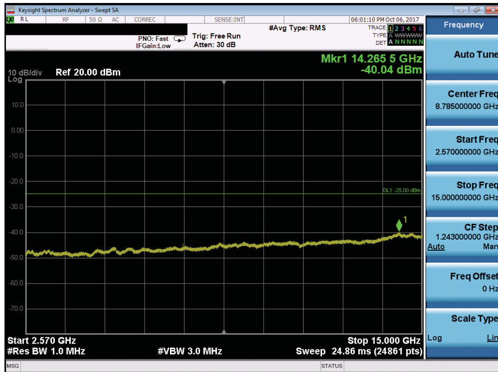
Plot 7-134. Conducted Spurious Plot (Band 7 - 5.0MHz QPSK - RB Size 1, RB Offset 0 - Low Channel)
