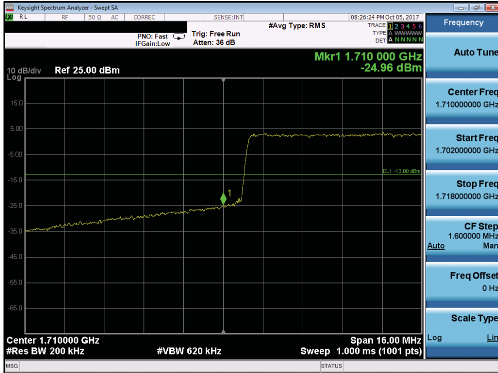
Plot 7-209. Lower Band Edge Plot (Band 66/4 - 20.0MHz QPSK - Full RB Configuration)
