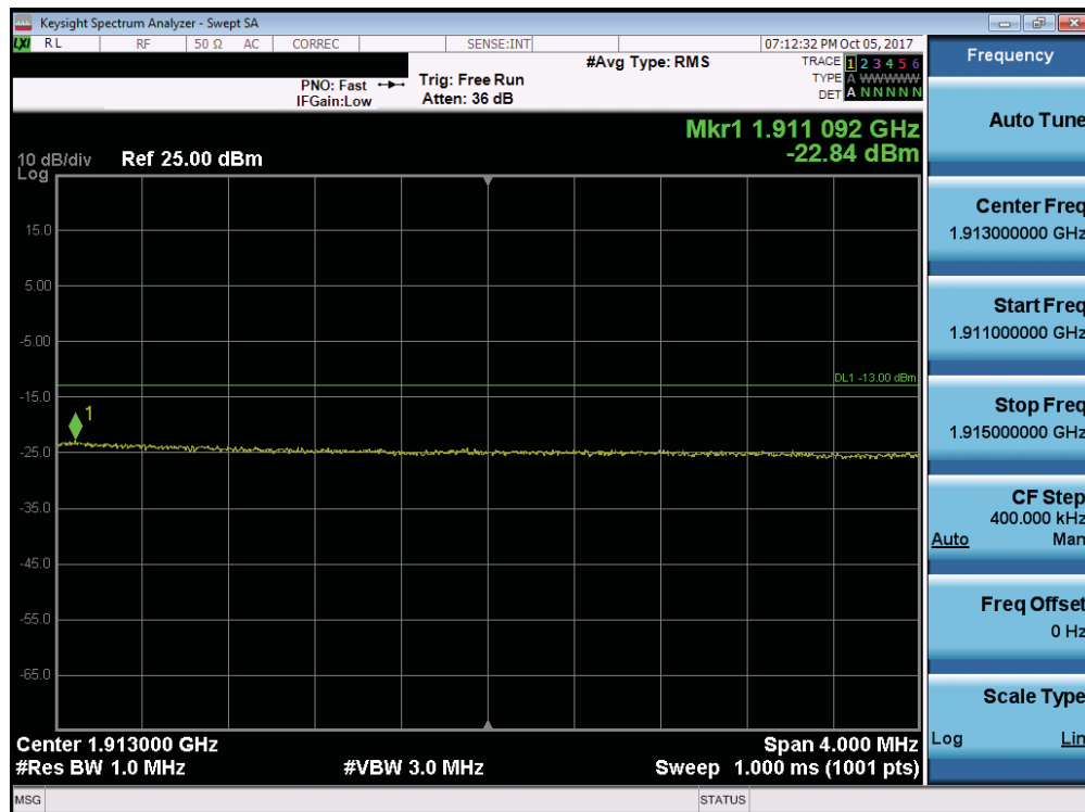
Plot 7-248. Upper Extended Band Edge Plot (Band 2 - 20.0MHz QPSK - Full RB Configuration)
