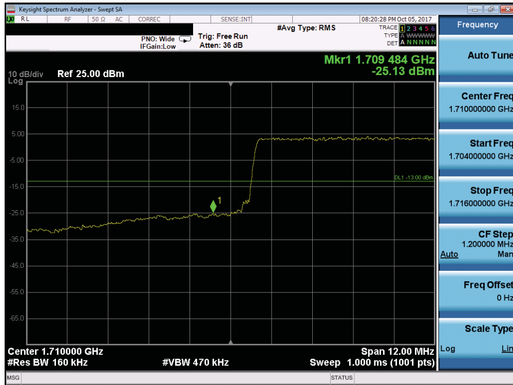
Plot 7-203. Lower Band Edge Plot (Band 66/4 - 15.0MHz QPSK - Full RB Configuration)
