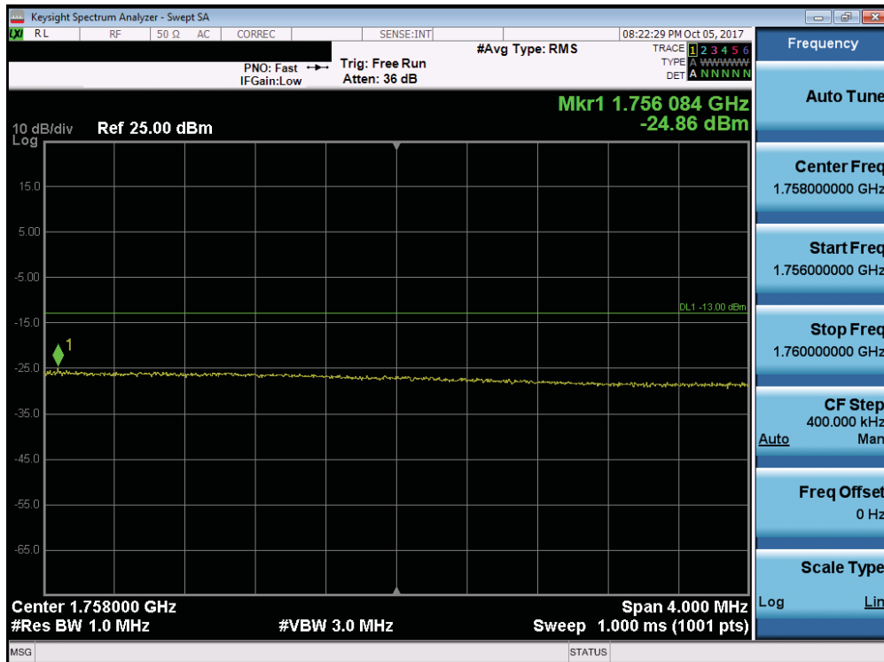
Plot 7-206. Upper Extended Band Edge Plot (Band 4 - 15.0MHz QPSK - Full RB Configuration)
