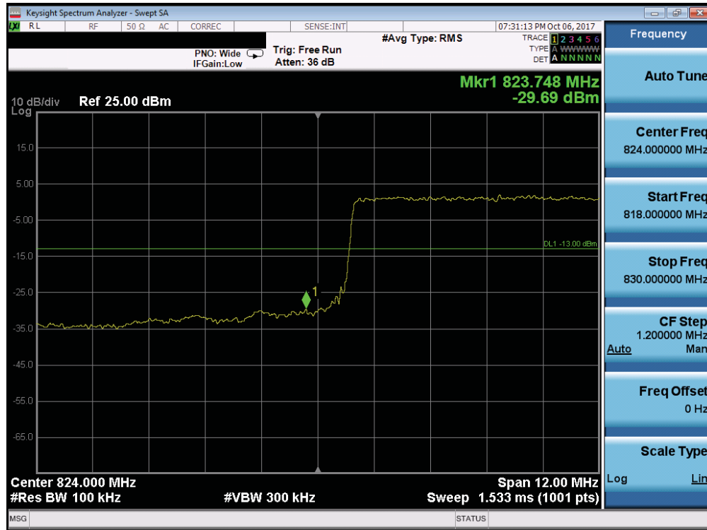
Plot 7-177. Lower Band Edge Plot (Band 26 - 15.0MHz QPSK - Full RB Configuration)
