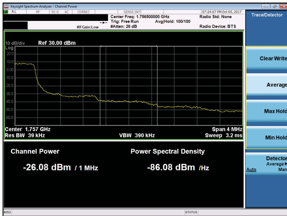
Plot 7-182. Upper Extended Band Edge Plot (Band 4 - 1.4MHz QPSK - Full RB Configuration)
