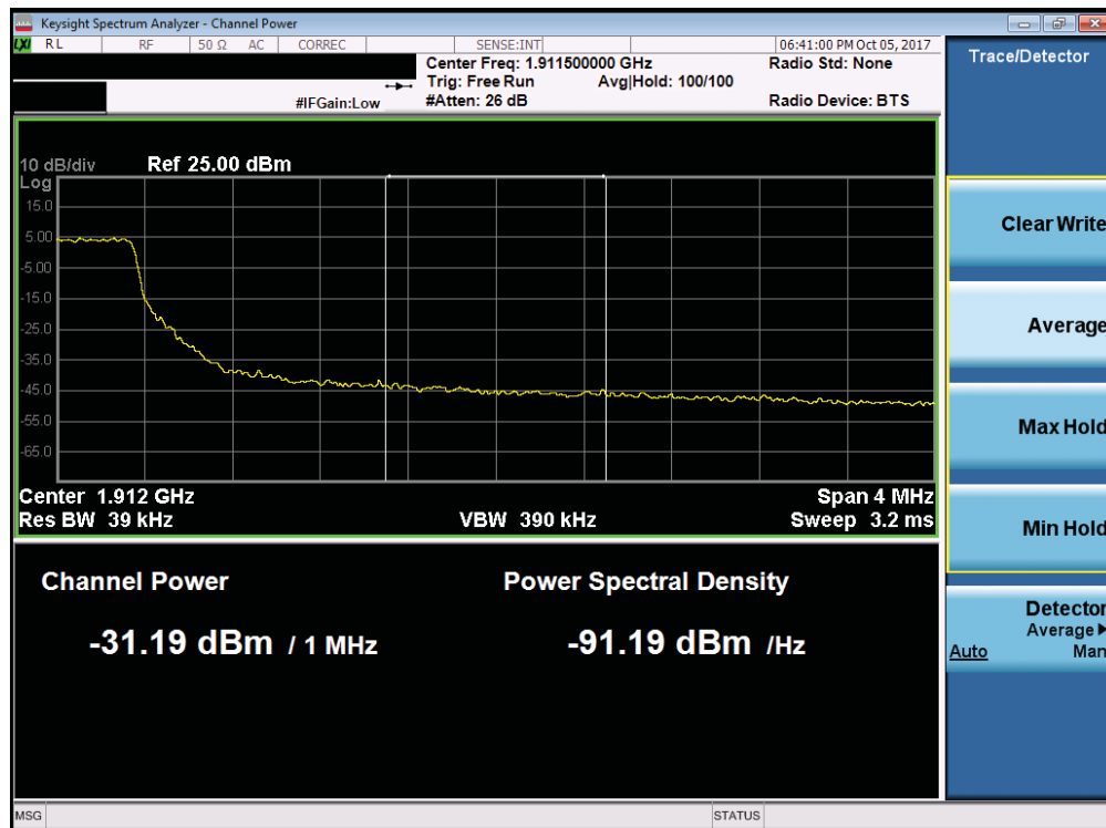
Plot 7-224. Upper Extended Band Edge Plot (Band 2 - 3.0MHz QPSK - Full RB Configuration)
