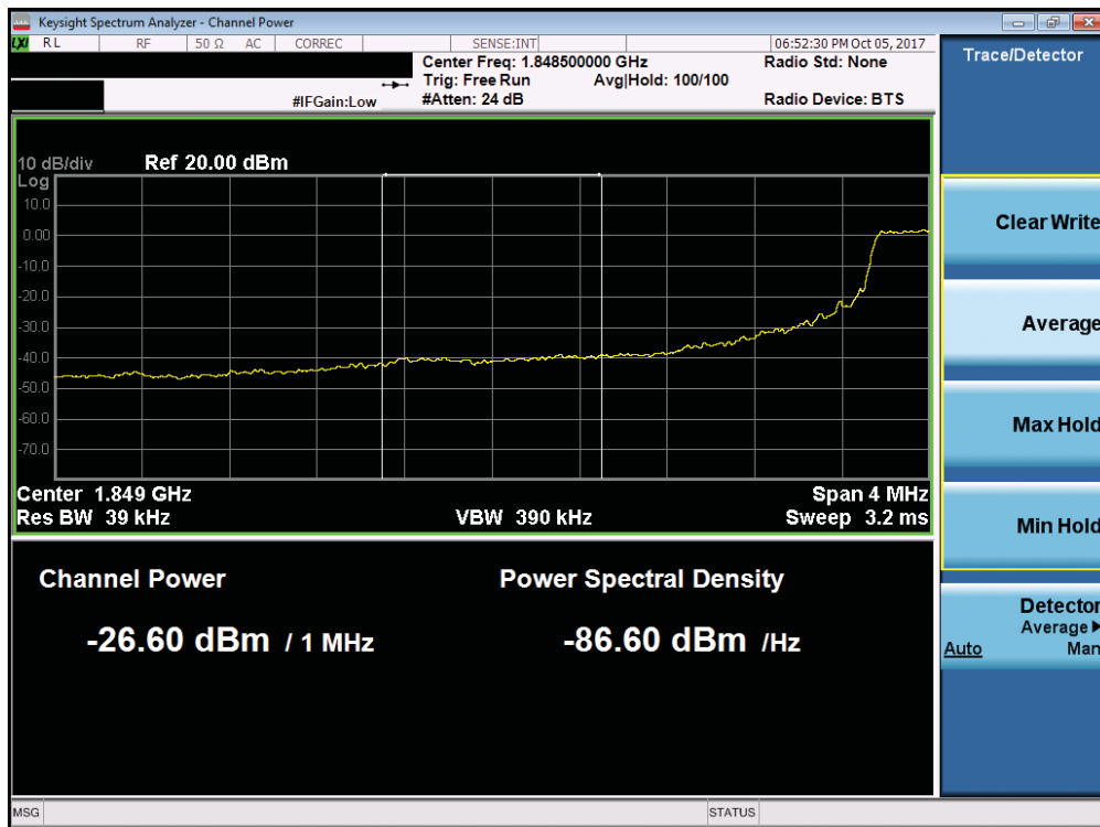
Plot 7-228. Lower Extended Band Edge Plot (Band 25/2 - 5.0MHz QPSK - Full RB Configuration)
