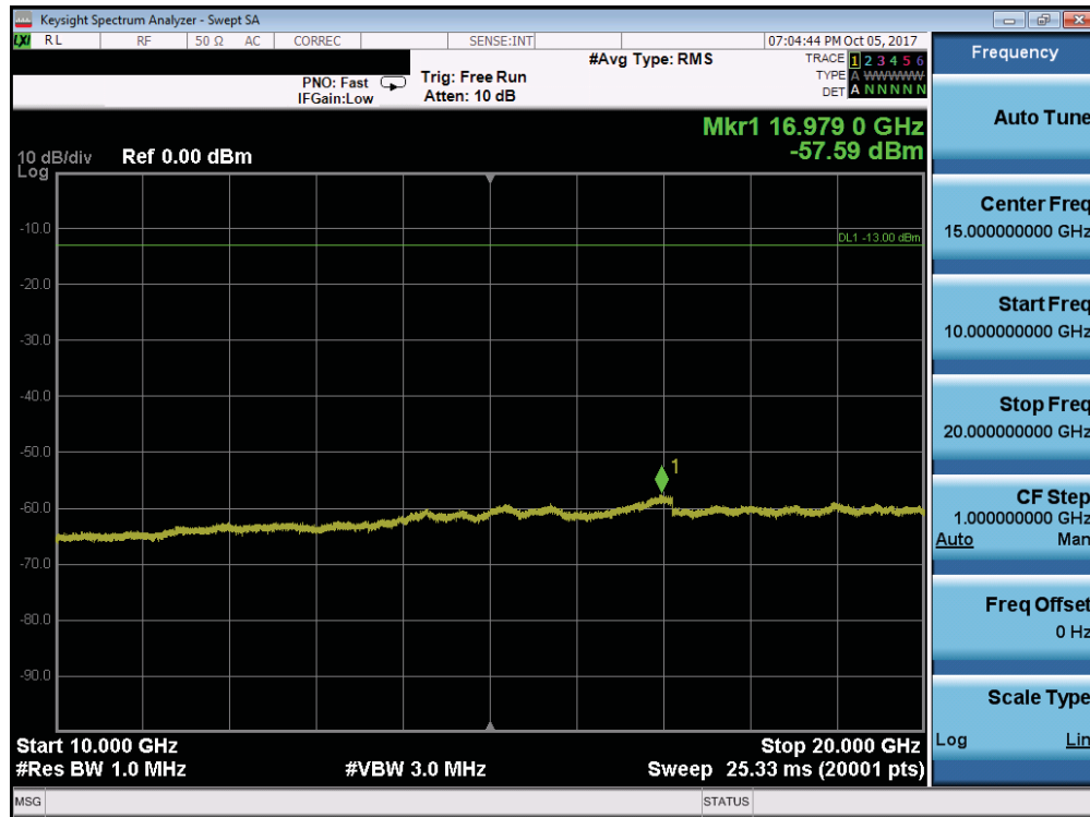
Plot 7-132. Conducted Spurious Plot (Band 25/2 - 15.0MHz QPSK - RB Size 1, RB Offset 0 - High Channel)
