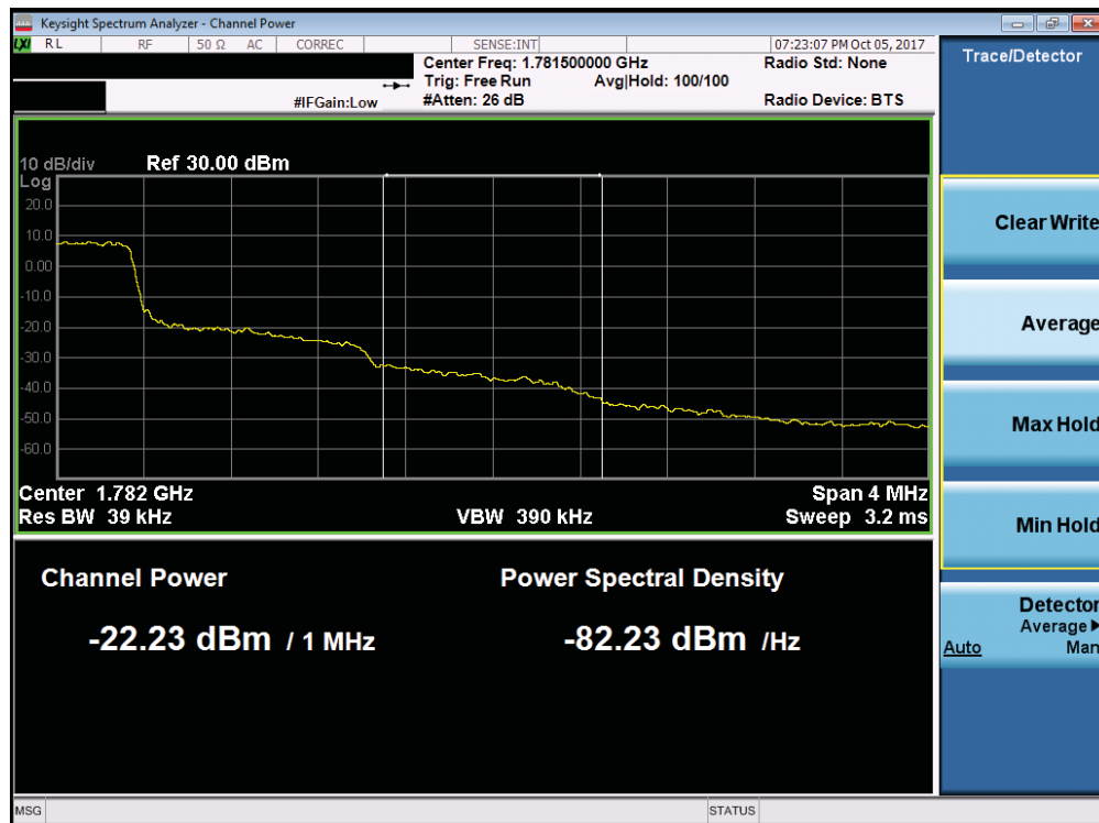
Plot 7-184. Upper Extended Band Edge Plot (Band 66 - 1.4MHz QPSK - Full RB Configuration)
