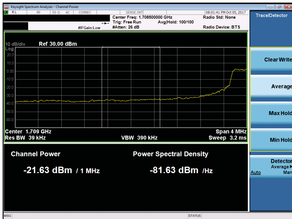
Plot 7-192. Lower Extended Band Edge Plot (Band 66/4 - 5.0MHz QPSK - Full RB Configuration)
