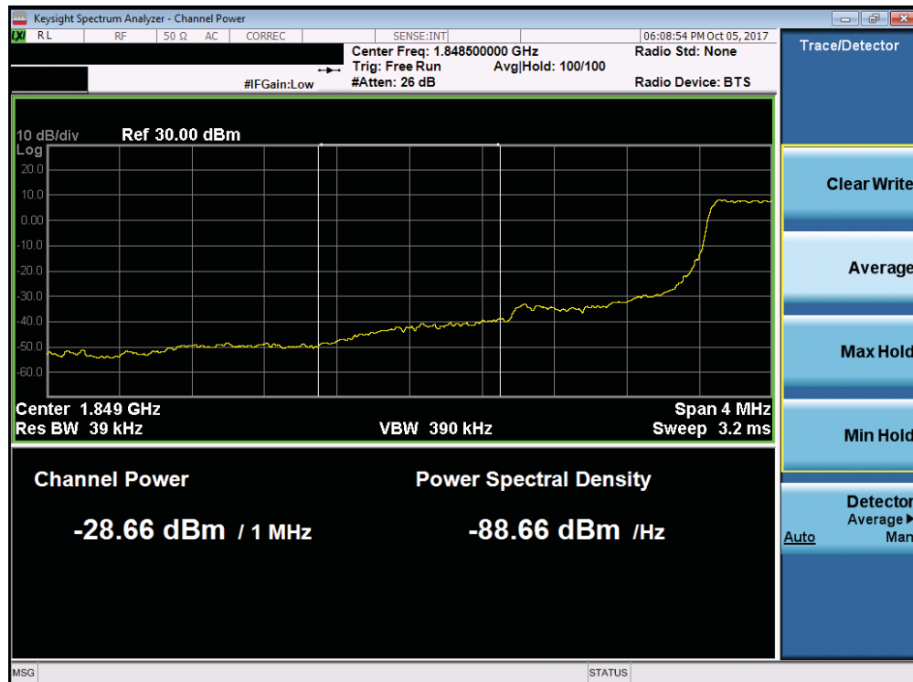
Plot 7-216. Lower Extended Band Edge Plot (Band 25/2 - 1.4MHz QPSK - Full RB Configuration)
