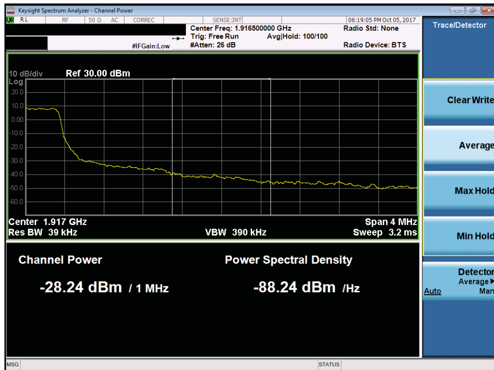
Plot 7-220. Upper Extended Band Edge Plot (Band 25 - 1.4MHz QPSK - Full RB Configuration)
