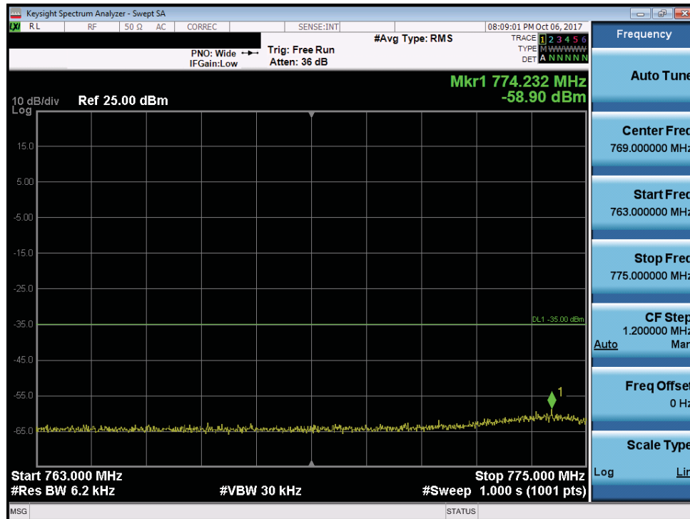
Plot 7-166. Lower Emission Mask (Band 13 - 10.0MHz QPSK - Full RB Configuration)
