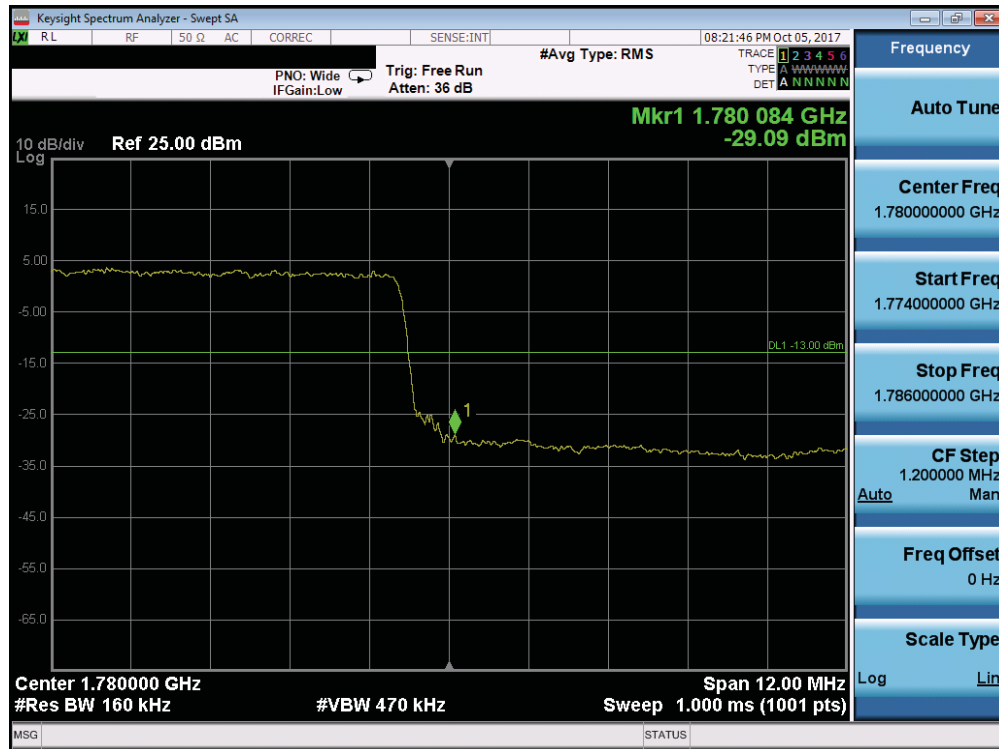
Plot 7-207. Upper Band Edge Plot (Band 66 - 15.0MHz QPSK - Full RB Configuration)
