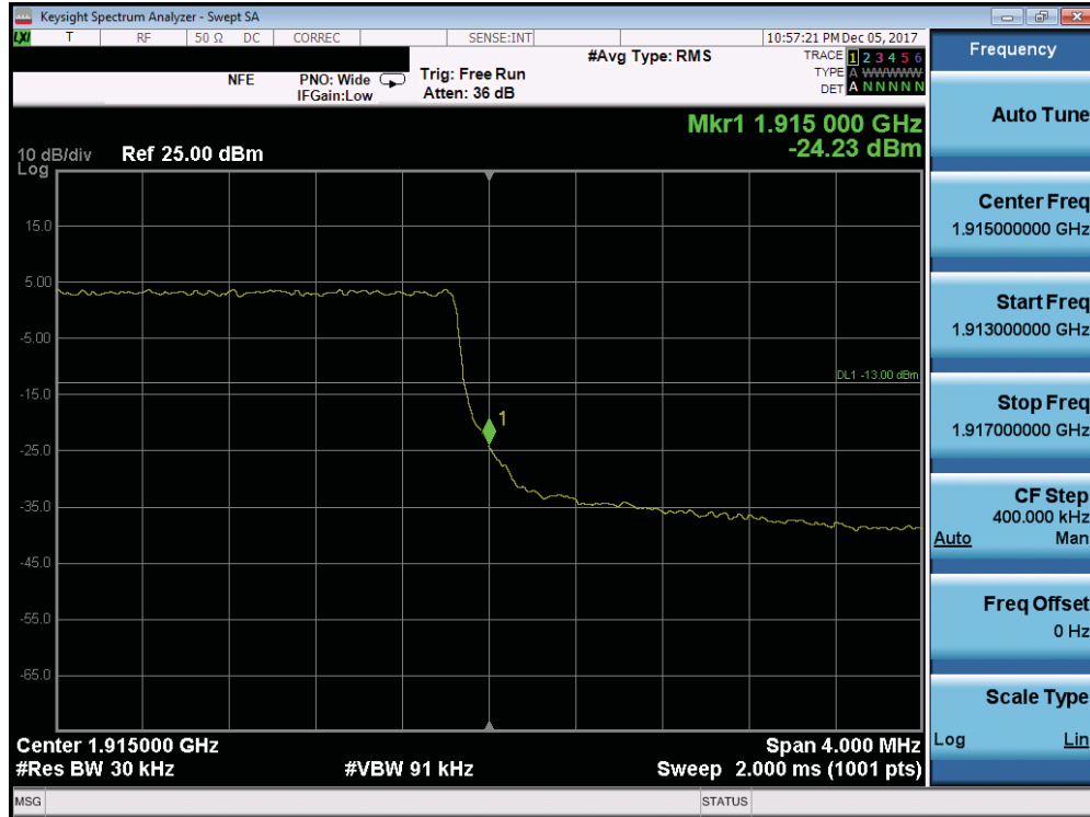
Plot 7-225. Upper Band Edge Plot (Band 25 - 3.0MHz QPSK - Full RB Configuration)
