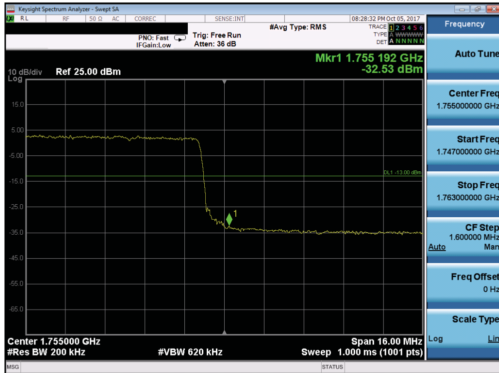
Plot 7-211. Upper Band Edge Plot (Band 4 - 20.0MHz QPSK - Full RB Configuration)
