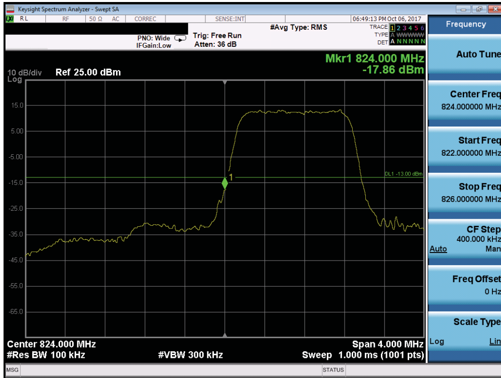
Plot 7-169. Lower Band Edge Plot (Band 5/26 – 1.4MHz QPSK - Full RB Configuration)
