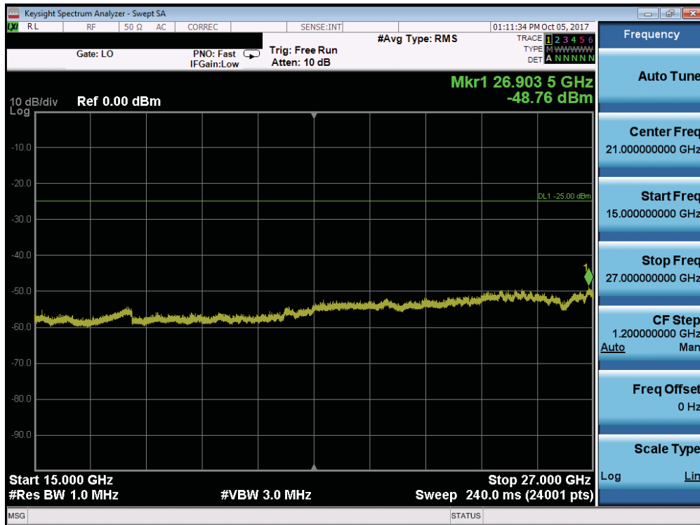
Plot 7-144. Conducted Spurious Plot (Band 38/41 - 10.0MHz QPSK - RB Size 1, RB Offset 0 - Low Channel)
