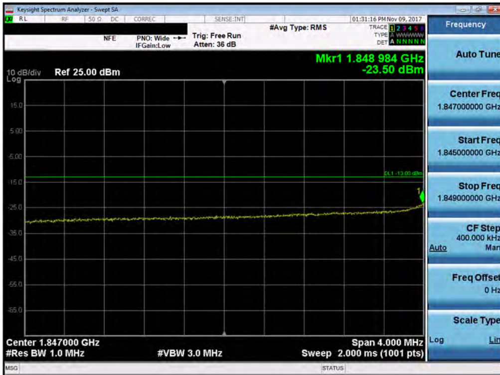
Plot 7-320. Lower Extended Band Edge Plot (Band 2/25 - 10.0MHz QPSK - Full RB Configuration)
