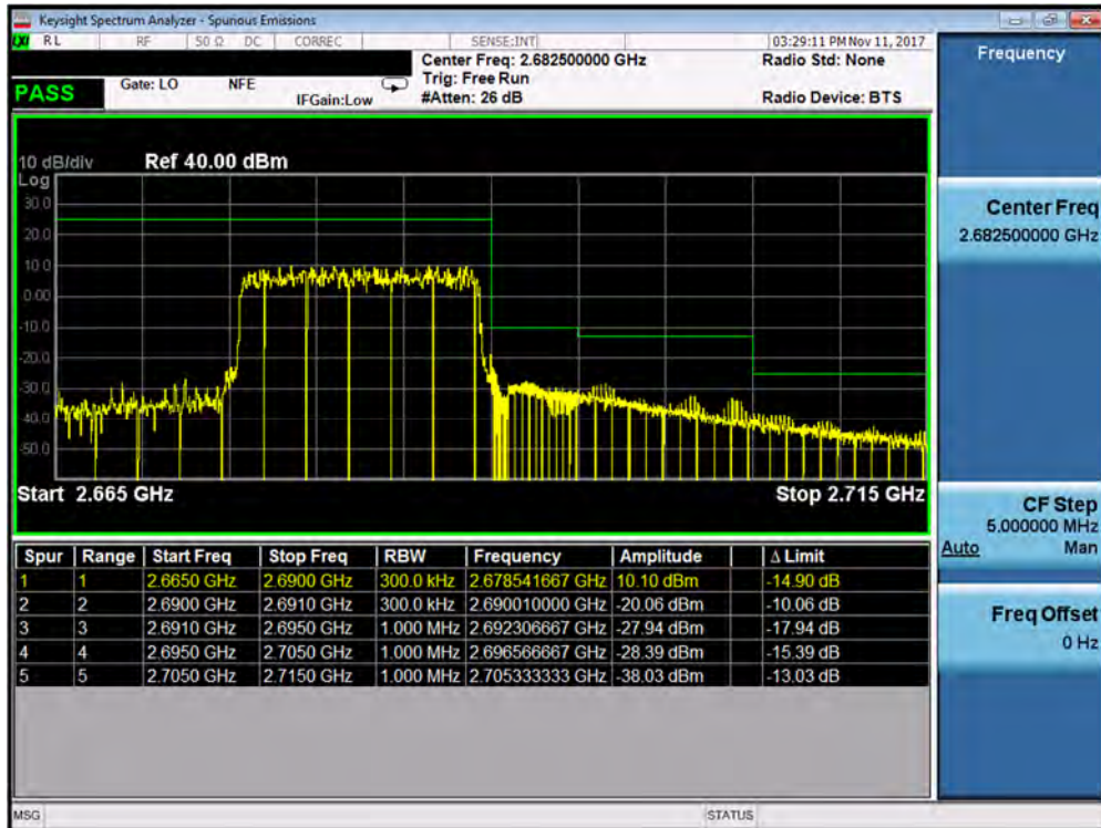
Plot 7-376. Upper ACP Plot (Band 41 – 15.0MHz QPSK – RB Size 75)
