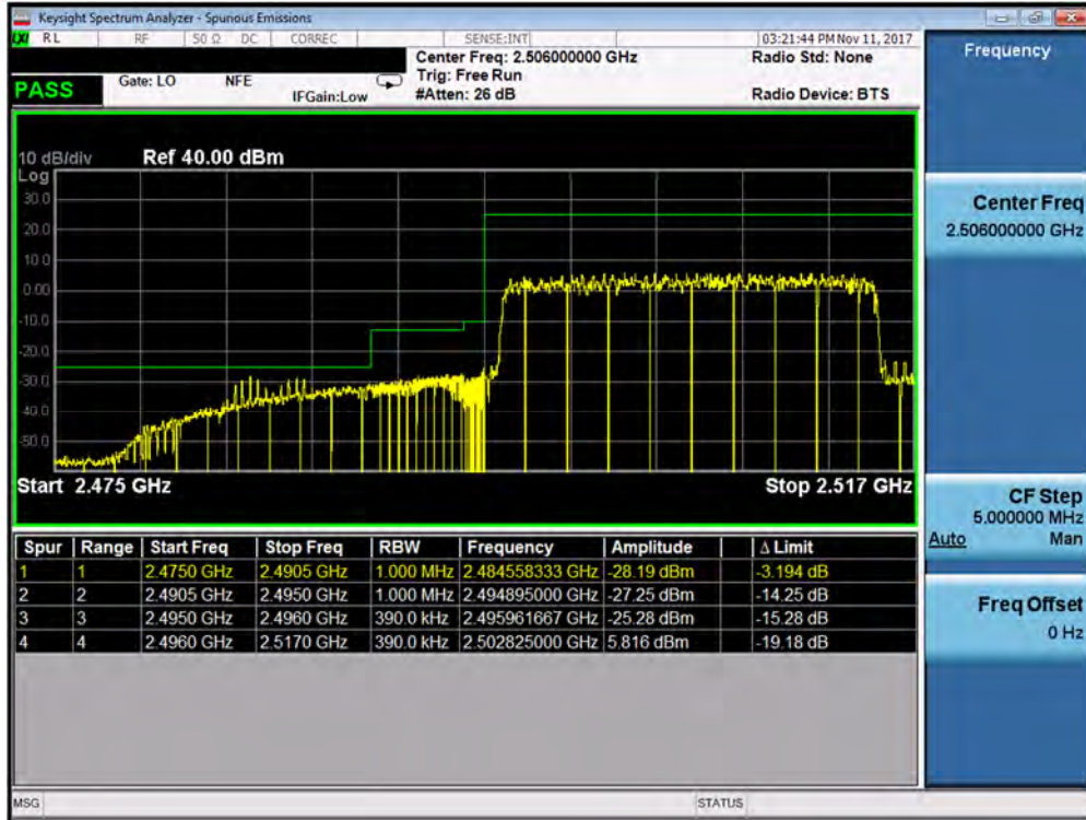
Plot 7-377. Lower ACP Plot (Band 41 – 20.0MHz QPSK – RB Size 100)
