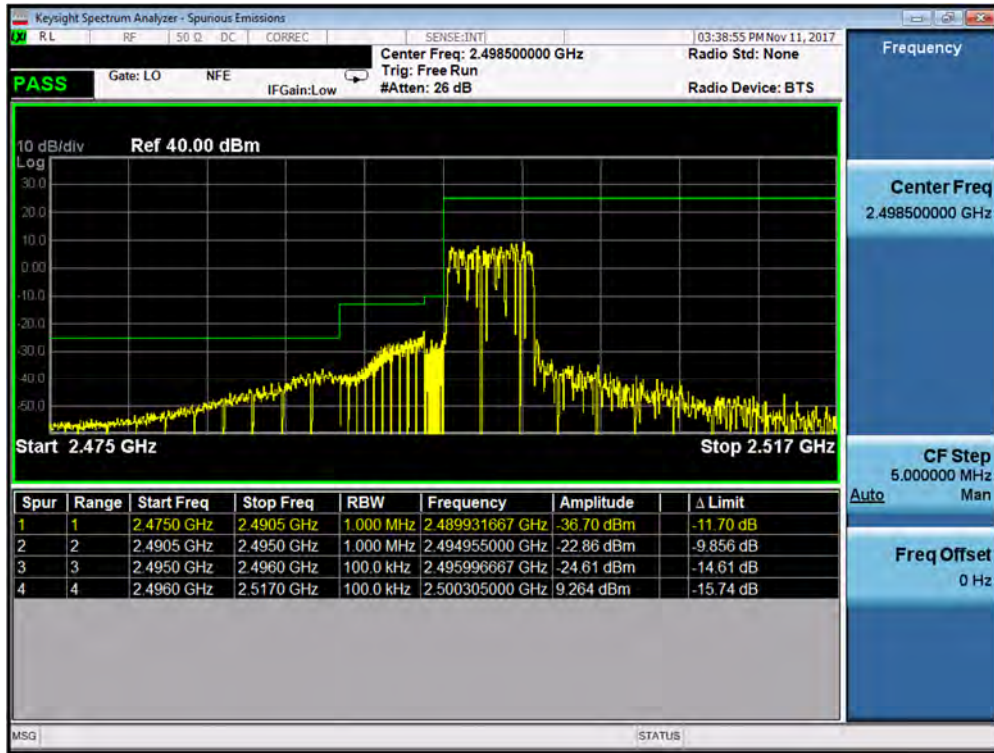
Plot 7-371. Lower ACP Plot (Band 41 – 5.0MHz QPSK – RB Size 25)
