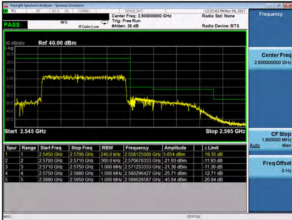
Plot 7-362. Upper ACP Plot (Band 7 – 20.0MHz QPSK – RB Size 100– Antenna B)
