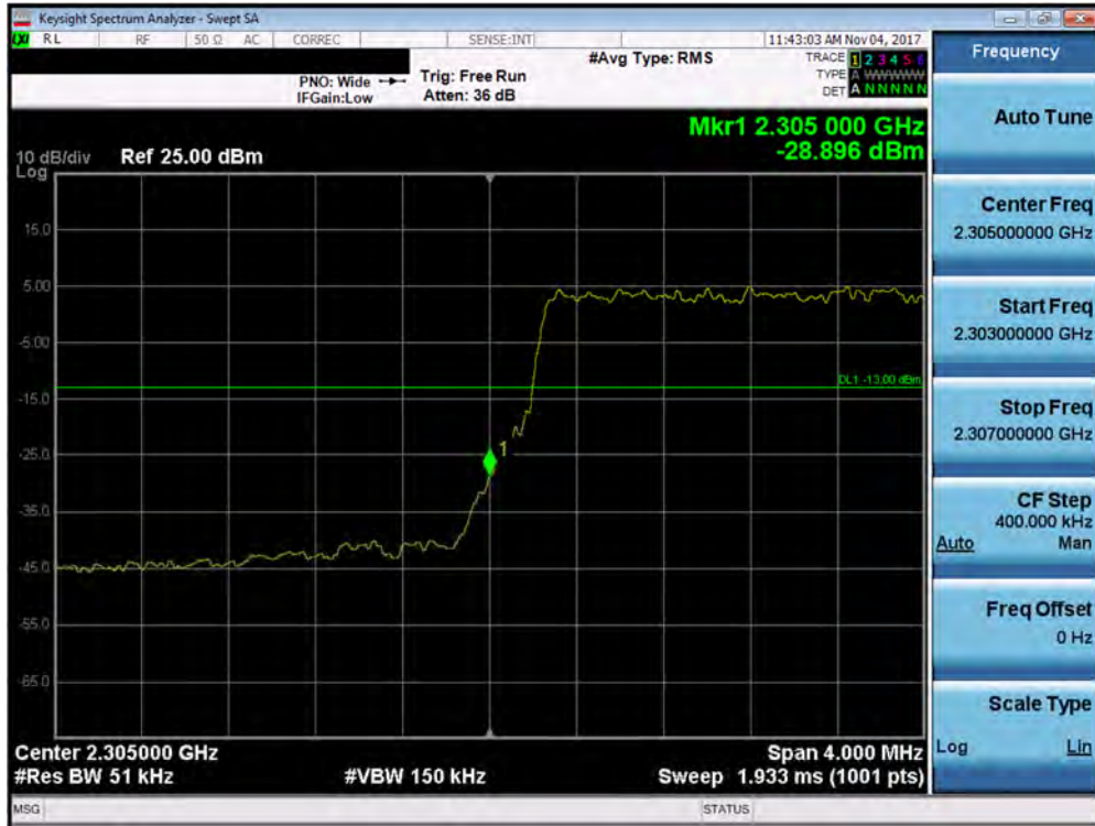
Plot 7-337. Lower Band Edge Plot (Band 30 - 5.0MHz QPSK - Full RB Configuration- Antenna B)
