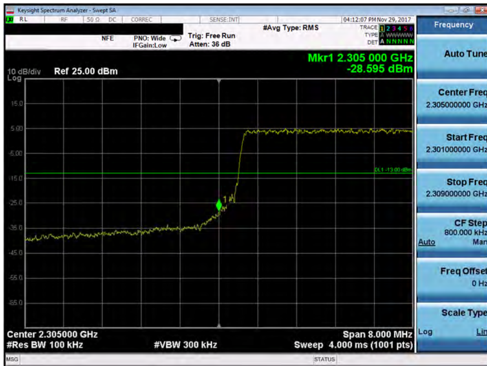
Plot 7-351. Lower Band Edge Plot (Band 30 - 10.0MHz QPSK - Full RB Configuration- Antenna A)
