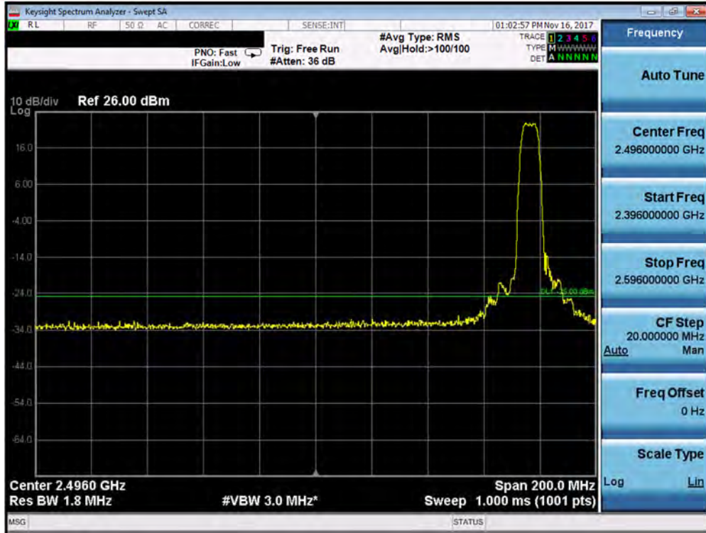
Plot 7-379. Lower ACP Plot (Band 38 – 5.0MHz QPSK – RB Size 25)
