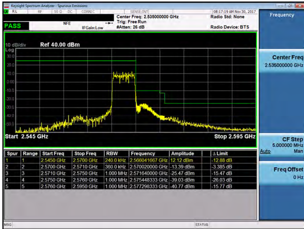
Plot 7-364. Upper ACP Plot (Band 7 – 5.0MHz QPSK – RB Size 25– Antenna A)
