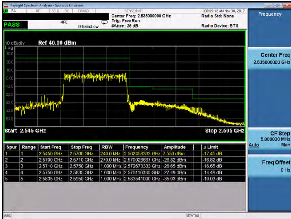
Plot 7-368. Upper ACP Plot (Band 7 – 15.0MHz QPSK – RB Size 75– Antenna A)
