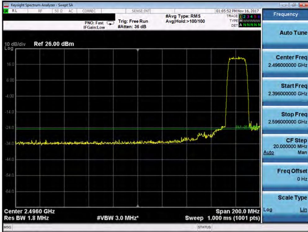
Plot 7-383. Lower ACP Plot (Band 38 – 15.0MHz QPSK – RB Size 75)
