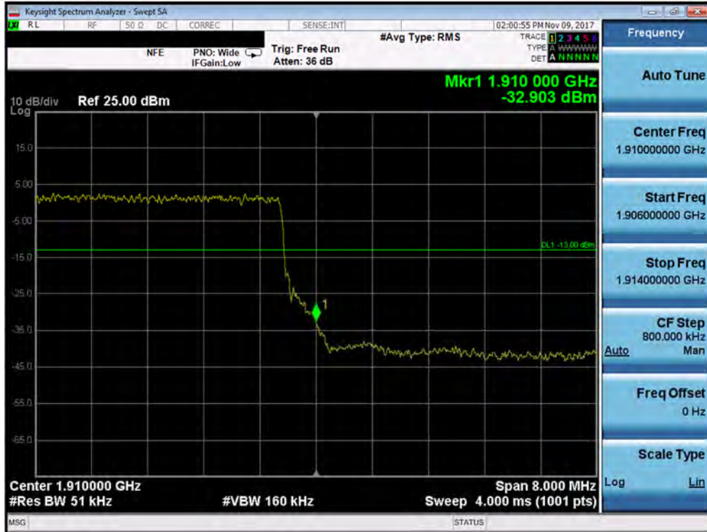
Plot 7-321. Upper Band Edge Plot (Band 2 - 10.0MHz QPSK - Full RB Configuration)
