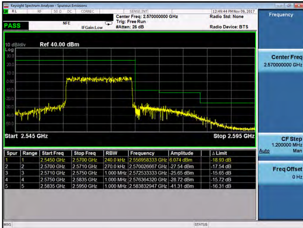
Plot 7-360. Upper ACP Plot (Band 7 – 15.0MHz QPSK – RB Size 75– Antenna B)
