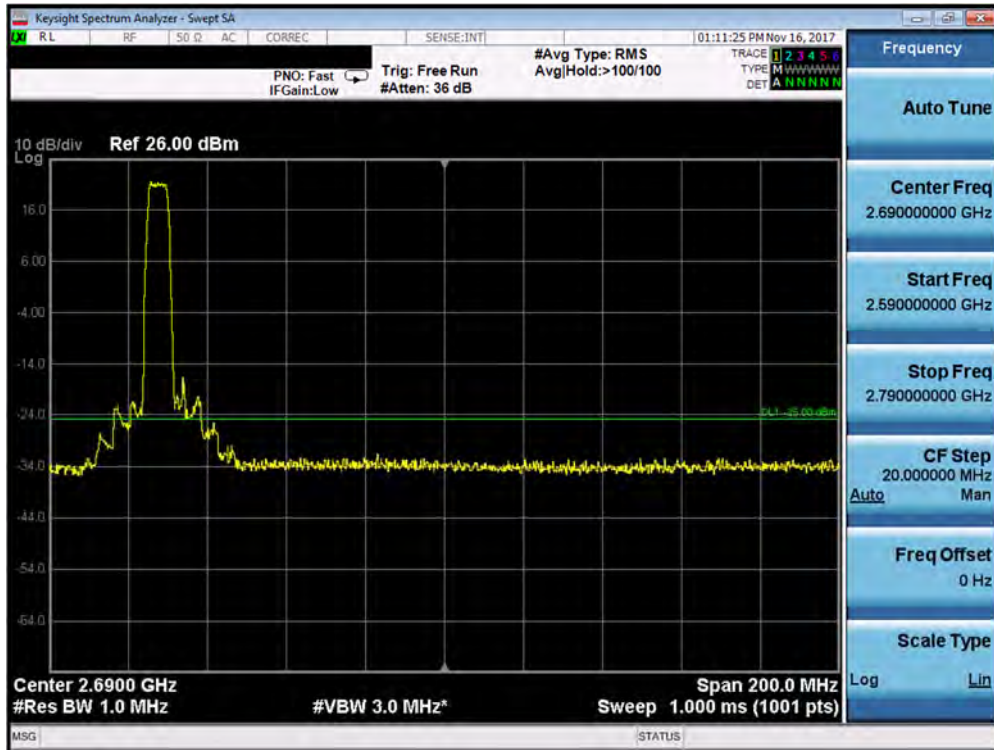
Plot 7-380. Upper ACP Plot (Band 38 – 5.0MHz QPSK – RB Size 25)
