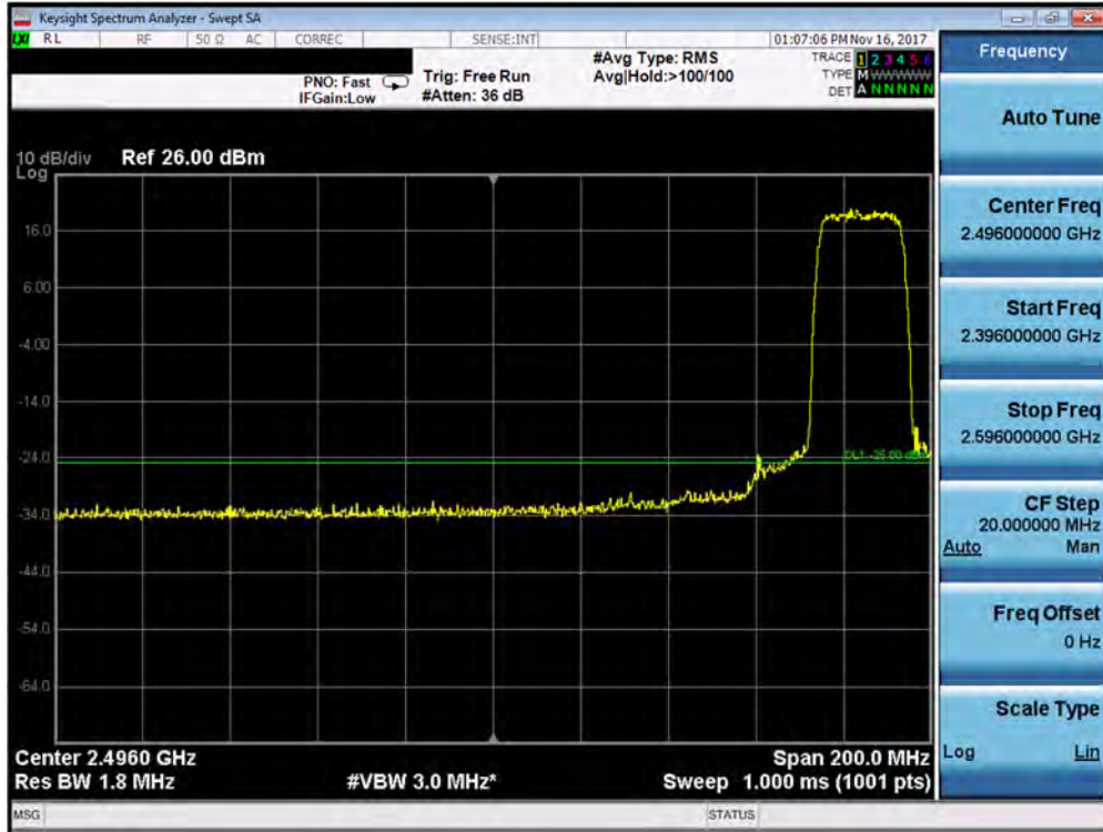
Plot 7-385. Lower ACP Plot (Band 38 – 20.0MHz QPSK – RB Size 100)
