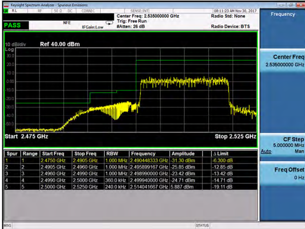
Plot 7-369. Lower ACP Plot (Band 7 – 20.0MHz QPSK – RB Size 100– Antenna A)
