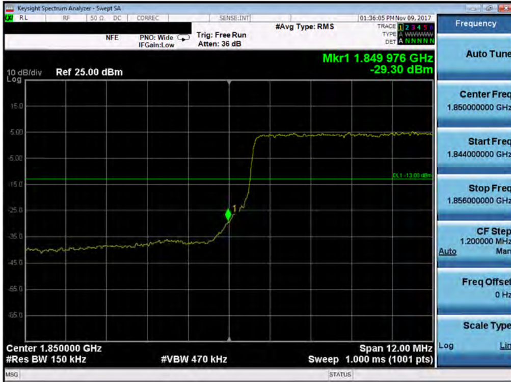
Plot 7-325. Lower Band Edge Plot (Band 2/25 - 15.0MHz QPSK - Full RB Configuration)
