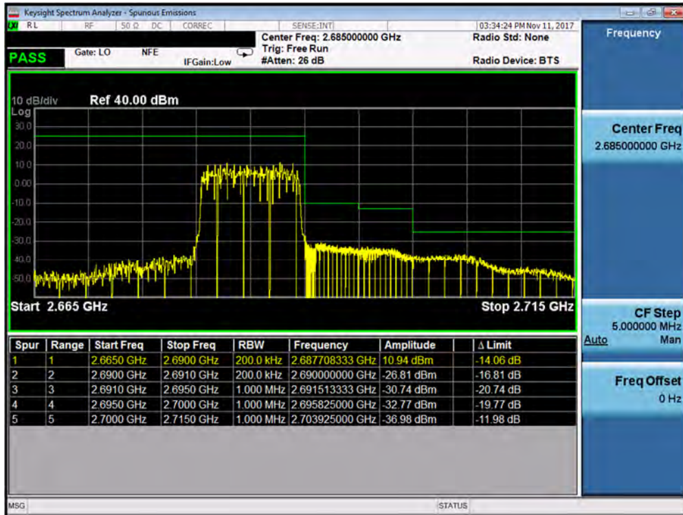
Plot 7-374. Upper ACP Plot (Band 41 – 10.0MHz QPSK – RB Size 50)
