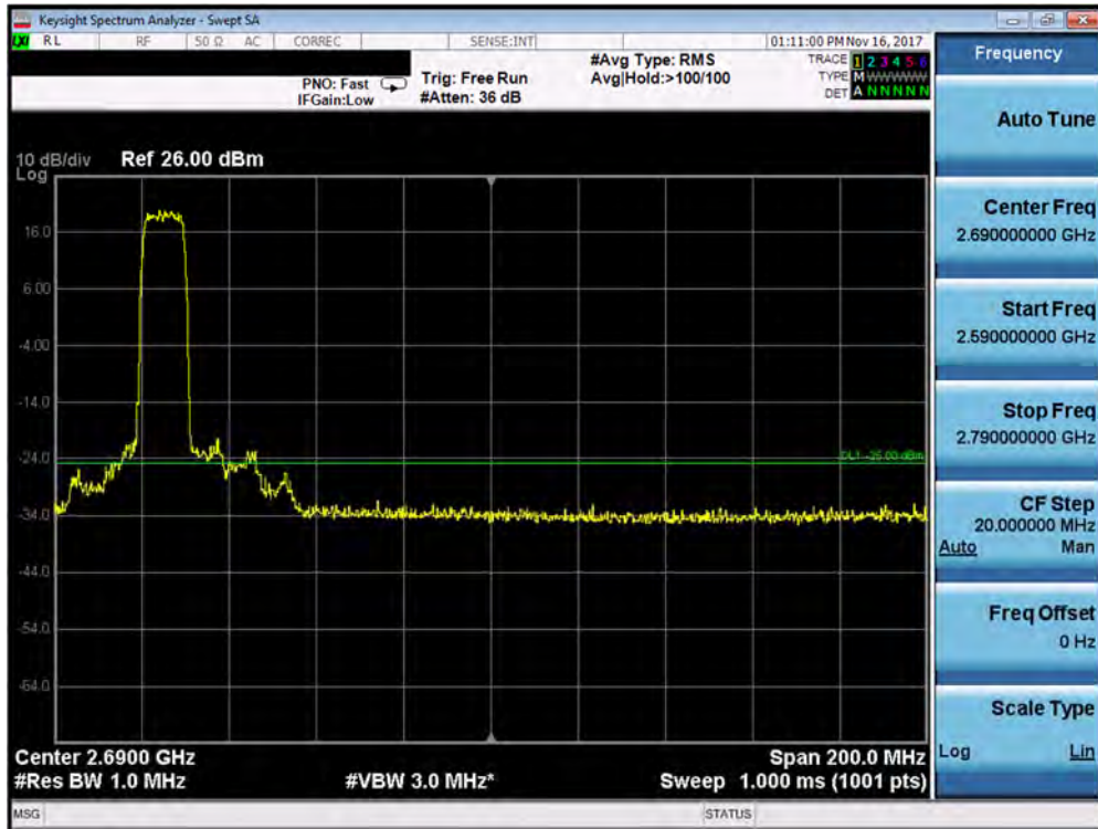
Plot 7-382. Upper ACP Plot (Band 38 – 10.0MHz QPSK – RB Size 50)
