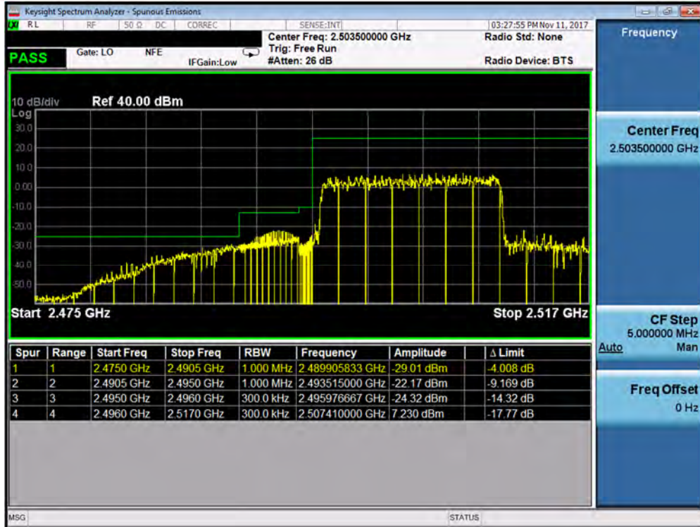
Plot 7-375. Lower ACP Plot (Band 41 – 15.0MHz QPSK – RB Size 75)
