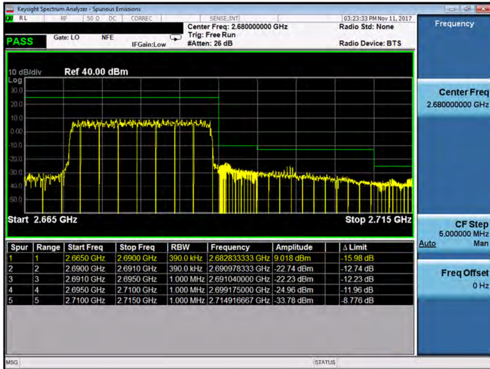
Plot 7-378. Upper ACP Plot (Band 41 – 20.0MHz QPSK – RB Size 100)
