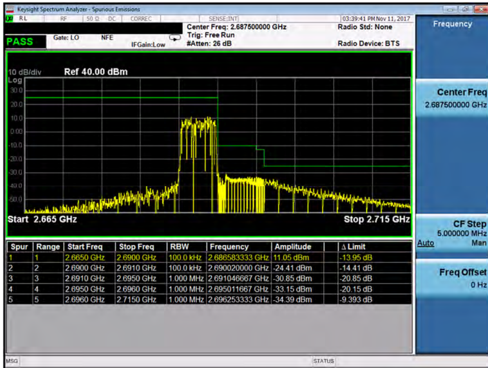
Plot 7-372. Upper ACP Plot (Band 41 – 5.0MHz QPSK – RB Size 25)
