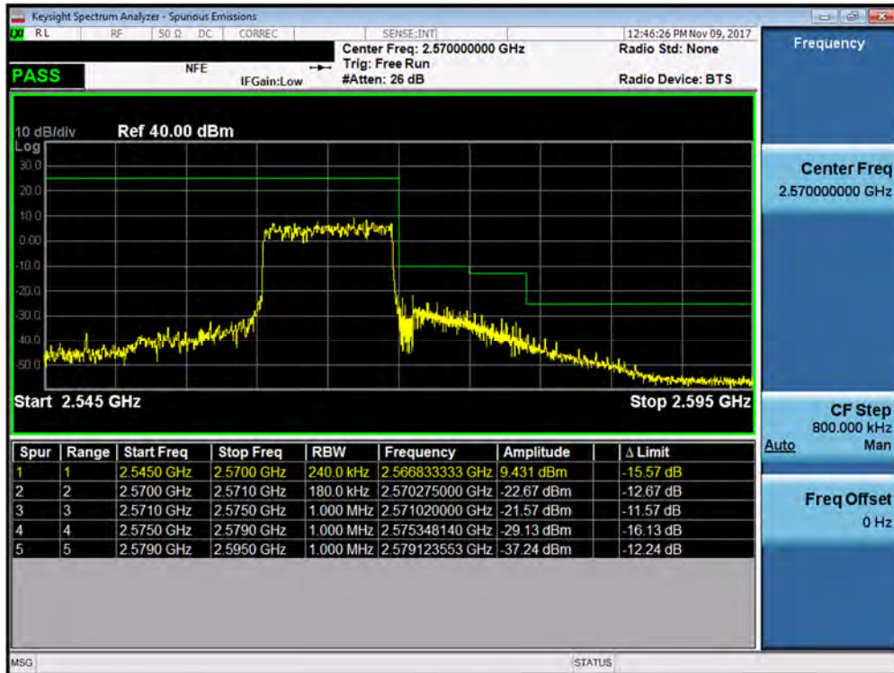
Plot 7-358. Upper ACP Plot (Band 7 – 10.0MHz QPSK – RB Size 50– Antenna B)
