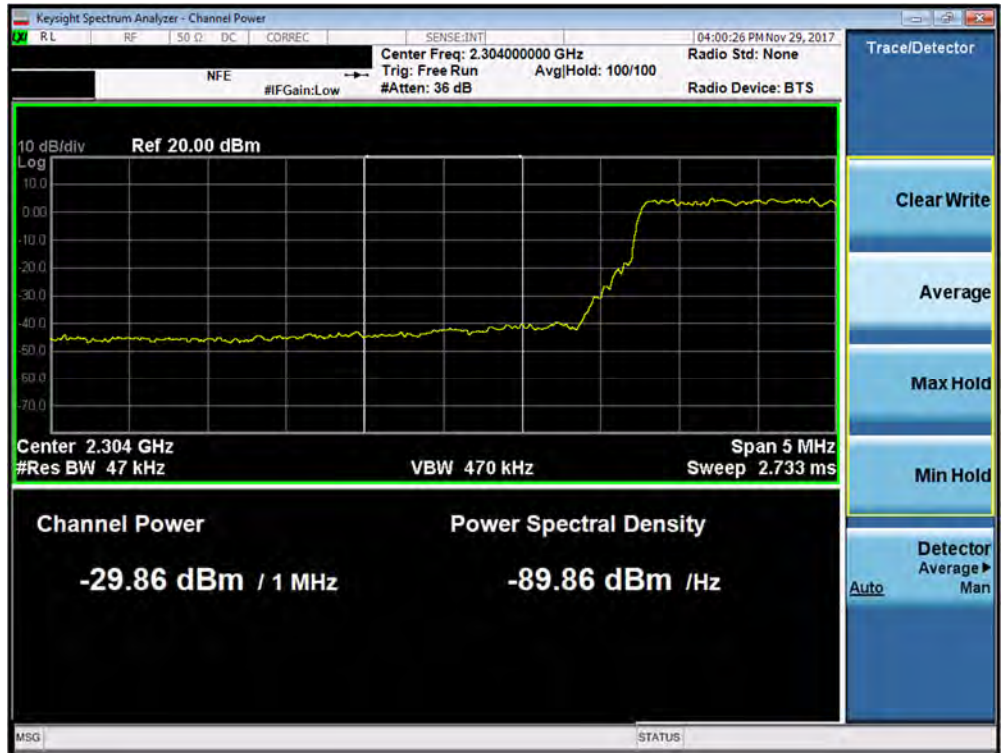
Plot 7-348. Lower Extended Band Edge Plot (Band 30 - 5.0MHz QPSK - Full RB Configuration- Antenna A)
