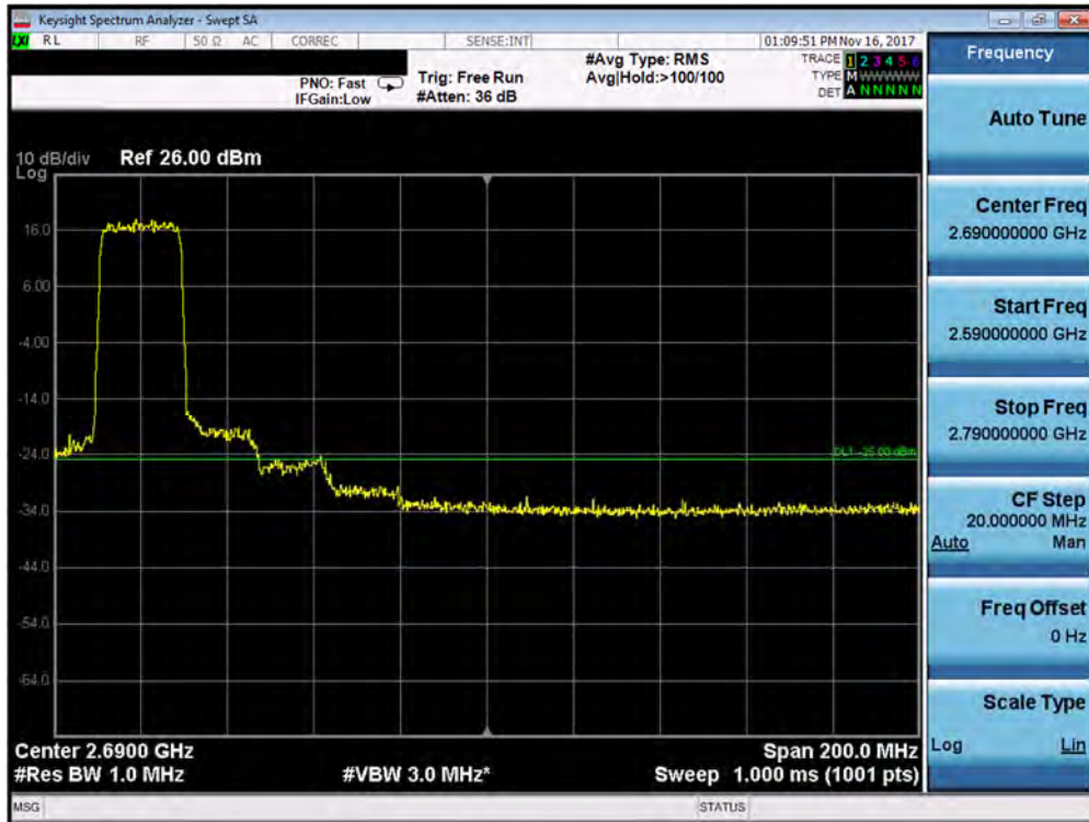
Plot 7-386. Upper ACP Plot (Band 38 – 20.0MHz QPSK – RB Size 100)
