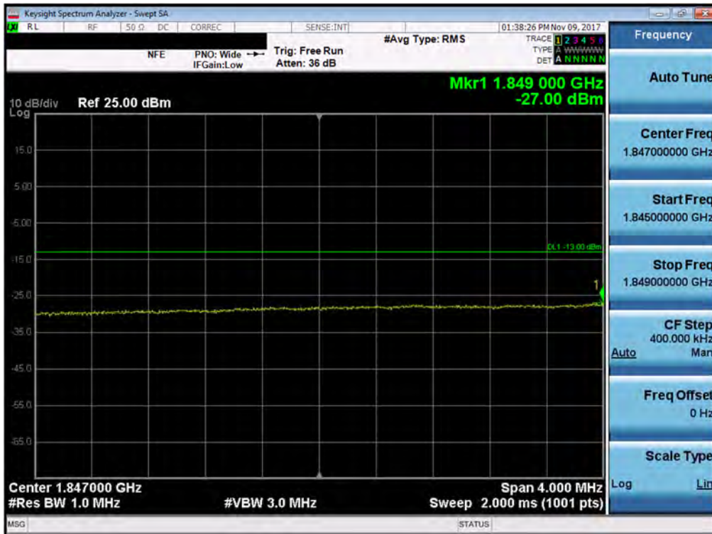
Plot 7-332. Lower Extended Band Edge Plot (Band 2/25 - 20.0MHz QPSK - Full RB Configuration)
