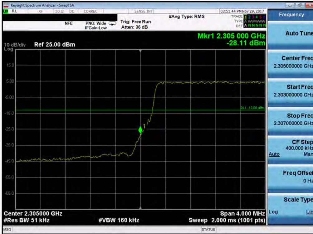
Plot 7-346. Lower Band Edge Plot (Band 30 - 5.0MHz QPSK - Full RB Configuration- Antenna A)
