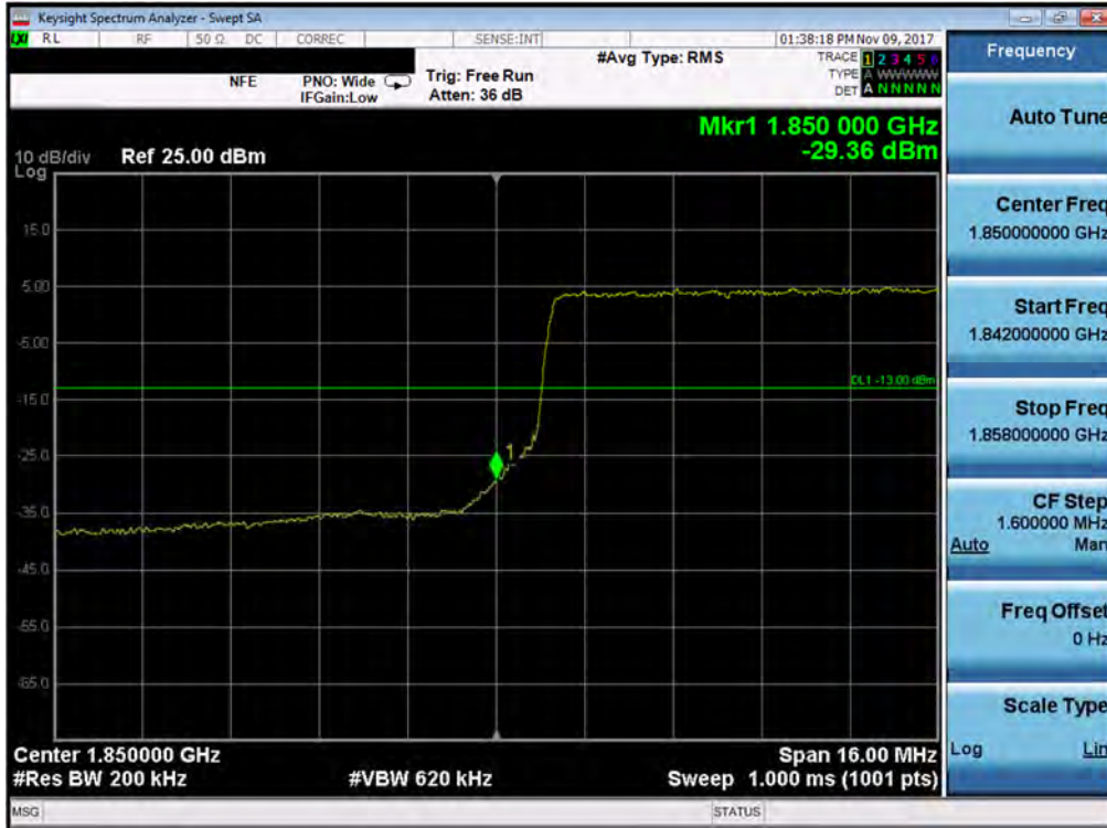
Plot 7-331. Lower Band Edge Plot (Band 2/25 - 20.0MHz QPSK - Full RB Configuration)
