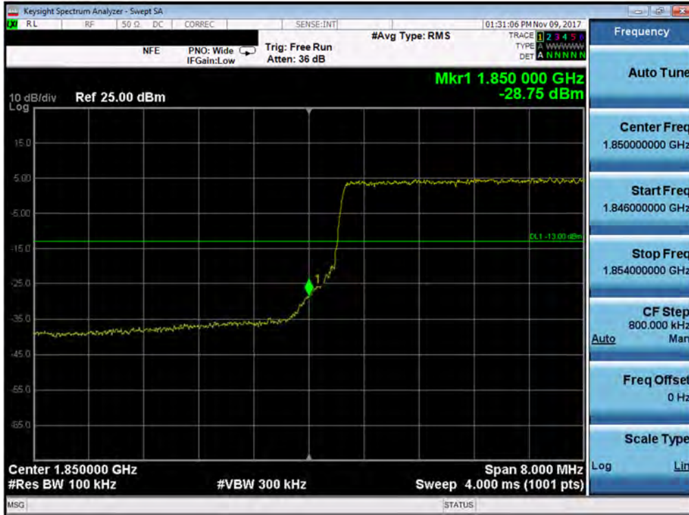
Plot 7-319. Lower Band Edge Plot (Band 2/25 - 10.0MHz QPSK - Full RB Configuration)
