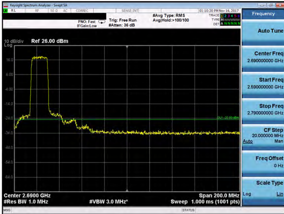
Plot 7-384. Upper ACP Plot (Band 38 – 15.0MHz QPSK – RB Size 75)
