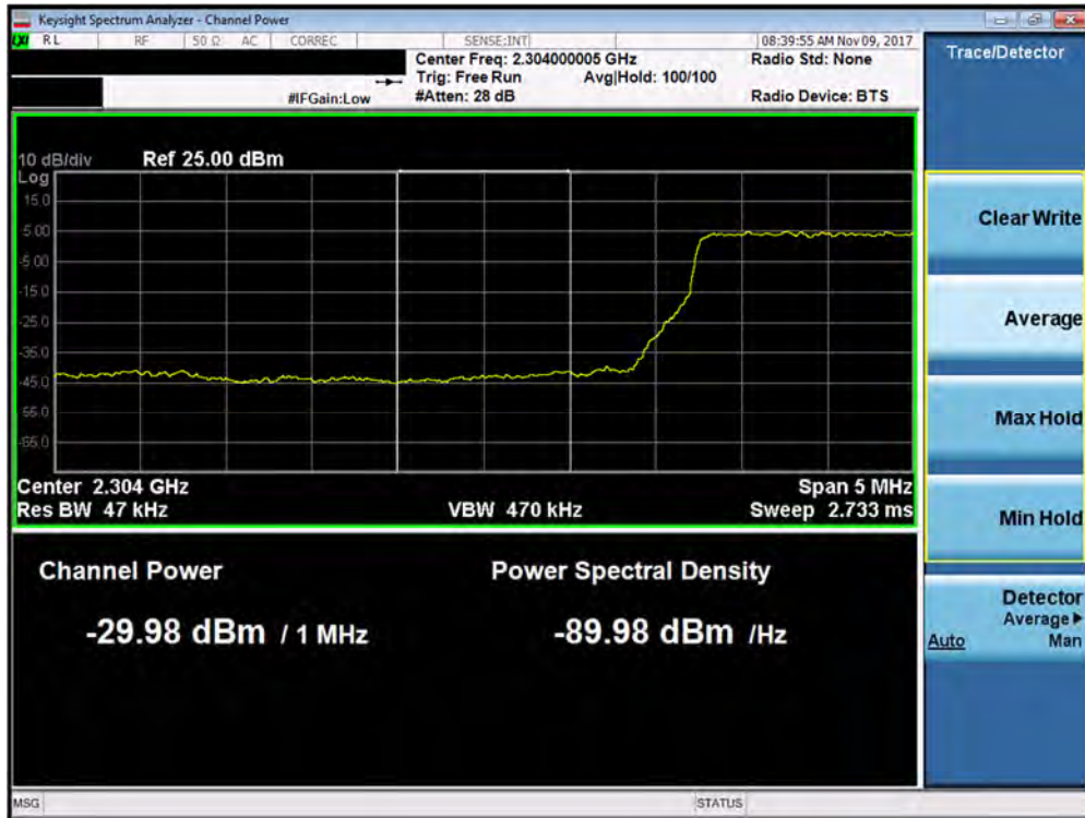
Plot 7-339. Lower Extended Band Edge Plot (Band 30 - 5.0MHz QPSK - Full RB Configuration- Antenna B)
