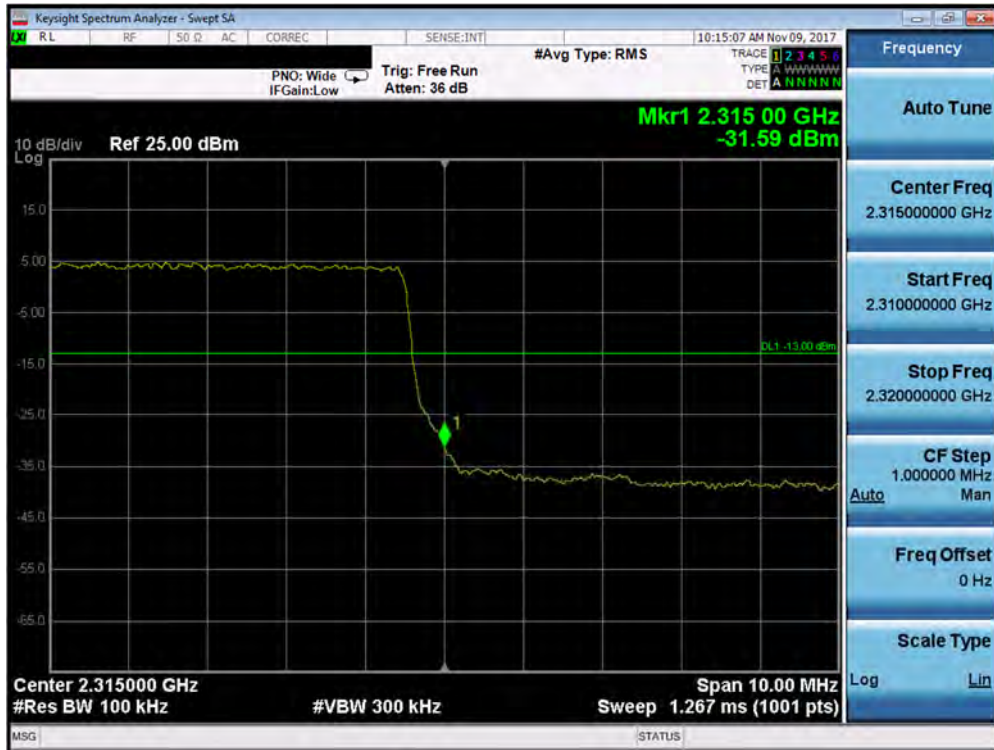
Plot 7-344. Upper Band Edge Plot (Band 30 - 10.0MHz QPSK - Full RB Configuration- Antenna B)
