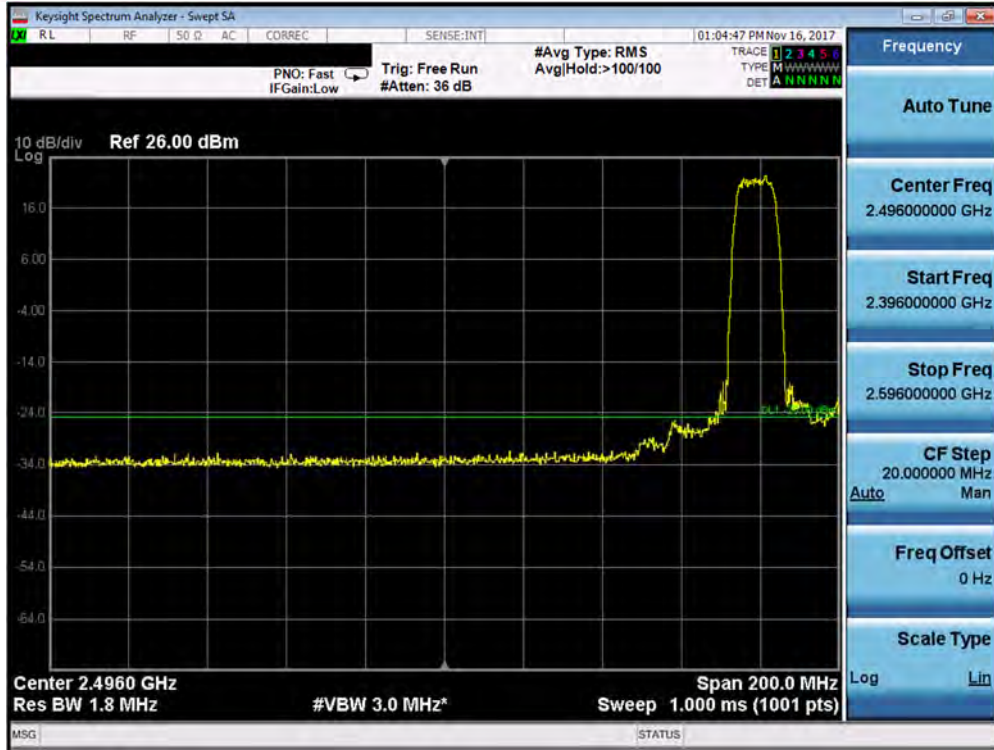
Plot 7-381. Lower ACP Plot (Band 38 – 10.0MHz QPSK – RB Size 50)
