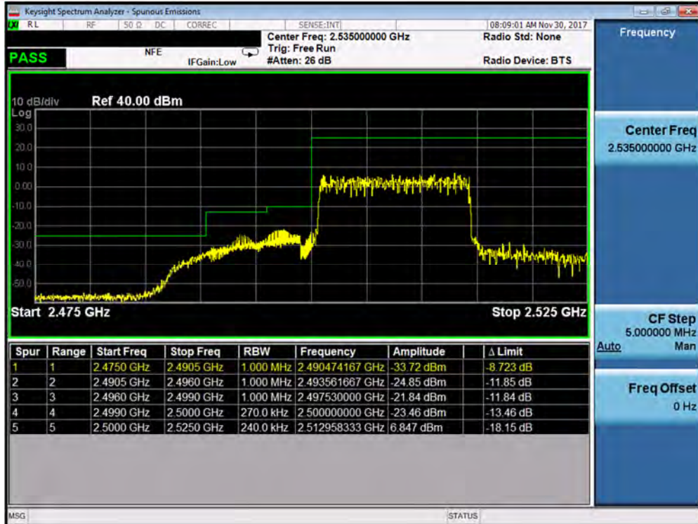
Plot 7-367. Lower ACP Plot (Band 7 – 15.0MHz QPSK – RB Size 75– Antenna A)
