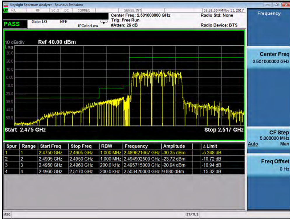
Plot 7-373. Lower ACP Plot (Band 41 – 10.0MHz QPSK – RB Size 50)
