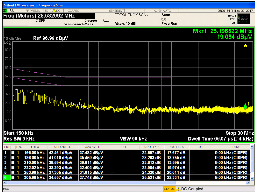
Plot 7-11. Line-Conducted Test Plot (N) - Terminated in 50Ω
