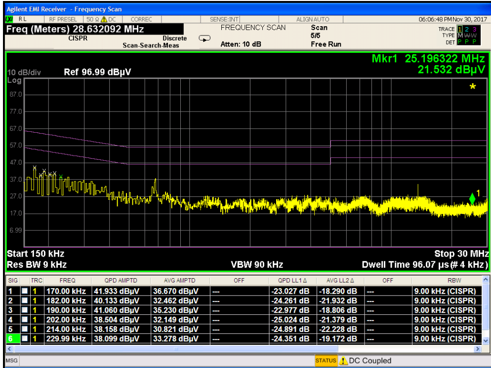
Plot 7-10. Line-Conducted Test Plot (L1) - Terminated in 50Ω
