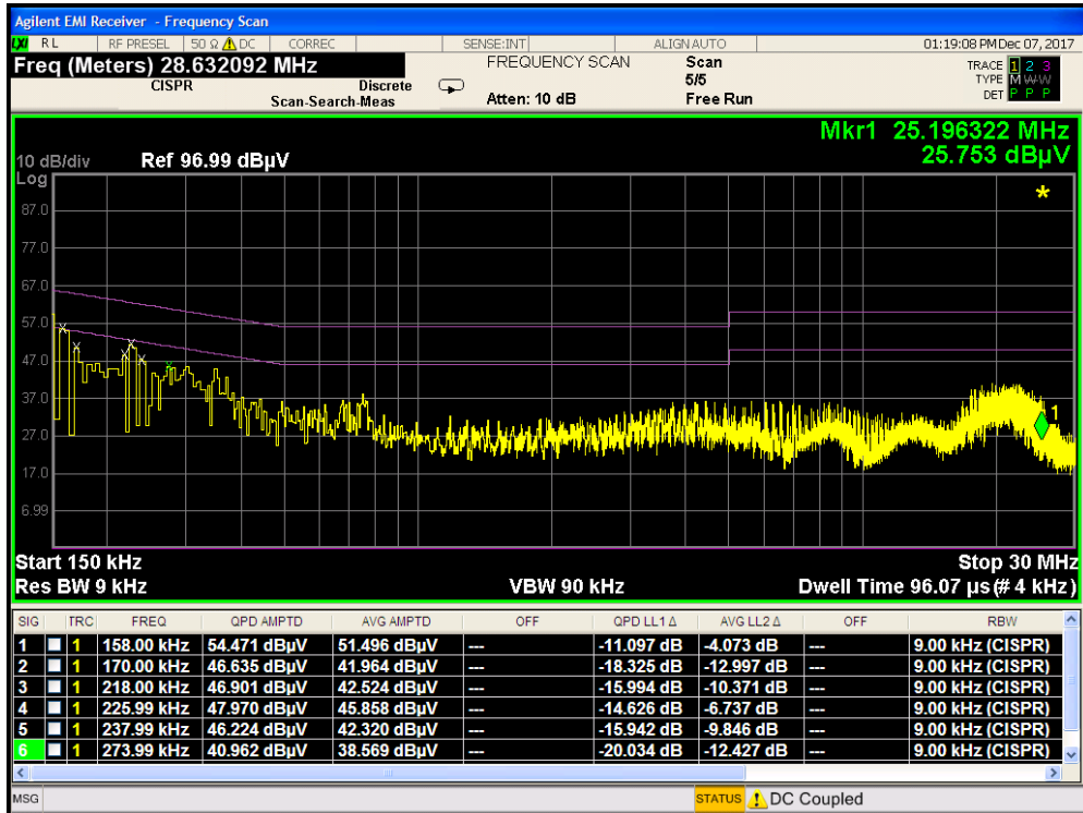
Plot 7-13. Line-Conducted Test Plot (N) with WCP - Terminated in 50Ω
