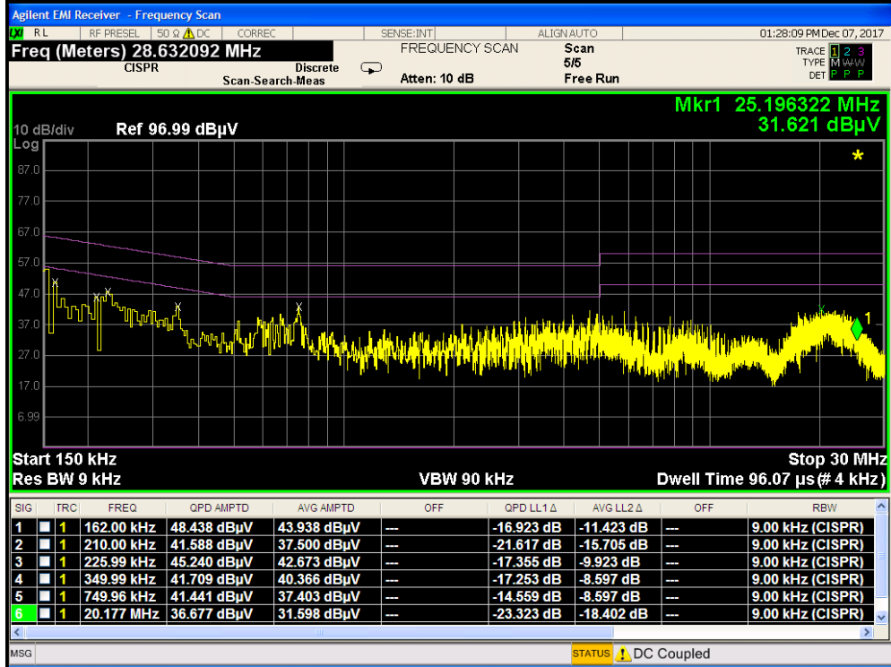
Plot 7-12. Line-Conducted Test Plot (L1) with WCP - Terminated in 50Ω
