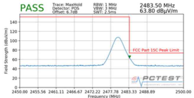
Plot 7-53. Radiated Restricted Upper Band Edge Measurement with WCP (Peak)
