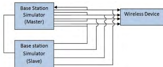
Figure I-5 Power Measurement Setup for LAA 4X4 MIMO
