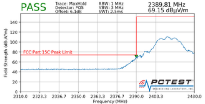
Plot 7-96. Radiated Restricted Band Edge Measurement (Peak)
