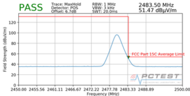
Plot 7-37. Radiated Restricted Upper Band Edge Measurement with WCP (Average)
