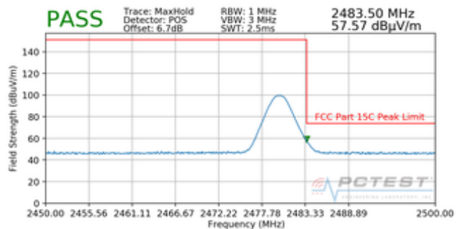
Plot 7-36. Radiated Restricted Upper Band Edge Measurement (Peak)
