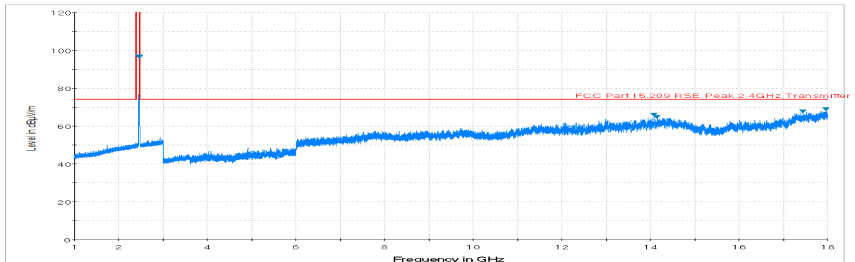
Plot 7-6. Radiated Spurious Plot above 1GHz (802.11b – Ch. 11, Ant. Pol. V)
