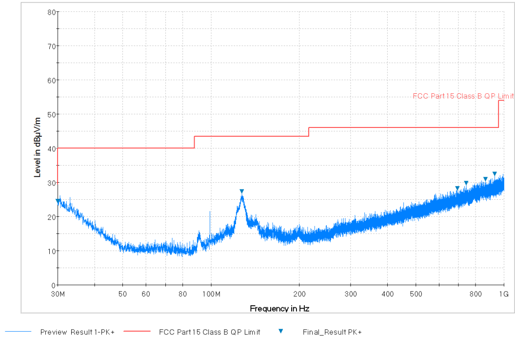
Plot 7-29. Radiated Spurious Plot below 1GHz (Pol. H)
