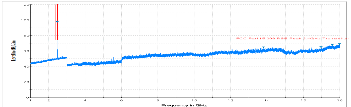
Plot 7-14. Radiated Spurious Plot above 1GHz (802.11b – Ch. 11, Ant. Pol. V)
