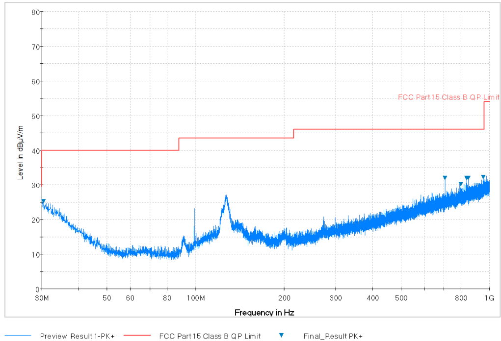
Plot 7-31. Radiated Spurious Plot below 1GHz (Pol. H)
