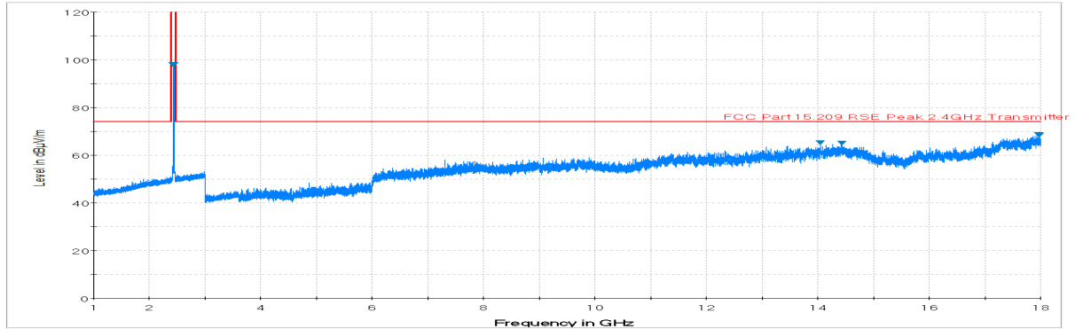
Plot 7-12. Radiated Spurious Plot above 1GHz (802.11b – Ch. 6, Ant. Pol. V)
