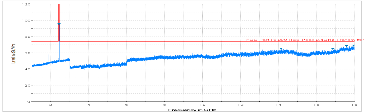
Plot 7-4. Radiated Spurious Plot above 1GHz (802.11b – Ch. 6, Ant. Pol. V)
