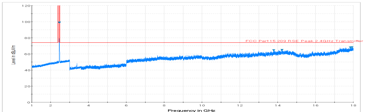
Plot 7-5. Radiated Spurious Plot above 1GHz (802.11b – Ch. 11, Ant. Pol. H)
