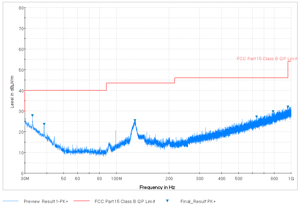
Plot 7-30. Radiated Spurious Plot below 1GHz (Pol. V)
