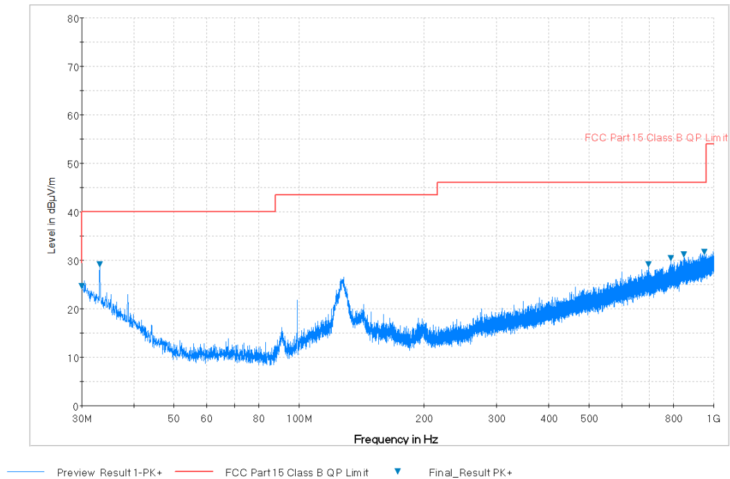
Plot 7-32. Radiated Spurious Plot below 1GHz (Pol. V)
