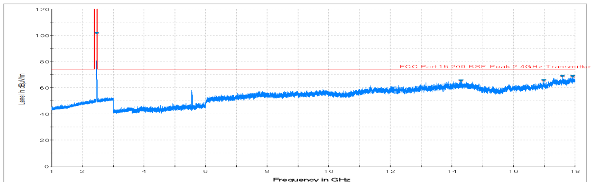
Plot 7-13. Radiated Spurious Plot above 1GHz (802.11b – Ch. 11, Ant. Pol. H)
