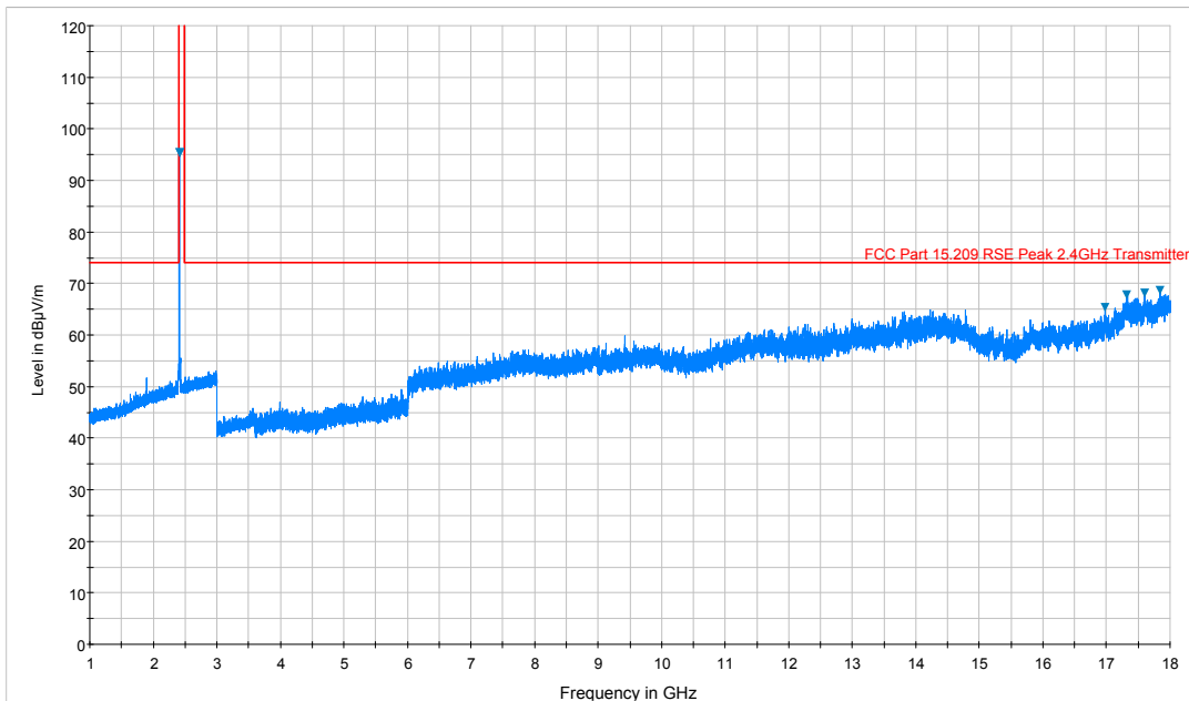
Plot 7-10. Radiated Spurious Plot above 1GHz (802.11b – Ch. 1, Ant. Pol. V)
