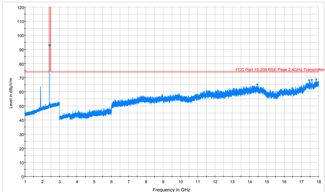
Plot 7-2. Radiated Spurious Plot above 1GHz (802.11b – Ch. 1, Ant. Pol. V)
