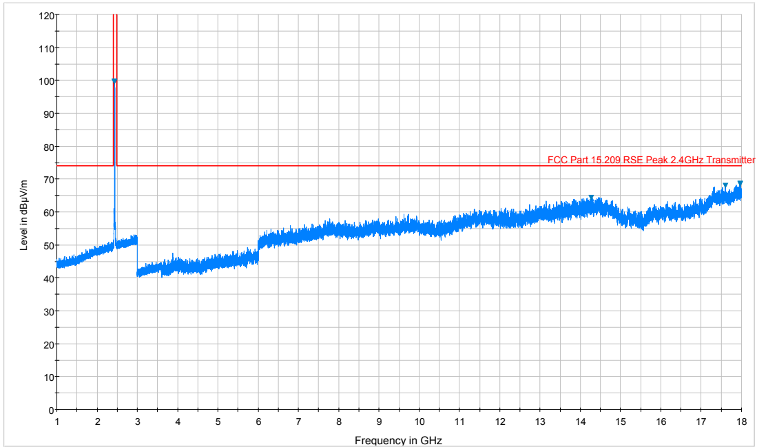
Plot 7-11. Radiated Spurious Plot above 1GHz (802.11b – Ch. 6, Ant. Pol. H)
