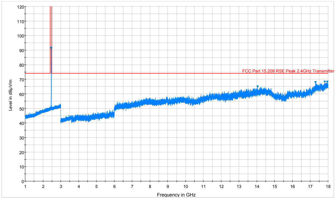
Plot 7-6. Radiated Spurious Plot above 1GHz (802.11b – Ch. 11, Ant. Pol. V)
