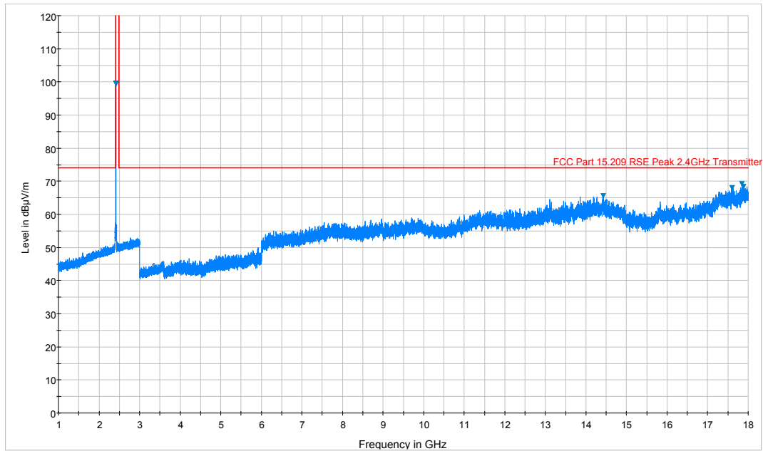
Plot 7-1. Radiated Spurious Plot above 1GHz (802.11b – Ch. 1, Ant. Pol. H)
