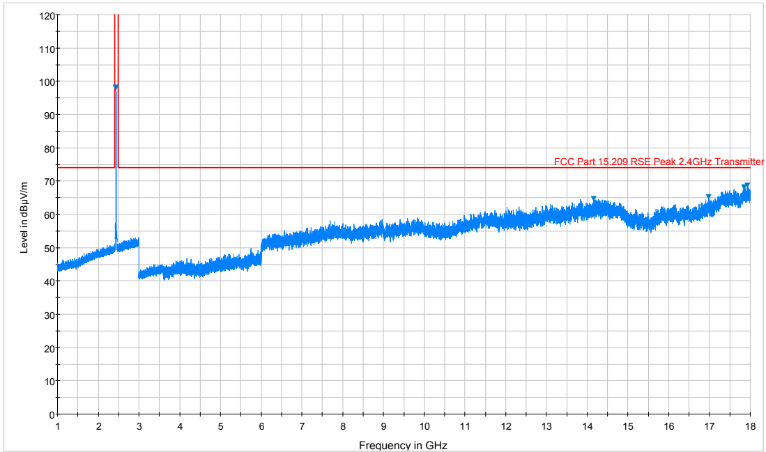
Plot 7-3. Radiated Spurious Plot above 1GHz (802.11b – Ch. 6, Ant. Pol. H)
