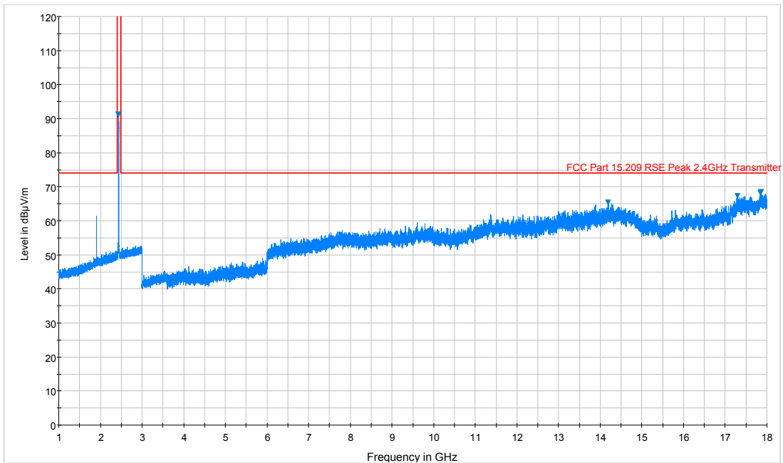
Plot 7-4. Radiated Spurious Plot above 1GHz (802.11b – Ch. 6, Ant. Pol. V)
