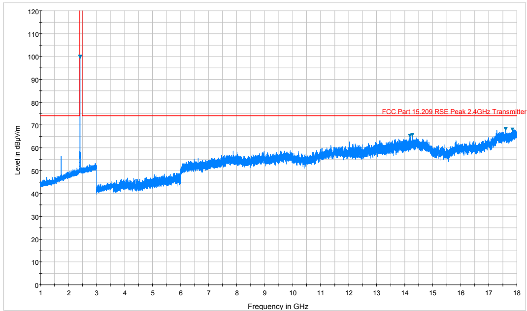
Plot 7-9. Radiated Spurious Plot above 1GHz (802.11b – Ch. 1, Ant. Pol. H)
