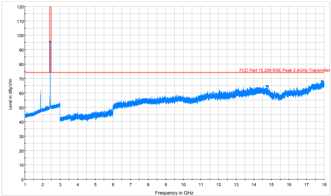
Plot 7-12. Radiated Spurious Plot above 1GHz (802.11b – Ch. 6, Ant. Pol. V)
