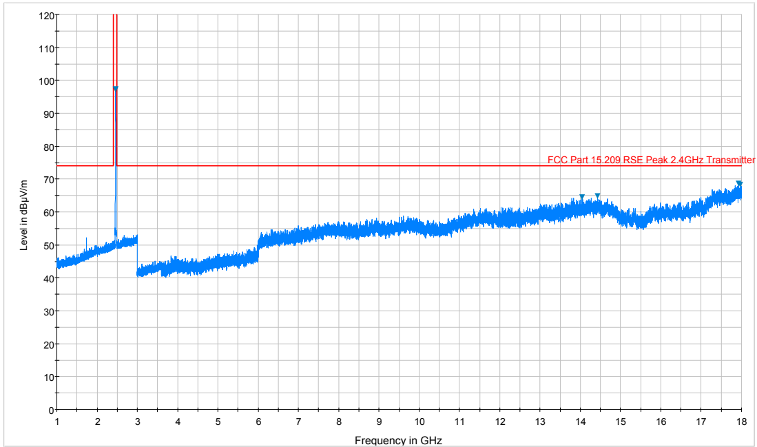
Plot 7-13. Radiated Spurious Plot above 1GHz (802.11b – Ch. 11, Ant. Pol. H)
