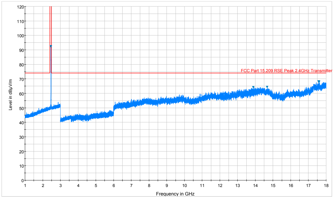
Plot 7-14. Radiated Spurious Plot above 1GHz (802.11b – Ch. 11, Ant. Pol. V)
