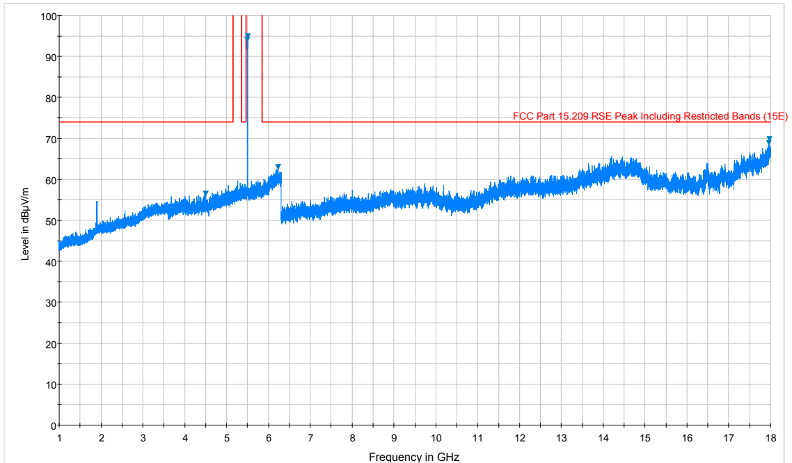
Plot 7-18. Radiated Spurious Plot above 1GHz (802.11a – U2C Ch. 116, Ant. Pol. V)
