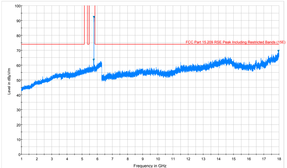
Plot 7-8. Radiated Spurious Plot above 1GHz (802.11a – U3 Ch. 157, Ant. Pol. V)
