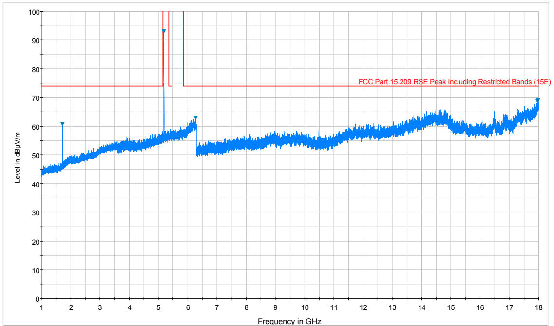
Plot 7-1. Radiated Spurious Plot above 1GHz (802.11a – U1 Ch. 40, Ant. Pol. H)
