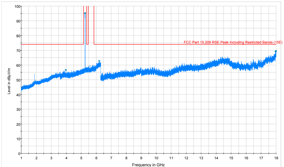
Plot 7-16. Radiated Spurious Plot above 1GHz (802.11a – U2A Ch. 56, Ant. Pol. V)
