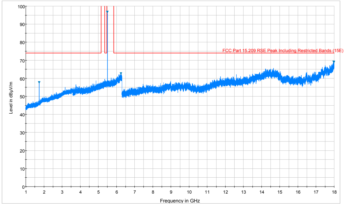
Plot 7-17. Radiated Spurious Plot above 1GHz (802.11a – U2C Ch. 116, Ant. Pol. H)
