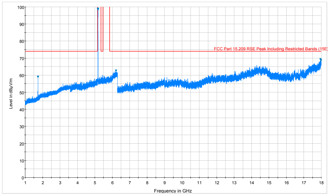
Plot 7-13. Radiated Spurious Plot above 1GHz (802.11a – U1 Ch. 40, Ant. Pol. H)
