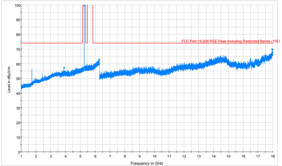
Plot 7-15. Radiated Spurious Plot above 1GHz (802.11a – U2A Ch. 56, Ant. Pol. H)
