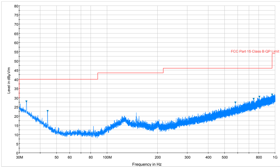
Plot 7-52. Radiated Spurious Plot below 1GHz (802.11a – U3 Ch. 157, Ant. Pol. V)
