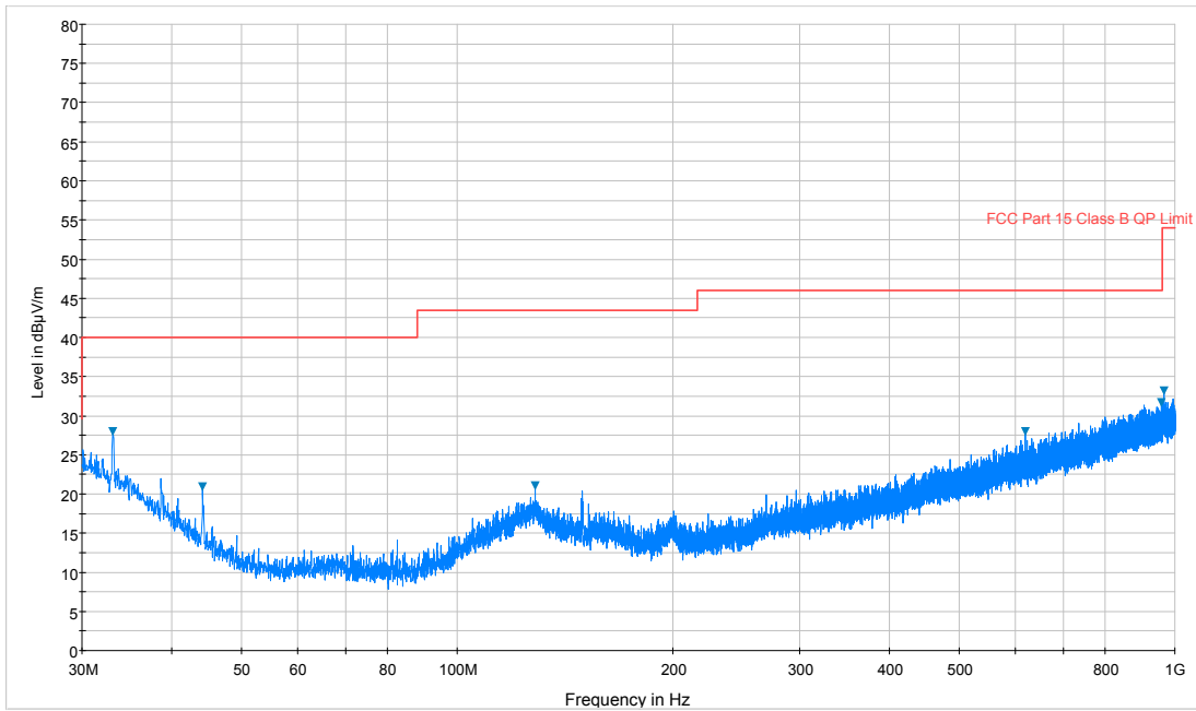
Plot 7-50. Radiated Spurious Plot below 1GHz (802.11a – U3 Ch. 157, Ant. Pol. V)
