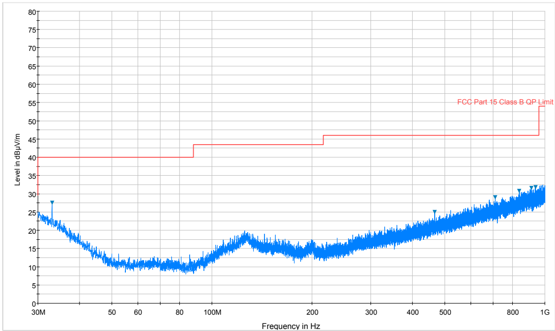
Plot 7-49. Radiated Spurious Plot below 1GHz (802.11a – U3 Ch. 157, Ant. Pol. H)
