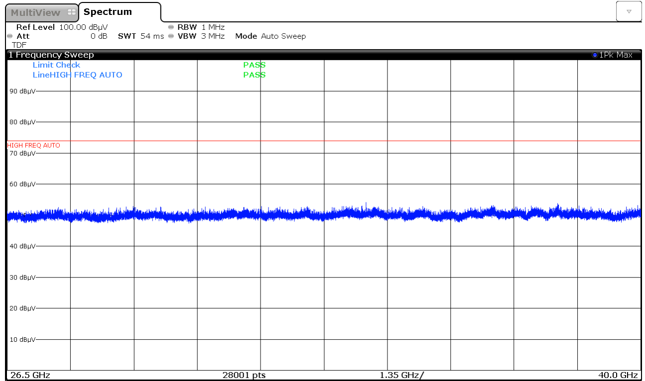
Plot 7-30. Radiated Spurious Plot above 26.5GHz (Config-1 RSDB, Ant. Pol. V)
