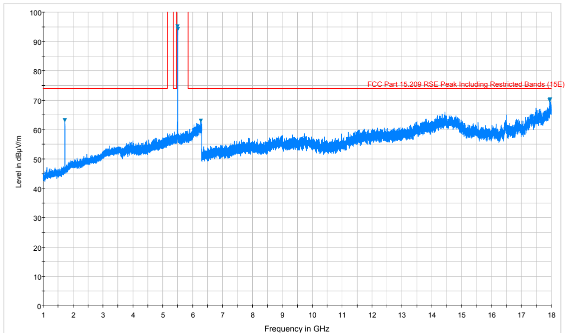
Plot 7-6. Radiated Spurious Plot above 1GHz (802.11a – U2C Ch. 116, Ant. Pol. V)
