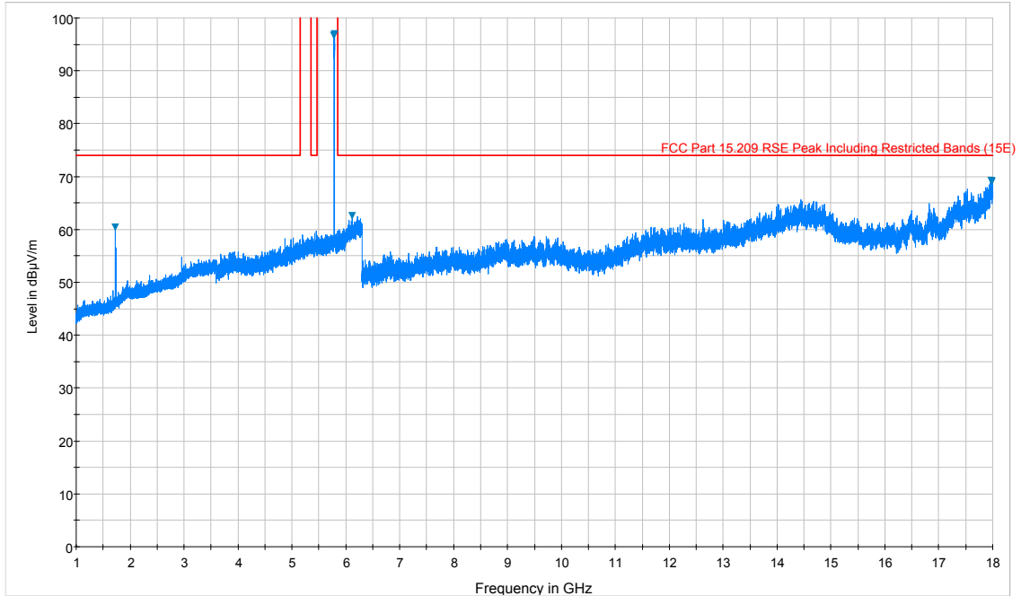
Plot 7-19. Radiated Spurious Plot above 1GHz (802.11a – U3 Ch. 157, Ant. Pol. H)
