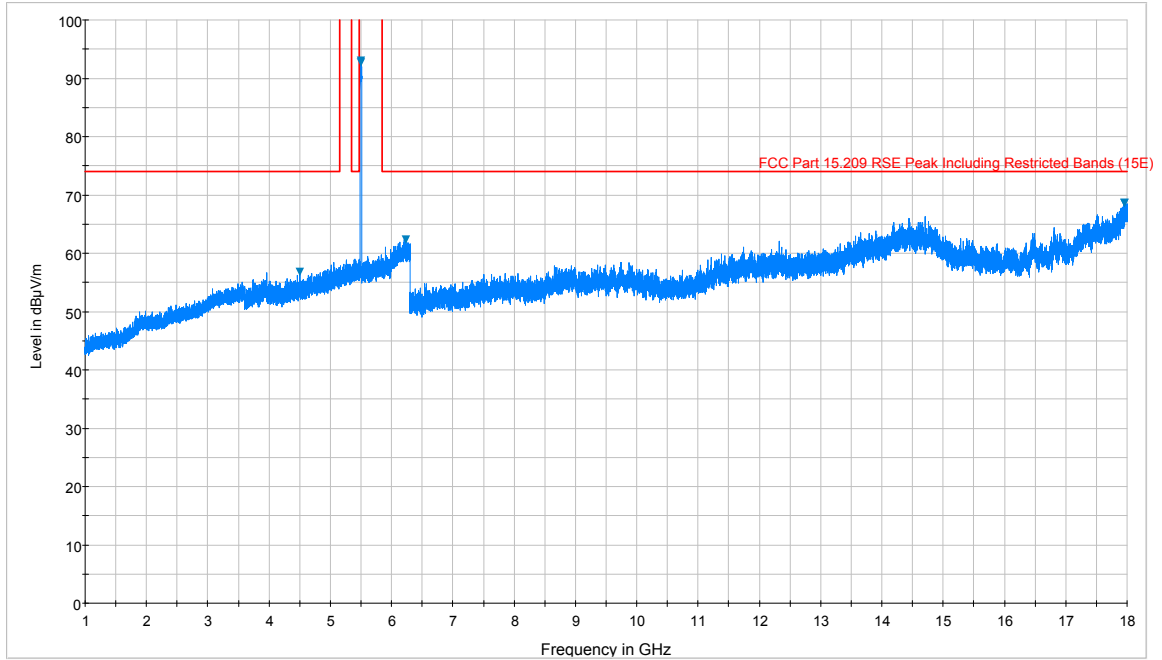
Plot 7-5. Radiated Spurious Plot above 1GHz (802.11a – U2C Ch. 116, Ant. Pol. H)
