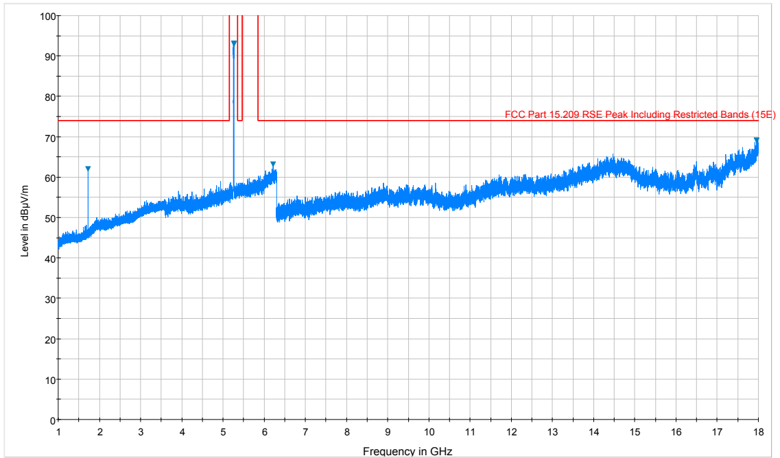
Plot 7-3. Radiated Spurious Plot above 1GHz (802.11a – U2A Ch. 56, Ant. Pol. H)
