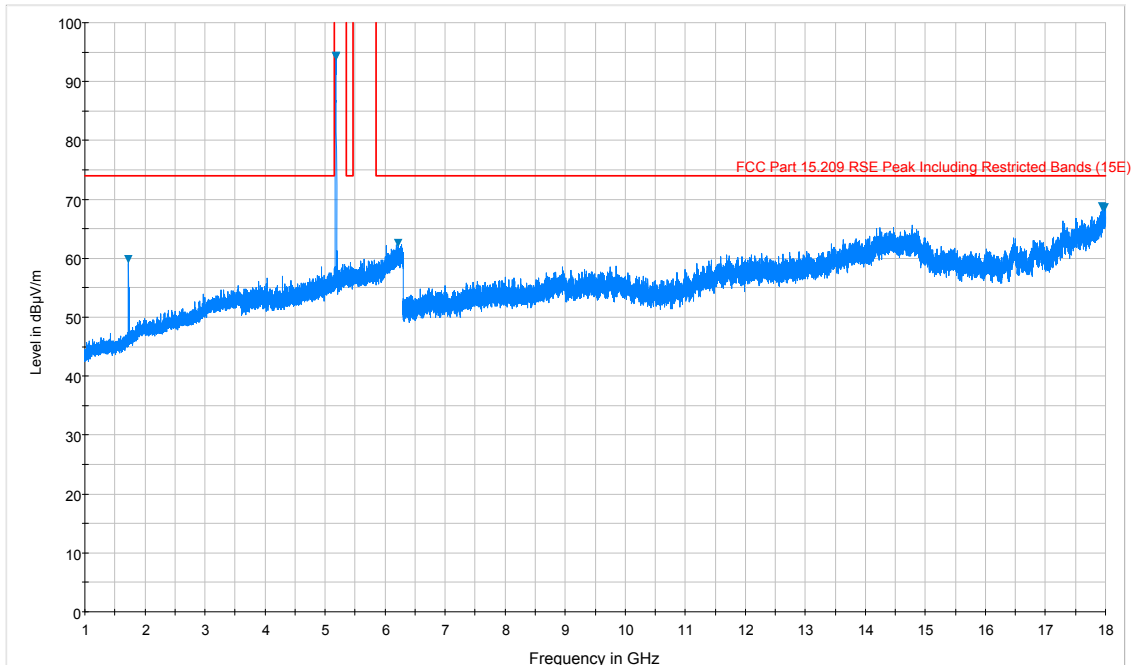
Plot 7-2. Radiated Spurious Plot above 1GHz (802.11a – U1 Ch. 40, Ant. Pol. V)
