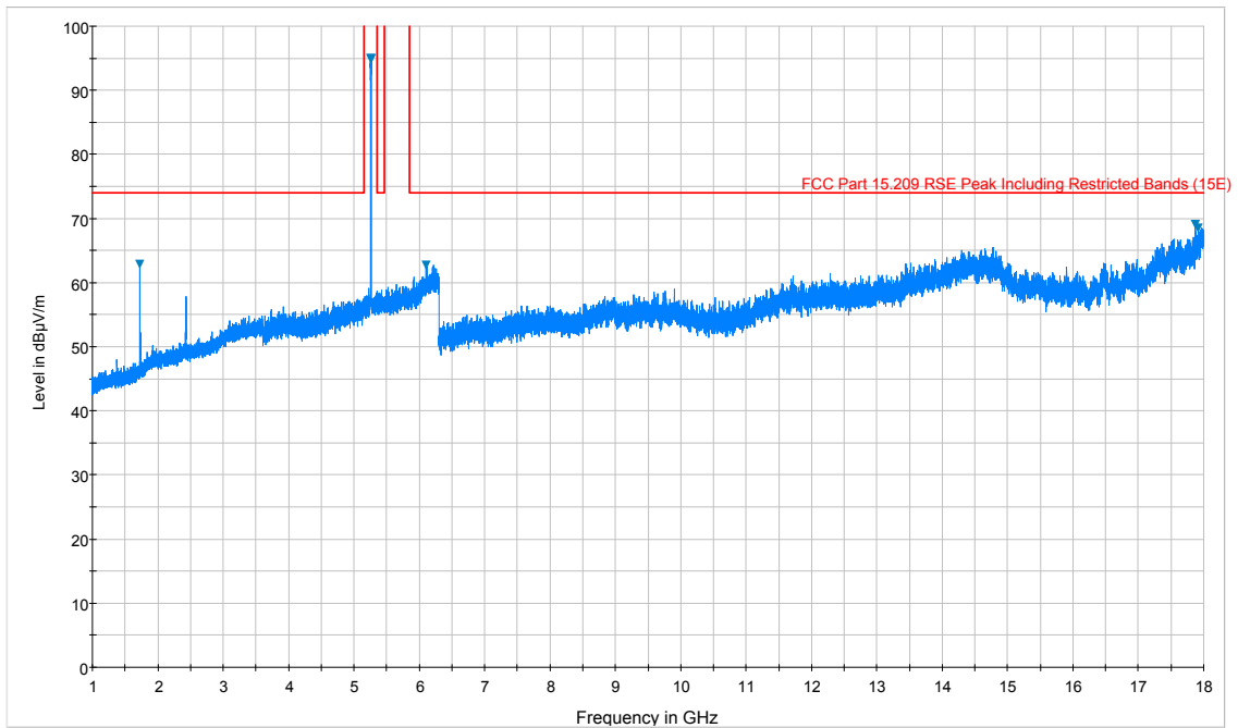
Plot 7-4. Radiated Spurious Plot above 1GHz (802.11a – U2A Ch. 56, Ant. Pol. V)
