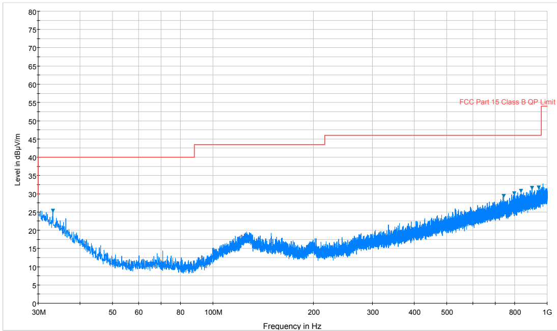
Plot 7-51. Radiated Spurious Plot below 1GHz (802.11a – U3 Ch. 157, Ant. Pol. H)
