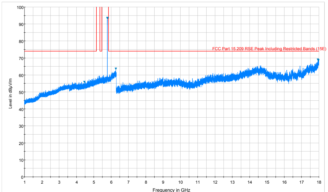
Plot 7-20. Radiated Spurious Plot above 1GHz (802.11a – U3 Ch. 157, Ant. Pol. V)
