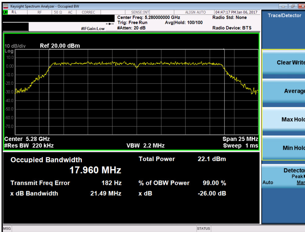
Plot 7-44. 26dB Bandwidth Plot (20MHz BW 802.11n (UNII Band 2A) – Ch. 56)
