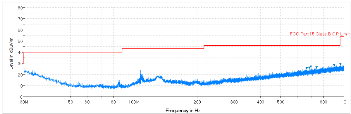
Plot 7-30. Radiated Spurious Plot below 1GHz (Pol. V)
