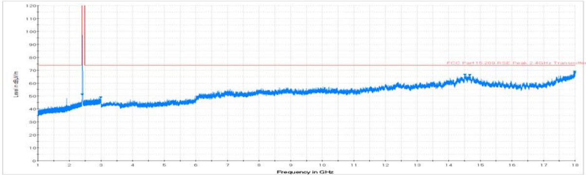
Plot 7-9. Radiated Spurious Plot above 1GHz (802.11b – Ch. 1, Ant. Pol. H)
