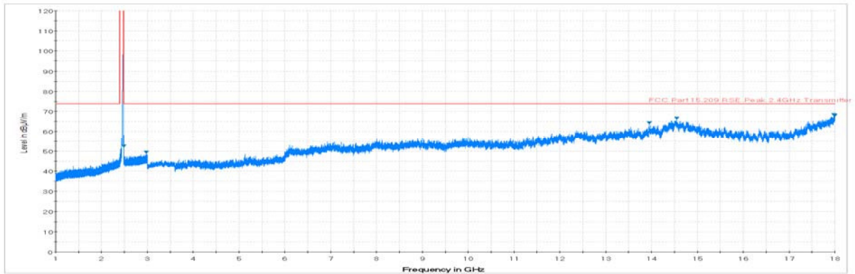
Plot 7-13. Radiated Spurious Plot above 1GHz (802.11b – Ch. 11, Ant. Pol. H)
