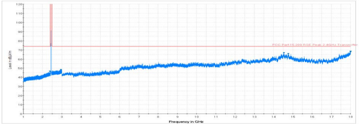
Plot 7-12. Radiated Spurious Plot above 1GHz (802.11b – Ch. 6, Ant. Pol. V)
