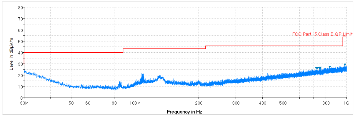
Plot 7-57. Radiated Spurious Plot below 1GHz (802.11a – U3 Ch. 157, Ant. Pol. V)
