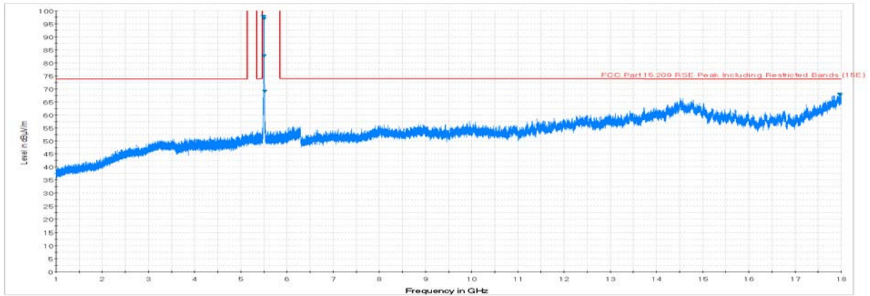
Plot 7-17. Radiated Spurious Plot above 1GHz (802.11a – U2C Ch. 120, Ant. Pol. H)
