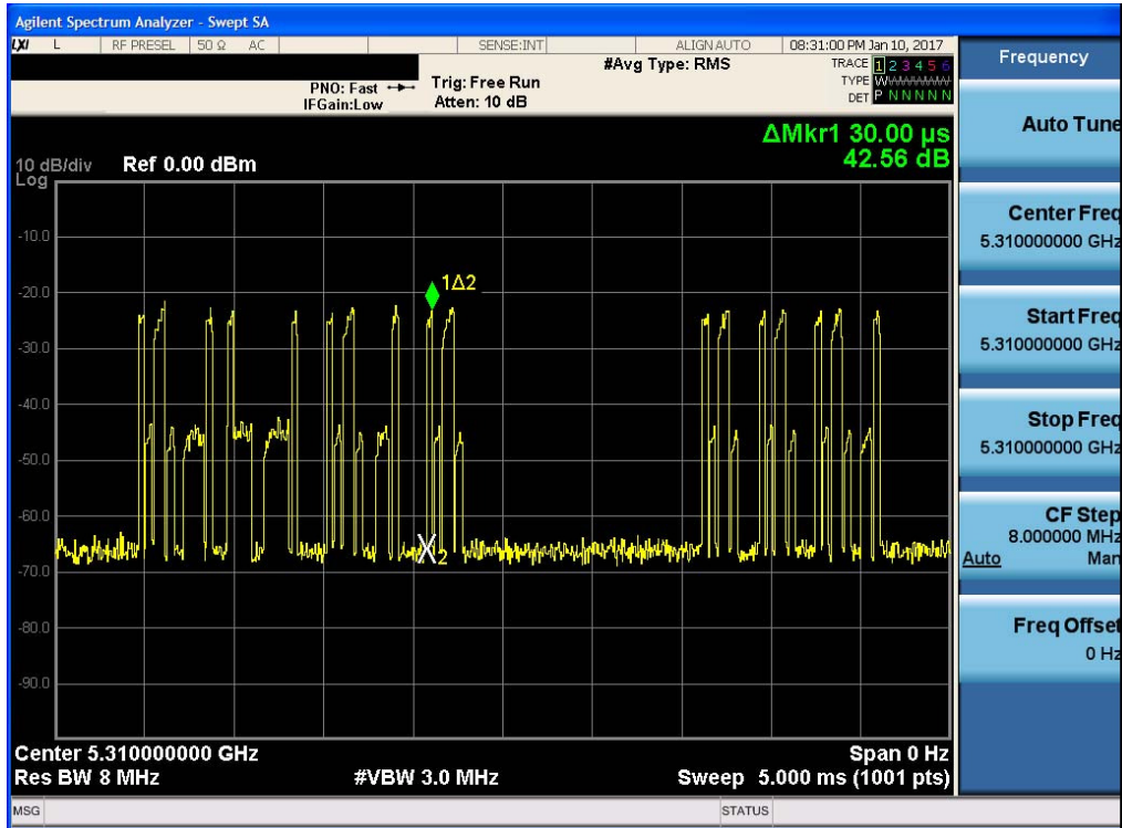
Figure 5-1. Band 2A Pulse Width
