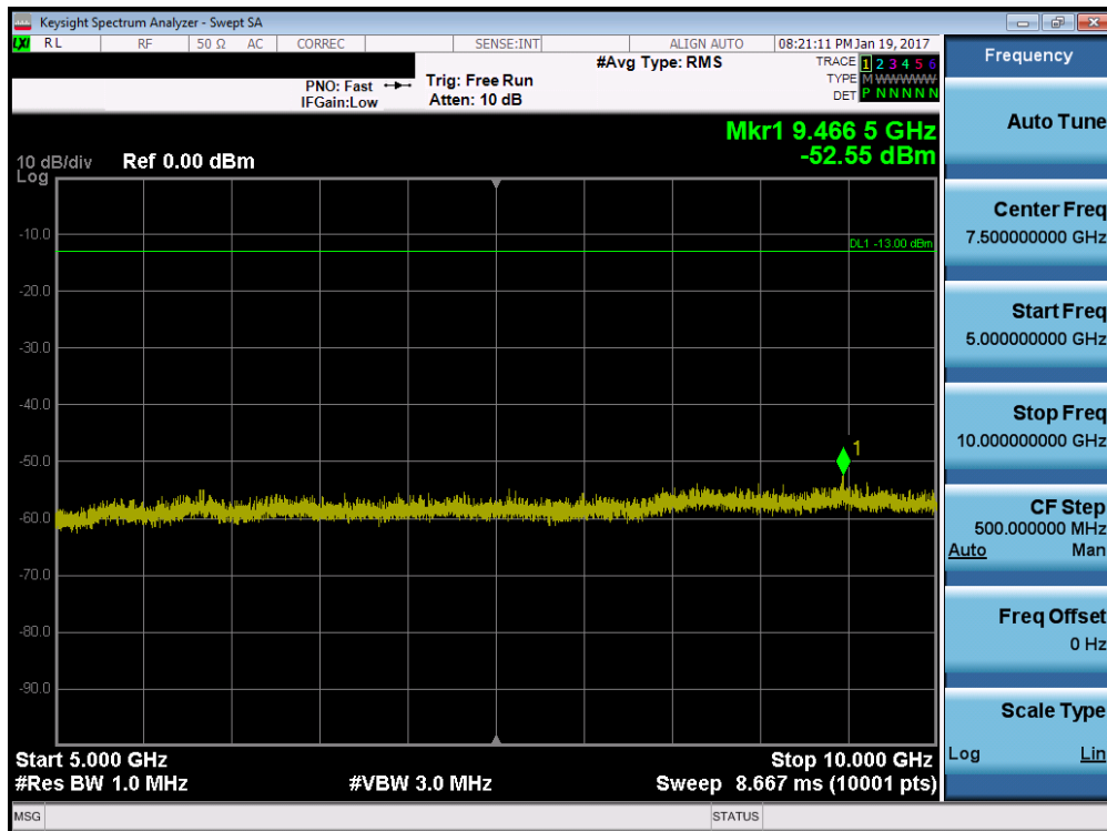
Plot 7-19. Conducted Spurious Plot (3MHz QPSK – RB Size 1, RB Offset 0 – High Channel)
