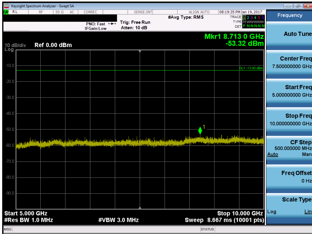
Plot 7-17. Conducted Spurious Plot (3MHz QPSK – RB Size 1, RB Offset 0 – Low Channel)
