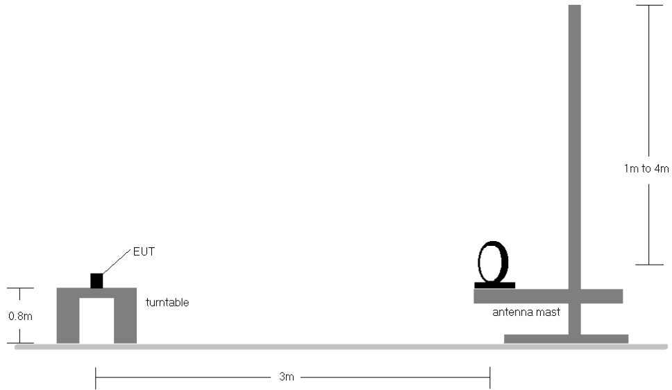
Figure 8-6. Radiated Test Setup < 30MHz
