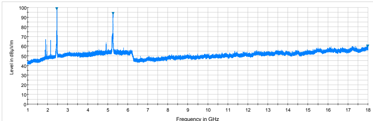
Plot 7-178. Radiated Spurious Plot above 1GHz (Simultaneous Transmission Config-1, Ant. Pol. V)
