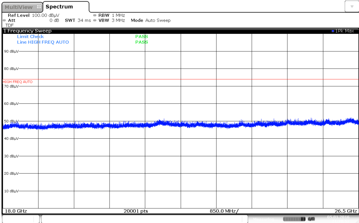
Plot 7-181. Radiated Spurious Plot 18GHz – 26.5GHz (Simultaneous Transmission Config-1 Ant. Pol. V)
