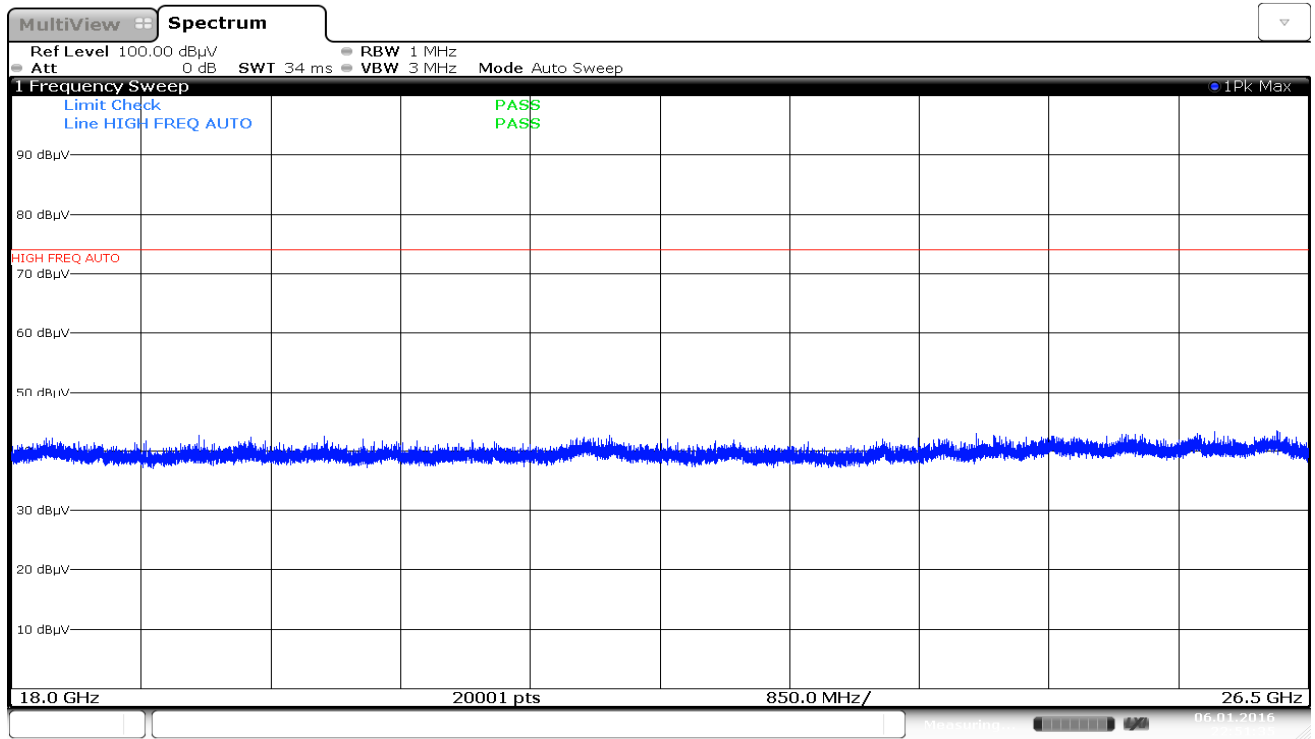
Plot 7-88. Radiated Spurious Plot above 18GHz (Pol. V)
