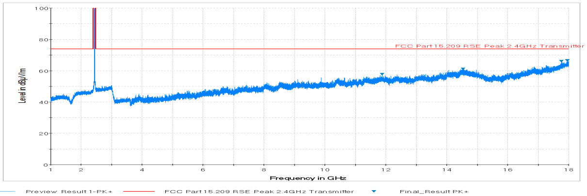
Plot 7-75. Radiated Spurious Plot above 1GHz (802.11b – Ch. 6, Ant. Pol. H)
