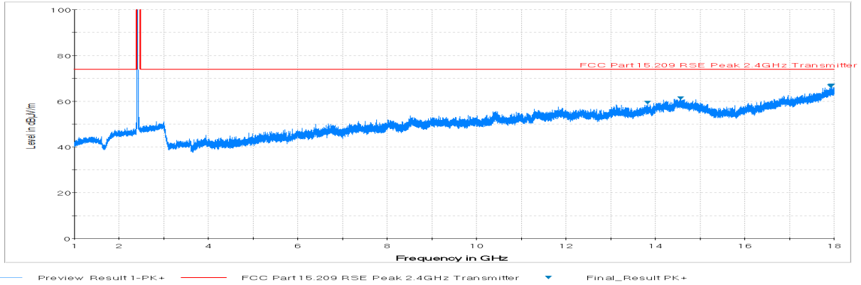
Plot 7-73. Radiated Spurious Plot above 1GHz (802.11b – Ch. 1, Ant. Pol. H)
