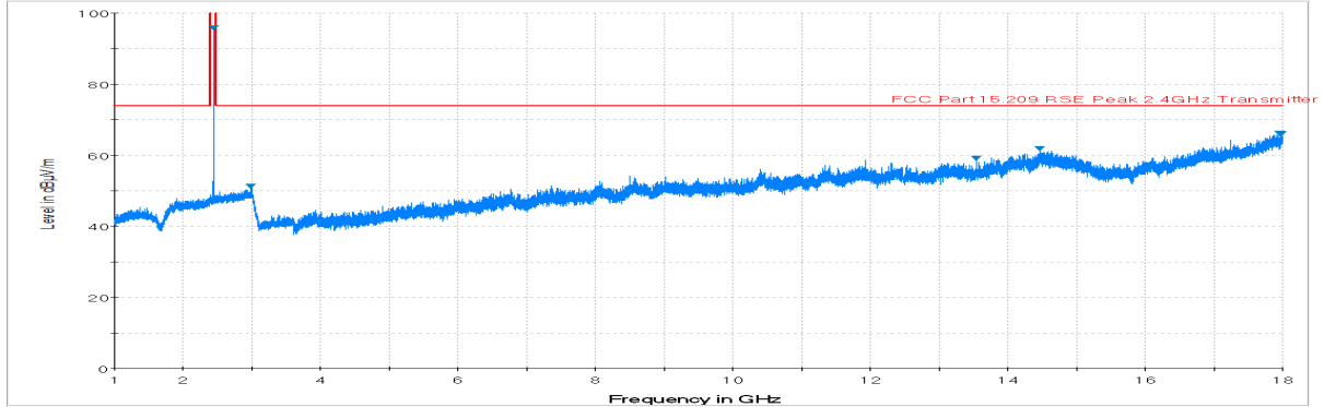
Plot 21. Radiated Spurious Plot above 1GHz (BT LE – Ch. 19, Ant. Pol. V)
