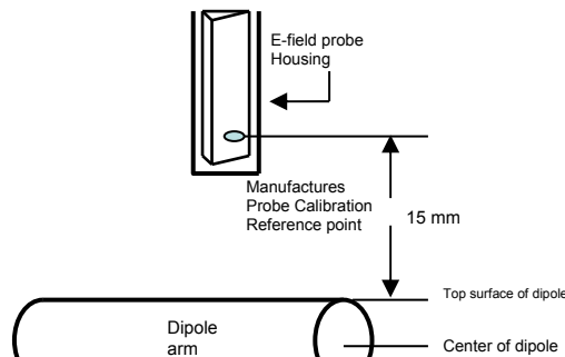
Figure 7-1 Separation Distance from Dipole to Field Probe
