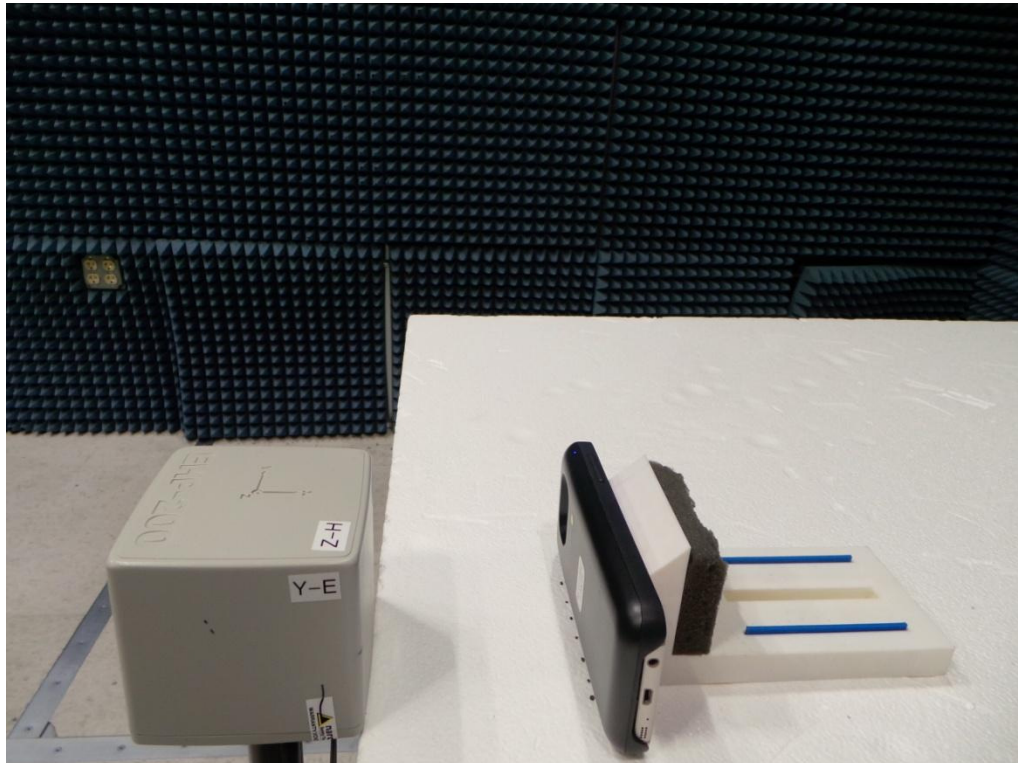
Figure 6. E-Field Measurement (Position F)
