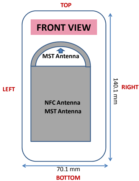
Figure F-2 NFC & MST Antenna Locations
