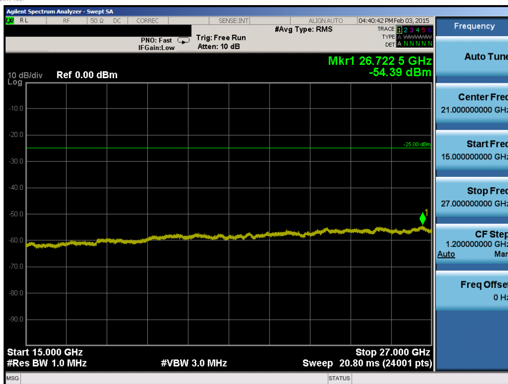
Plot 6-89. Conducted Spurious Plot (Band 41 – 5.0MHz QPSK – RB Size 1, RB Offset 0 – Low Channel)
