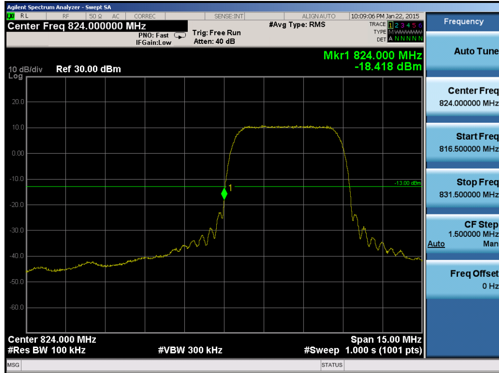
Plot 6-77. Band Edge Plot (Cellular WCDMA Mode – Ch. 4132)
