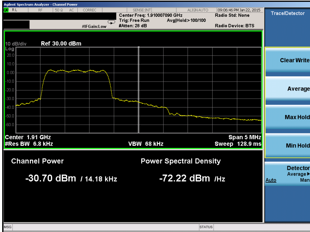
Plot 6-75. Band Edge Plot (PCS CDMA Mode – Ch. 1175)
