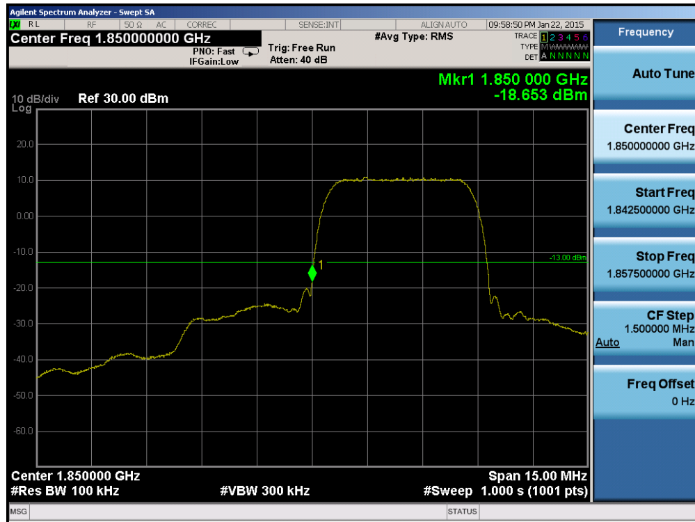
Plot 6-79. Band Edge Plot (PCS WCDMA Mode – Ch. 9262)
