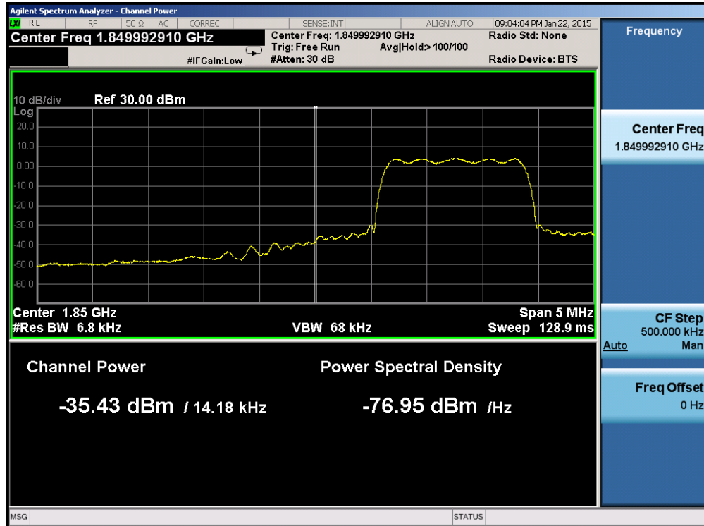
Plot 6-73. Band Edge Plot (PCS CDMA Mode – Ch. 25)
