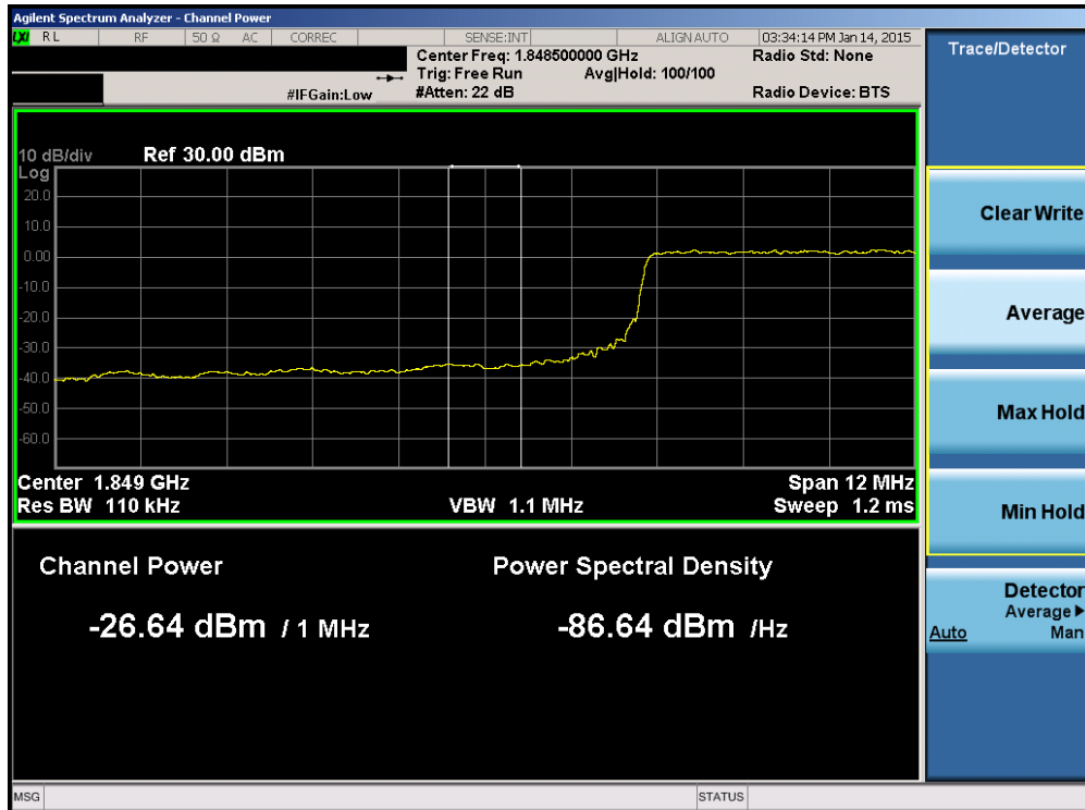
Plot 6-84. Lower Extended Band Edge Plot (Band 2 – 15.0MHz QPSK – RB Size 75)
