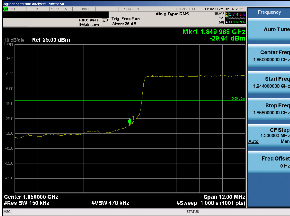
Plot 6-83. Lower Band Edge Plot (Band 2 – 15.0MHz QPSK – RB Size 75)
