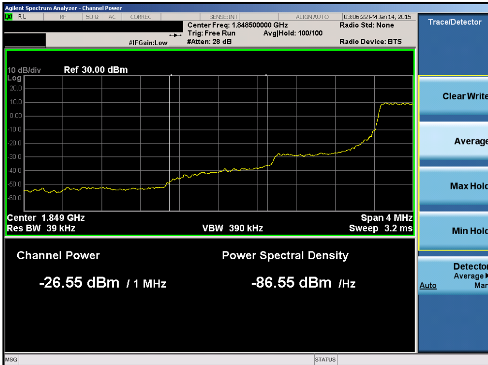
Plot 6-68. Lower Extended Band Edge Plot (Band 2 – 1.4MHz QPSK – RB Size 6)
