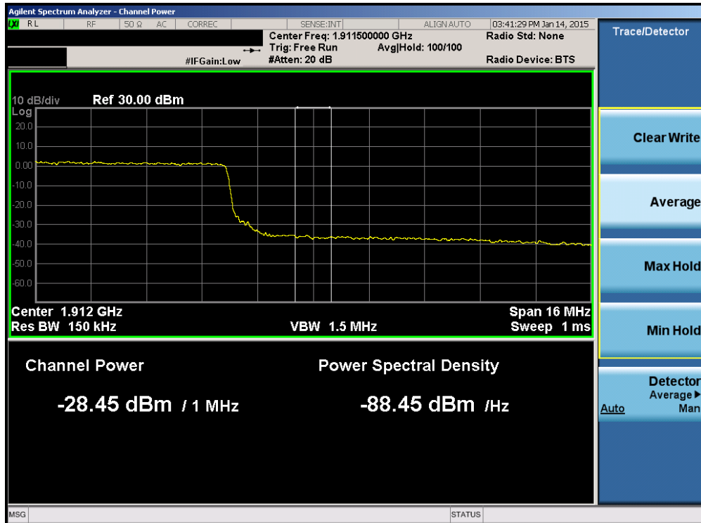
Plot 6-90. Upper Extended Band Edge Plot (Band 2 – 20.0MHz QPSK – RB Size 100)
