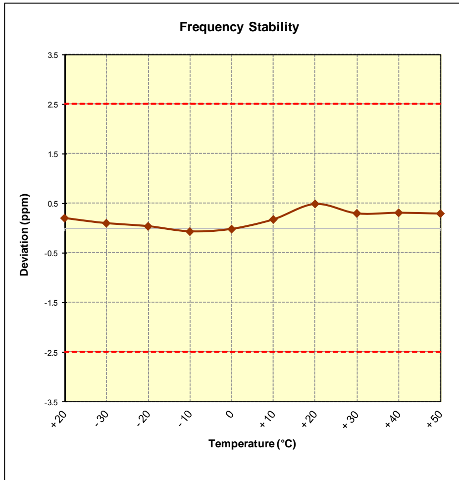
Figure 6-10. Frequency Stability Graph (Band 17)
