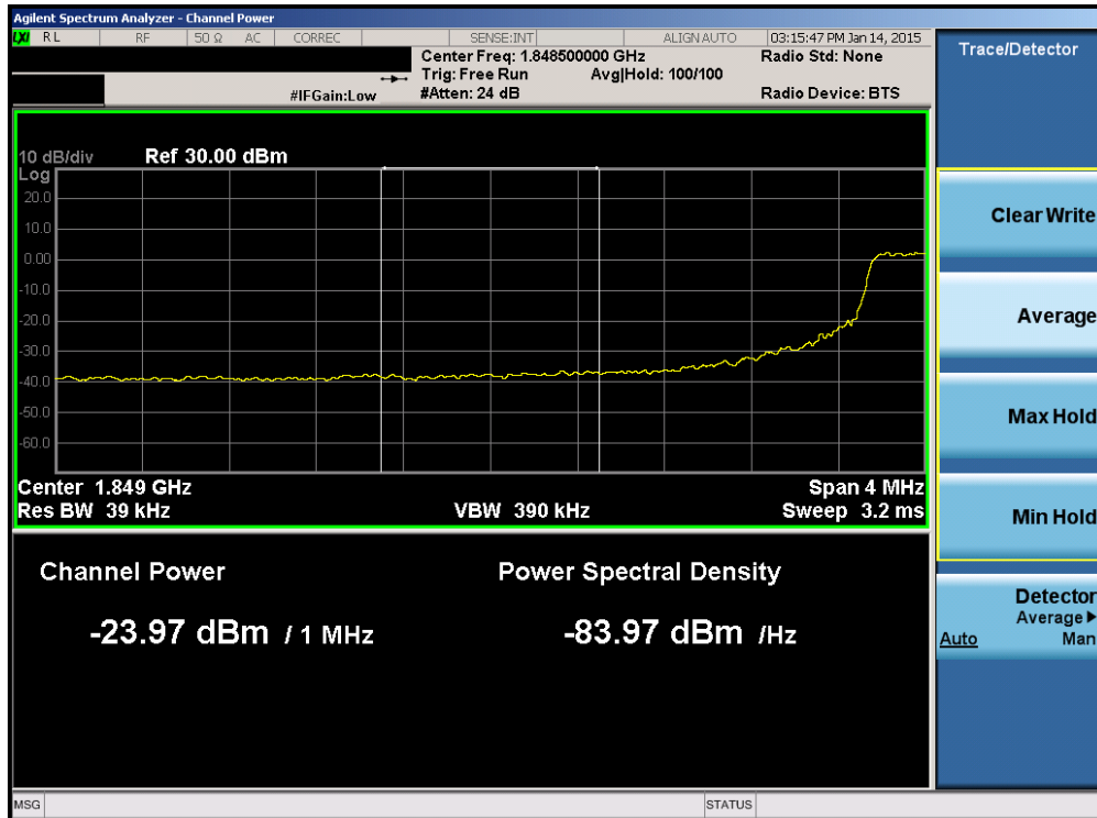
Plot 6-76. Lower Extended Band Edge Plot (Band 2 – 5.0MHz QPSK – RB Size 25)
