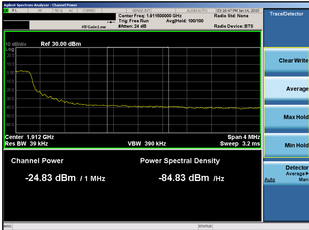
Plot 6-78. Upper Extended Band Edge Plot (Band 2 – 5.0MHz QPSK – RB Size 25)
