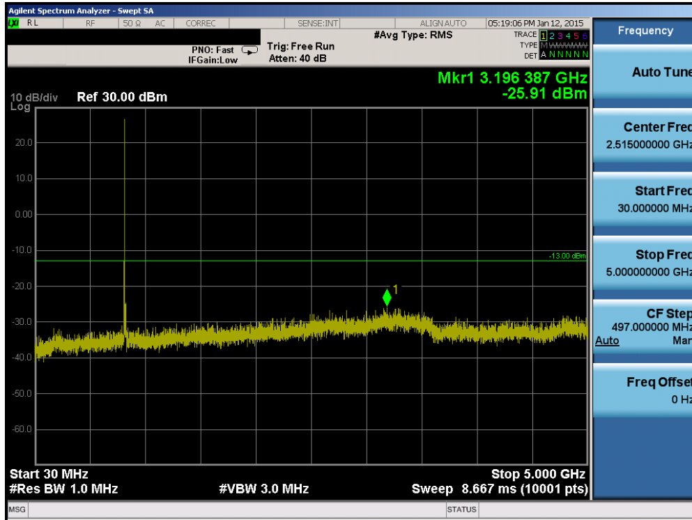
Plot 6-37. Conducted Spurious Plot (Band 26 – 3.0MHz QPSK – RB Size 1, RB Offset 0 – High Channel)
