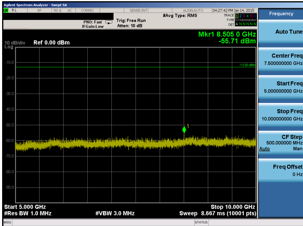
Plot 6-30. Conducted Spurious Plot (Band 17 – 5.0MHz QPSK – RB Size 1, RB Offset 0 – Mid Channel)
