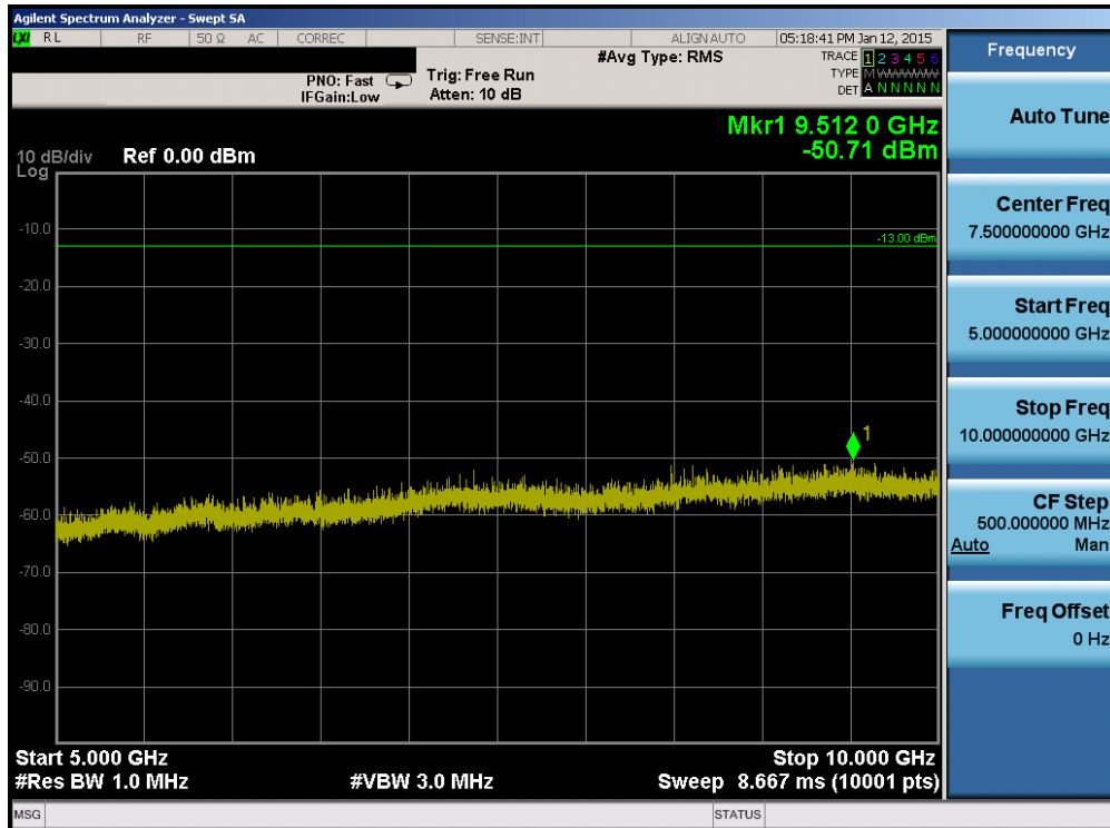
Plot 6-36. Conducted Spurious Plot (Band 26 – 3.0MHz QPSK – RB Size 1, RB Offset 0 – Mid Channel)
