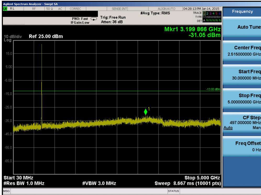
Plot 6-31. Conducted Spurious Plot (Band 17 – 5.0MHz QPSK – RB Size 1, RB Offset 0 – High Channel)
