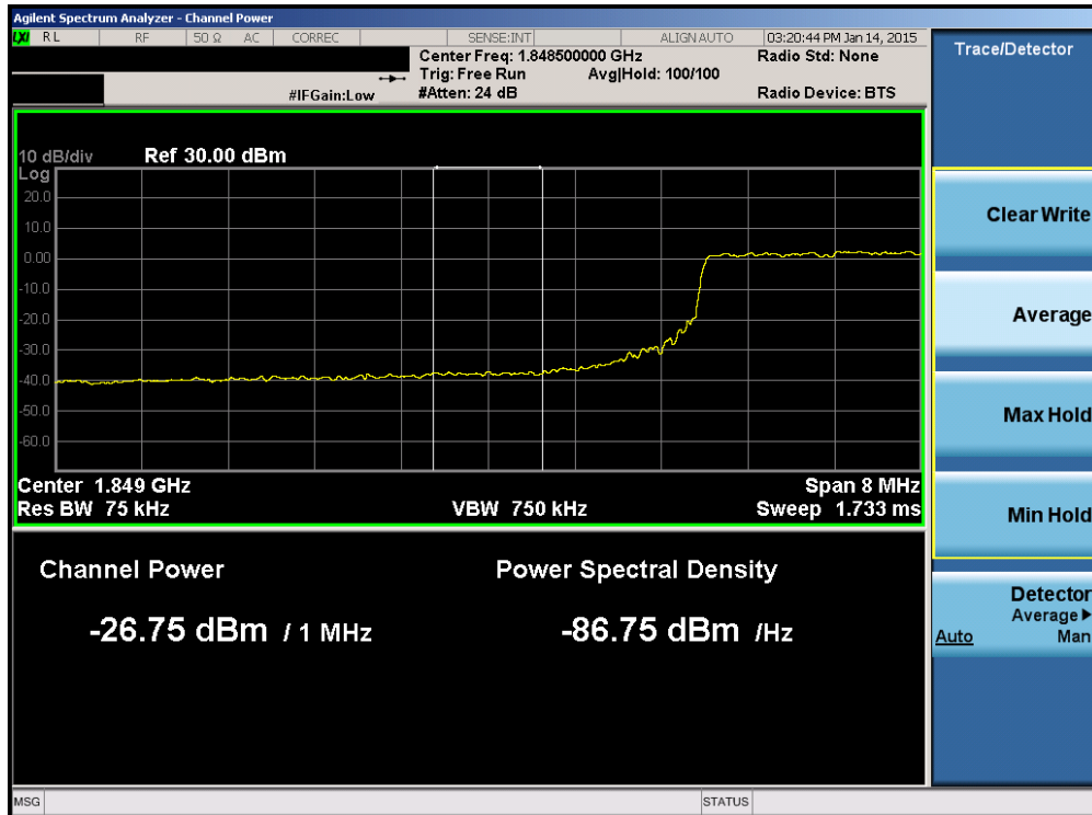
Plot 6-80. Lower Extended Band Edge Plot (Band 2 – 10.0MHz QPSK – RB Size 50)
