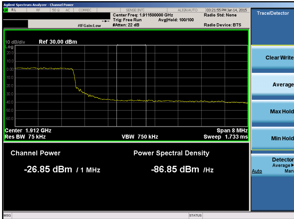
Plot 6-82. Upper Extended Band Edge Plot (Band 2 – 10.0MHz QPSK – RB Size 50)
