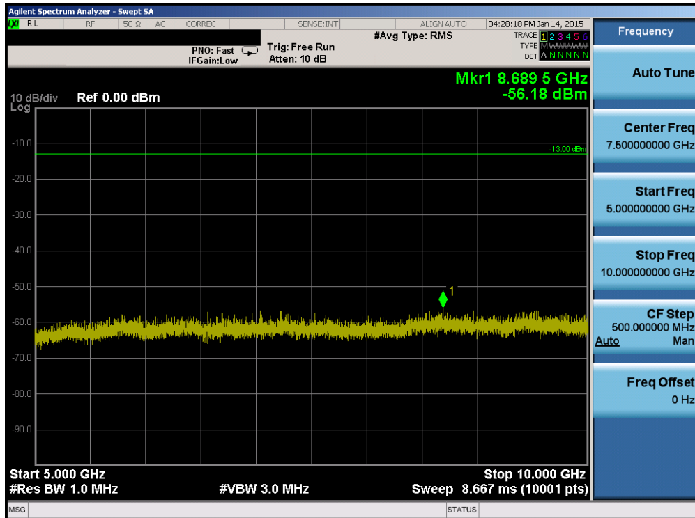
Plot 6-32. Conducted Spurious Plot (Band 17 – 5.0MHz QPSK – RB Size 1, RB Offset 0 – High Channel)
