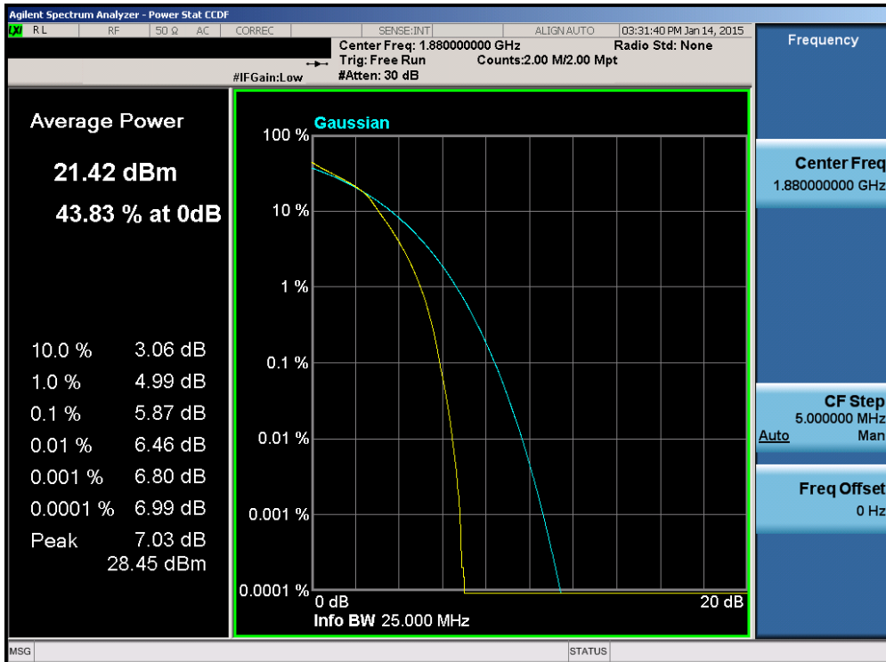
Plot 6-100. PAR Plot (Band 2 – 15.0MHz 16-QAM – RB Size 75)
