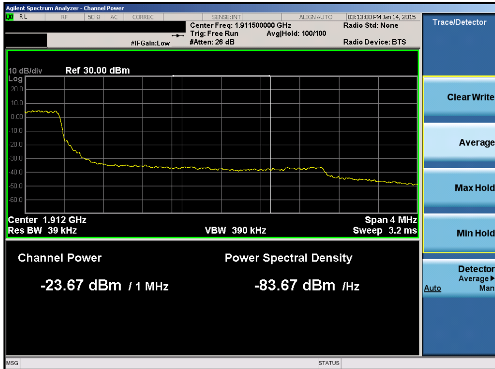
Plot 6-74. Upper Extended Band Edge Plot (Band 2 – 3.0MHz QPSK – RB Size 15)
