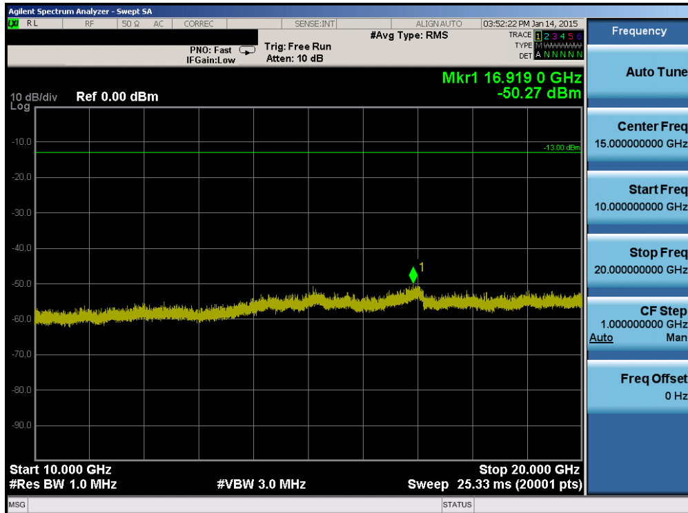
Plot 6-42. Conducted Spurious Plot (Band 2 – 20.0MHz QPSK – RB Size 1, RB Offset 0 – Mid Channel)
