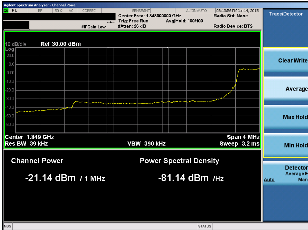
Plot 6-72. Lower Extended Band Edge Plot (Band 2 – 3.0MHz QPSK – RB Size 15)
