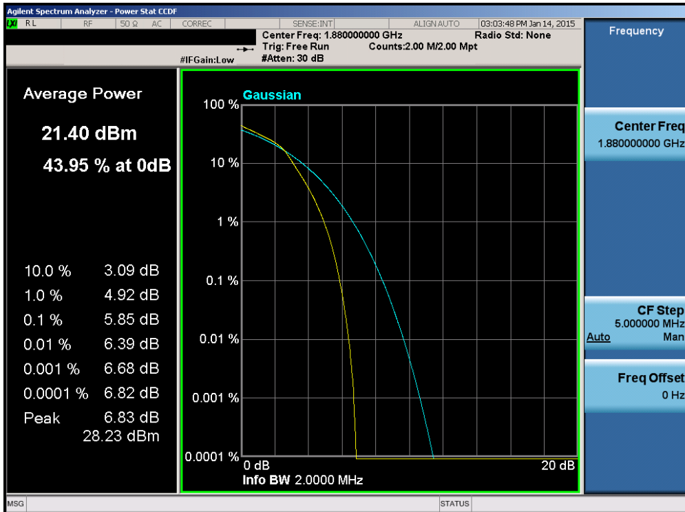
Plot 6-92. PAR Plot (Band 2 – 1.4MHz 16-QAM – RB Size 6)
