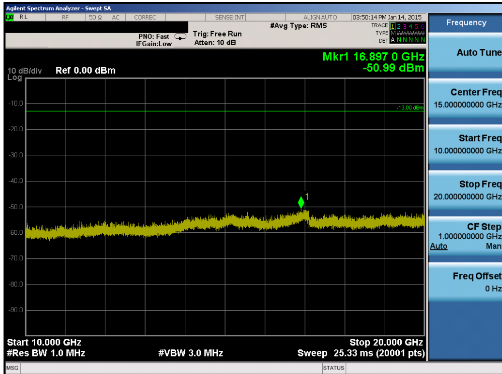
Plot 6-40. Conducted Spurious Plot (Band 2 – 20.0MHz QPSK – RB Size 1, RB Offset 0 – Low Channel)
