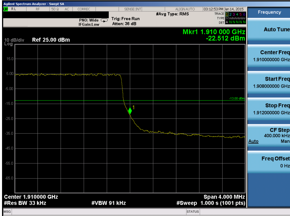
Plot 6-73. Upper Band Edge Plot (Band 2 – 3.0MHz QPSK – RB Size 15)
