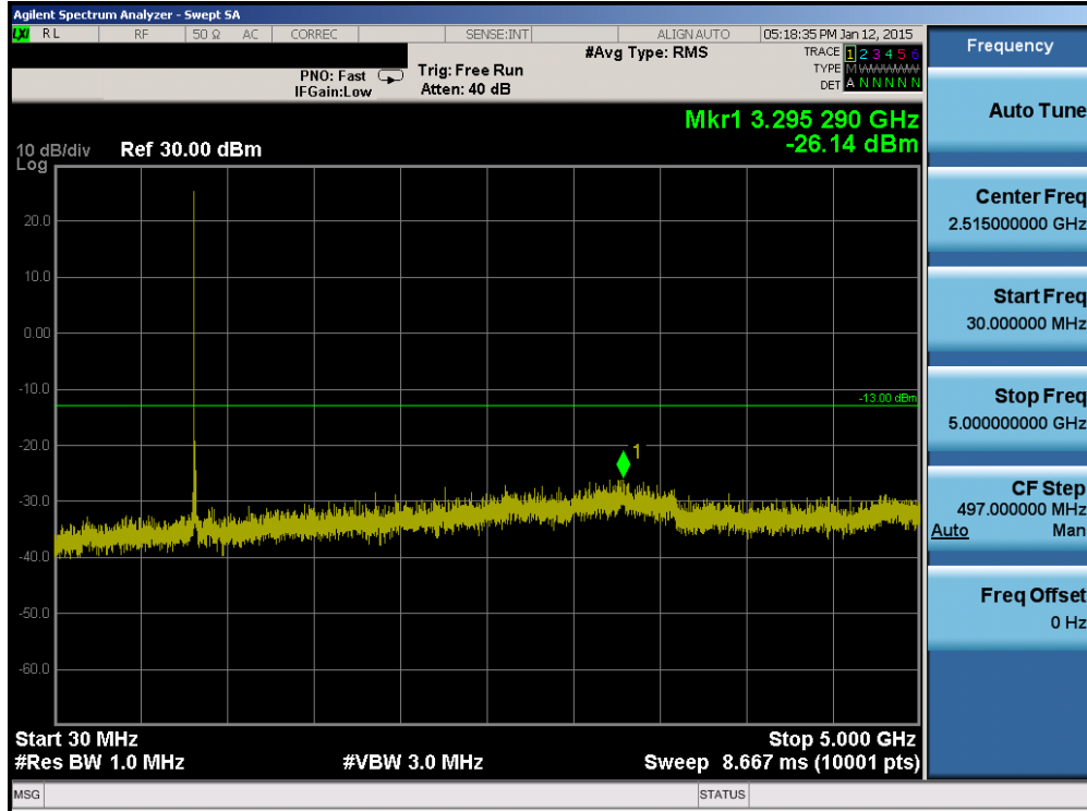
Plot 6-35. Conducted Spurious Plot (Band 26 – 3.0MHz QPSK – RB Size 1, RB Offset 0 – Mid Channel)
