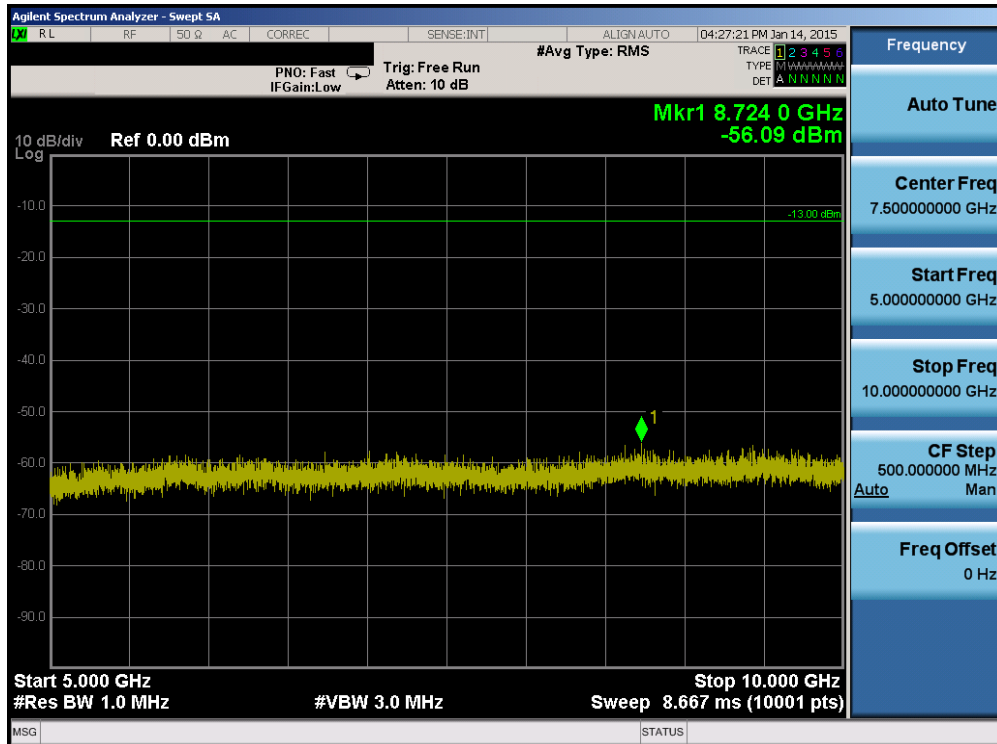
Plot 6-28. Conducted Spurious Plot (Band 17 – 5.0MHz QPSK – RB Size 1, RB Offset 0 – Low Channel)
