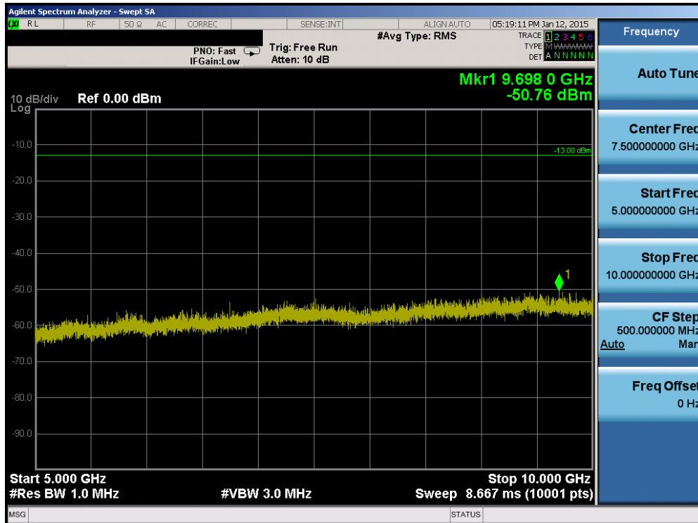
Plot 6-38. Conducted Spurious Plot (Band 26 – 3.0MHz QPSK – RB Size 1, RB Offset 0 – High Channel)
