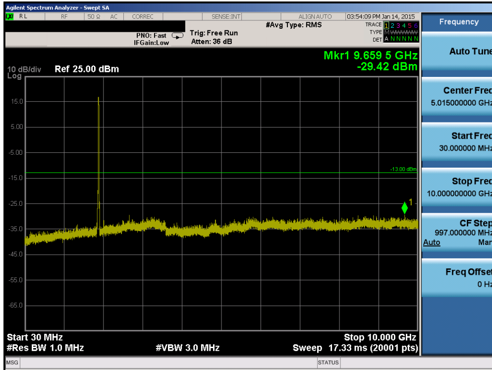
Plot 6-43. Conducted Spurious Plot (Band 2 – 20.0MHz QPSK – RB Size 1, RB Offset 0 – High Channel)
