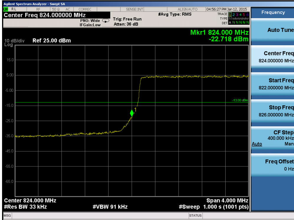
Plot 6-55. Lower Band Edge Plot (Band 26 – 3.0MHz QPSK – RB Size 15)
