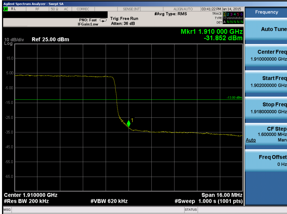
Plot 6-89. Upper Band Edge Plot (Band 2 – 20.0MHz QPSK – RB Size 100)
