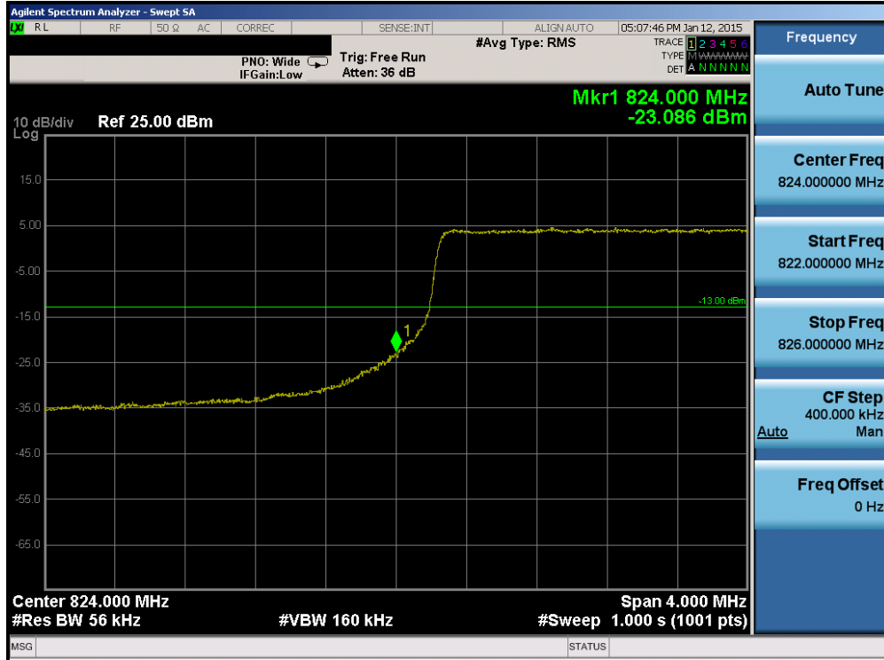
Plot 6-59. Lower Band Edge Plot (Band 26 – 5.0MHz QPSK – RB Size 25)
