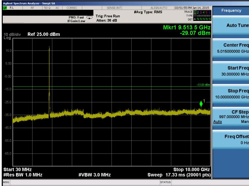
Plot 6-41. Conducted Spurious Plot (Band 2 – 20.0MHz QPSK – RB Size 1, RB Offset 0 – Mid Channel)
