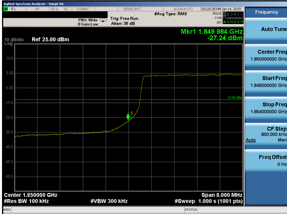
Plot 6-79. Lower Band Edge Plot (Band 2 – 10.0MHz QPSK – RB Size 50)
