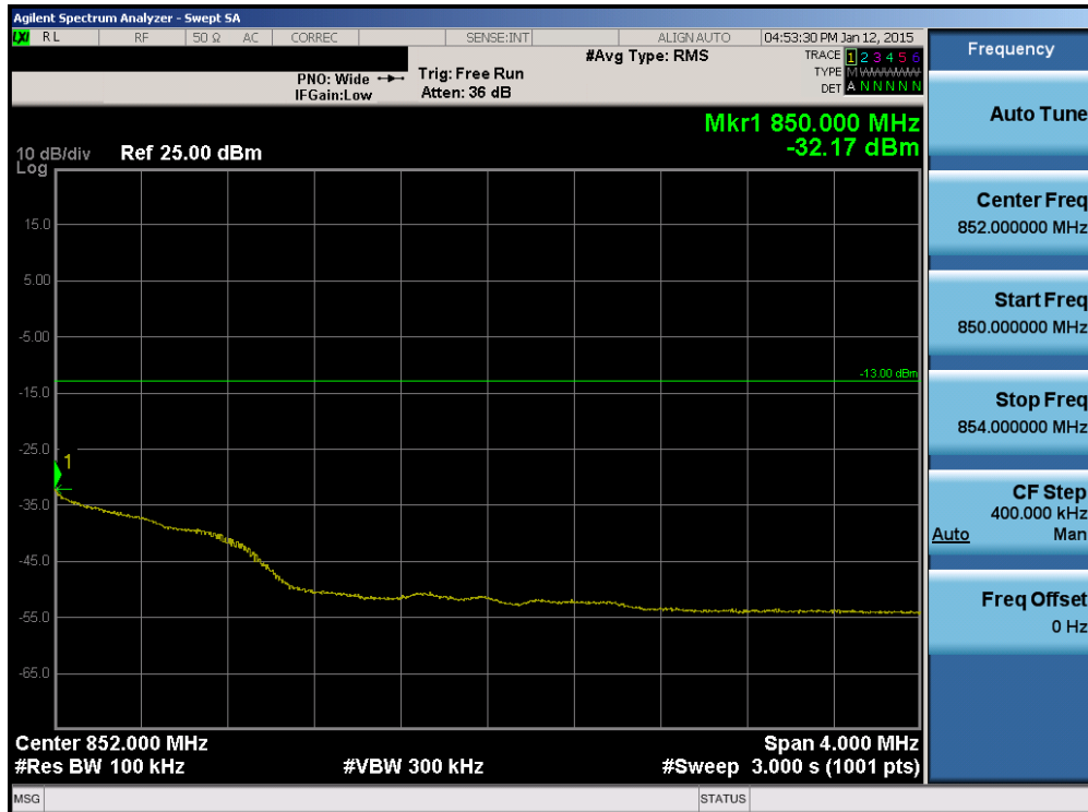
Plot 6-54. Upper Extended Band Edge Plot (Band 26 – 1.4MHz QPSK – RB Size 6)
