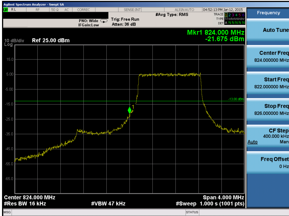
Plot 6-51. Lower Band Edge Plot (Band 26 – 1.4MHz QPSK – RB Size 6)
