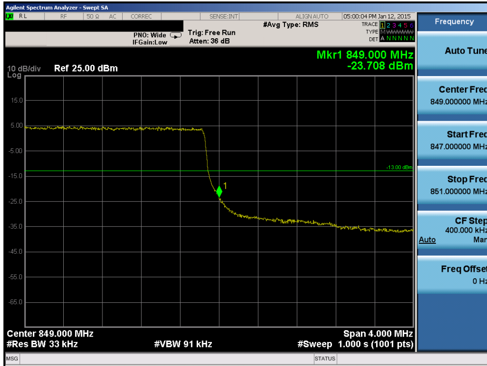
Plot 6-57. Upper Band Edge Plot (Band 26 – 3.0MHz QPSK – RB Size 15)
