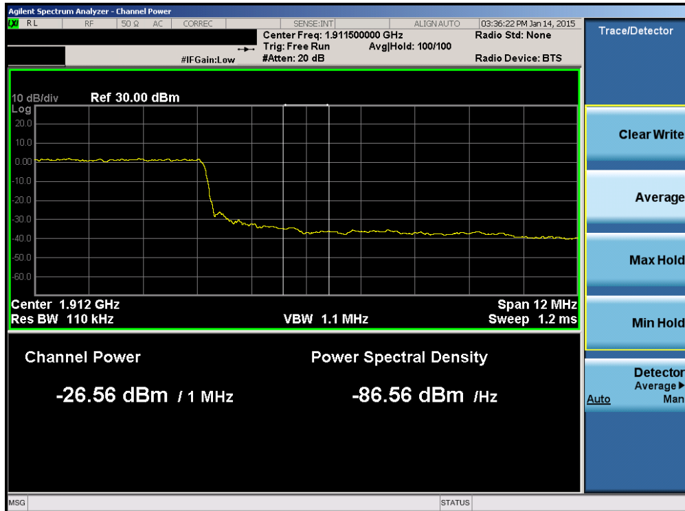
Plot 6-86. Upper Extended Band Edge Plot (Band 2 – 15.0MHz QPSK – RB Size 75)
