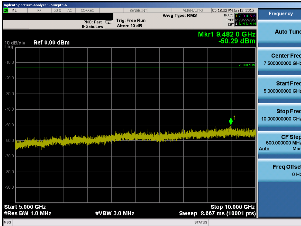
Plot 6-34. Conducted Spurious Plot (Band 26 – 3.0MHz QPSK – RB Size 1, RB Offset 0 – Low Channel)
