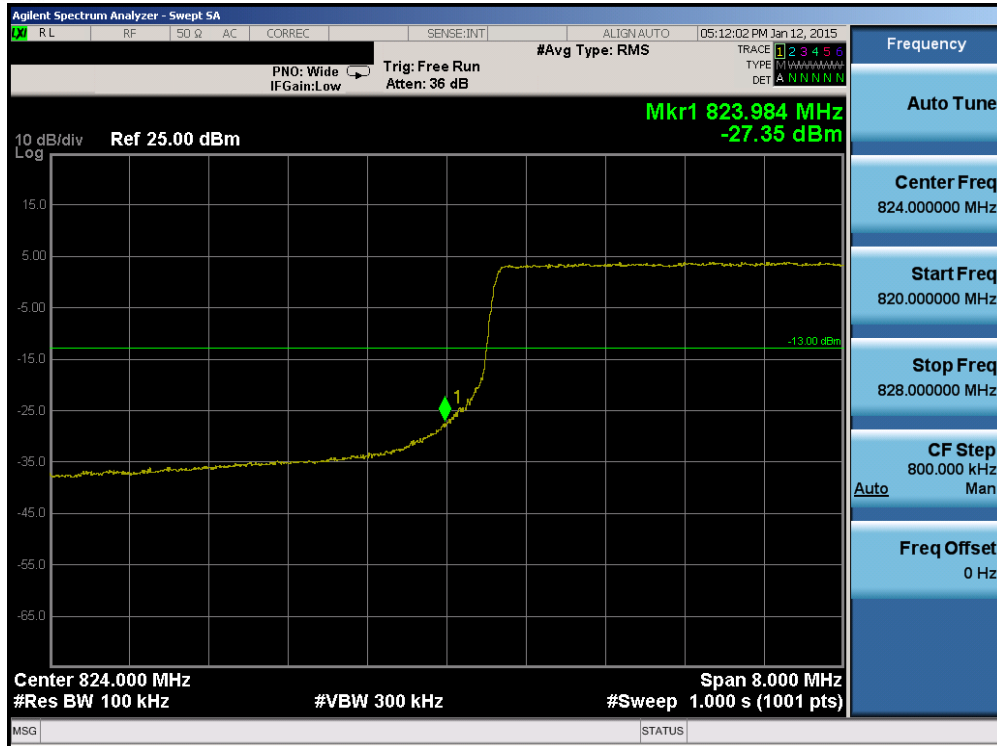
Plot 6-63. Lower Band Edge Plot (Band 26 – 10.0MHz QPSK – RB Size 50)
