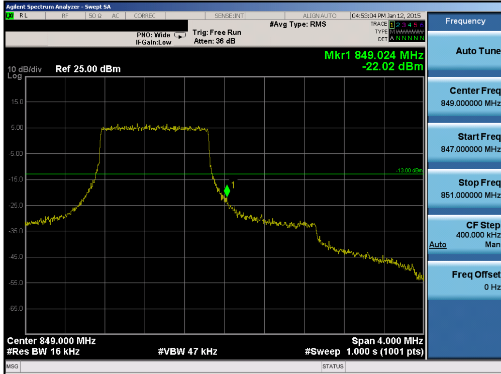
Plot 6-53. Upper Band Edge Plot (Band 26 – 1.4MHz QPSK – RB Size 6)
