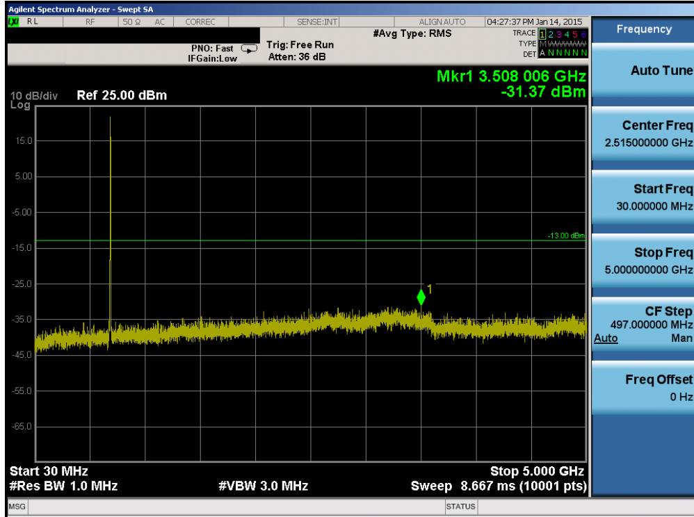
Plot 6-29. Conducted Spurious Plot (Band 17 – 5.0MHz QPSK – RB Size 1, RB Offset 0 – Mid Channel)
