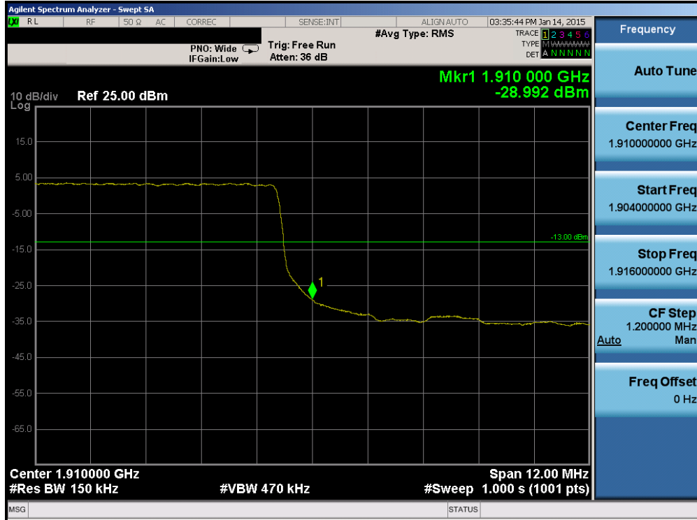
Plot 6-85. Upper Band Edge Plot (Band 2 – 15.0MHz QPSK – RB Size 75)
