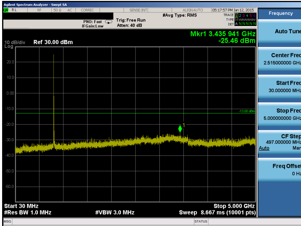
Plot 6-33. Conducted Spurious Plot (Band 26 – 3.0MHz QPSK – RB Size 1, RB Offset 0 – Low Channel)
