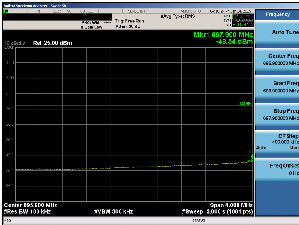
Plot 6-46. Lower Extended Band Edge Plot (Band 17 – 5.0MHz QPSK – RB Size 25)
