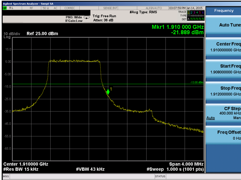
Plot 6-69. Upper Band Edge Plot (Band 2 – 1.4MHz QPSK – RB Size 6)
