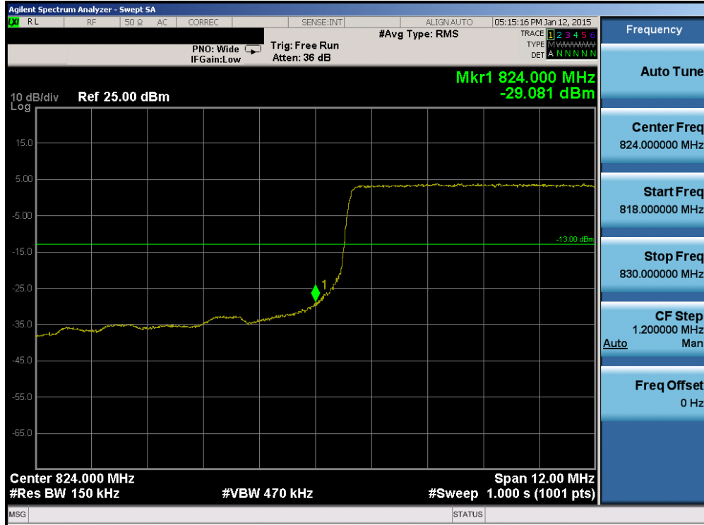
Plot 6-65. Lower Band Edge Plot (Band 26 – 15.0MHz QPSK – RB Size 75)
