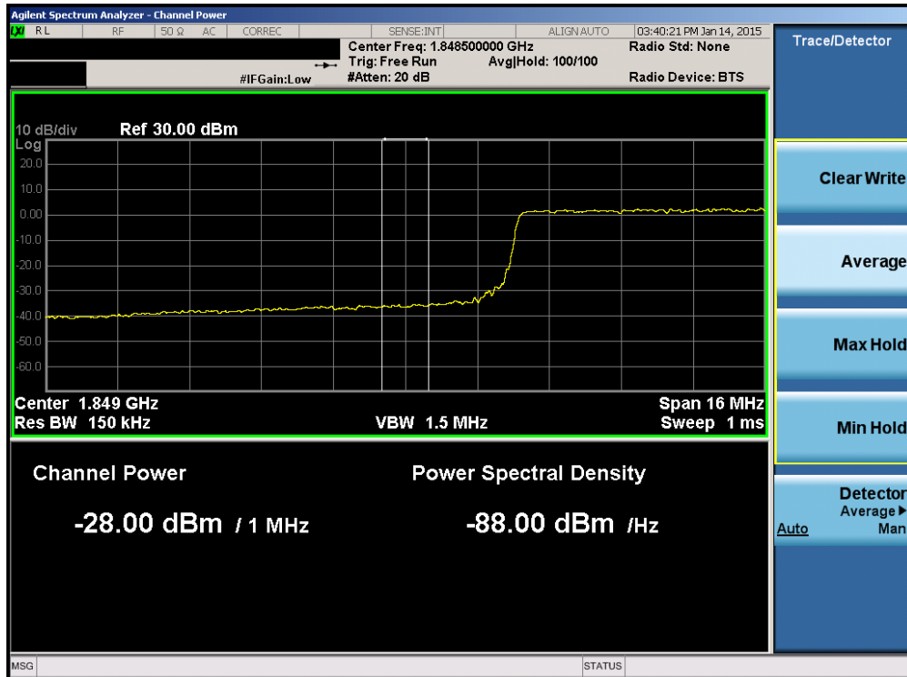
Plot 6-88. Lower Extended Band Edge Plot (Band 2 – 20.0MHz QPSK – RB Size 100)
