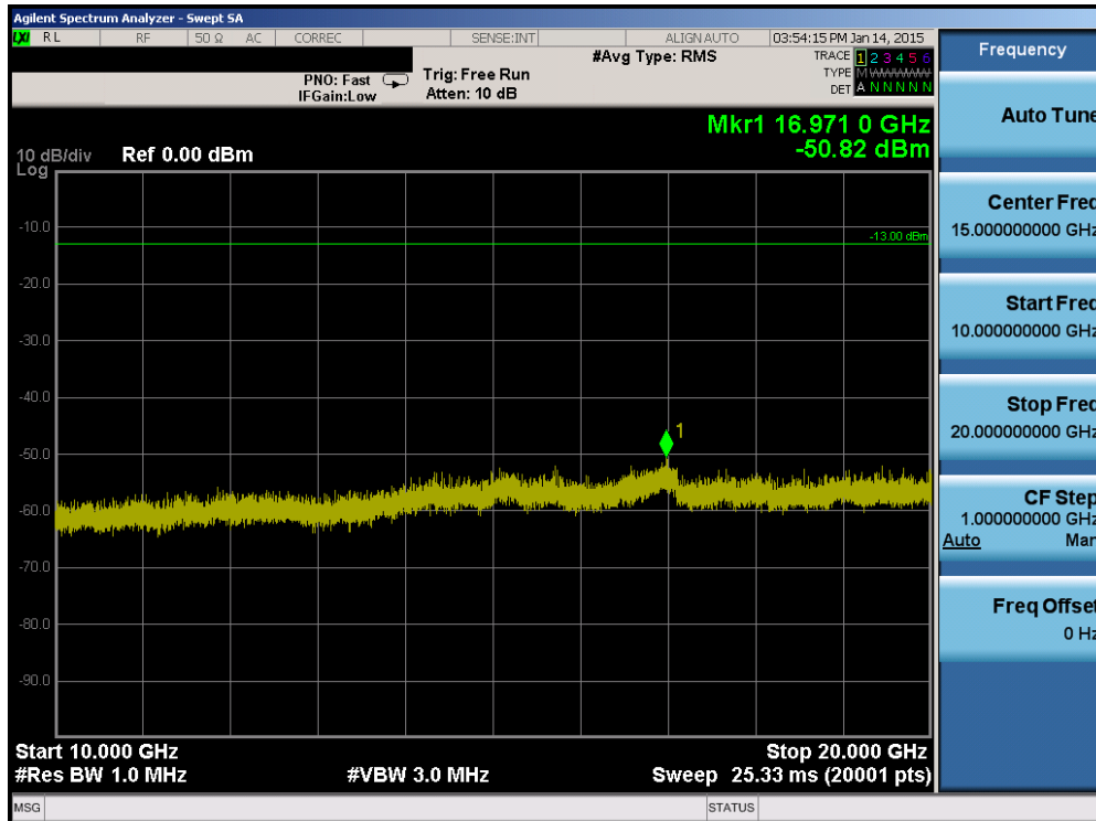
Plot 6-44. Conducted Spurious Plot (Band 2 – 20.0MHz QPSK – RB Size 1, RB Offset 0 – High Channel)
