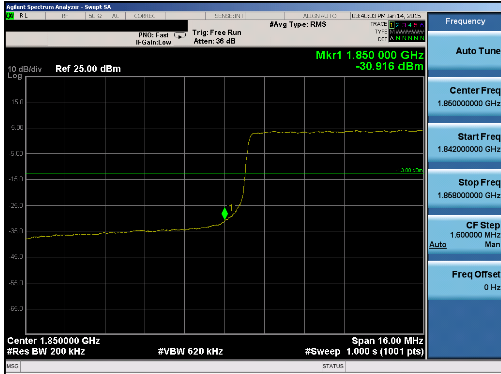
Plot 6-87. Lower Band Edge Plot (Band 2 – 20.0MHz QPSK – RB Size 100)
