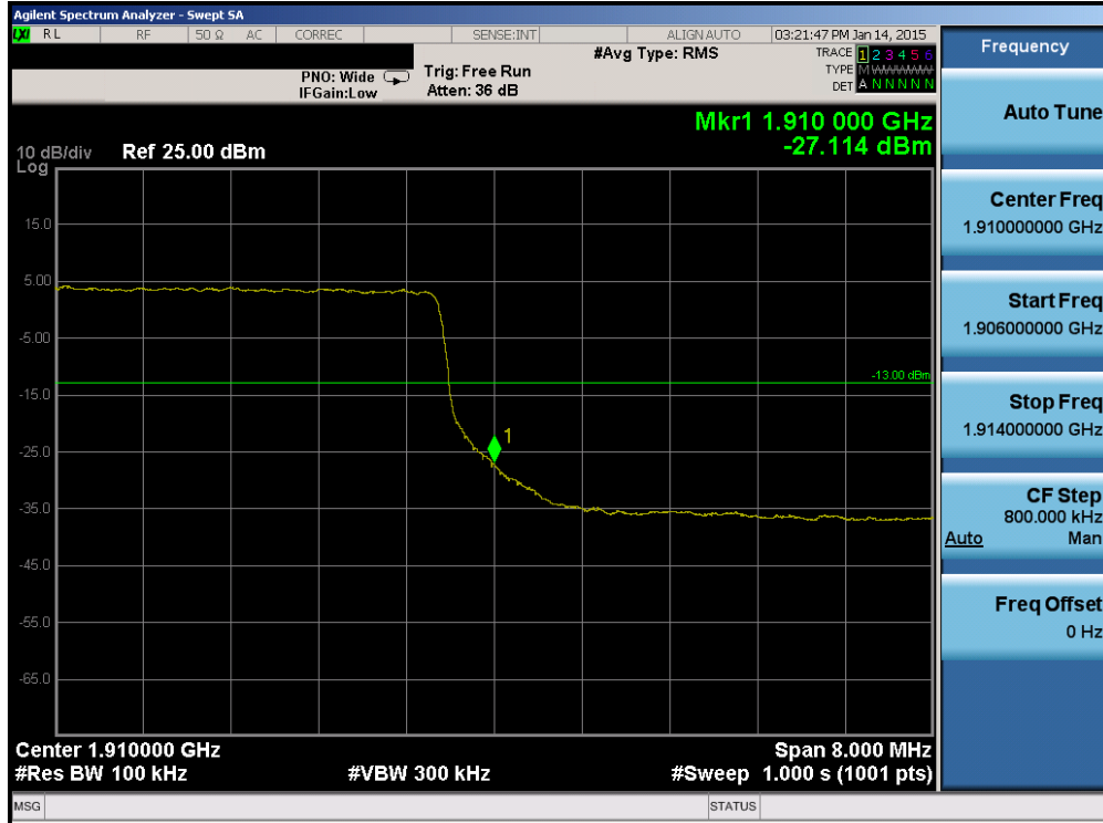
Plot 6-81. Upper Band Edge Plot (Band 2 – 10.0MHz QPSK – RB Size 50)
