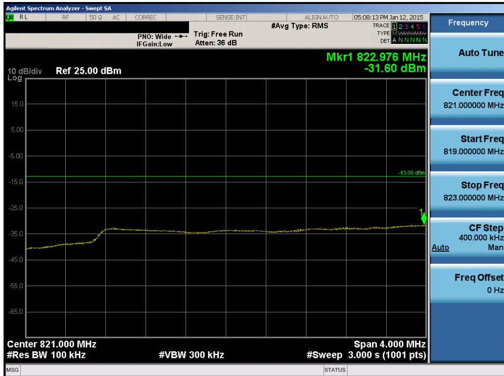
Plot 6-60. Lower Extended Band Edge Plot (Band 26 – 5.0MHz QPSK – RB Size 25)
