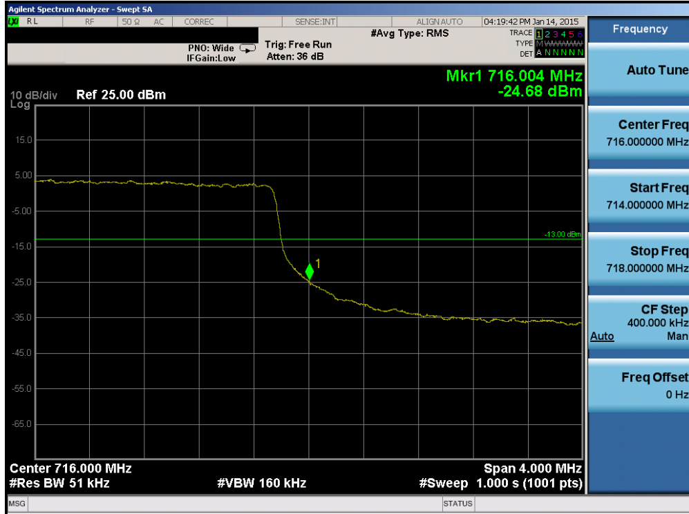
Plot 6-47. Upper Band Edge Plot (Band 17 – 5.0MHz QPSK – RB Size 25)
