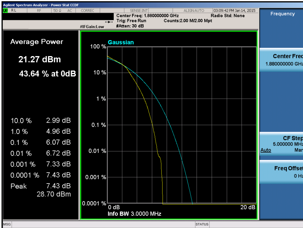
Plot 6-94. PAR Plot (Band 2 – 3.0MHz 16-QAM – RB Size 15)
