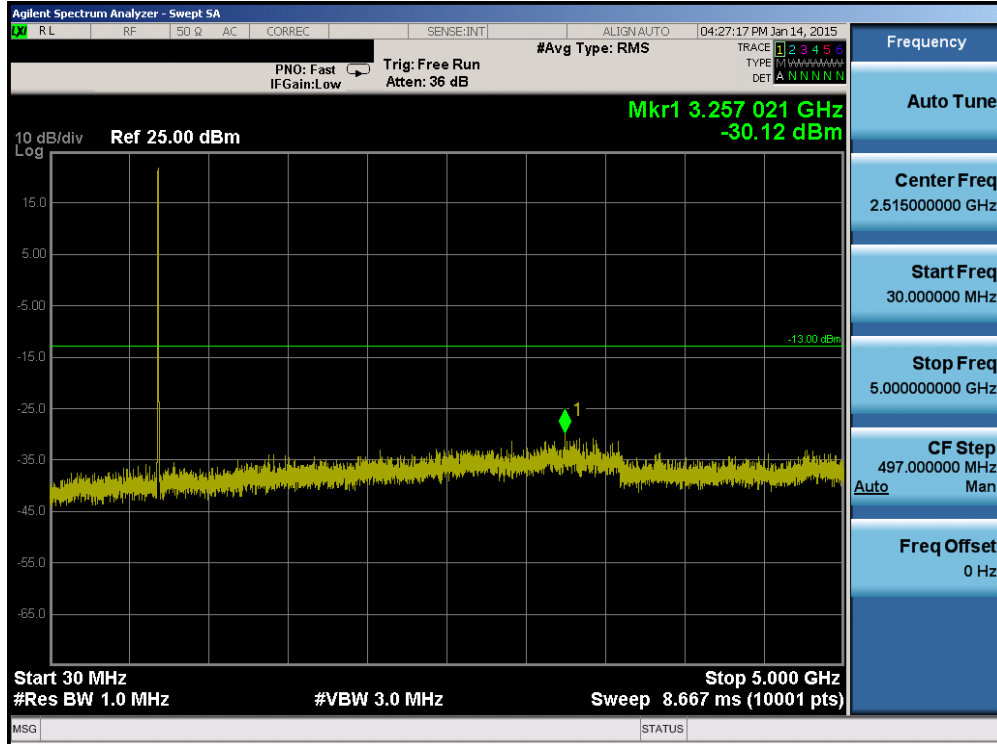
Plot 6-27. Conducted Spurious Plot (Band 17 – 5.0MHz QPSK – RB Size 1, RB Offset 0 – Low Channel)
