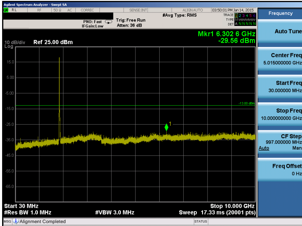
Plot 6-39. Conducted Spurious Plot (Band 2 – 20.0MHz QPSK – RB Size 1, RB Offset 0– Low Channel)
