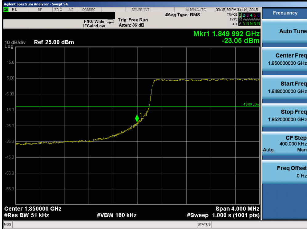
Plot 6-75. Lower Band Edge Plot (Band 2 – 5.0MHz QPSK – RB Size 25)
