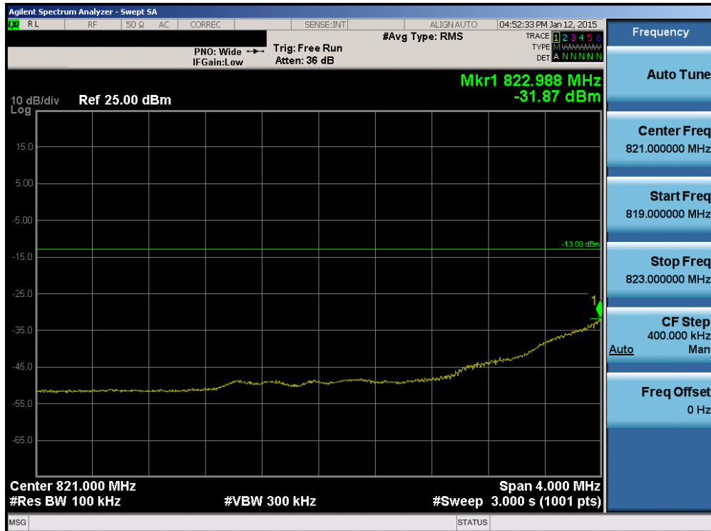
Plot 6-52. Lower Extended Band Edge Plot (Band 26 – 1.4MHz QPSK – RB Size 6)
