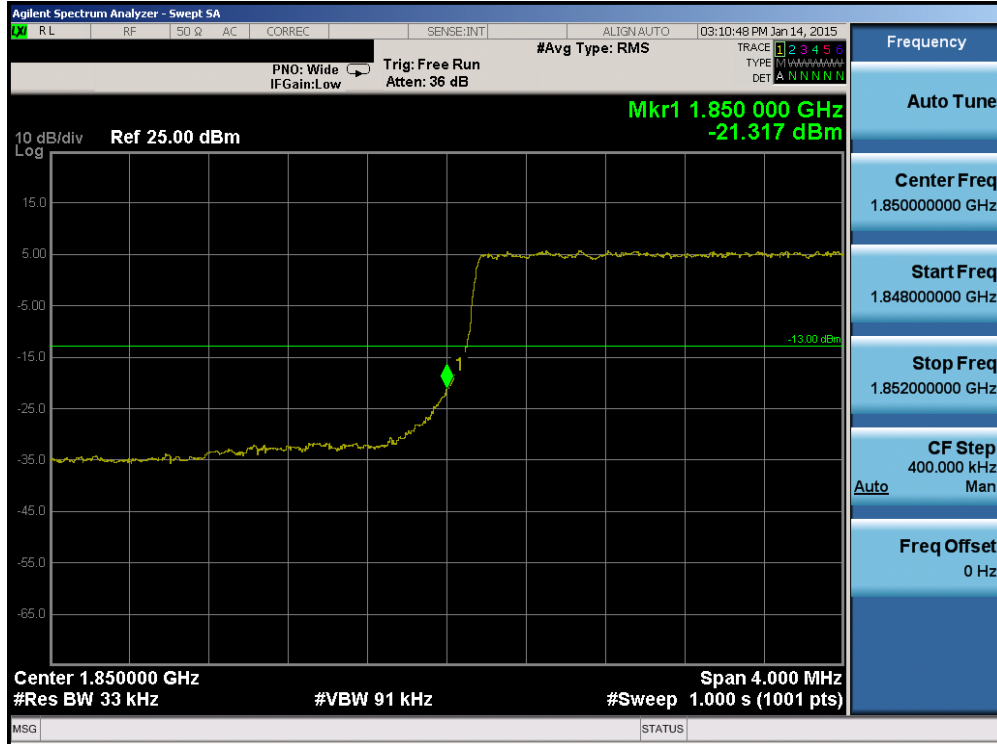
Plot 6-71. Lower Band Edge Plot (Band 2 – 3.0MHz QPSK – RB Size 15)
