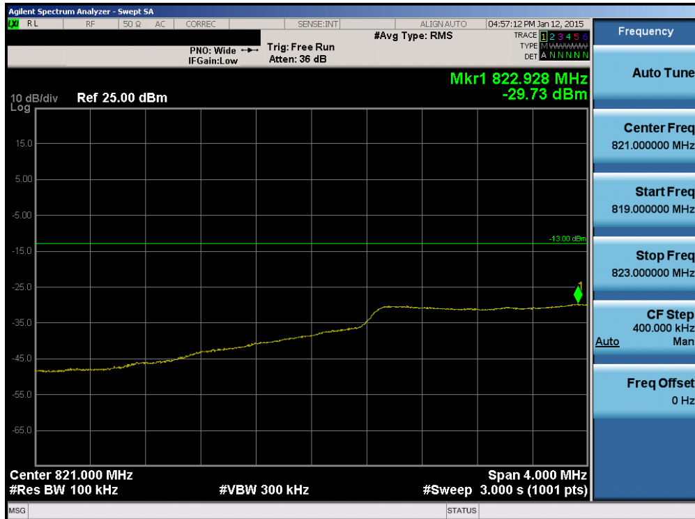
Plot 6-56. Lower Extended Band Edge Plot (Band 26 – 3.0MHz QPSK – RB Size 15)
