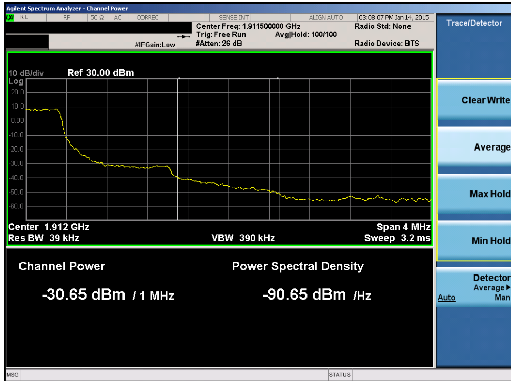
Plot 6-70. Upper Extended Band Edge Plot (Band 2 – 1.4MHz QPSK – RB Size 6)
