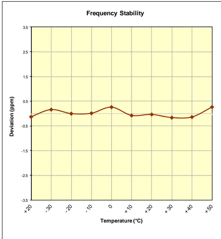
Figure 6-11. Frequency Stability Graph (Band 26)
