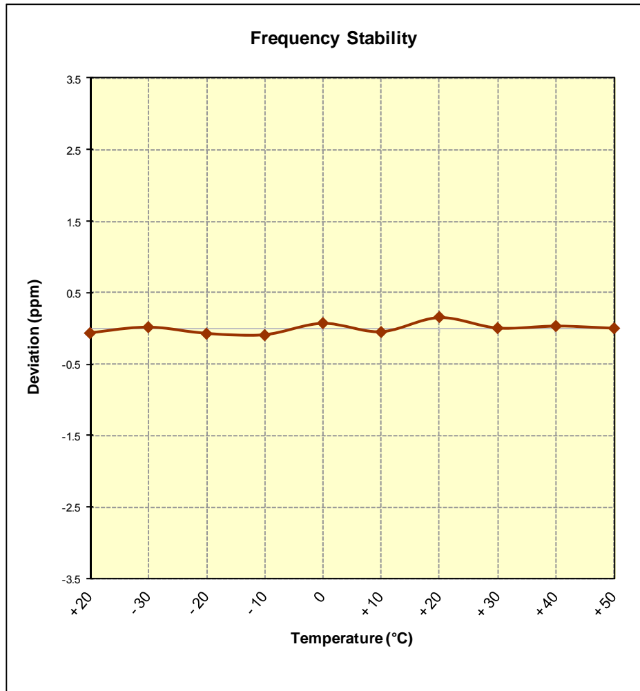
Figure 6-12. Frequency Stability Graph (Band 2)
