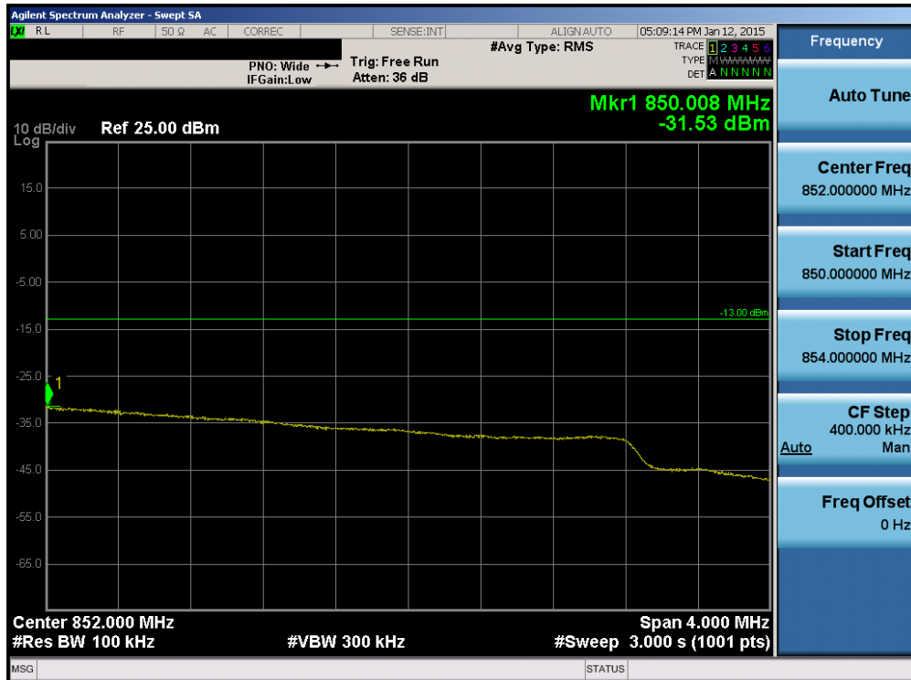
Plot 6-62. Upper Extended Band Edge Plot (Band 26 – 5.0MHz QPSK – RB Size 25)
