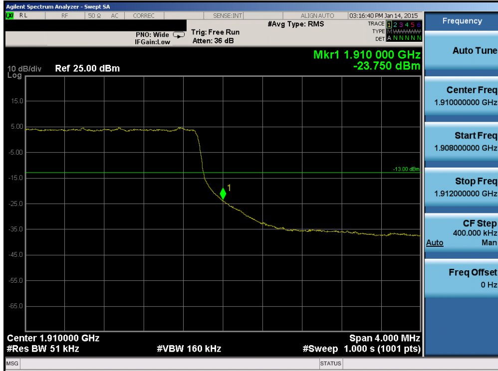
Plot 6-77. Upper Band Edge Plot (Band 2 – 5.0MHz QPSK – RB Size 25)
