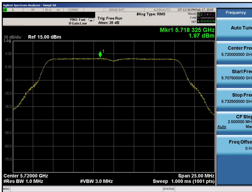
Plot 6-135. Power Spectral Density Plot (802.11a (UNII Band 2C) – Ch. 144)
