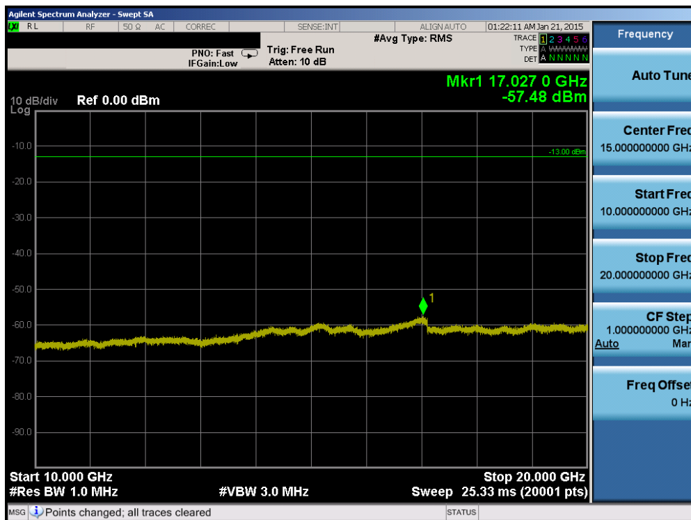
Plot 6-56. Conducted Spurious Plot (Band 4 – 5.0MHz QPSK – RB Size 1, RB Offset 0 – Mid Channel)
