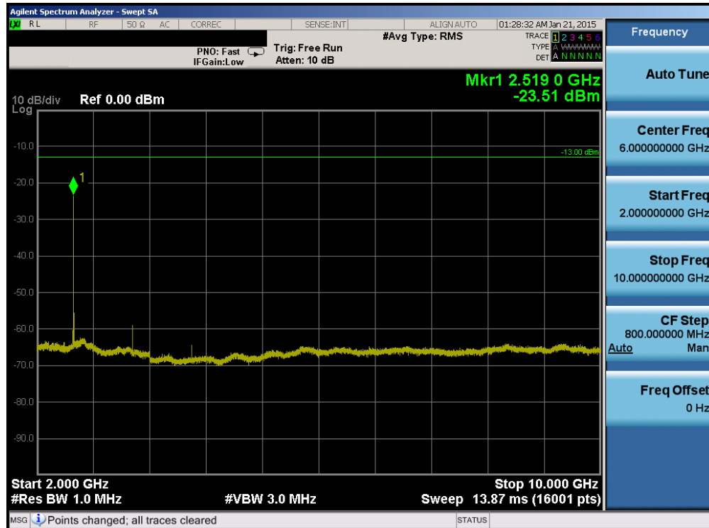
Plot 6-50. Conducted Spurious Plot (Band 5 – 5.0MHz QPSK – RB Size 1, RB Offset 0 – High Channel)
