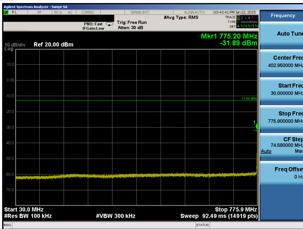
Plot 6-33. Conducted Spurious Plot (Band 13 – 5.0MHz QPSK – RB Size 1, RB Offset 0 – Low Channel)
