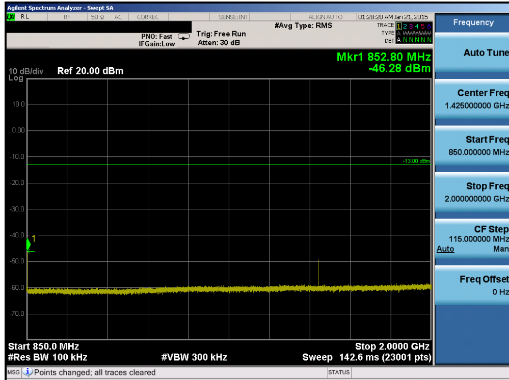
Plot 6-49. Conducted Spurious Plot (Band 5 – 5.0MHz QPSK – RB Size 1, RB Offset 0 – High Channel)
