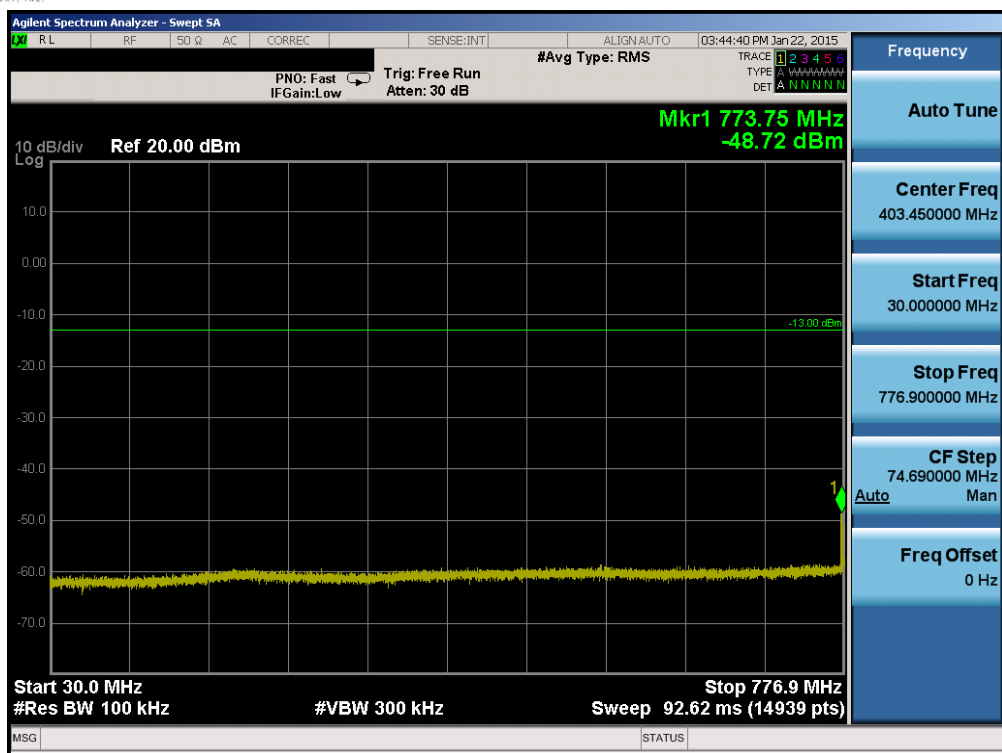
Plot 6-39. Conducted Spurious Plot (Band 13 – 5.0MHz QPSK – RB Size 1, RB Offset 0 – High Channel)
