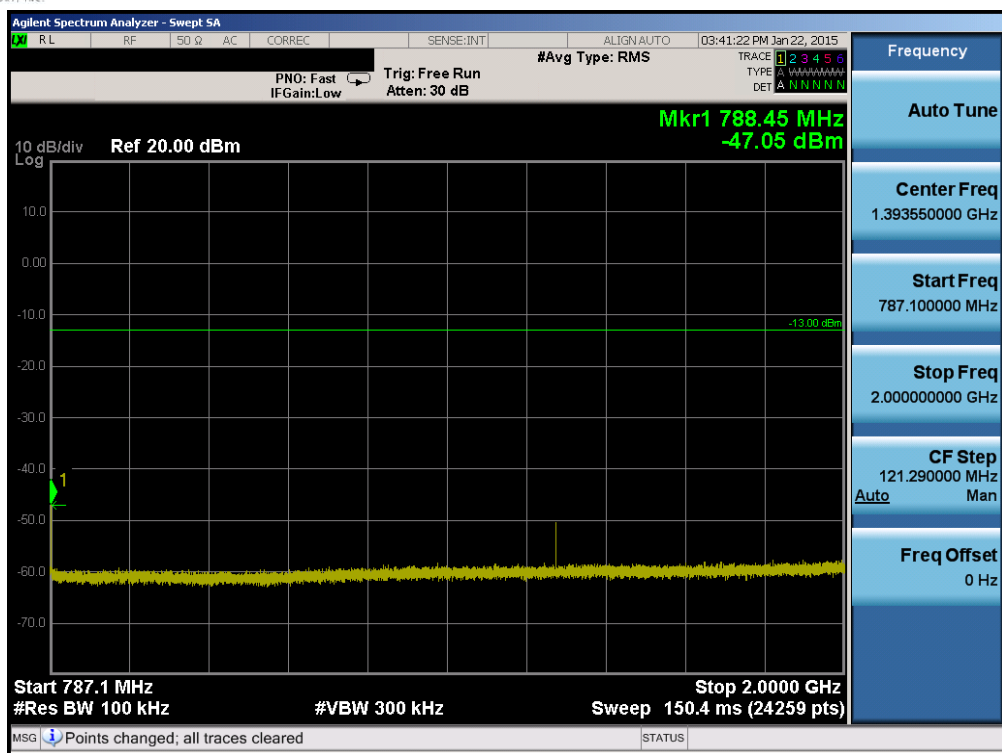
Plot 6-37. Conducted Spurious Plot (Band 13 – 5.0MHz QPSK – RB Size 1, RB Offset 0 – Mid Channel)
