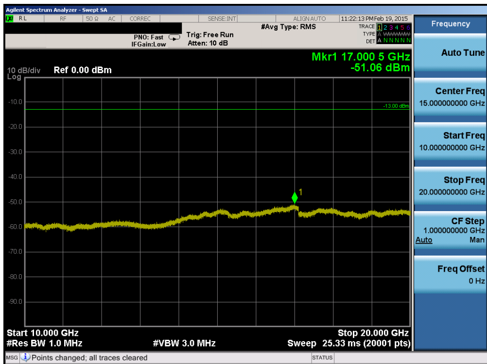
Plot 6-68. Conducted Spurious Plot (Band 2 – 10.0MHz QPSK – RB Size 1, RB Offset 0 – High Channel)
