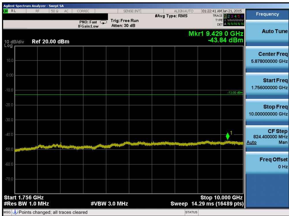
Plot 6-52. Conducted Spurious Plot (Band 4 – 5.0MHz QPSK – RB Size 1, RB Offset 0 – Low Channel)
