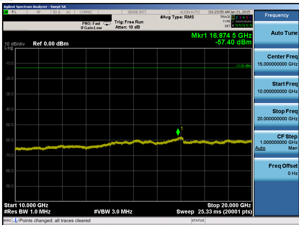
Plot 6-59. Conducted Spurious Plot (Band 4 – 5.0MHz QPSK – RB Size 1, RB Offset 0 – High Channel)
