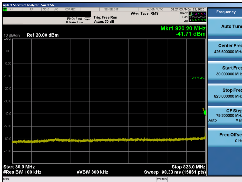
Plot 6-42. Conducted Spurious Plot (Band 5 – 5.0MHz QPSK – RB Size 1, RB Offset 0 – Low Channel)
