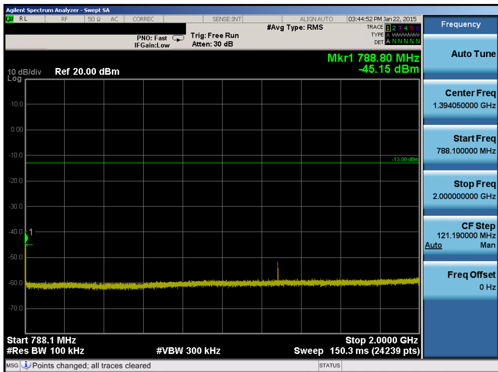
Plot 6-40. Conducted Spurious Plot (Band 13 – 5.0MHz QPSK – RB Size 1, RB Offset 0 – High Channel)
