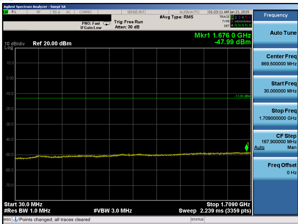
Plot 6-57. Conducted Spurious Plot (Band 4 – 5.0MHz QPSK – RB Size 1, RB Offset 0 – High Channel)
