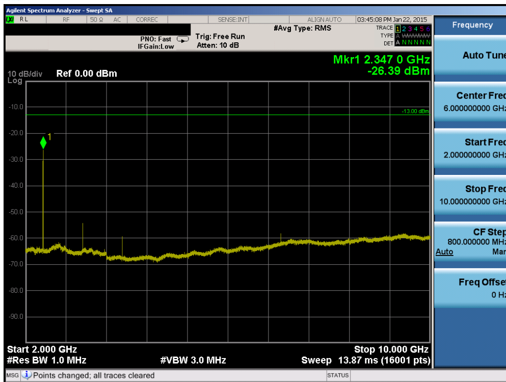
Plot 6-41. Conducted Spurious Plot (Band 13 – 5.0MHz QPSK – RB Size 1, RB Offset 0 – High Channel)
