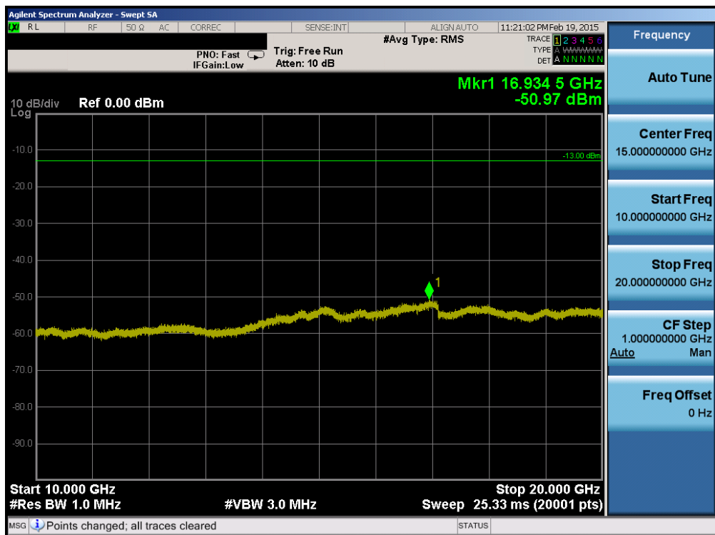
Plot 6-62. Conducted Spurious Plot (Band 2 – 10.0MHz QPSK – RB Size 1, RB Offset 0 – Low Channel)
