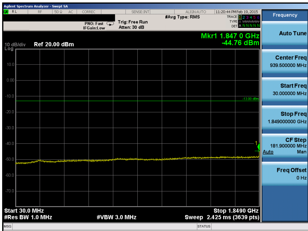
Plot 6-60. Conducted Spurious Plot (Band 2 – 10.0MHz QPSK – RB Size 1, RB Offset 0– Low Channel)
