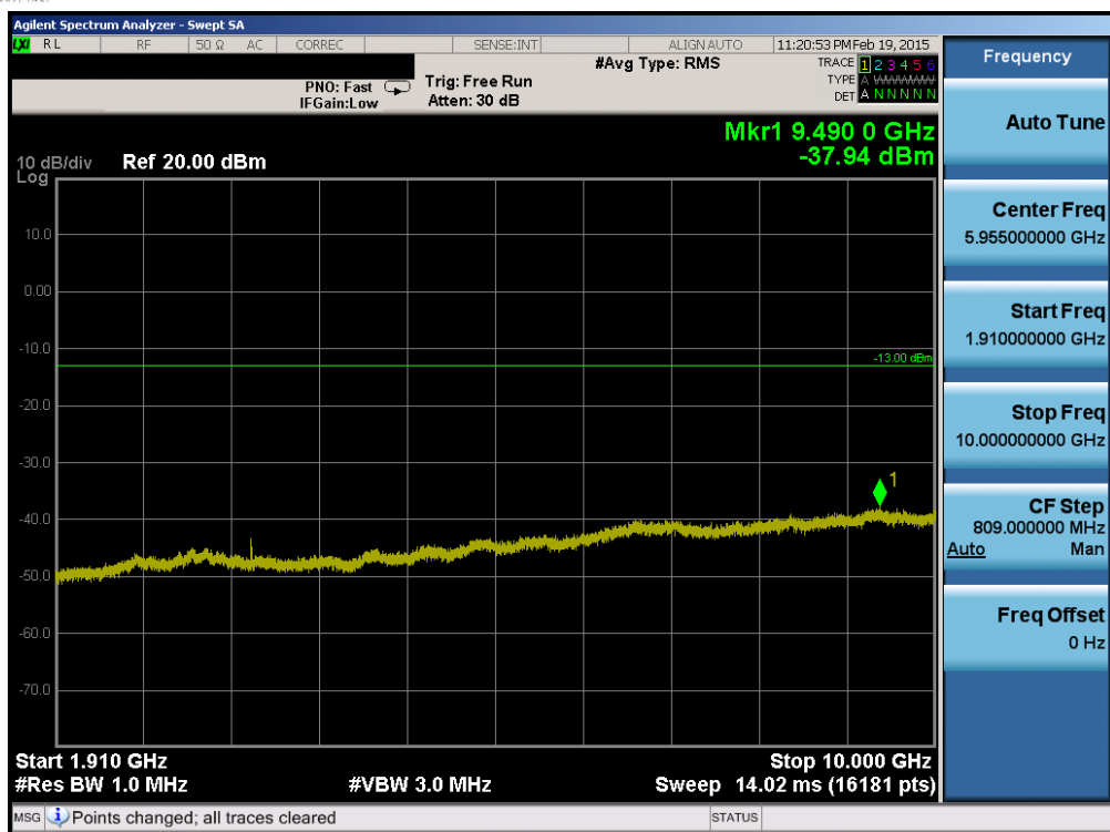
Plot 6-61. Conducted Spurious Plot (Band 2 – 10.0MHz QPSK – RB Size 1, RB Offset 0 – Low Channel)
