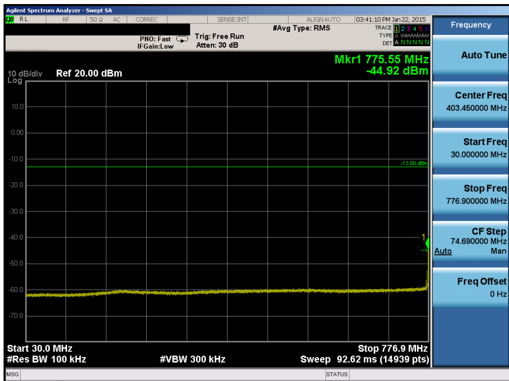
Plot 6-36. Conducted Spurious Plot (Band 13 – 5.0MHz QPSK – RB Size 1, RB Offset 0 – Mid Channel)
