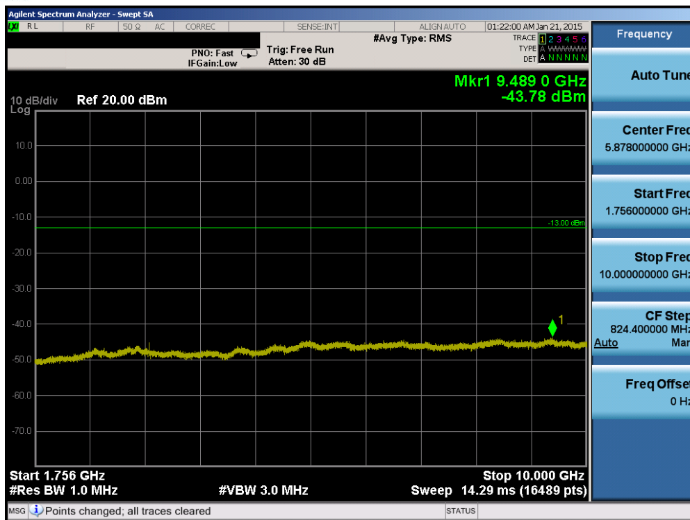
Plot 6-55. Conducted Spurious Plot (Band 4 – 5.0MHz QPSK – RB Size 1, RB Offset 0 – Mid Channel)
