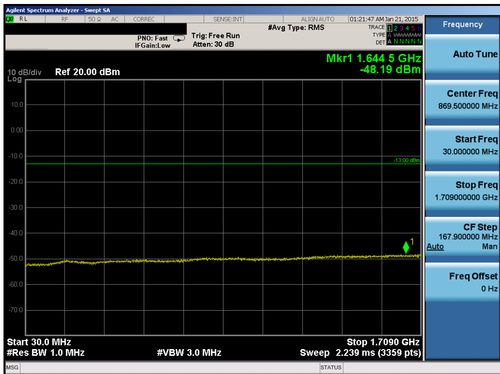
Plot 6-54. Conducted Spurious Plot (Band 4 – 5.0MHz QPSK – RB Size 1, RB Offset 0 – Mid Channel)
