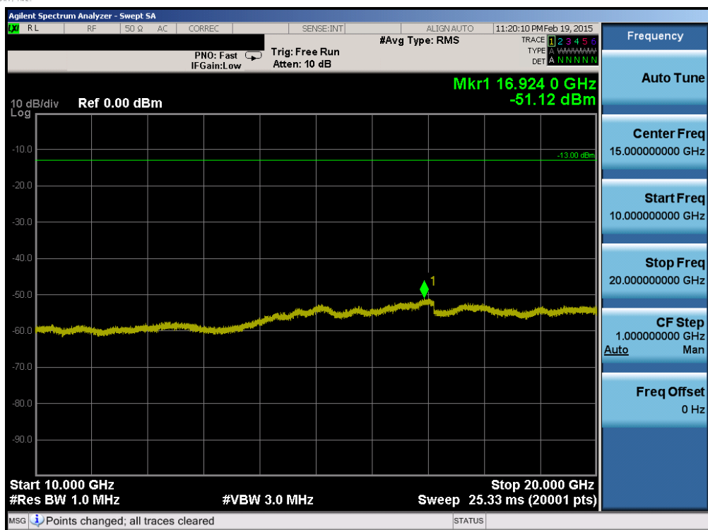
Plot 6-65. Conducted Spurious Plot (Band 2 – 10.0MHz QPSK – RB Size 1, RB Offset 0 – Mid Channel)
