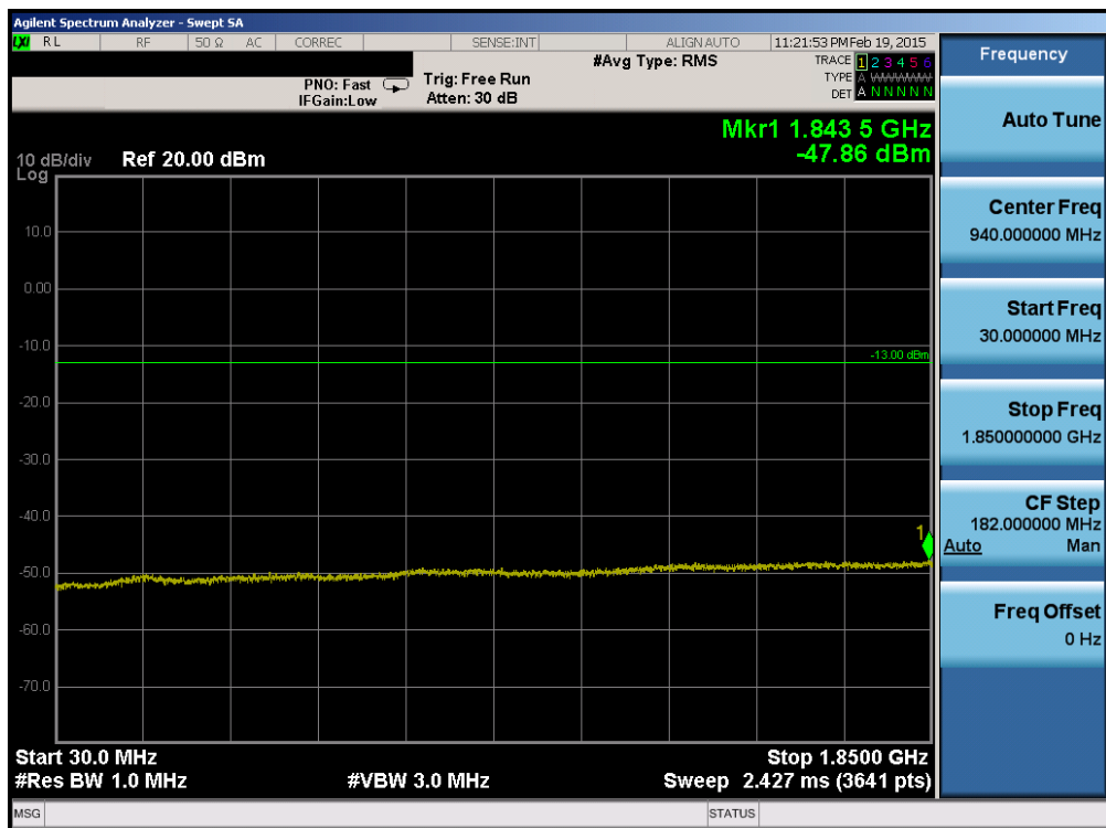
Plot 6-66. Conducted Spurious Plot (Band 2 – 10.0MHz QPSK – RB Size 1, RB Offset 0 – High Channel)
