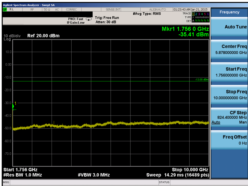
Plot 6-58. Conducted Spurious Plot (Band 4 – 5.0MHz QPSK – RB Size 1, RB Offset 0 – High Channel)
