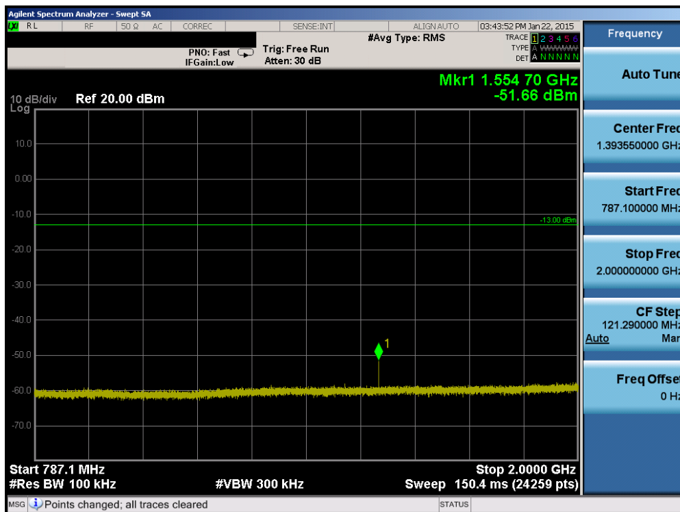
Plot 6-34. Conducted Spurious Plot (Band 13 – 5.0MHz QPSK – RB Size 1, RB Offset 0 – Low Channel)
