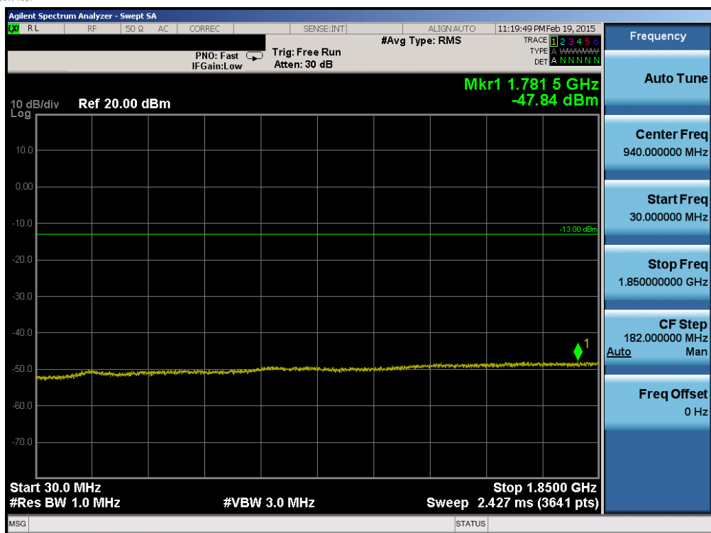
Plot 6-63. Conducted Spurious Plot (Band 2 – 10.0MHz QPSK – RB Size 1, RB Offset 0 – Mid Channel)
