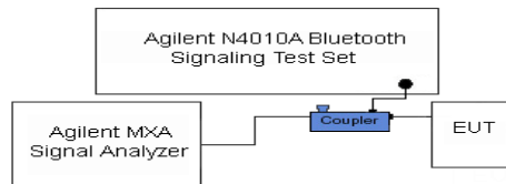
Figure 6-2. Test Instrument & Measurement Setup
