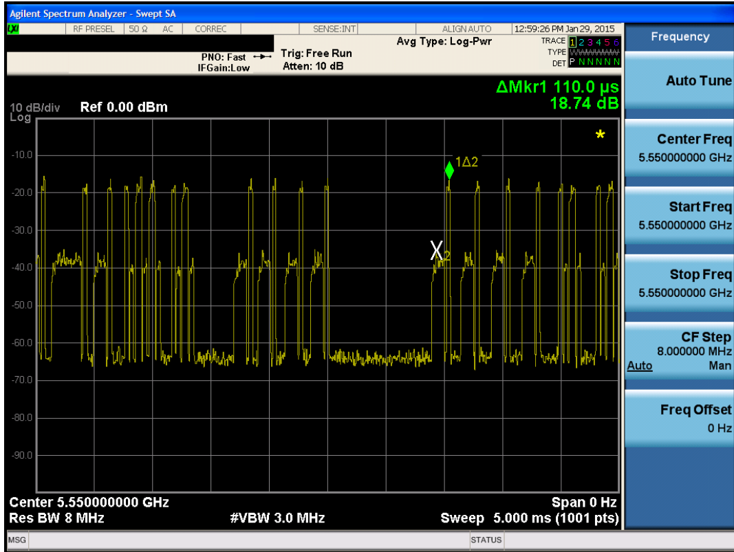
Figure 5-3. Band 2C Pulse Width
