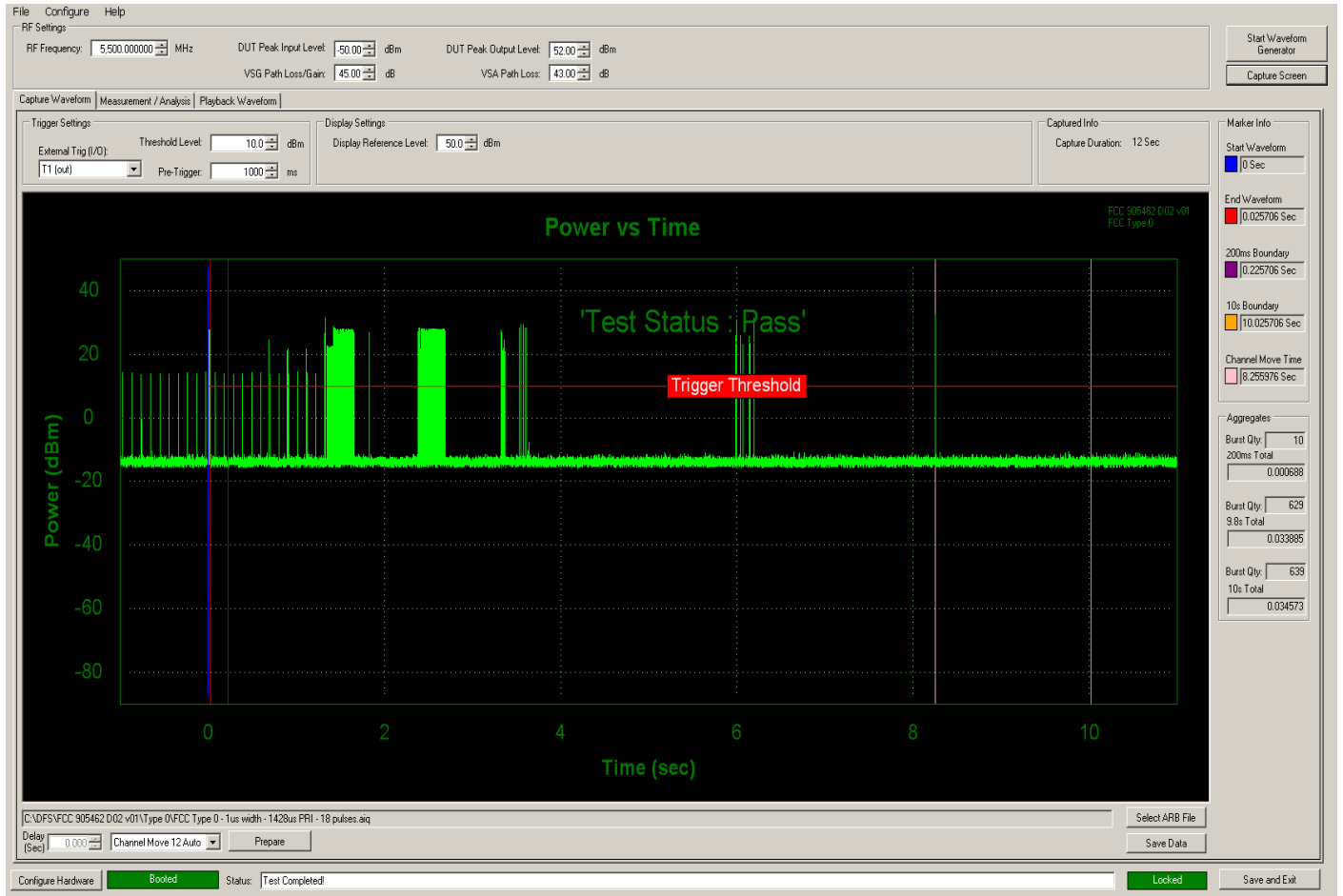
Figure 5-6. Band 2C Move Time and Aggregate Time
