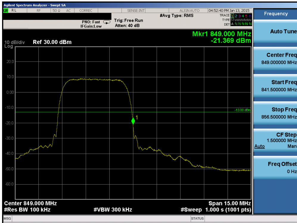
Plot 6-36. Band Edge Plot (Cellular WCDMA Mode – Ch. 4233)
