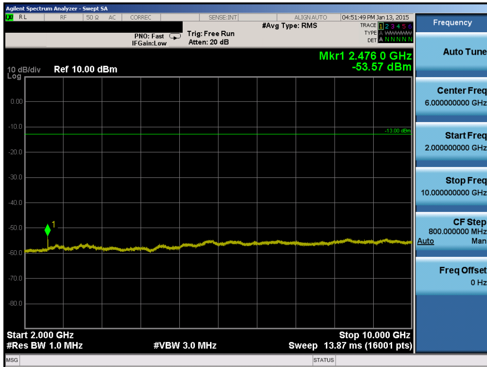
Plot 6-15. Conducted Spurious Plot (Cellular WCDMA Mode – Ch. 4132)
