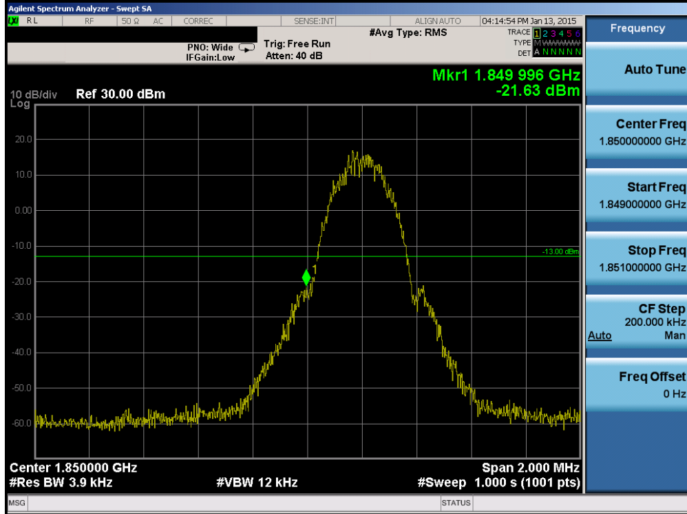
Plot 6-31. Band Edge Plot (PCS GSM Mode – Ch. 512)
