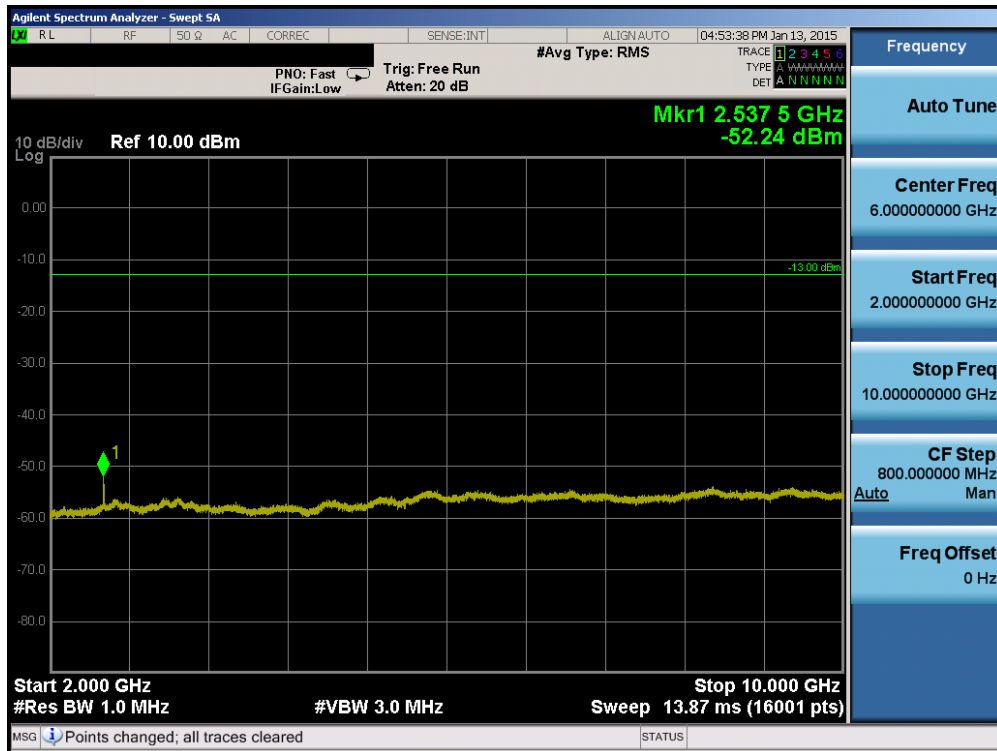
Plot 6-21. Conducted Spurious Plot (Cellular WCDMA Mode – Ch. 4233)
