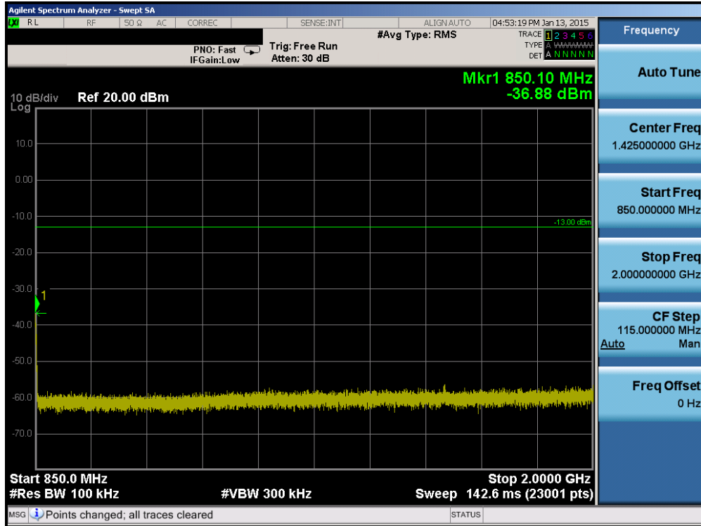
Plot 6-20. Conducted Spurious Plot (Cellular WCDMA Mode – Ch. 4233)
