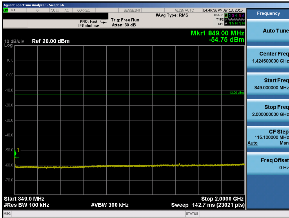
Plot 6-17. Conducted Spurious Plot (Cellular WCDMA Mode – Ch. 4183)
