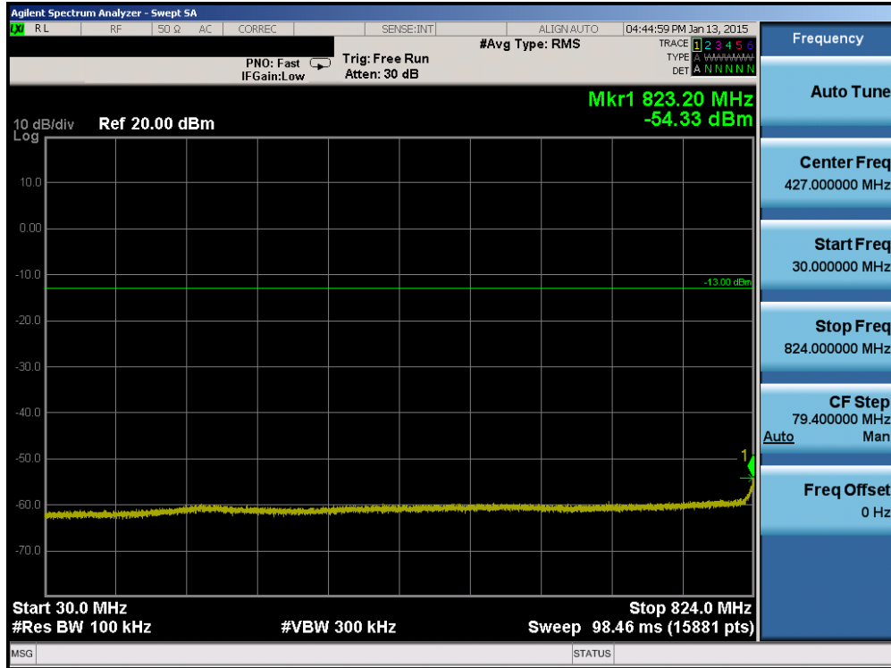
Plot 6-16. Conducted Spurious Plot (Cellular WCDMA Mode – Ch. 4183)
