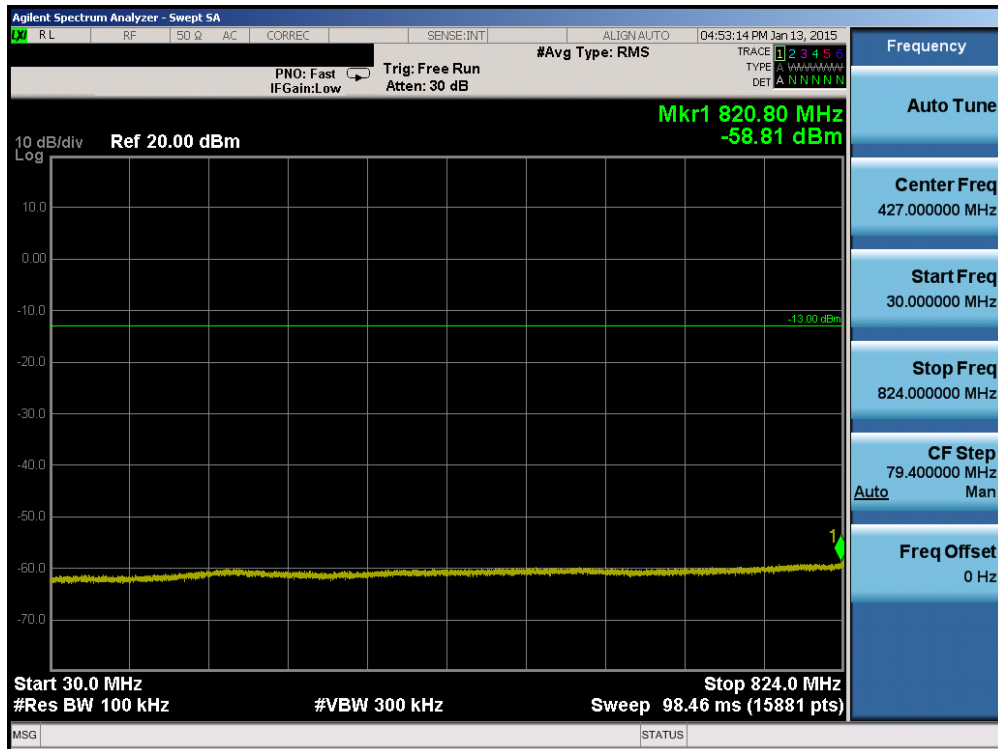
Plot 6-19. Conducted Spurious Plot (Cellular WCDMA Mode – Ch. 4233)
