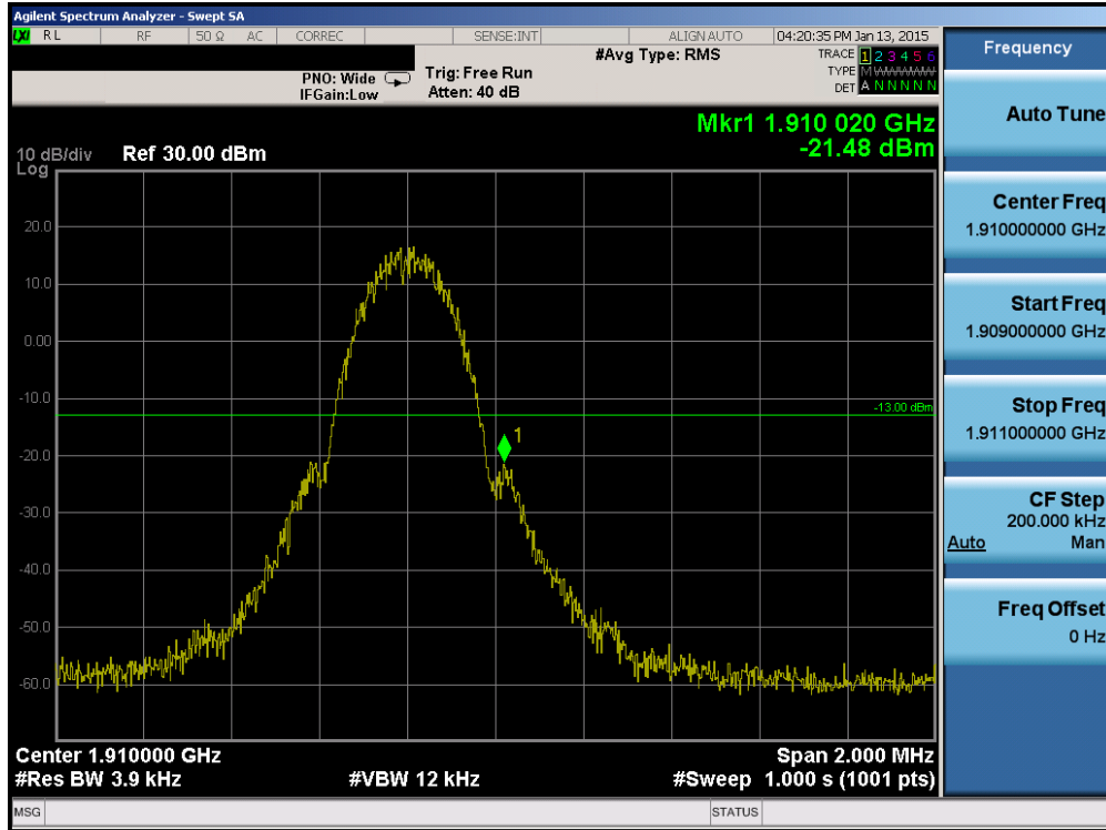
Plot 6-33. Band Edge Plot (PCS GSM Mode – Ch. 810)
