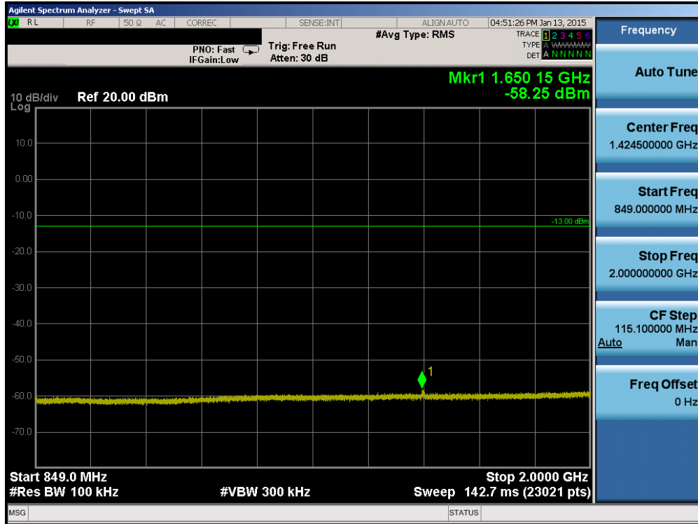
Plot 6-14. Conducted Spurious Plot (Cellular WCDMA Mode – Ch. 4132)
