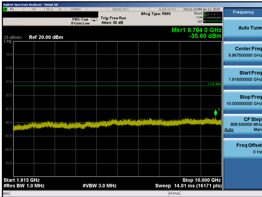
Plot 6-11. Conducted Spurious Plot (PCS GSM Mode – Ch. 810)
