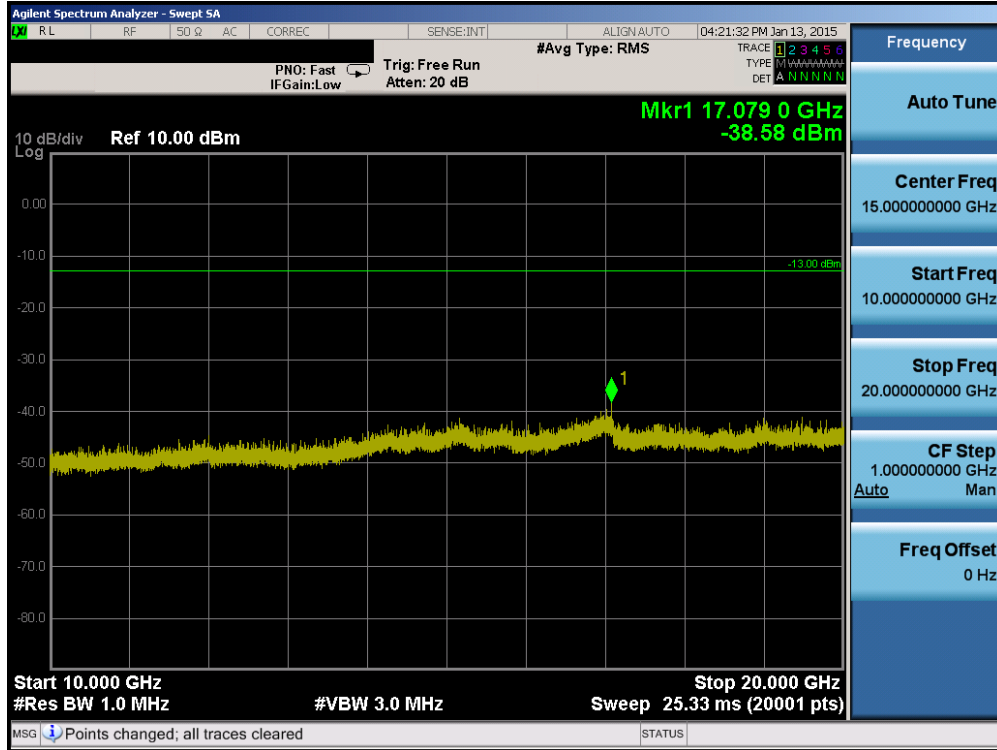
Plot 6-12. Conducted Spurious Plot (PCS GSM Mode – Ch. 810)
