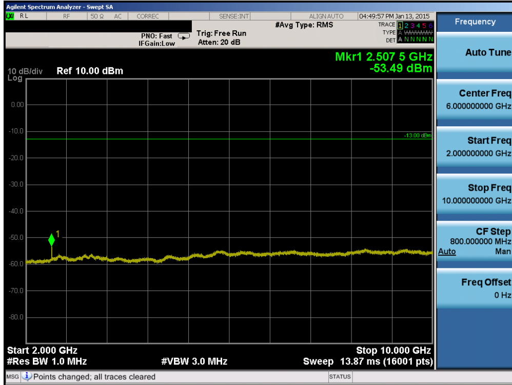
Plot 6-18. Conducted Spurious Plot (Cellular WCDMA Mode – Ch. 4183)
