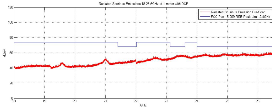
Plot 6-76. Radiated Spurious Plot above 18GHz (Pol. V)
