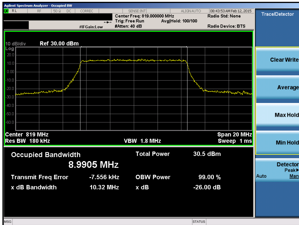
Plot 7-19. Occupied Bandwidth Plot (10MHz 16-QAM – RB Size 50)
