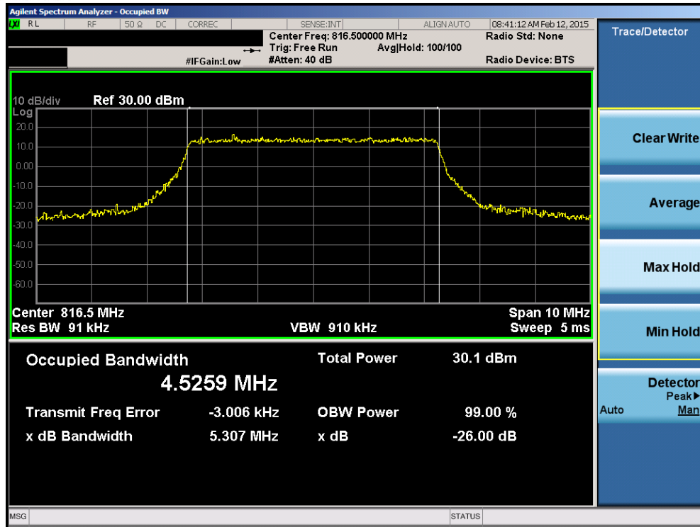
Plot 7-16. Occupied Bandwidth Plot (5MHz 16-QAM – RB Size 25– Low Channel)
