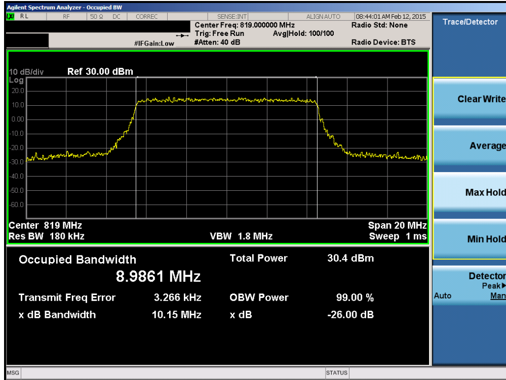
Plot 7-18. Occupied Bandwidth Plot (10MHz QPSK – RB Size 50)
