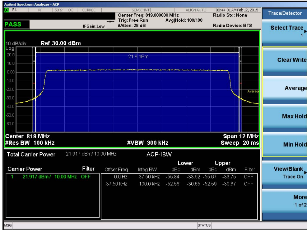
Plot 7-20. Channel Edge Plot (10MHz QPSK – RB Size 50)
