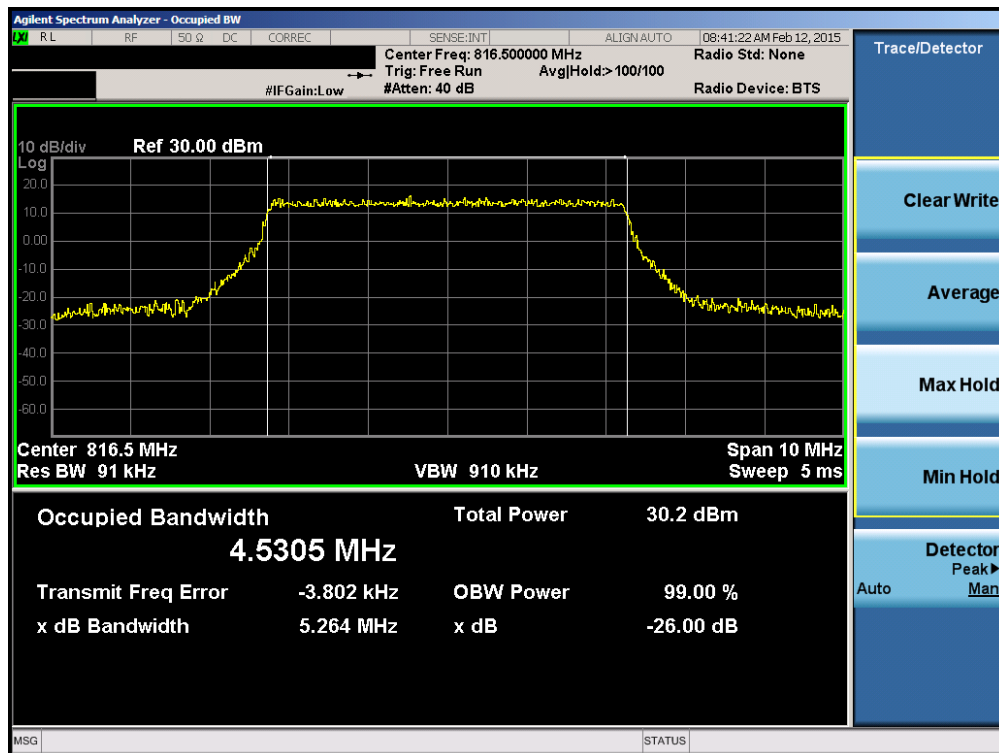
Plot 7-15. Occupied Bandwidth Plot (5MHz QPSK – RB Size 25– Low Channel)
