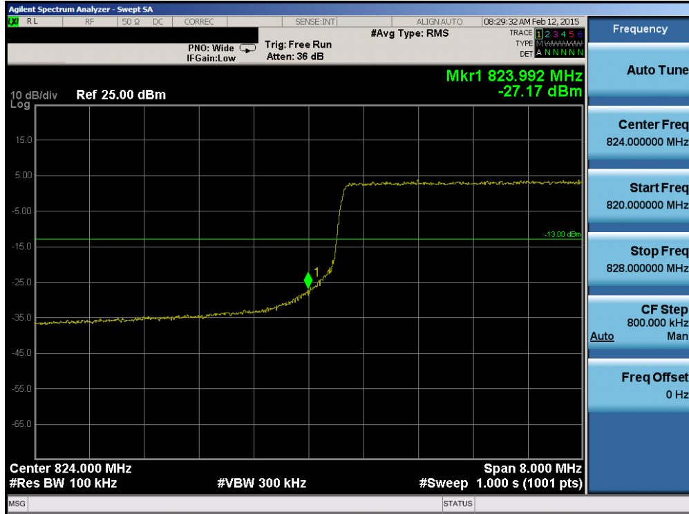
Plot 6-105. Lower Band Edge Plot (Band 26 – 10.0MHz QPSK – RB Size 50)
