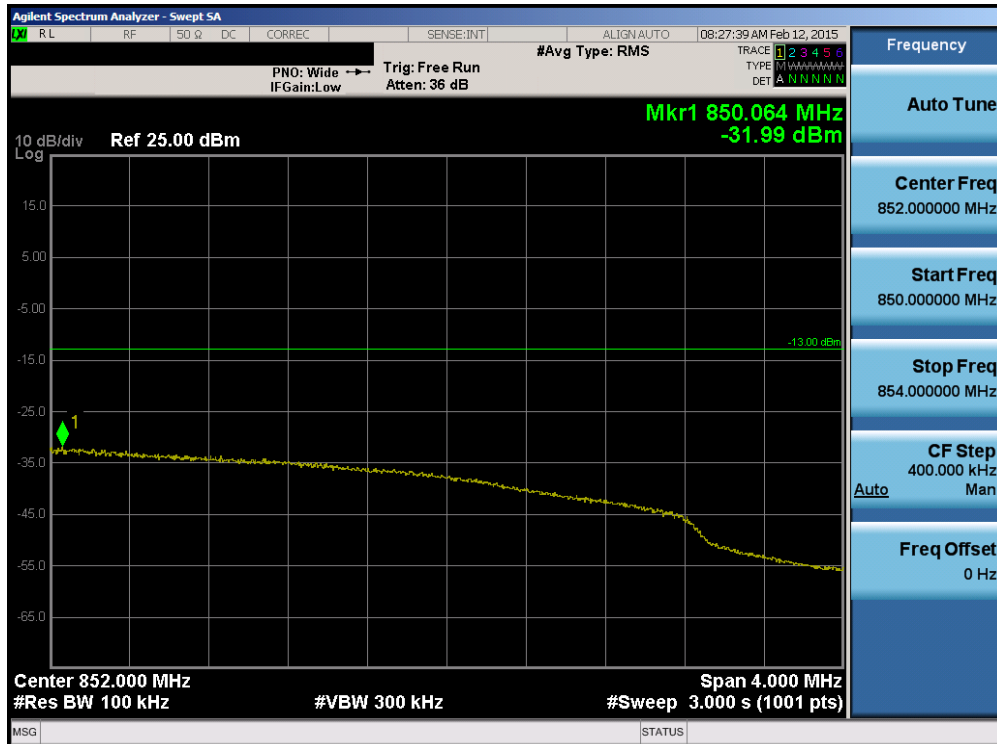
Plot 6-104. Upper Extended Band Edge Plot (Band 26 – 5.0MHz QPSK – RB Size 25)
