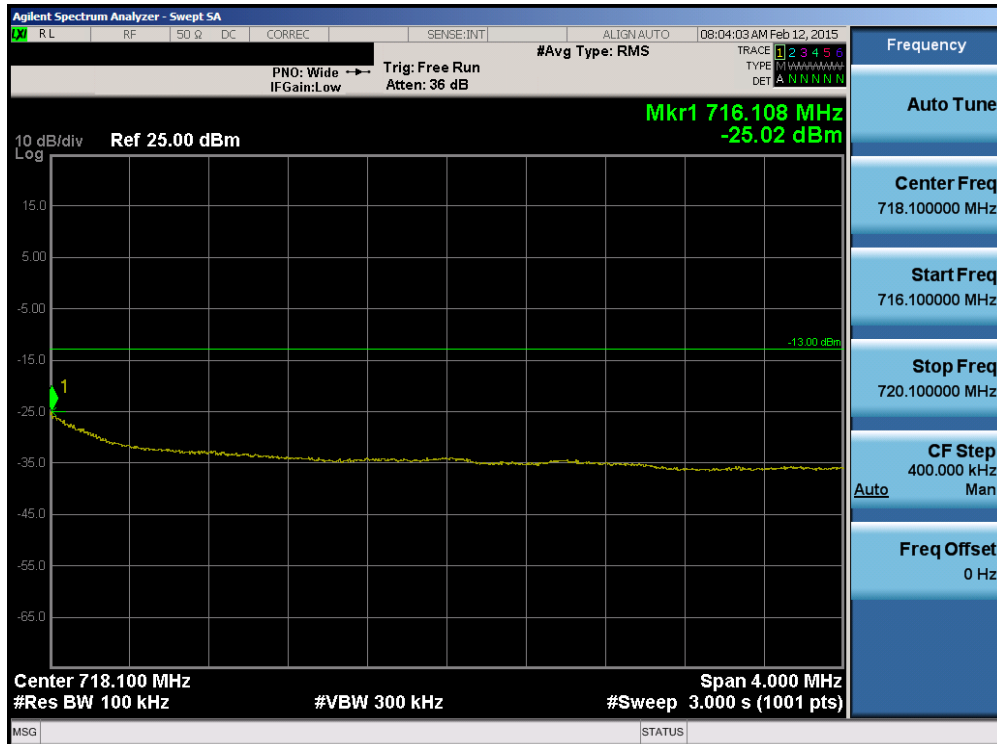
Plot 6-90. Upper Extended Band Edge Plot (Band 12 – 5.0MHz QPSK – RB Size 25)
