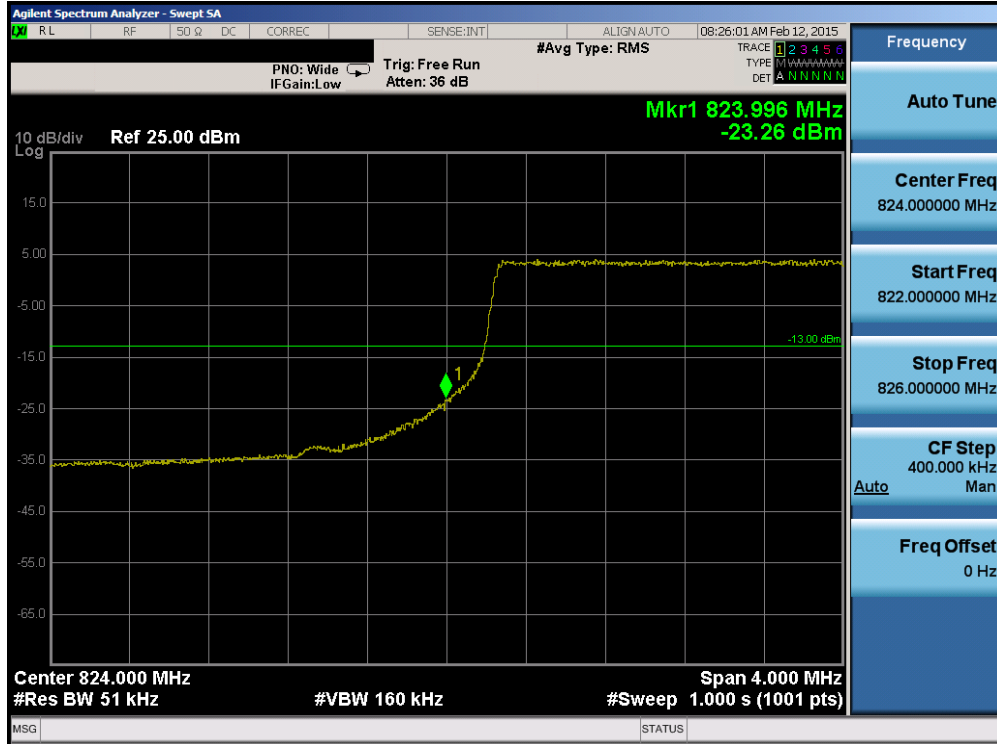
Plot 6-101. Lower Band Edge Plot (Band 26 – 5.0MHz QPSK – RB Size 25)
