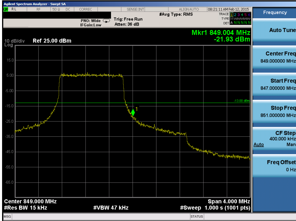
Plot 6-95. Upper Band Edge Plot (Band 26 – 1.4MHz QPSK – RB Size 6)
