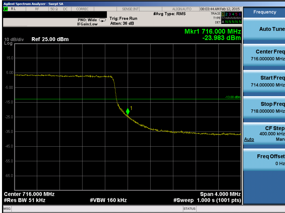
Plot 6-89. Upper Band Edge Plot (Band 12 – 5.0MHz QPSK – RB Size 25)
