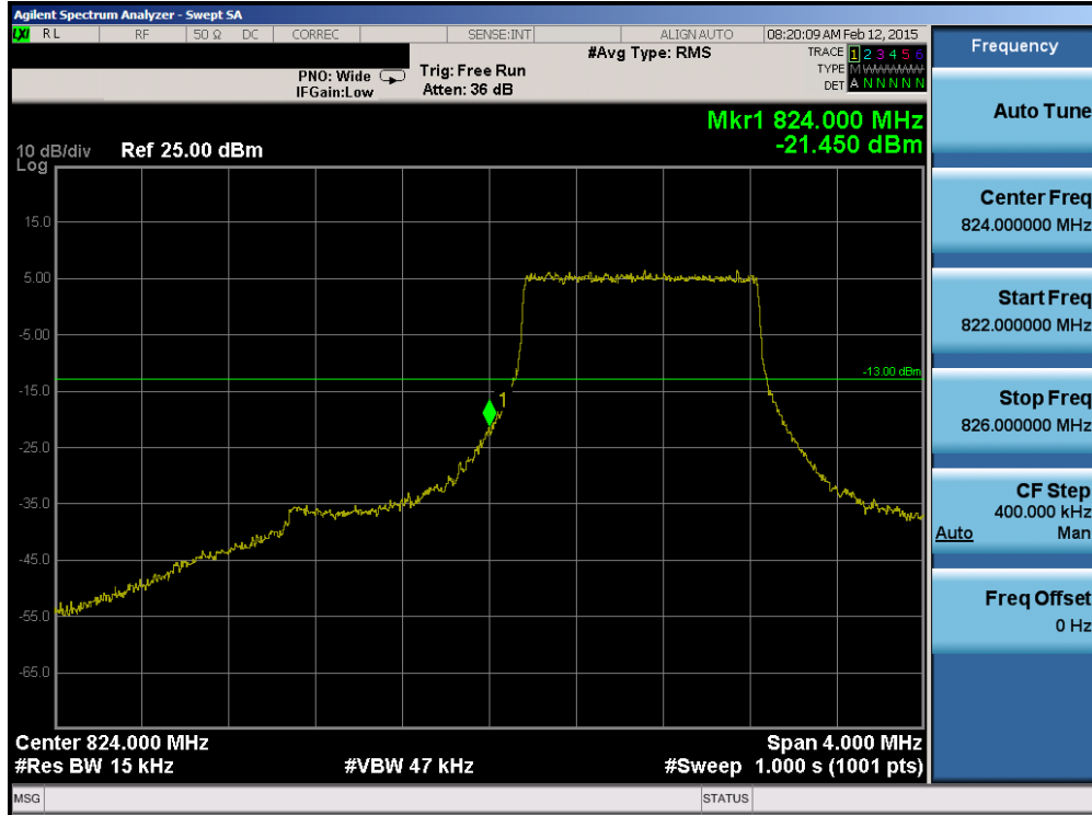
Plot 6-93. Lower Band Edge Plot (Band 26 – 1.4MHz QPSK – RB Size 6)
