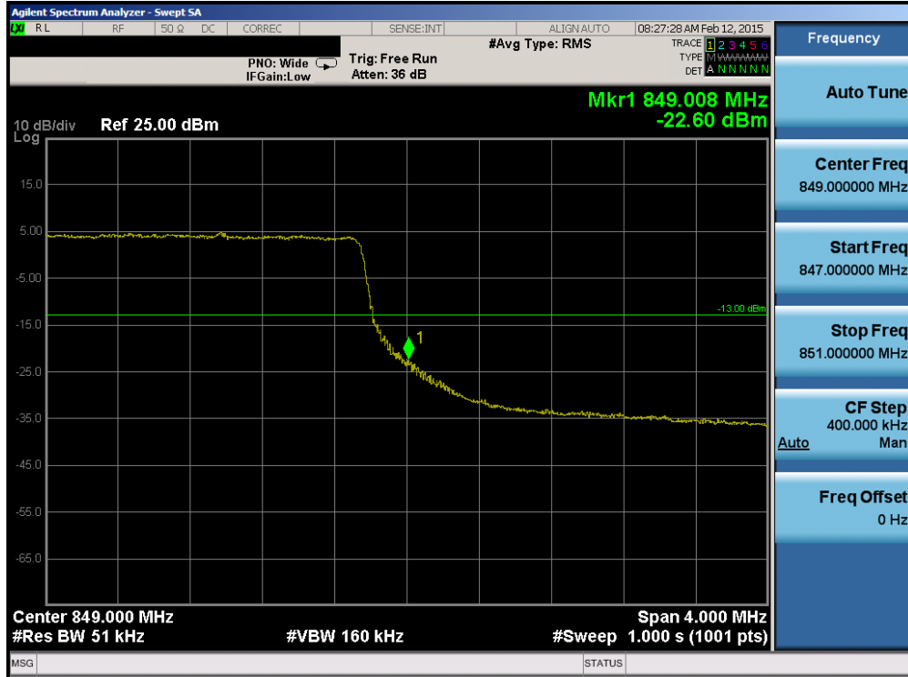
Plot 6-103. Upper Band Edge Plot (Band 26 – 5.0MHz QPSK – RB Size 25)
