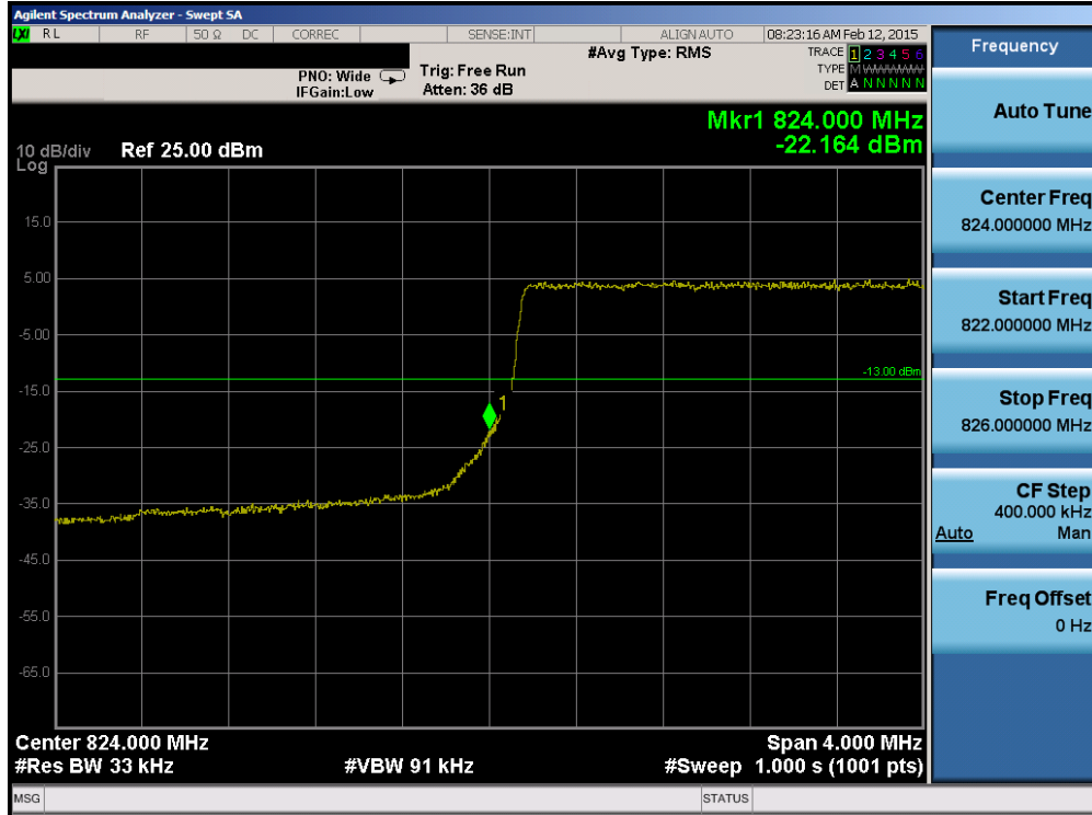
Plot 6-97. Lower Band Edge Plot (Band 26 – 3.0MHz QPSK – RB Size 15)
