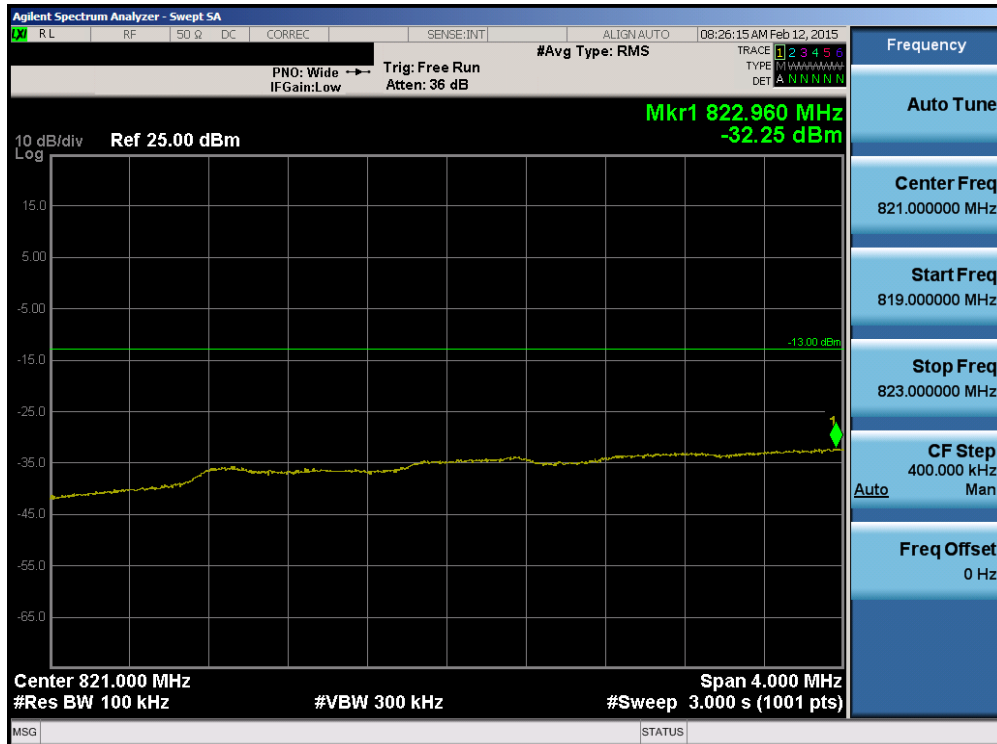
Plot 6-102. Lower Extended Band Edge Plot (Band 26 – 5.0MHz QPSK – RB Size 25)
