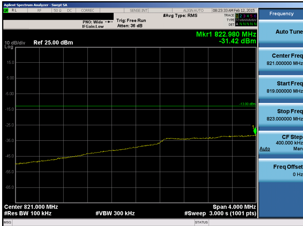
Plot 6-98. Lower Extended Band Edge Plot (Band 26 – 3.0MHz QPSK – RB Size 15)
