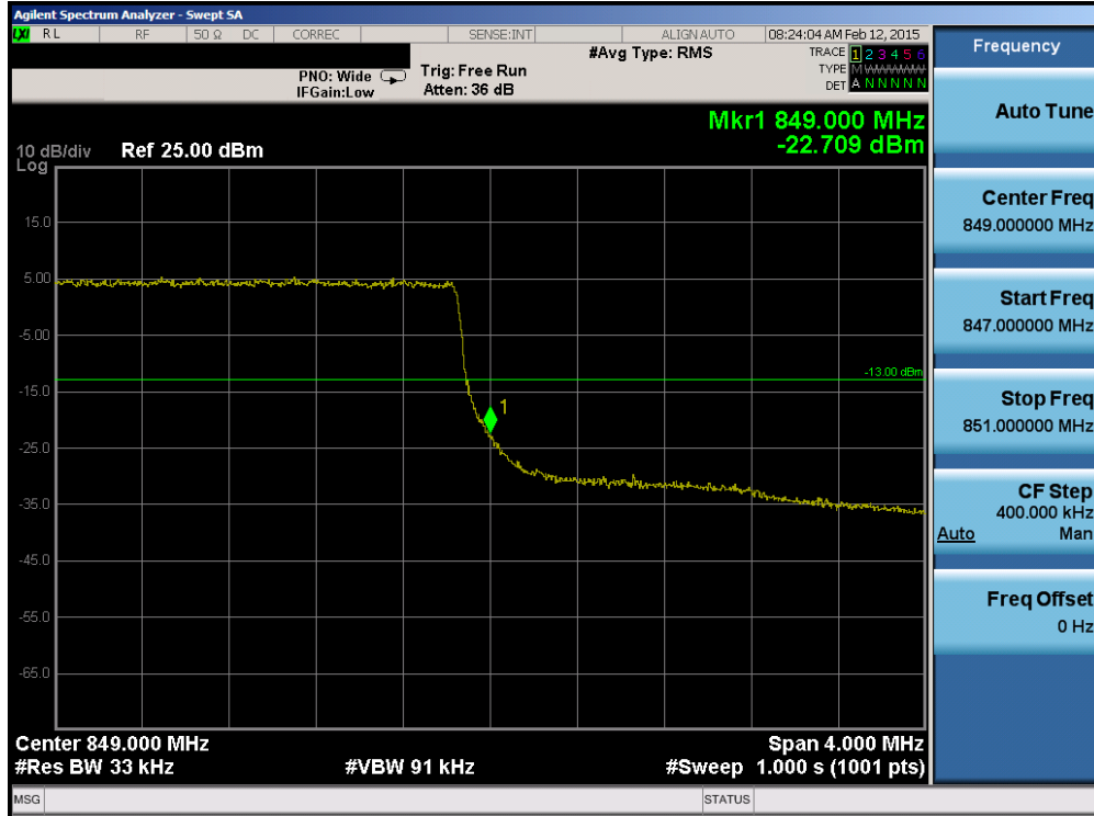
Plot 6-99. Upper Band Edge Plot (Band 26 – 3.0MHz QPSK – RB Size 15)
