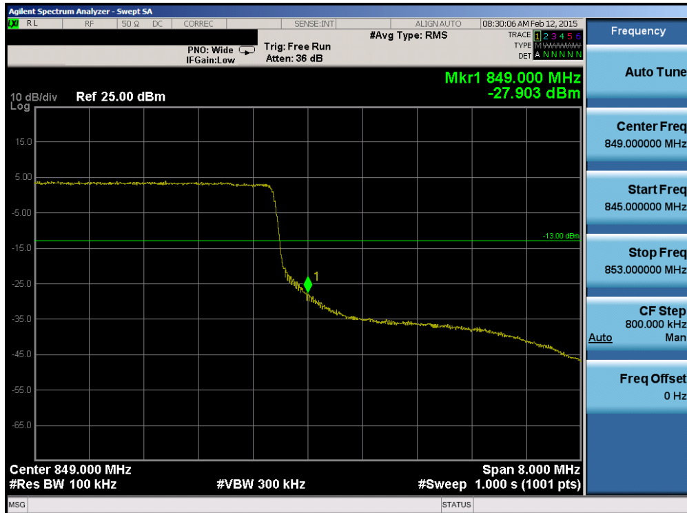
Plot 6-106. Upper Band Edge Plot (Band 26 – 10.0MHz QPSK – RB Size 50)
